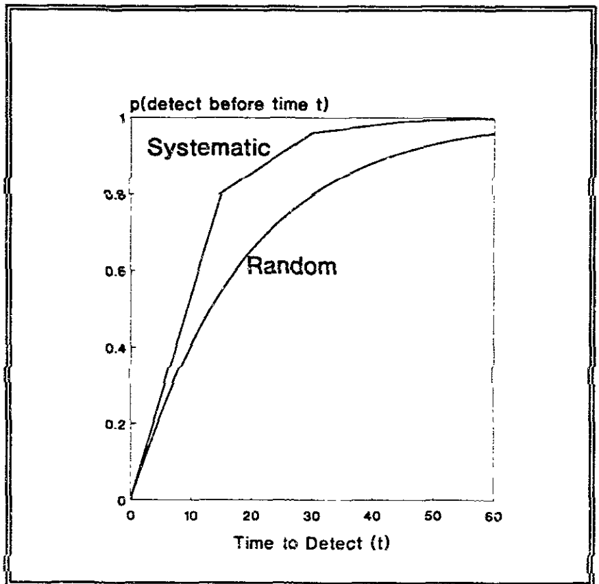
Figure 5.10 Typical Cumulative Search Time Distribution, Giving the SAOC for Visual Search
