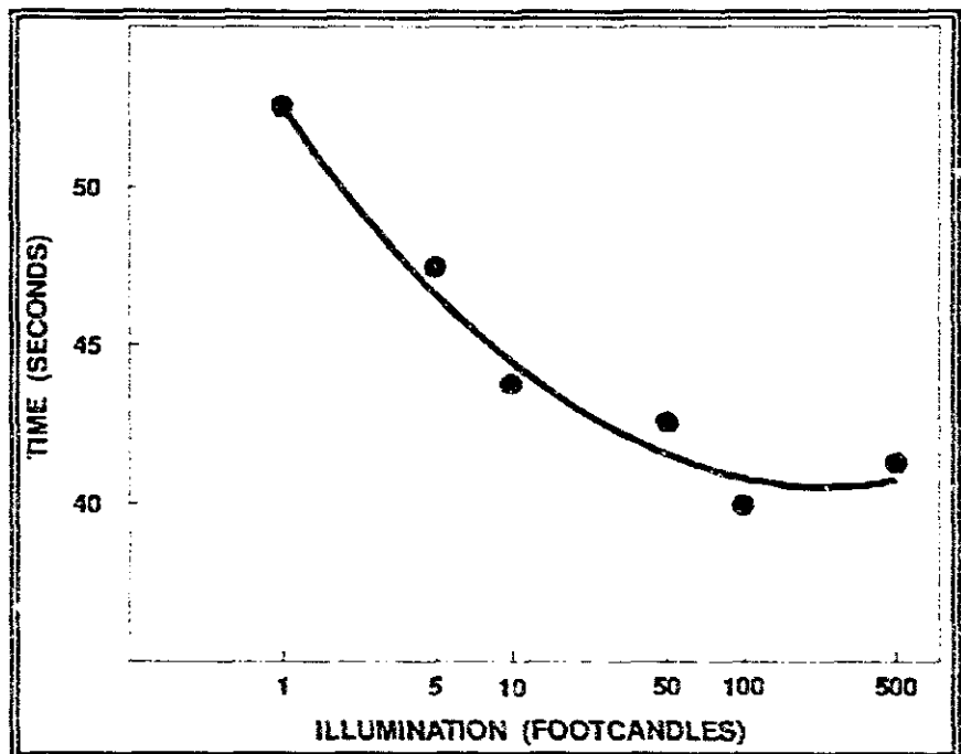
Figure 1 Effect of illumination level on time to complete a typical industrial task (micrometer reading). Adapted from Sanders and McCormick, 1987 .
