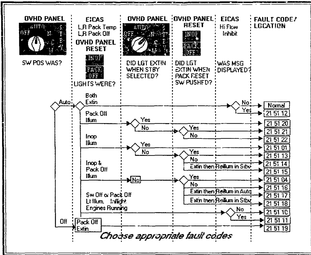
Figure 4.5 Fault Isolation Maintenance Manual
