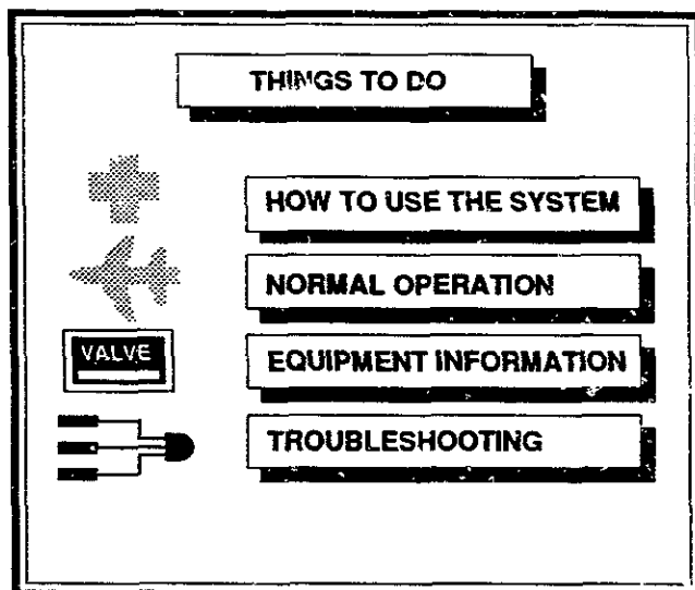
Figure 4.3 Menu Options
