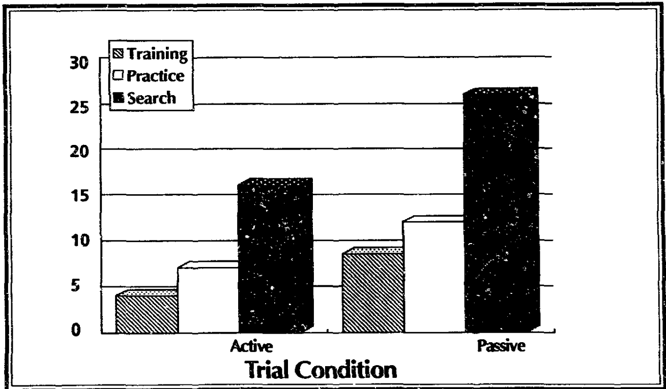
Figure 3.6 Training Condition
