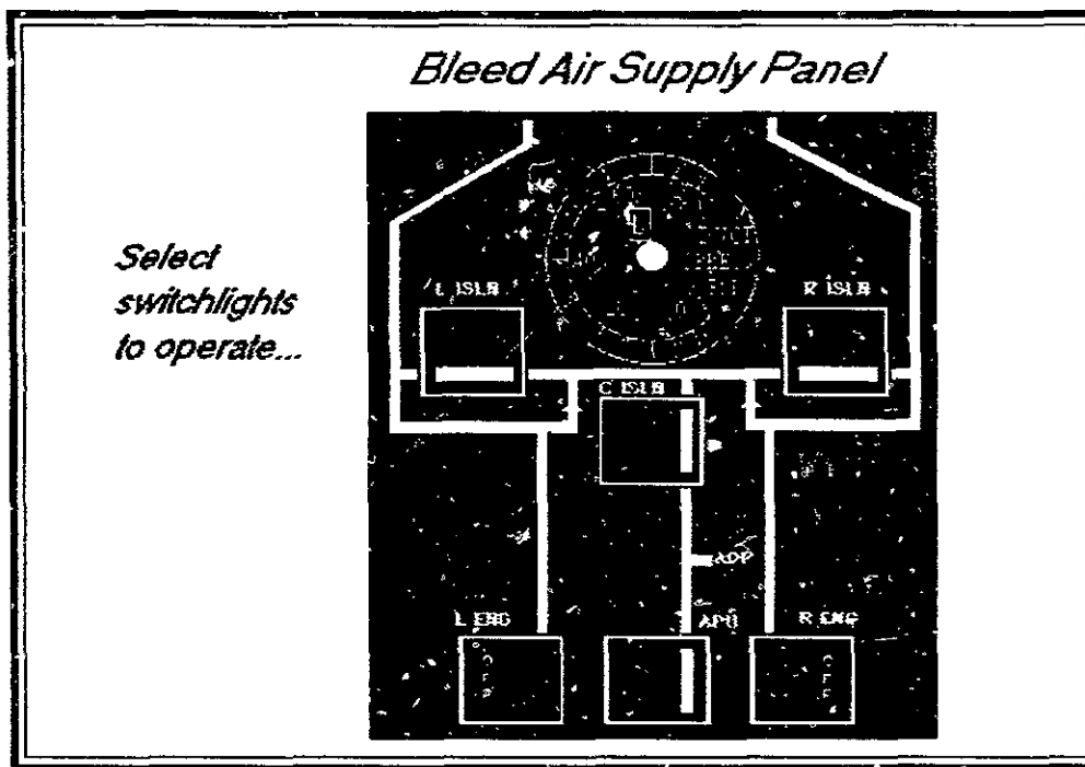
Figure 4.4 Bleed Air Supply Panel
