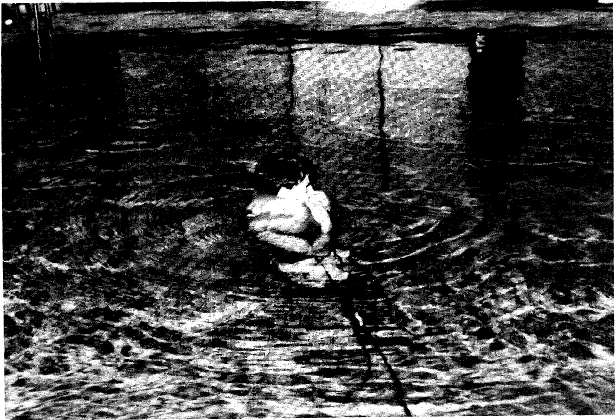
Figure 9. Subject demonstrating a face-up flotation position while wearing the prototype life preserver.
