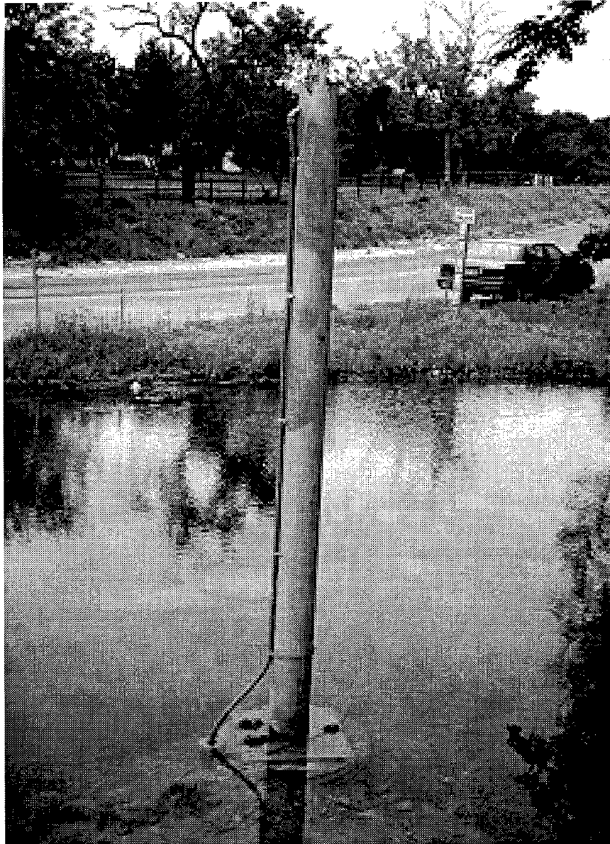
Figure 3.4 Water-level sensor
