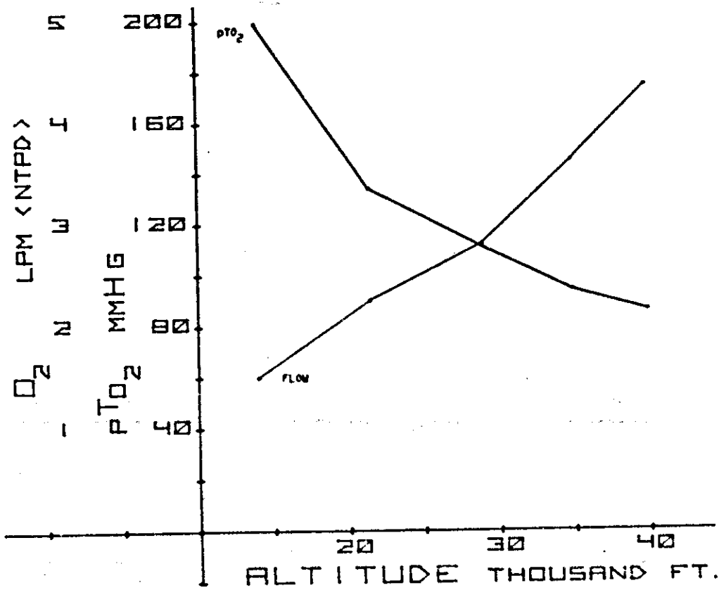
FIGURE 2. Tracheal oxygen partial pressure following 3 min of exercise at the indicated minimum oxygen flow rates.
