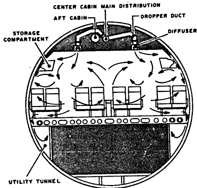
FIGURE 3. Cabin air circulation and exhaust diagram.
