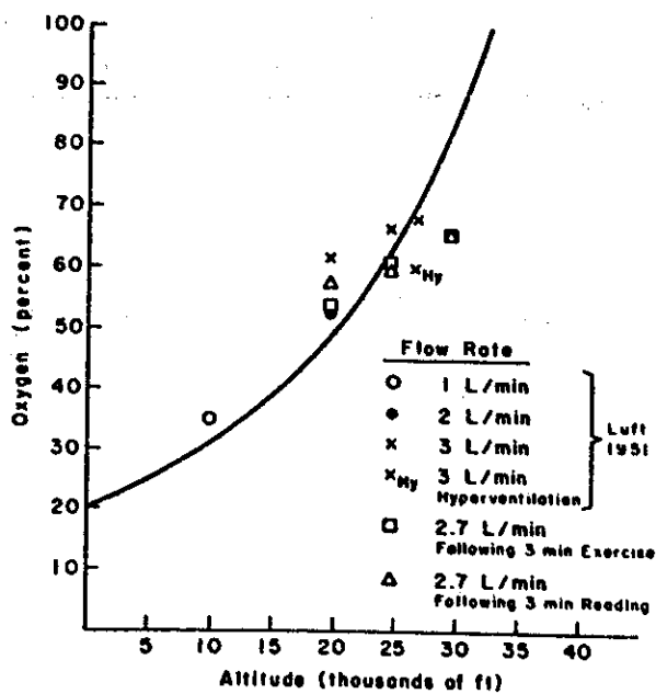
FIGURE 8. Concentration of inspired gas using the Cessna mask superimposed over Luft's plot of the K-S mask in 1951. Oxygen flow controlled by a Zep-Aro orifice F 365-1080-2 with a flow of 2.7 L/min at a pressure of 70 psi. Curve represents inspired oxygen required to theoretically maintain sea-level conditions.
