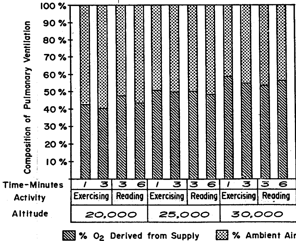
FIGURE 6. Histogram showing dilution of inspired gas with ambient air as calculated from the end expiratory nitrogen concentration. Subjects exercising and reading at 20,000, 25,000, and 30,000 feet while wearing the Cessna mask.
