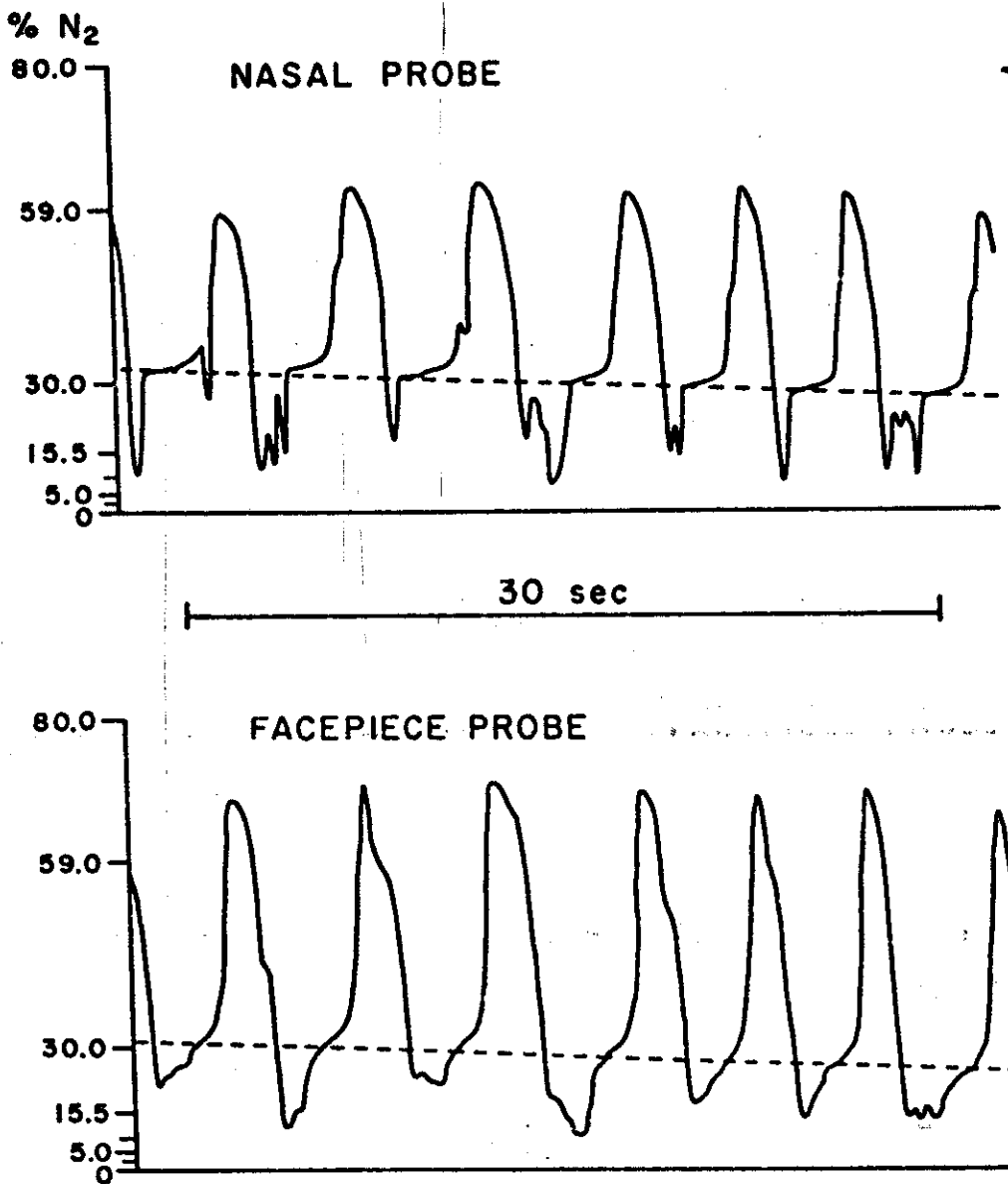
FIGURE 4. Simultaneous measurement of nitrogen by probes inserted in nostril and the Cessna mask facepiece. A dashed line is drawn through the end expiratory points. Subject DD. First minute of exercise at 30,000 feet. The slope indicates the increase in end expiratory nitrogen during transition from resting to exercise. Recording must be read from right to left.
