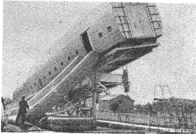
Figure 2. The evacuation simulator positioned 12^{\circ} nose down and in a 12^{\circ} left roll as in an emergency landing with nose gear and left main gear failure.
