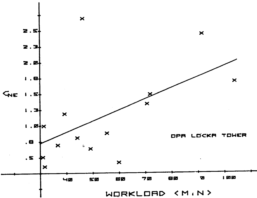
FIGURE 6. Relationship between c_e and workload represented by minutes of radio communication time.
