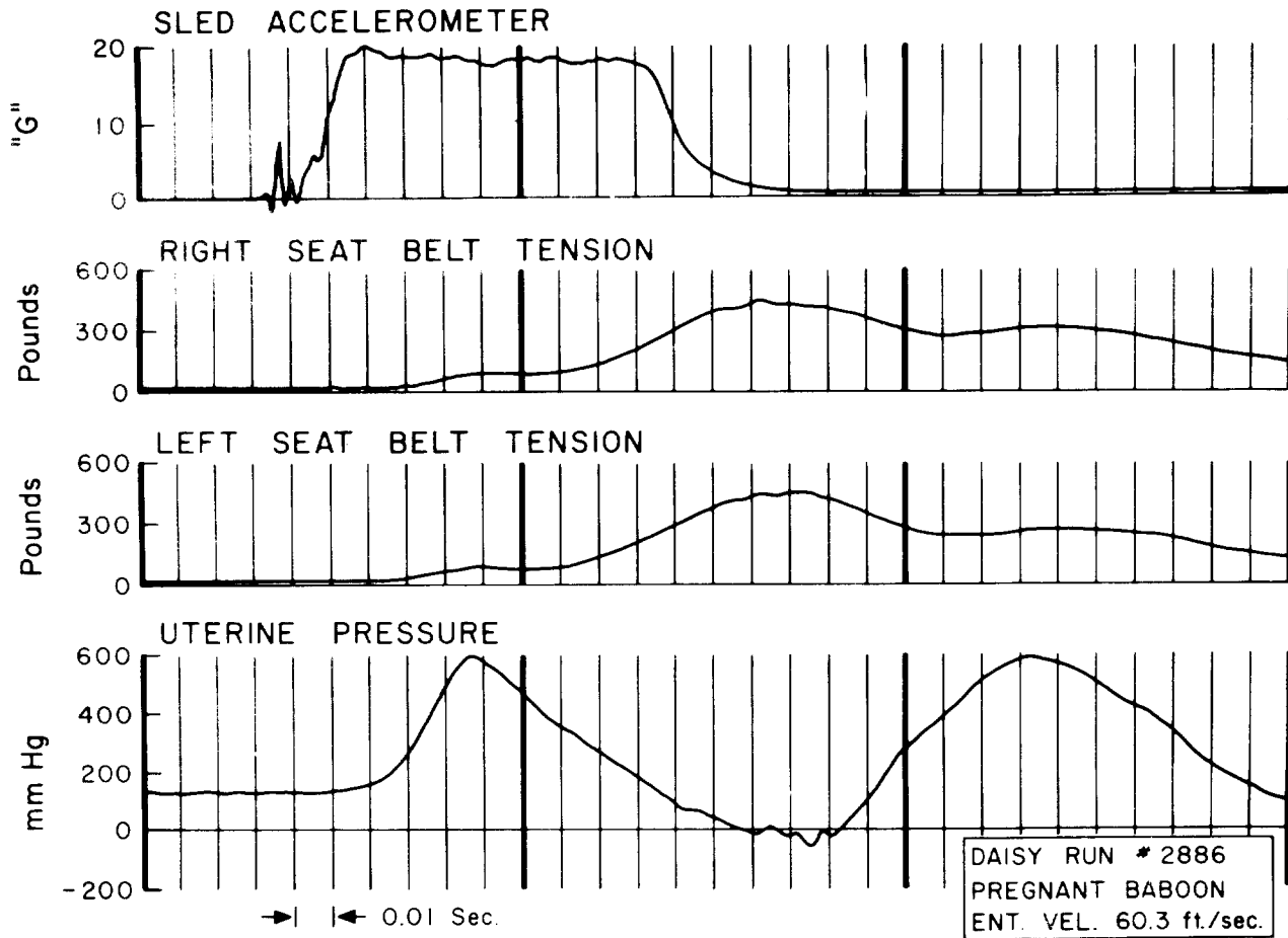
FIGURE 6. Results of impact test No. A-4 (Daisy Run No. 2886).
