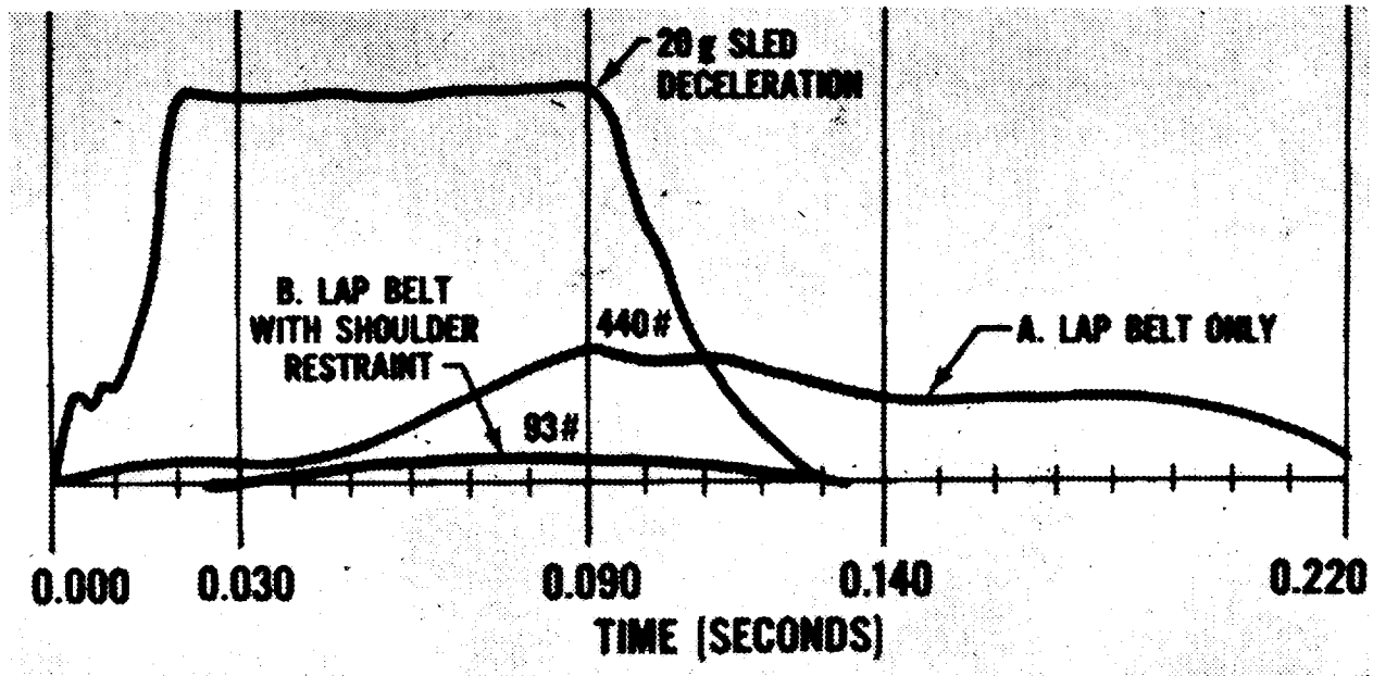
FIGURE 8. Comparison of lap belt with lap belt plus shoulder restraint.
