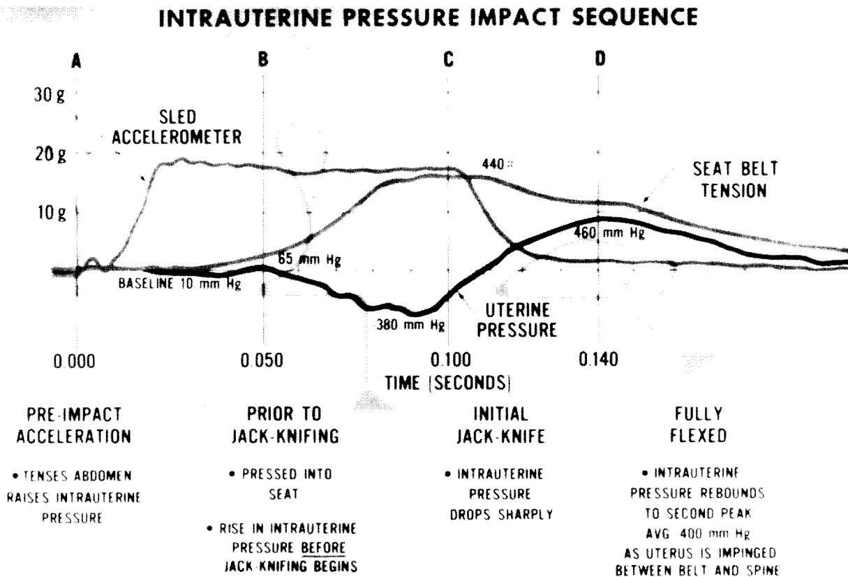
FIGURE 9. Intrauterine pressure impact sequence.
