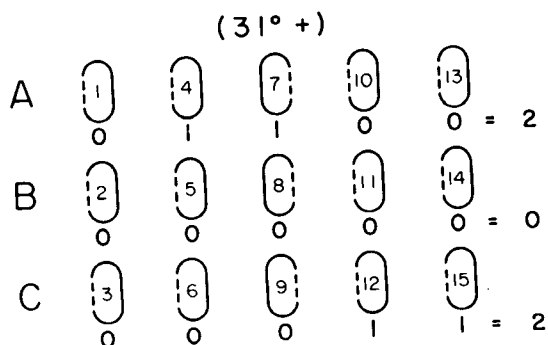
FIGURE 16. Number of heading variation events in excess of 10 degrees during flight on outbound leg is shown on the right. The least number of deviation events occurred in Mode B (peripheral cues added to normal instrument display).
