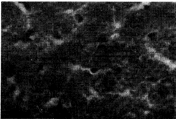
FIGURE 5. Rat 5. Modified Weil. There is little differentiation and stain is quite uniform.
