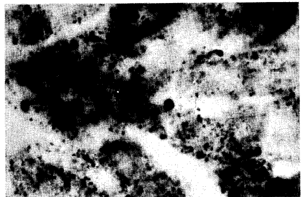
FIGURE 3. Rat 5. Powers' Marchi. Portal canal to left. The fat is in small droplets. The centrolobular areas were free of fat. 700x
