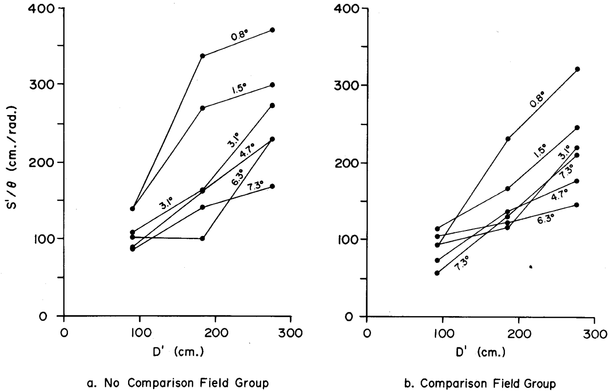
FIGURE 2. The relation between perceived size S' (per unit of retinal size \theta ) and perceived distance D' , for two groups of O 's in the first set of dynamic situations.
