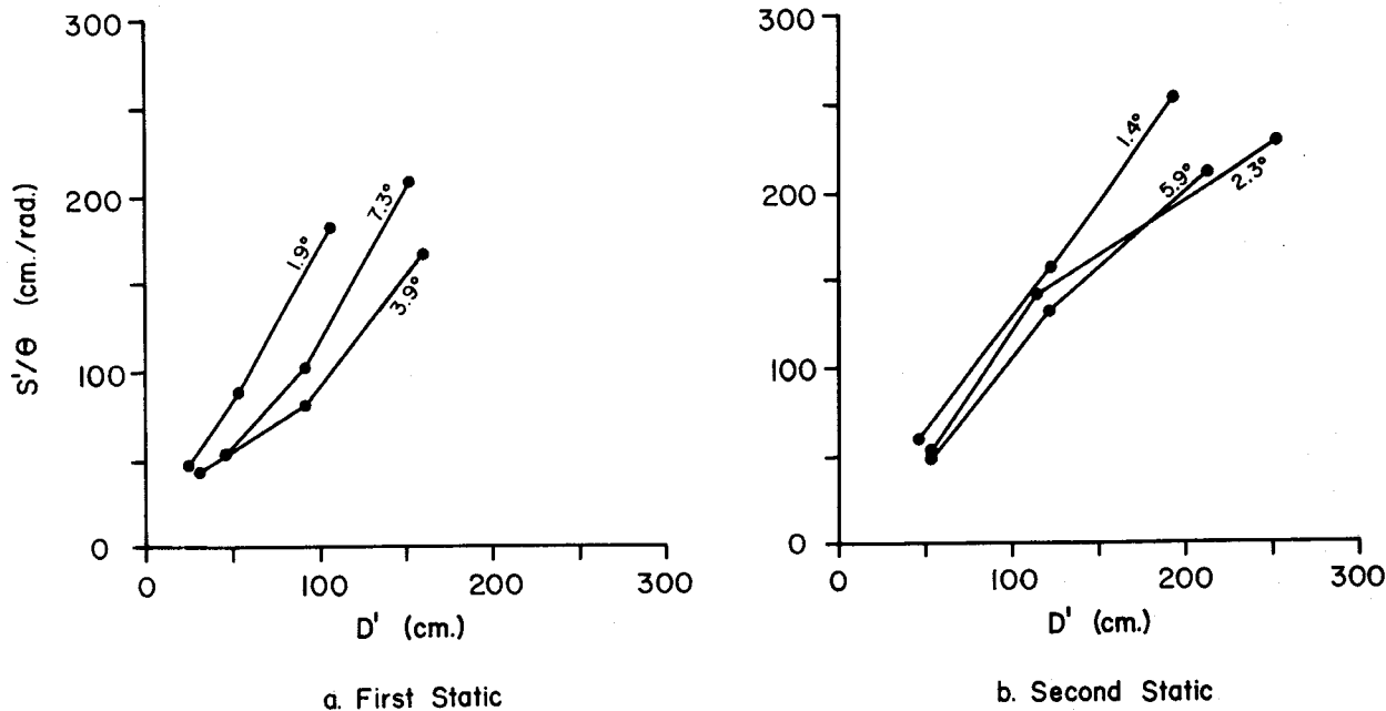
FIGURE 3. The relation between perceived size S' (per unit of retinal size \theta ) and perceived distance D' , for the first and second set of static situations.
