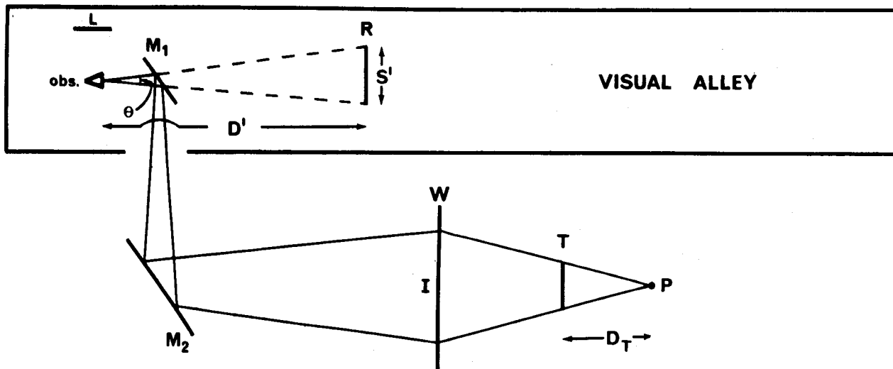
FIGURE 1. A top-view schematic drawing of the apparatus and visual alley.
