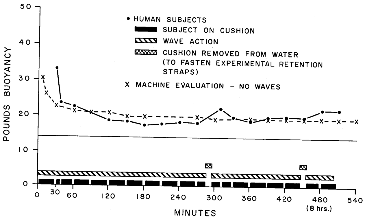
FIGURE A12. Dynamic seat-cushion evaluation conducted in February 1965 in the survival tank. B. F. Goodrich multifoam crew seat cushion. Blue-canvas stitched unsealed cover. Waves 2 to 2½ feet in height.
