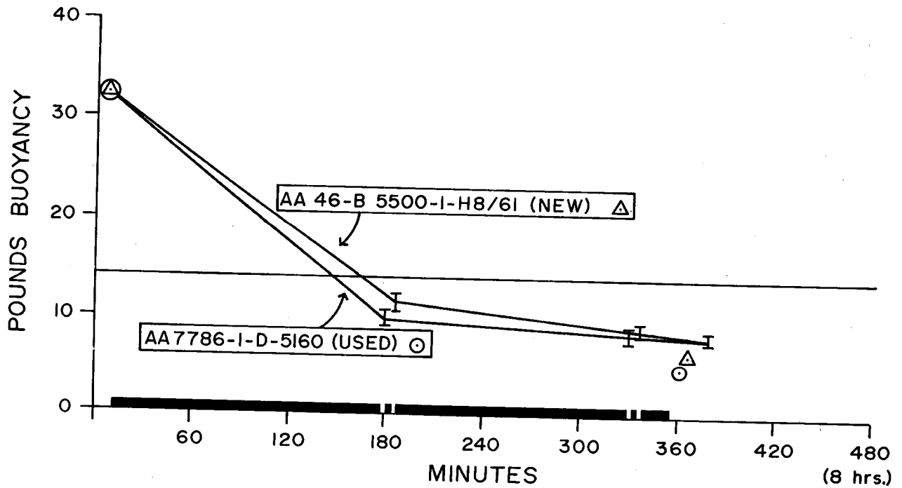
FIGURE A4. Dynamic seat-cushion test conducted on January 8, 1964, in CARI survival tank. Technique same as Figure 3. Lower horizontal portion of bracket \perp indicates weight cushion supported. Upper \top indicates the weight that caused failure (sinking) of cushion. Both cushions tested simultaneously. Subjects were relieved hourly by new subjects during the test. Bar at lower edge of graph indicates time cushion in water and being used for flotation by subjects.
