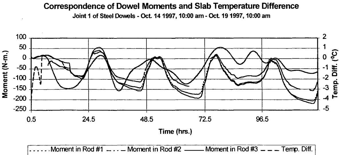
Figure 5.1 – Initial Steel Dowel Environmental Moment Data
