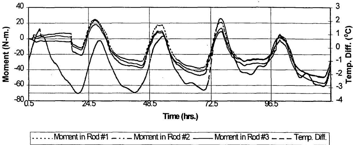
Figure 5.2– Initial Fiberglass Dowel Environmental Moment Data
