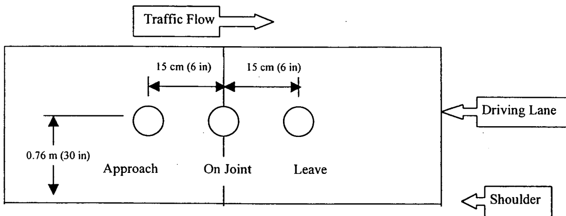
Figure 5.3 – Locations of FWD Load Plates
