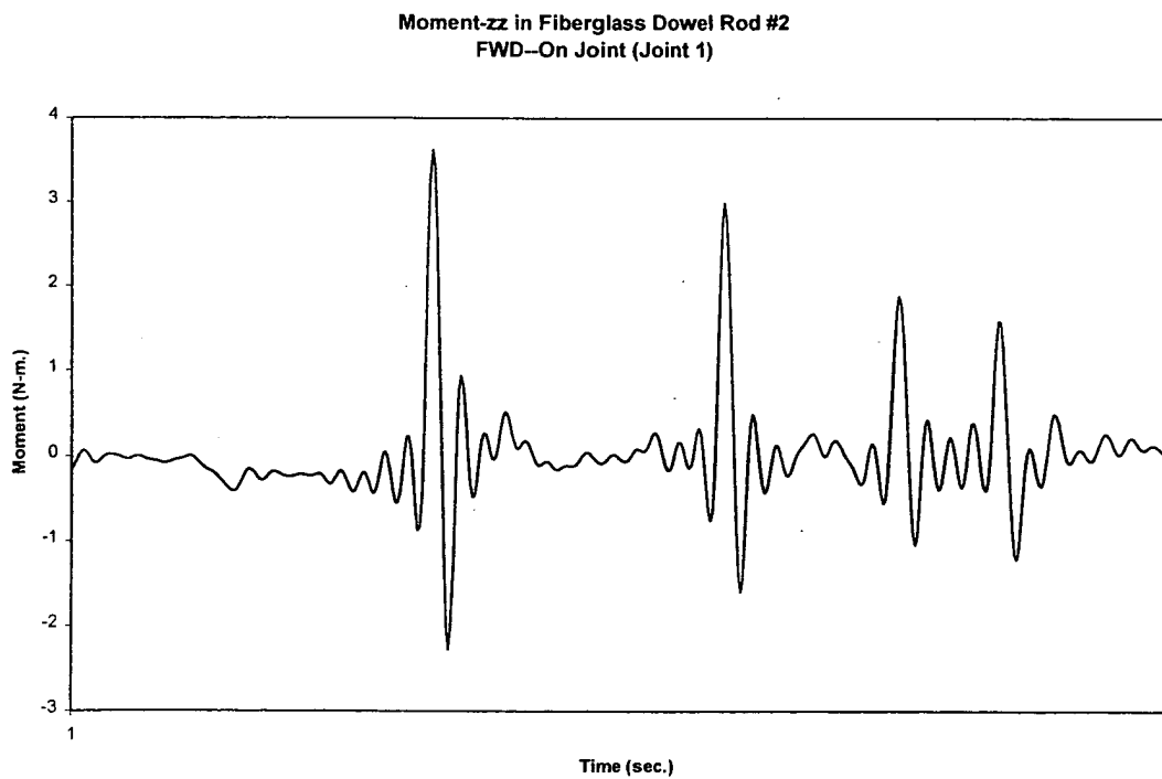
Figure 5.5 – Typical Fiberglass Dowel FWD Moment Data
