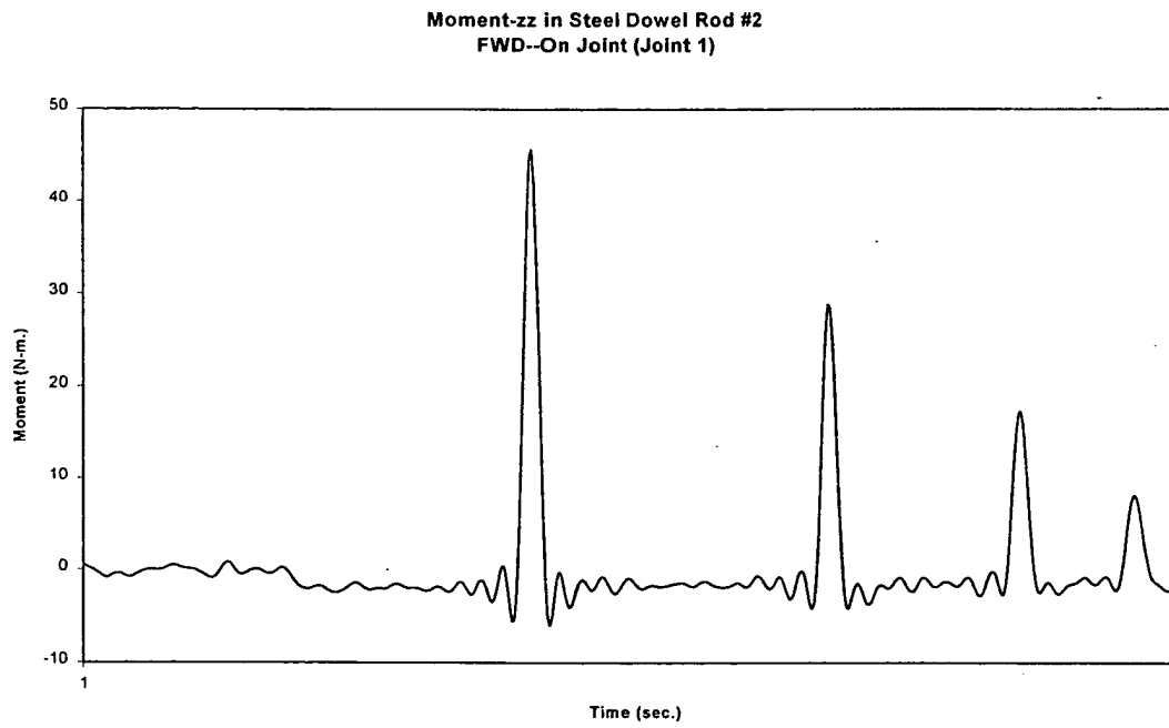
Figure 5.4 – Typical Steel Dowel FWD Moment Data
