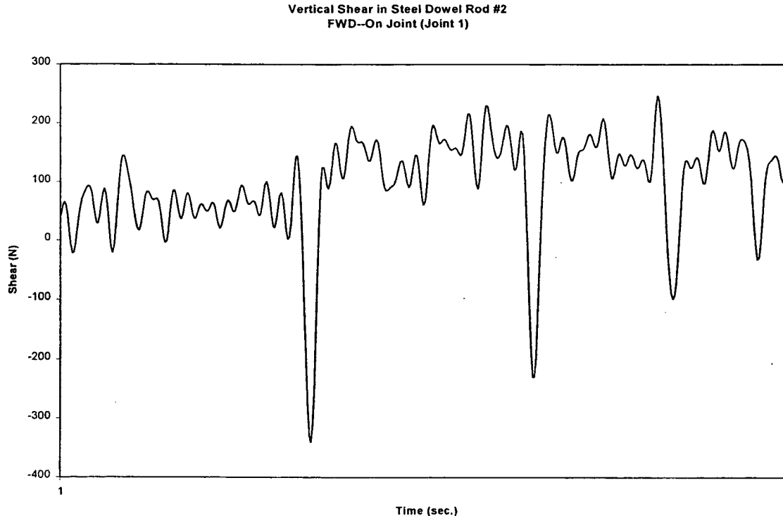
Figure 5.6 – Typical Steel Dowel FWD Shear Data
