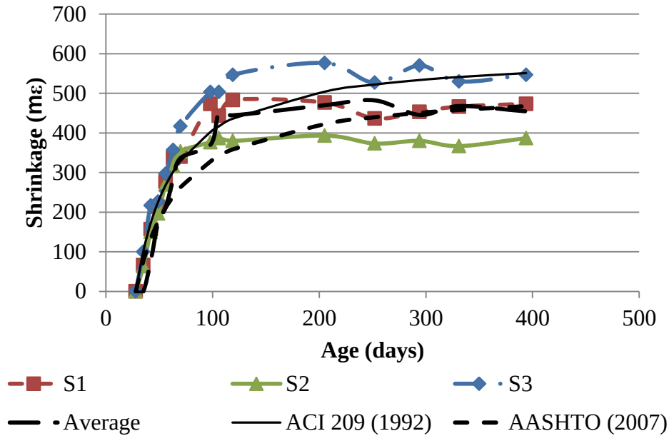
Figure 3-1: Shrinkage strains from sampled concrete batches under standard curing
