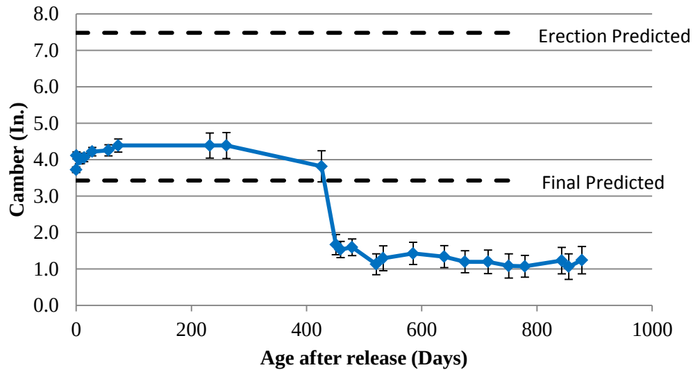
Figure 6-3: Comparison of predicted and measured camber (1 in. = 2.54 cm)
