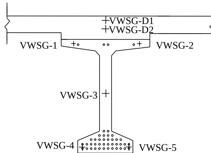
Figure 1-4: Instrumentation of girder and bridge deck
