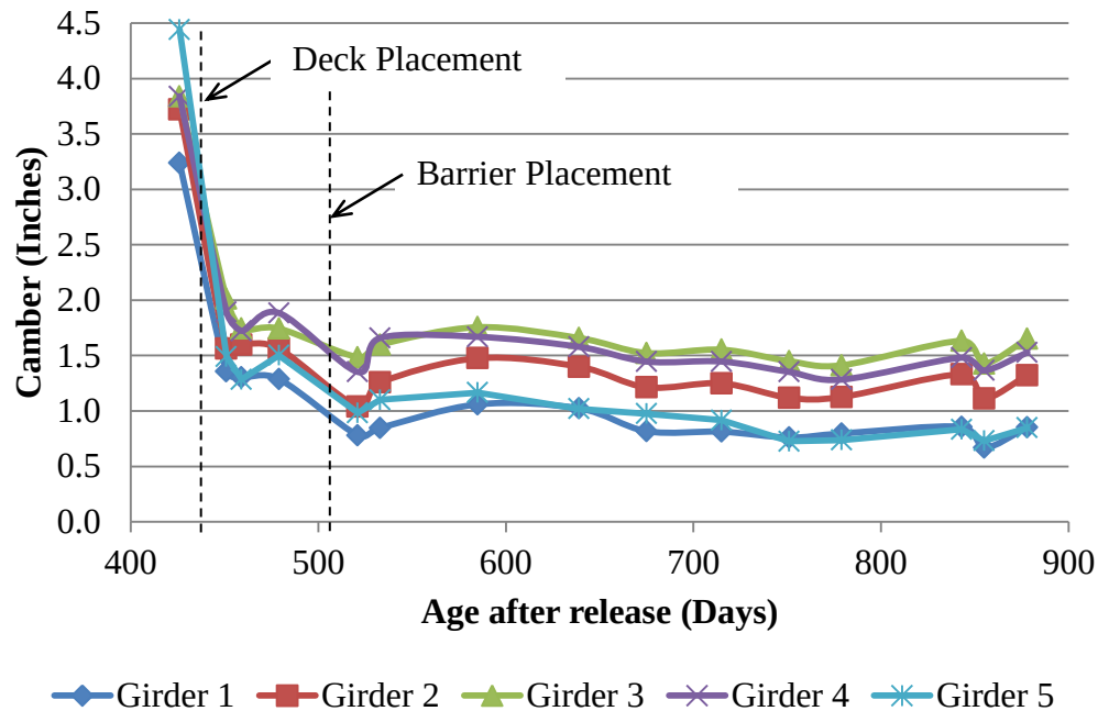
Figure 6-2: Observed camber after deck placement (1in = 2.54cm)
