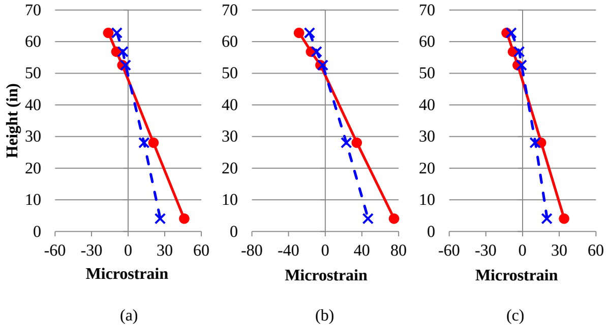
Figure 4-14: Strain profiles of girder 4 due to (a) LT1, (b) LT2, and (c) LT3 (1 in. = 2.54 cm)
