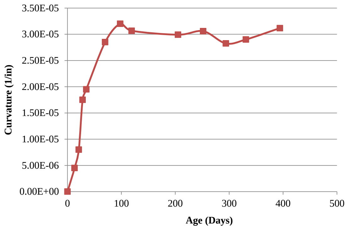
Figure 3-5: Curvature of slab specimens due to shrinkage (1 in. = 2.54 cm)
