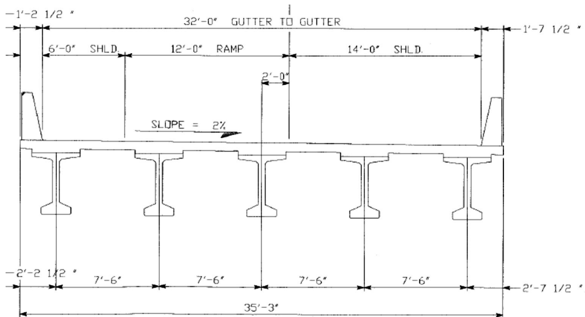
Figure 1-3. Bridge cross section showing all 5 girders.
