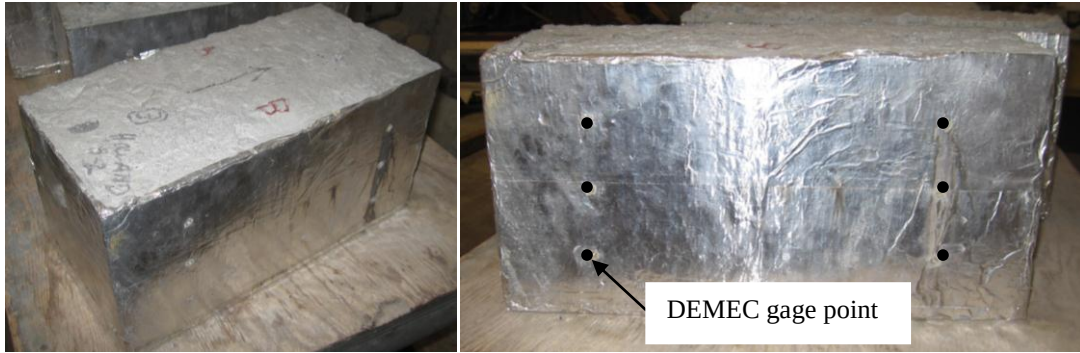
Figure 3-3: Slab shrinkage specimen and gage point locations
