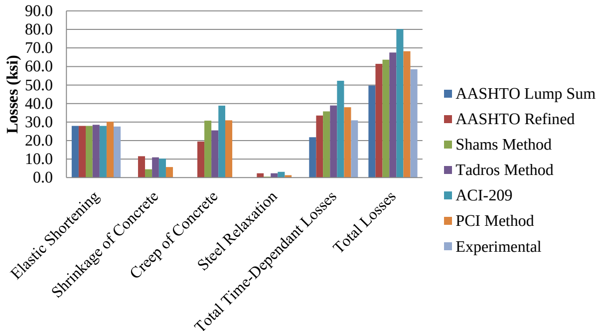
Figure 5-3: Comparison between estimation methods and measured values for losses by type (1ksi = 6.895MPa)
