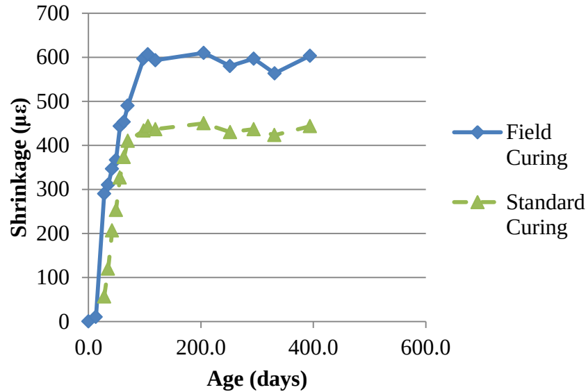
Figure 3-2: Shrinkage strains of field cured and standard cured samples
