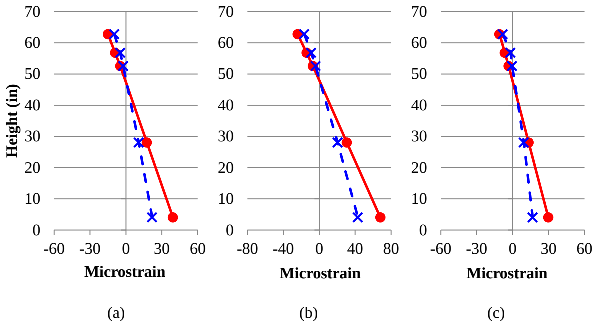
Figure 4-12: Strain profiles of girder 2 due to (a) LT1, (b) LT2, and (c) LT3 (1 in. = 2.54 cm)
