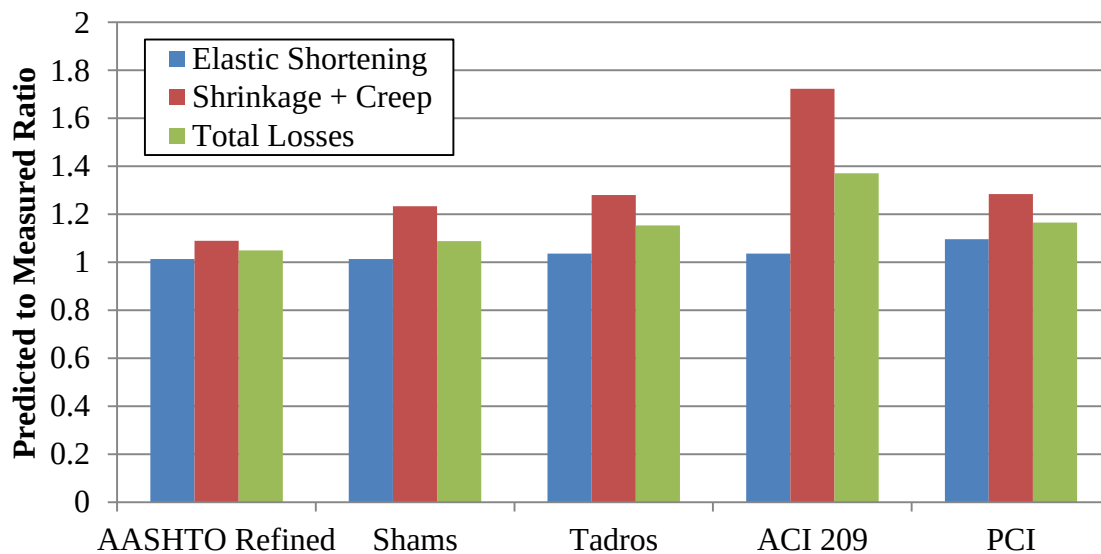
Figure 5-4: Comparison of predicted to measured ratios for loss types
