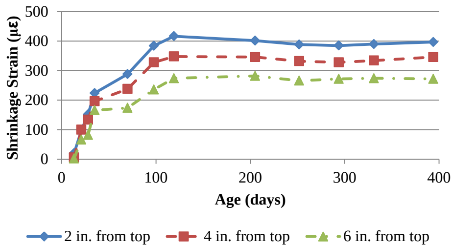
Figure 3-4: Shrinkage strains at depths into slab specimens
