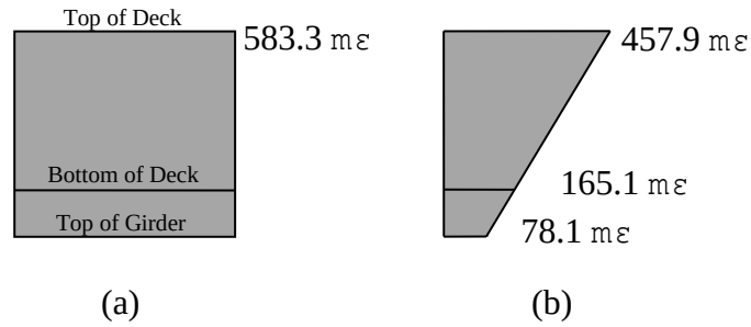
Figure 6-4: Shrinkage gradients for (a) uniform, and (b) linear gradient
