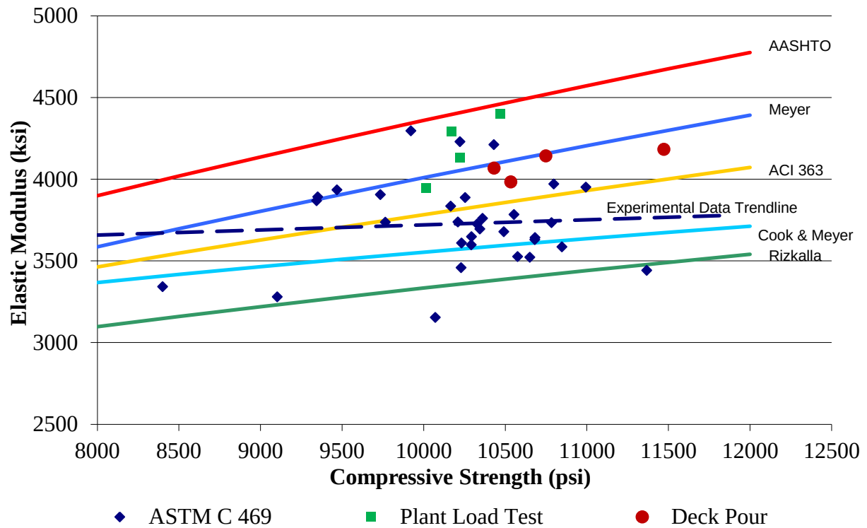
Figure 2-3: HSLW cylinder data comparison with estimator equations, (1 psi = 6.89 kPa)
