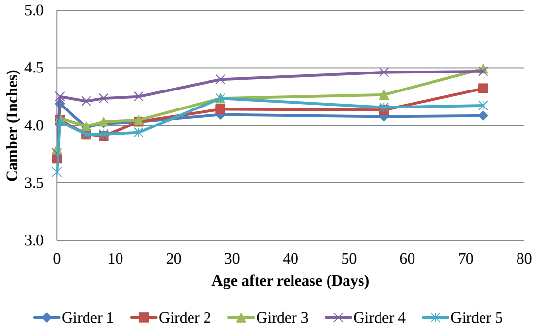
Figure 6-1: Observed camber before deck placement (1in = 2.54cm)
