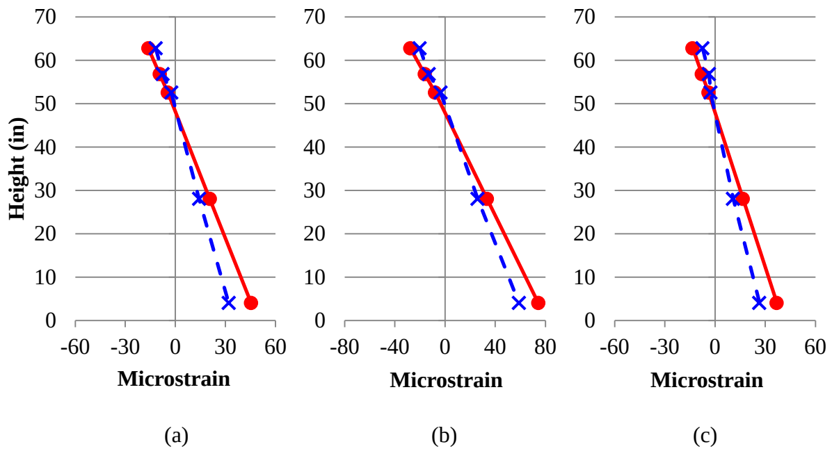
Figure 4-15: Strain profiles of girder 5 due to (a) LT1, (b) LT2, and (c) LT3 (1 in. = 2.54 cm)
