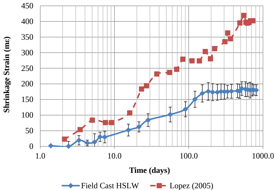
Figure 2-6: Average shrinkage of HSLW
