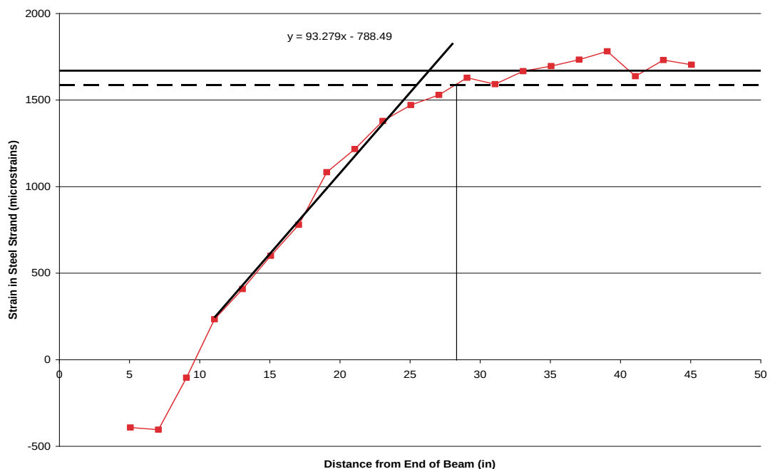
Figure D-5: Smoothed CSS readings for the South end of Girder 1 at day 8.
