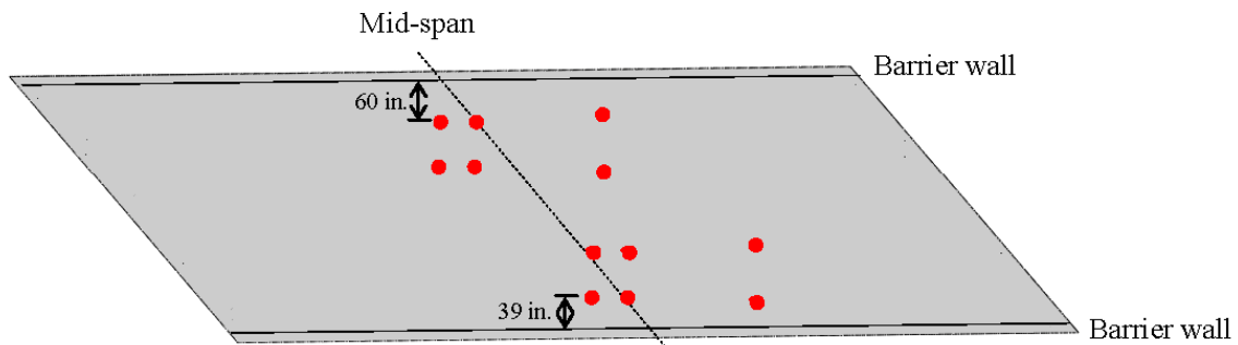
Figure 4-3: Truck positions during LT2 (1 in. = 2.54 cm)
