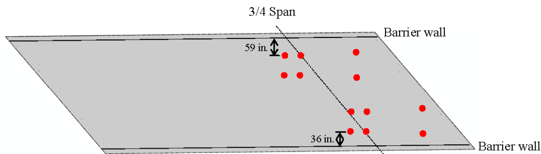
Figure 4-4: Truck positions during LT3 (1in. = 2.54 cm)
