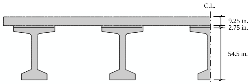
(c) Cross-section of the bridge model
