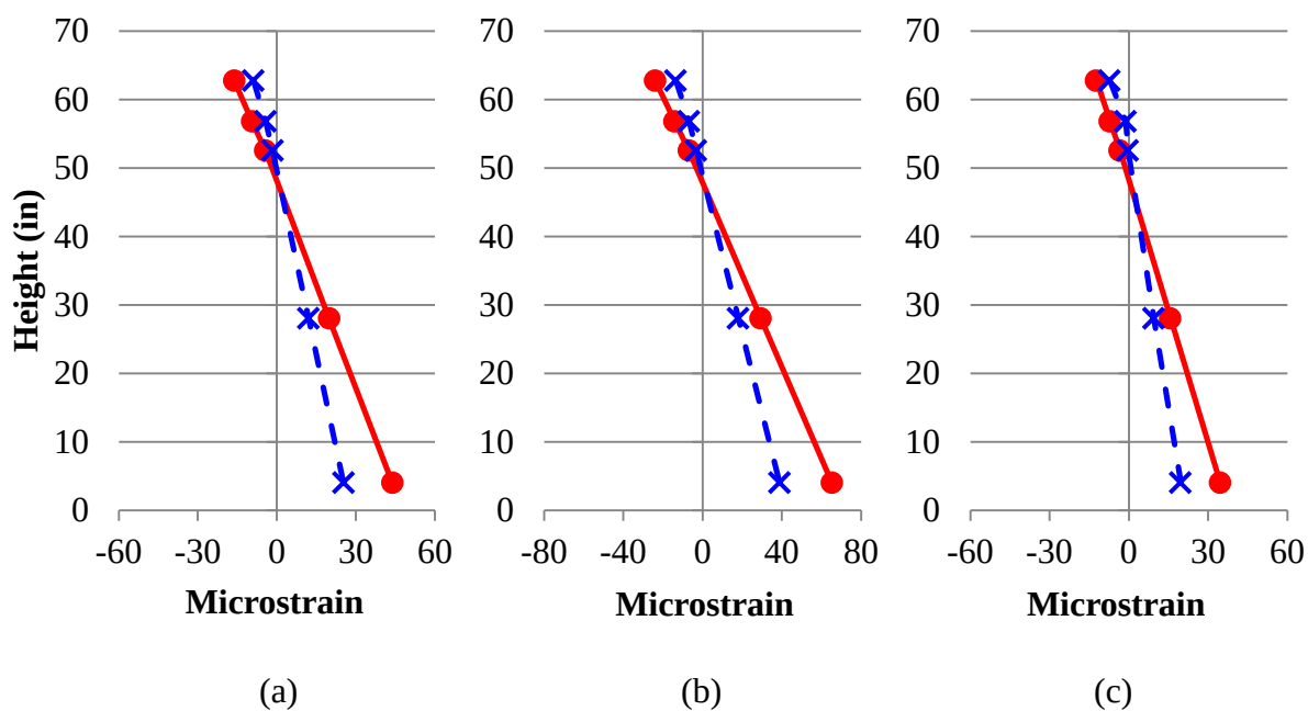
Figure 4-13: Strain profiles of girder 3 due to (a) LT1, (b) LT2, and (c) LT3 (1 in. = 2.54 cm)
