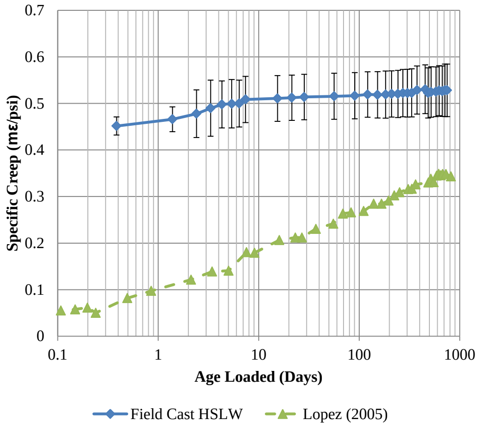
Figure 2-7: Specific creep of HSLW
