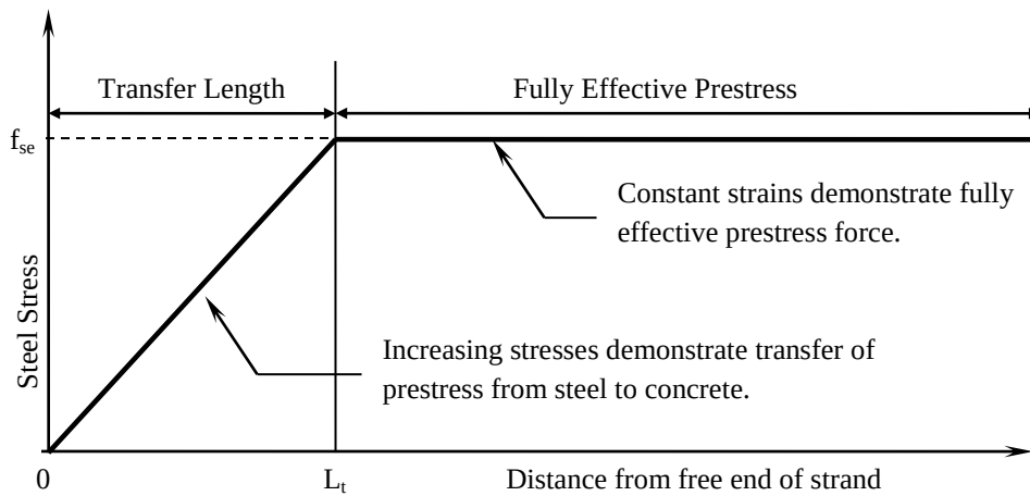
Figure D-1: Idealized stress in steel strand in a prestressed concrete member
