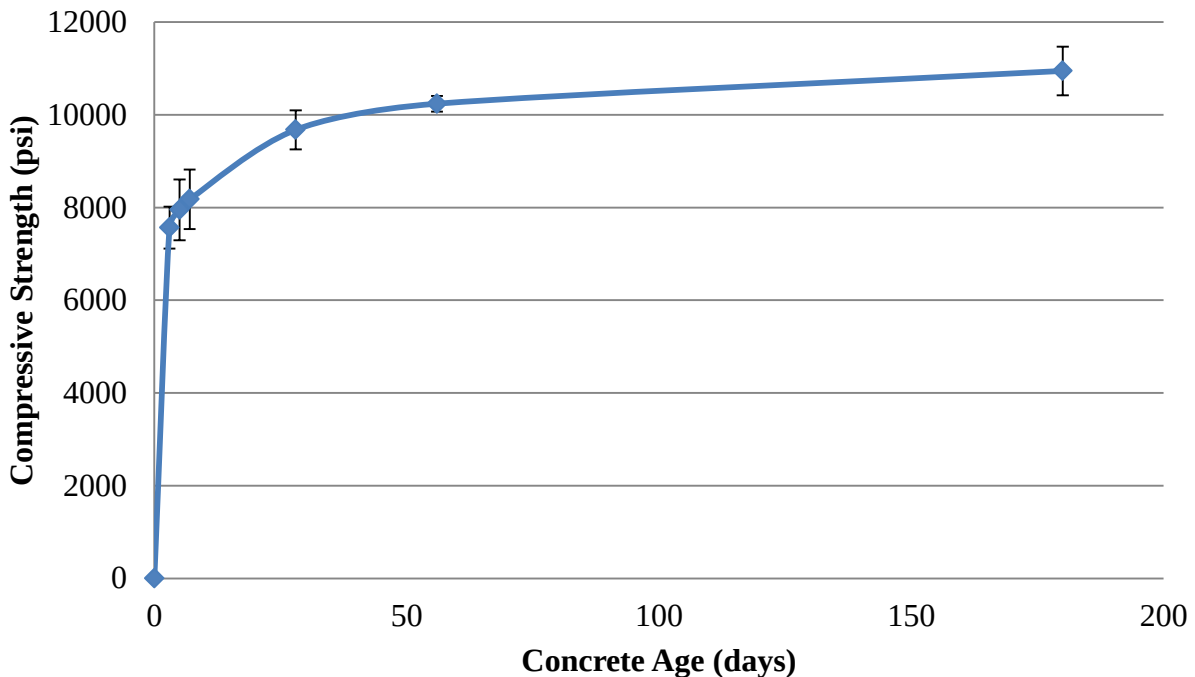
Figure 2-1: HSLW compressive strength gain curve, (1 psi = 6.89 kPa)
