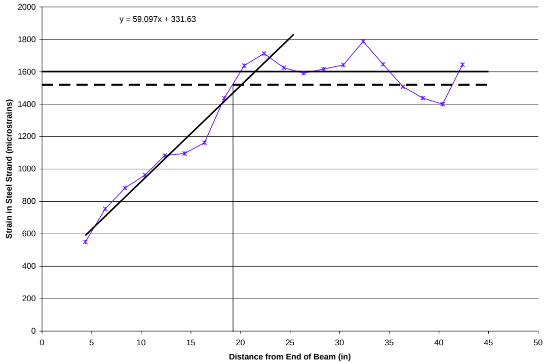
Figure D-6: Smoothed CSS readings for the South end of Girder 5 at day 80.
