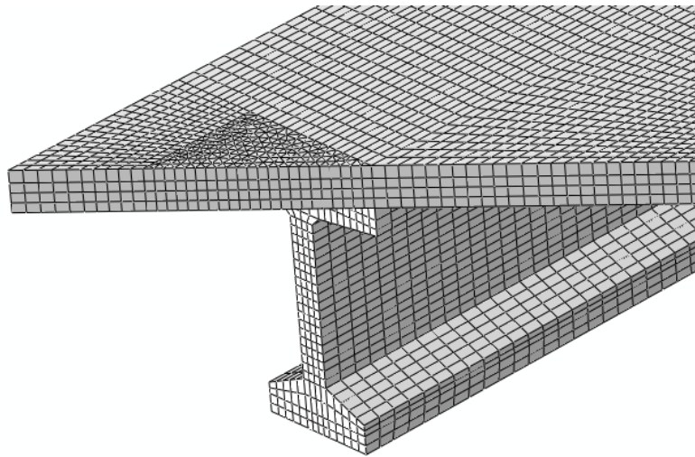
Figure 4-6: Finite element mesh of the bridge structure
