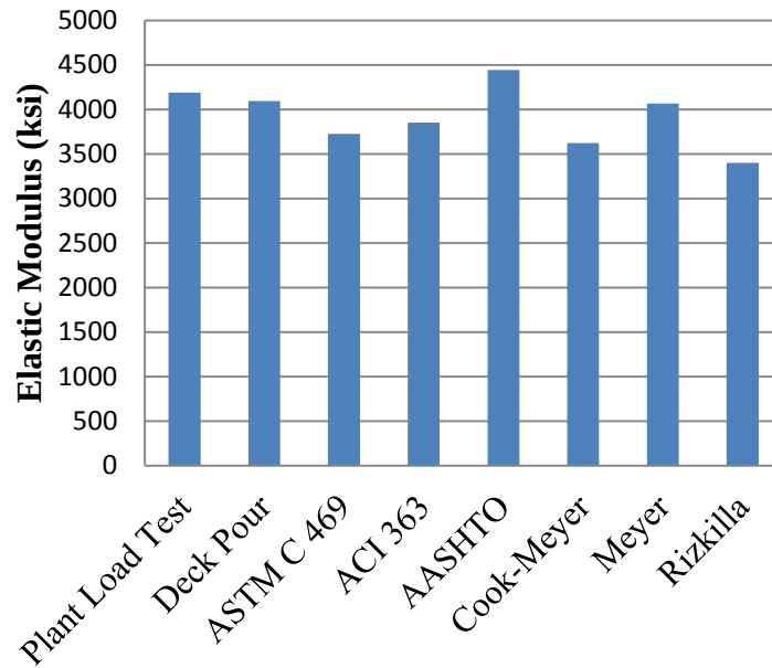
Figure 2-4: Elastic modulus comparison for HSLW with prediction methods (1ksi = 6.89MPa)
