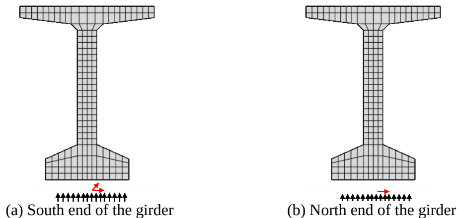
Figure 4-7: Support boundary conditions
