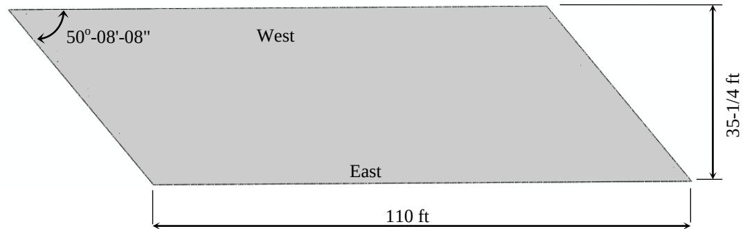
(b) Top plane view (bridge deck) of the bridge model (1ft = 30.48cm)
