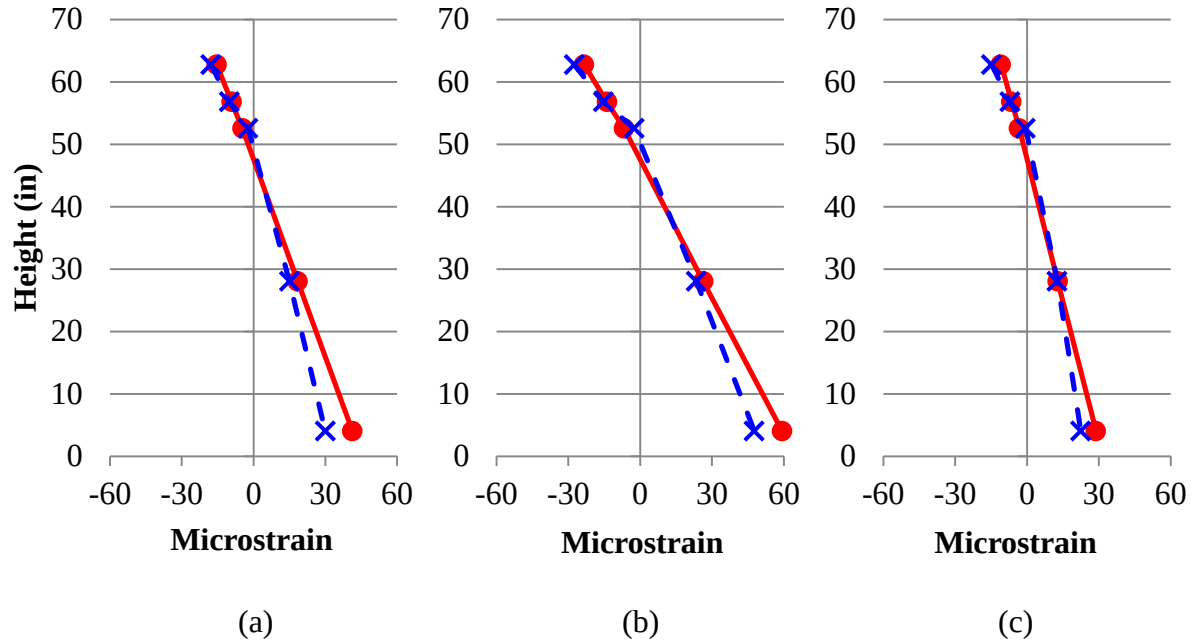
Figure 4-11: Strain profiles of girder 1 due to (a) LT1, (b) LT2, and (c) LT3 (1 in. = 2.54 cm)
