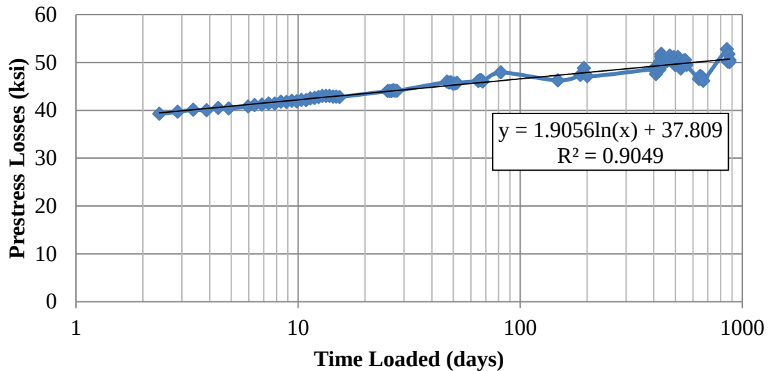
Figure 5-2: Lognormal regression of loss data (1 ksi = 6.9 MPa)
