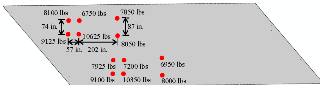
Figure 4-1: Load and arrangements of the truck wheels (1lb = 0.454kg)
