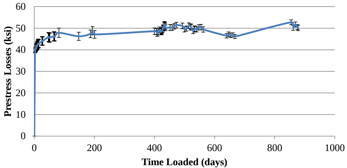
Figure 5-1: Measured prestress losses from HSLW girders (relaxation not included) (1 ksi = 6.9MPa)
