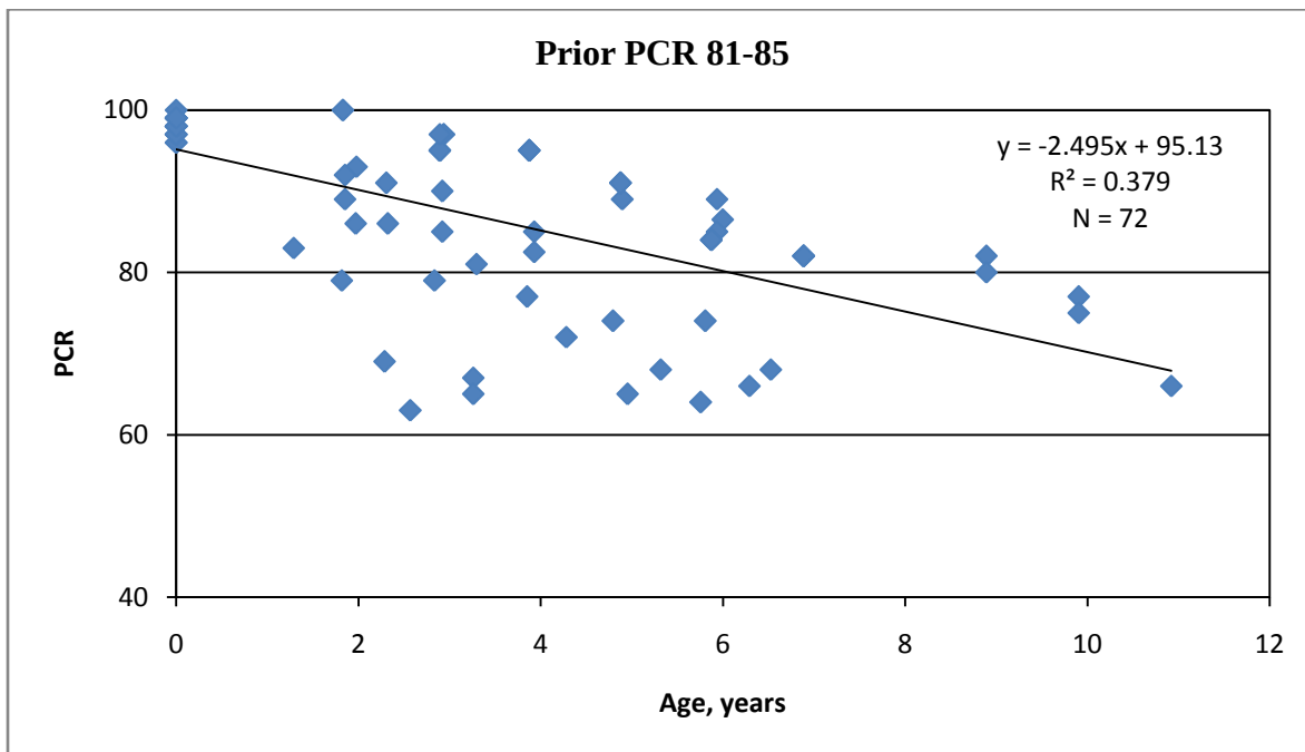
Figure 41. Performance Prediction Model for Micro Surfacing Treatment, Priority System, Prior PCR 81-85
