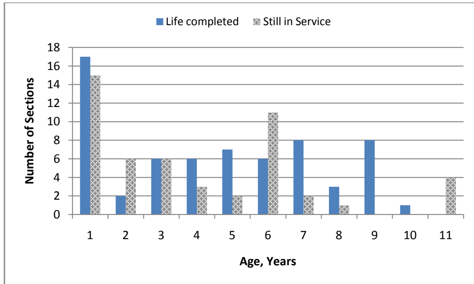
Figure 26. Service Life of Micro Surfacing Treatments on General System
