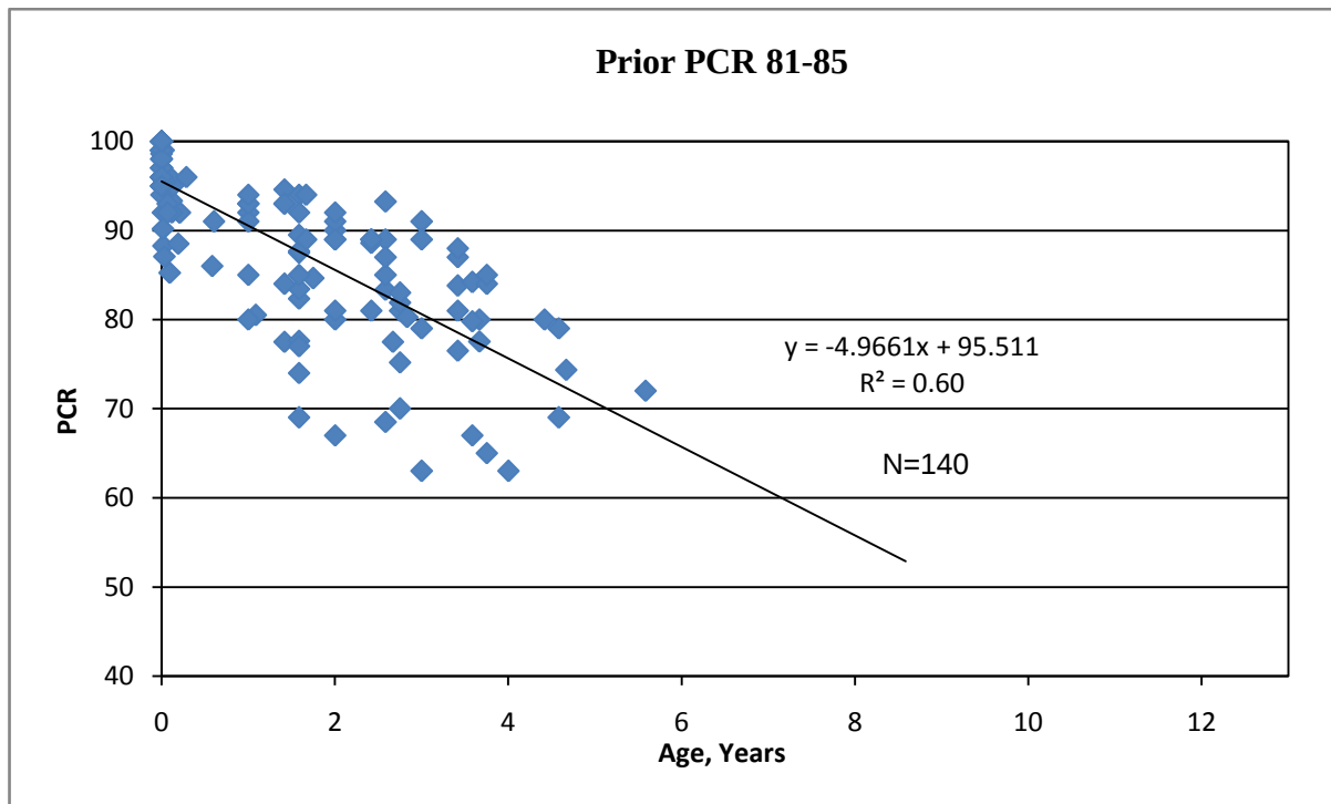
Figure 23. Performance Prediction Model for Chip Seal Treatment, Prior PCR 81-85
