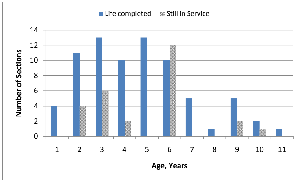
Figure 35. Service Life of Micro Surfacing Treatments on Priority System
