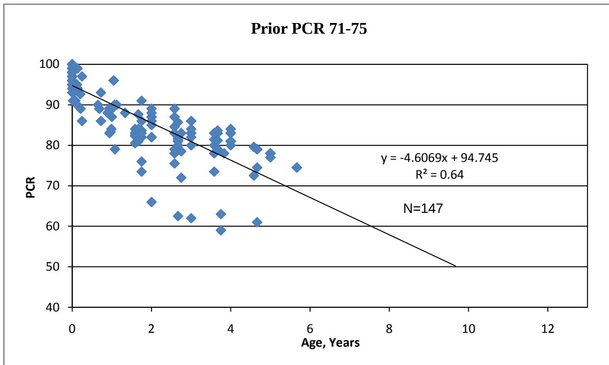
Figure 21. Performance Prediction Model for Chip Seal Treatment, Prior PCR 71-75
