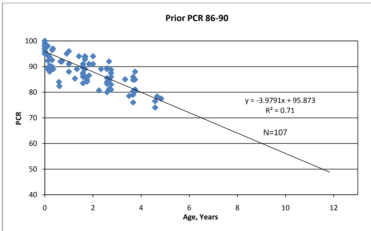
Figure 24. Performance Prediction Model for Chip Seal Treatment, Prior PCR 86-90
