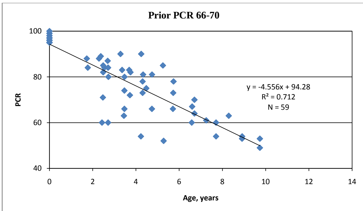
Figure 30. Performance Prediction Model for Micro Surfacing Treatment, General System, Prior PCR 66-70
