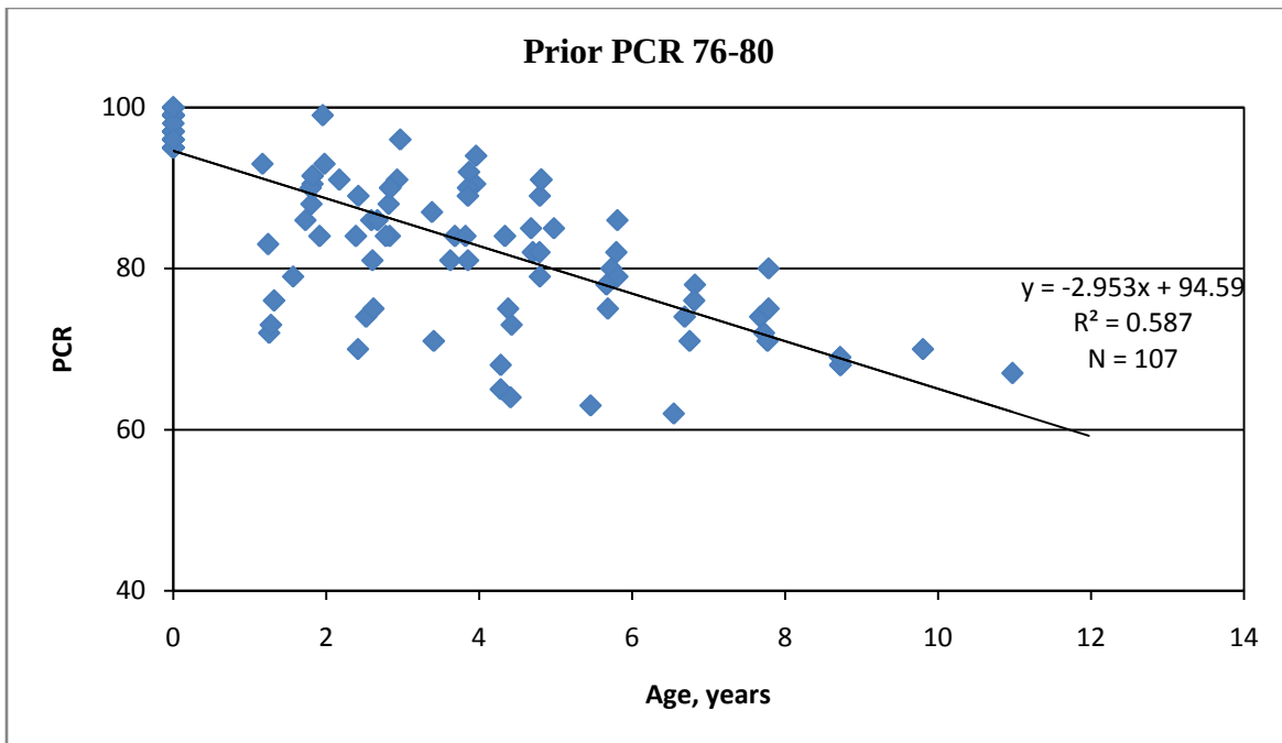
Figure 32. Performance Prediction Model for Micro Surfacing Treatment, General System, Prior PCR 76-80
