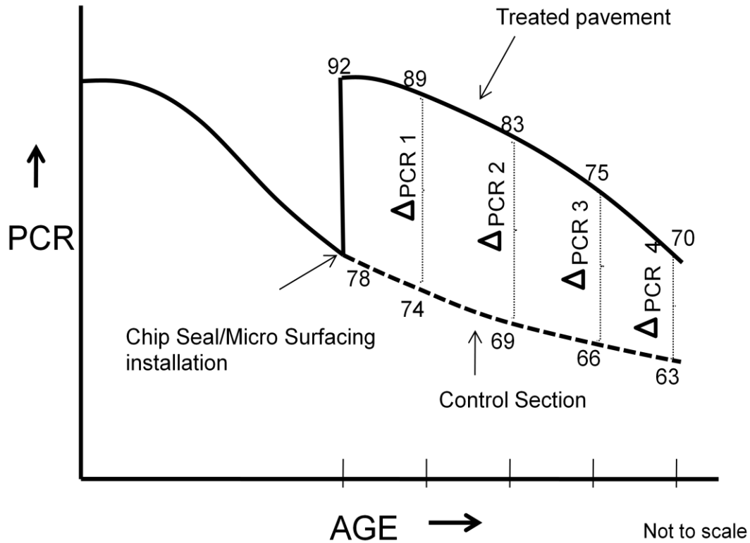
Figure 10. Calculating Performance Gain
