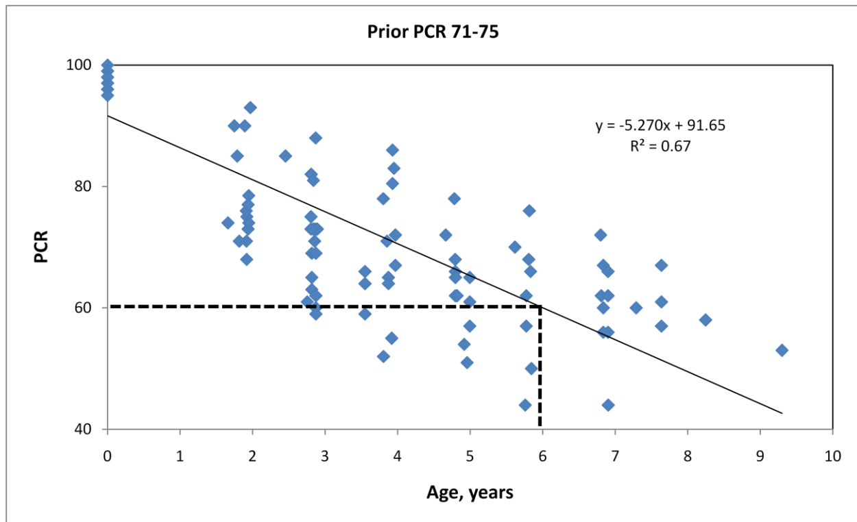
Figure 11. Calculating Life of Treatments Using Performance Prediction Models
