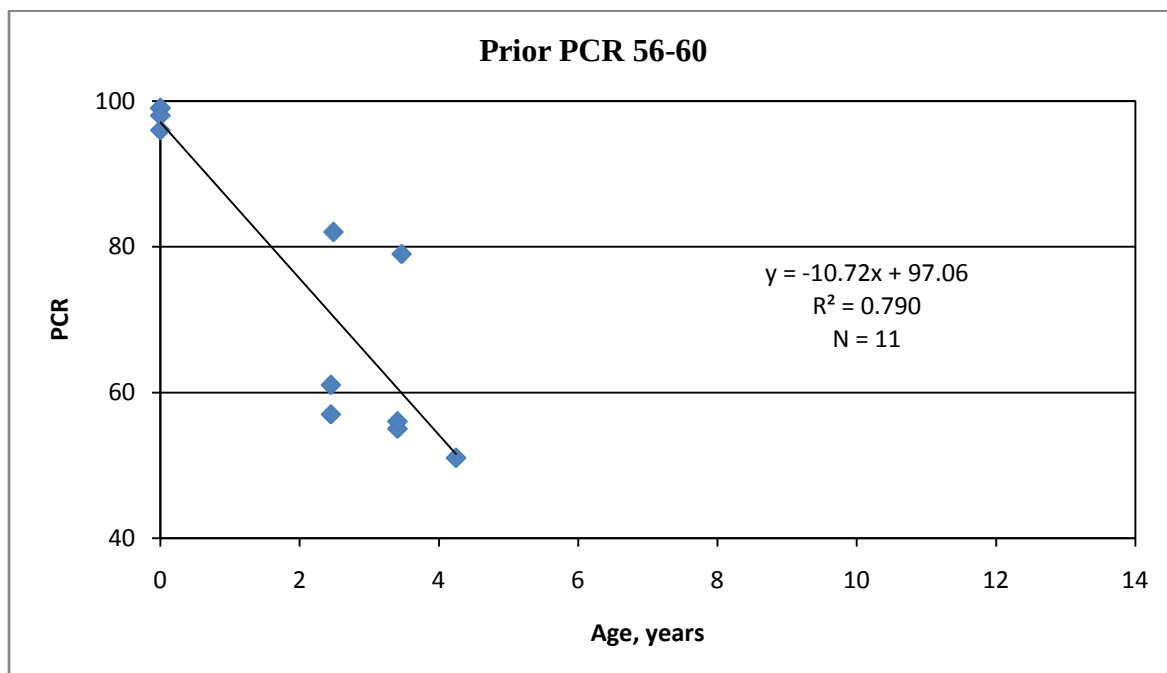
Figure 28. Performance Prediction Model for Micro Surfacing Treatment, General System, Prior PCR 56-60
