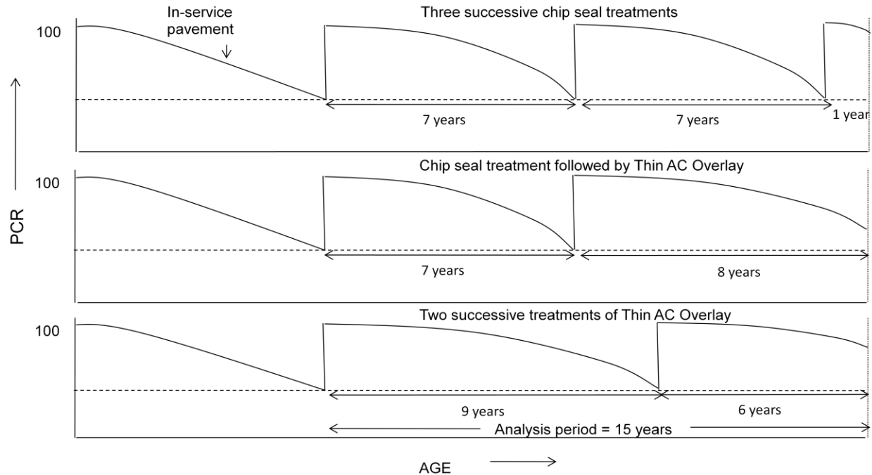
Figure 15. Life Cycle Cost Analysis of Chip Seal Treatment
