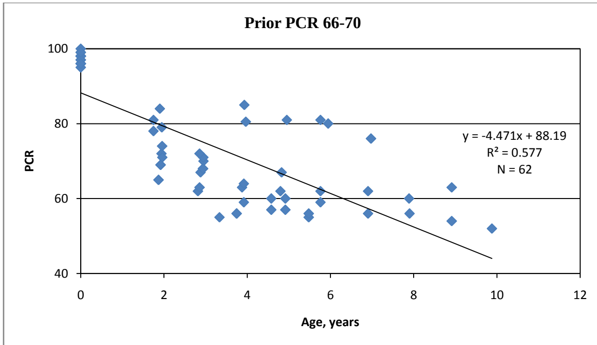
Figure 38. Performance Prediction Model for Micro Surfacing Treatment, Priority System, Prior PCR 66-70
