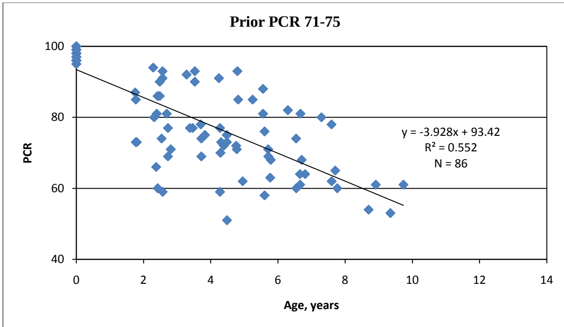
Figure 31. Performance Prediction Model for Micro Surfacing Treatment, General System, Prior PCR 71-75
