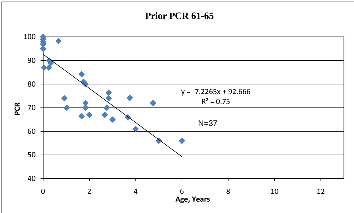
Figure 19. Performance Prediction Model for Chip Seal Treatment Prior, PCR 61-65
