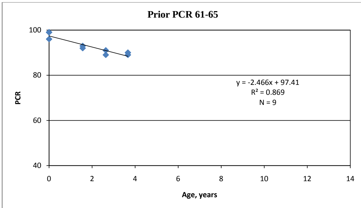
Figure 29. Performance Prediction Model for Micro Surfacing Treatment, General System, Prior PCR 61-65
