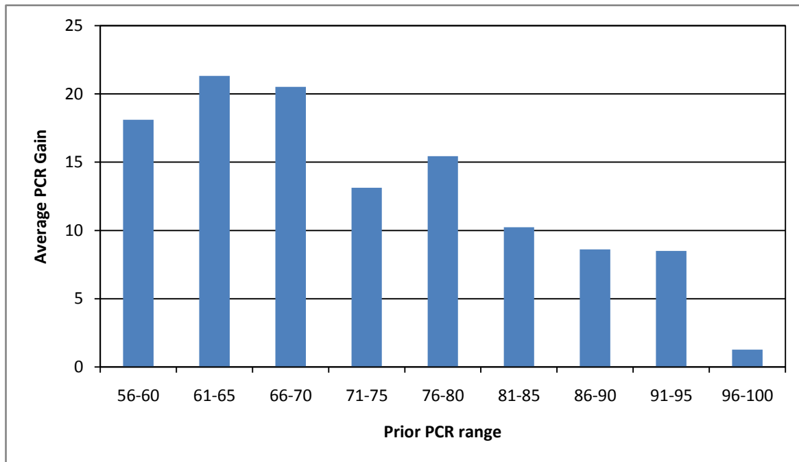
Figure 27. Average PCR Gain for Micro Surfacing Treatment on General System
