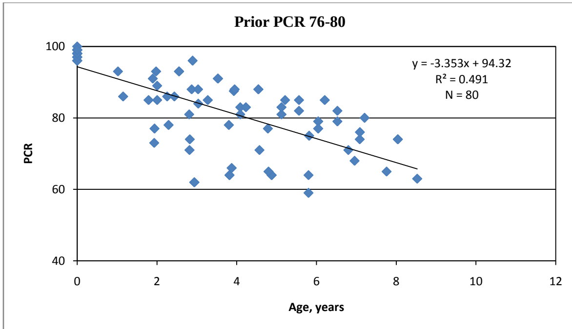
Figure 40. Performance Prediction Model for Micro Surfacing Treatment, Priority System, Prior PCR 76-80
