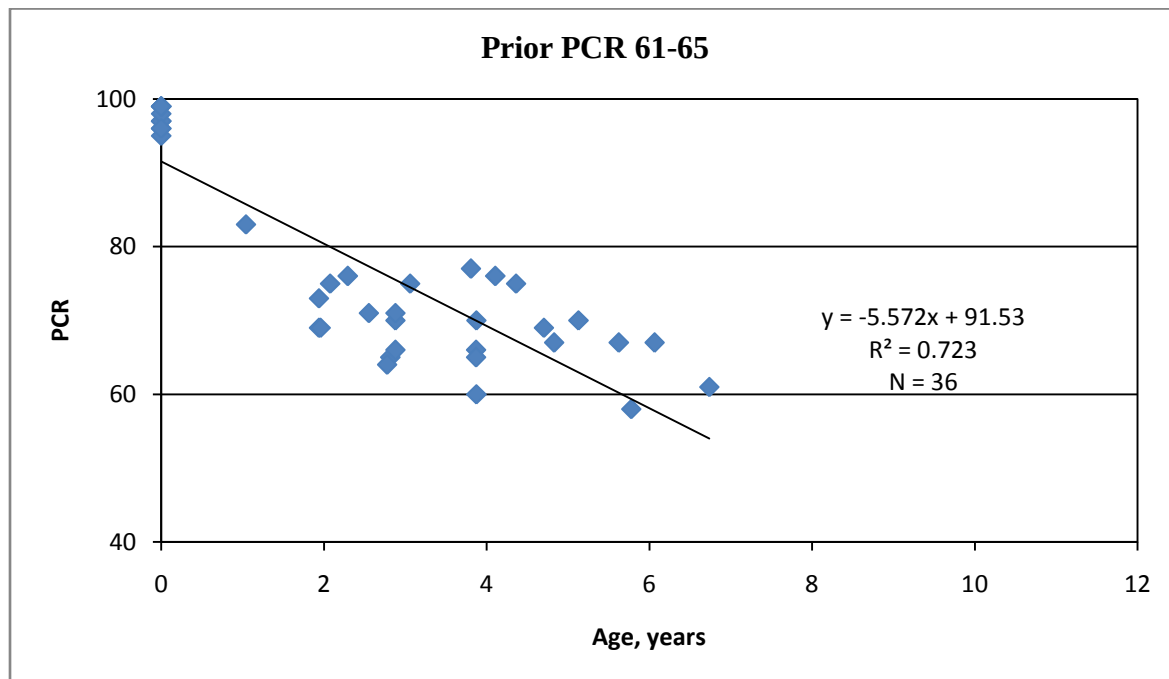
Figure 37. Performance Prediction Model for Micro Surfacing Treatment, Priority System, Prior PCR 61-65
