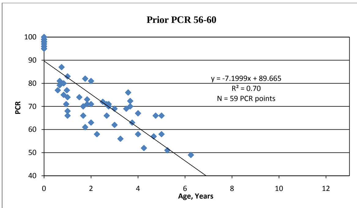
Figure 18. Performance Prediction Model for Chip Seal Treatment, Prior PCR 56-60
