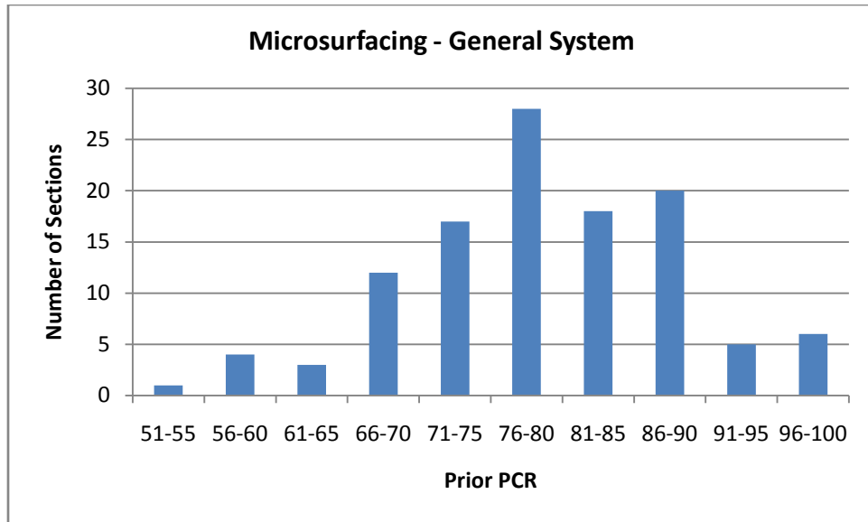
Figure 8. Condition of Pavements Before Micro Surfacing on General System
