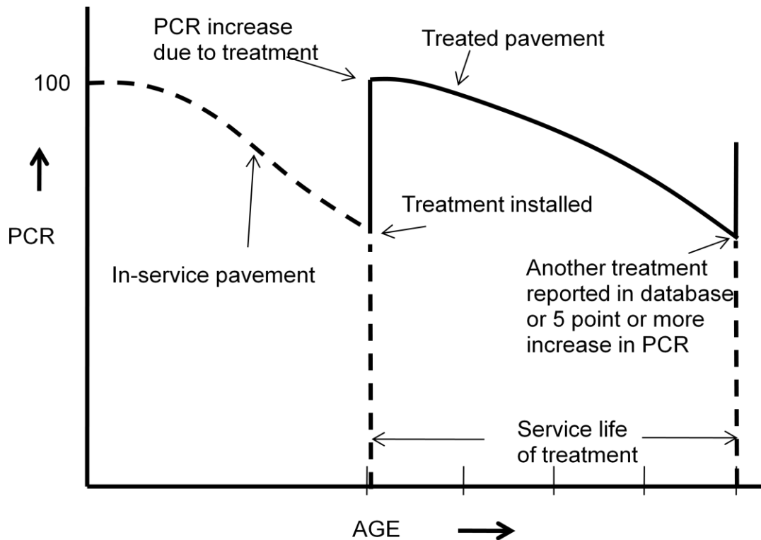
Figure 9. Calculating Service Life of Treatments Using Historic Data
