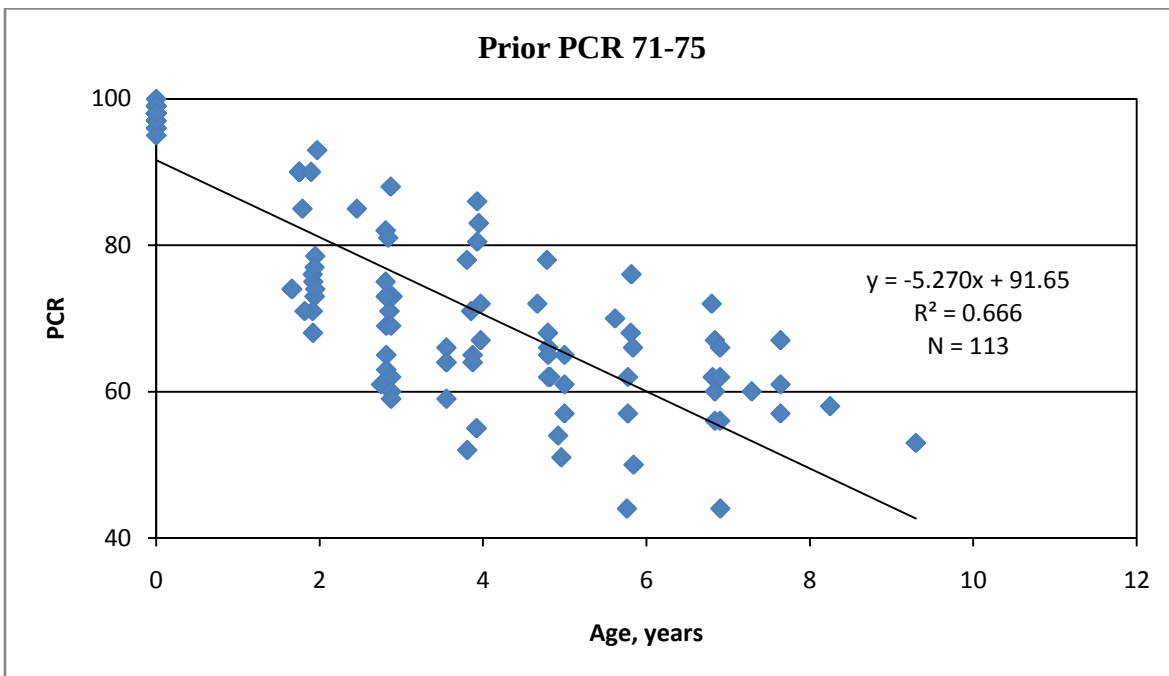
Figure 39. Performance Prediction Model for Micro Surfacing Treatment, Priority System, Prior PCR 71-75
