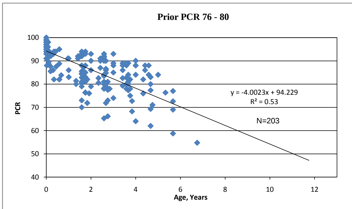
Figure 22. Performance Prediction Model for Chip Seal Treatment, Prior PCR 76-80
