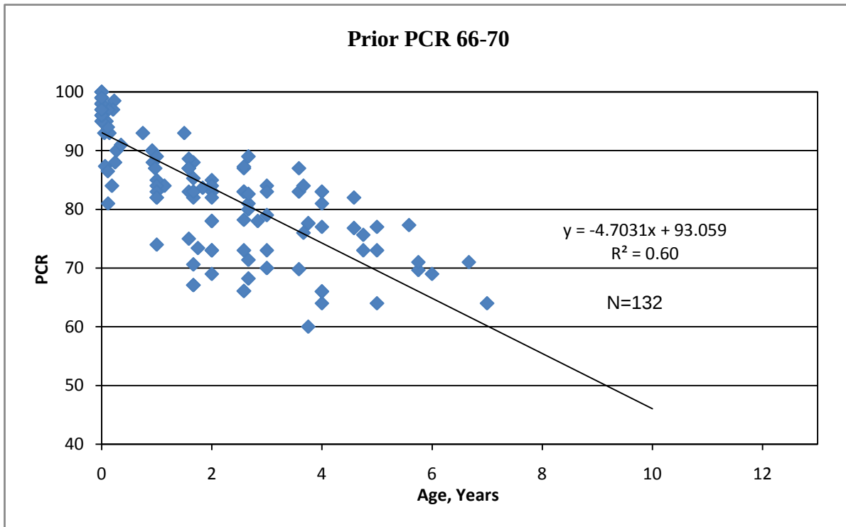
Figure 20. Performance Prediction Model for Chip Seal Treatment, Prior PCR 66-70
