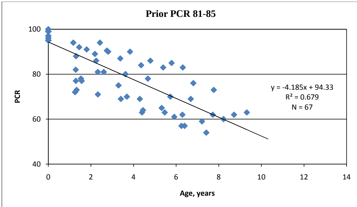
Figure 33. Performance Prediction Model for Micro Surfacing Treatment, General System, Prior PCR 81-85
