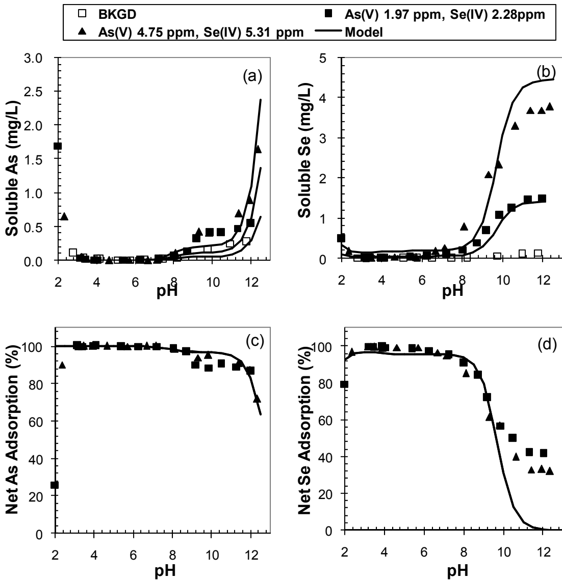
Figure 1. As and Se leaching and adsorption from raw ash #034. Symbols are experimental data, solid curves are modeling results. Experimental conditions: L/S = 10, temperature = 20–25 °C, leaching time = 24 hours.
