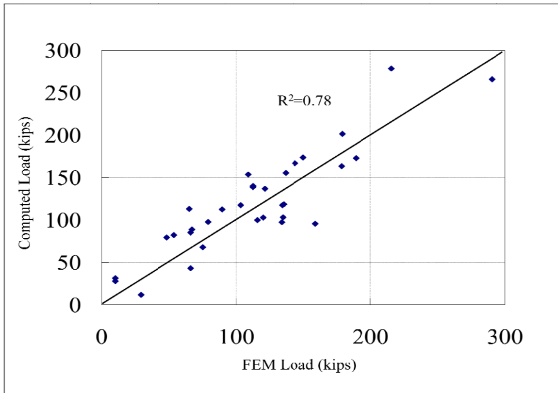
Figure 3.17: Comparison of Net Force on Shaft by Semi-empirical Equations and FEM
