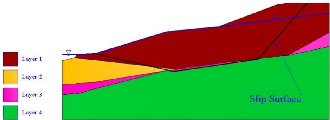
Figure 5.18: Representative Cross Section of WAS-7 Site
