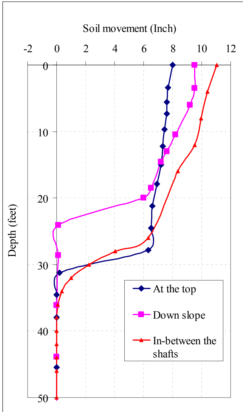
Figure 4.29: Computed Ground Movement Profiles due to Extreme Surcharge Loads
