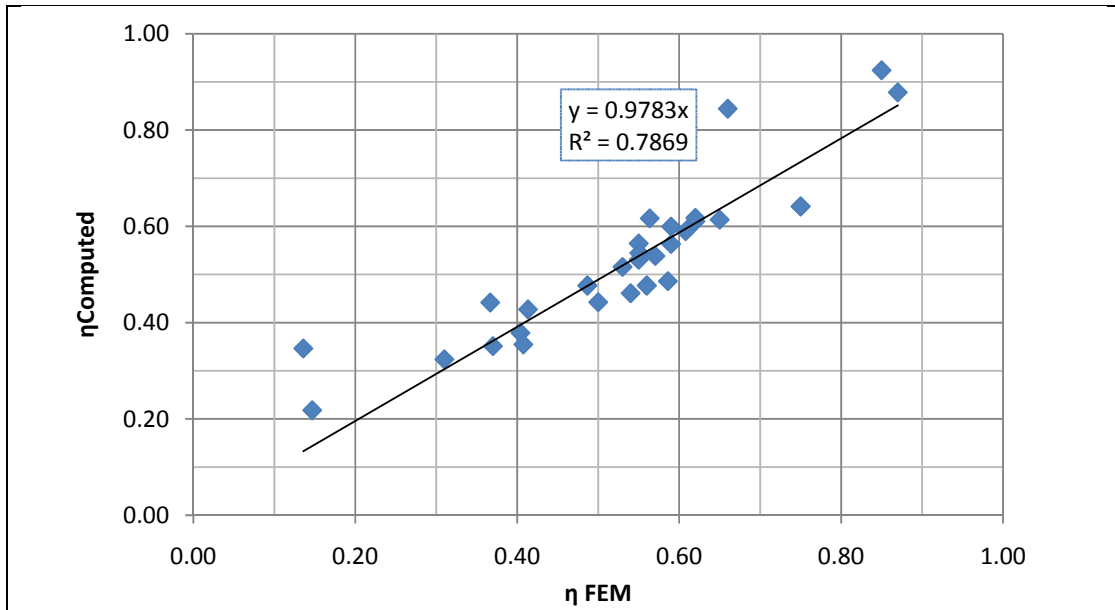
Figure 3.15: Comparison of Load Transfer Factor Computed by Semi-Empirical Equation and FEM
