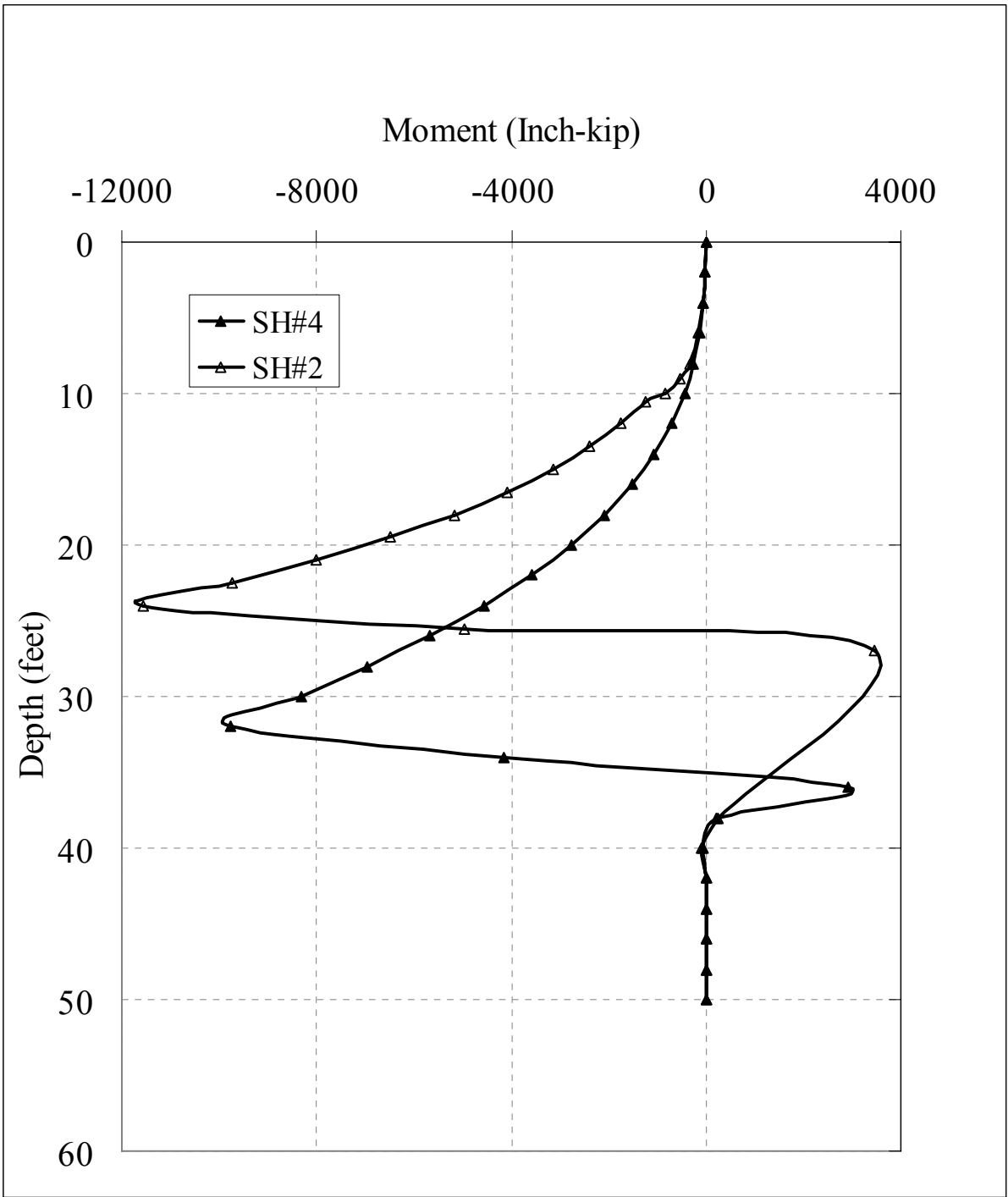
Figure 4.31: Computed Bending Moments in Drilled Shafts at Extreme Surcharge Loads
