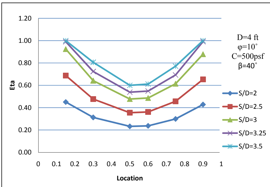
Figure 3.13: Variation of \eta Versus Shaft Location and S/D
