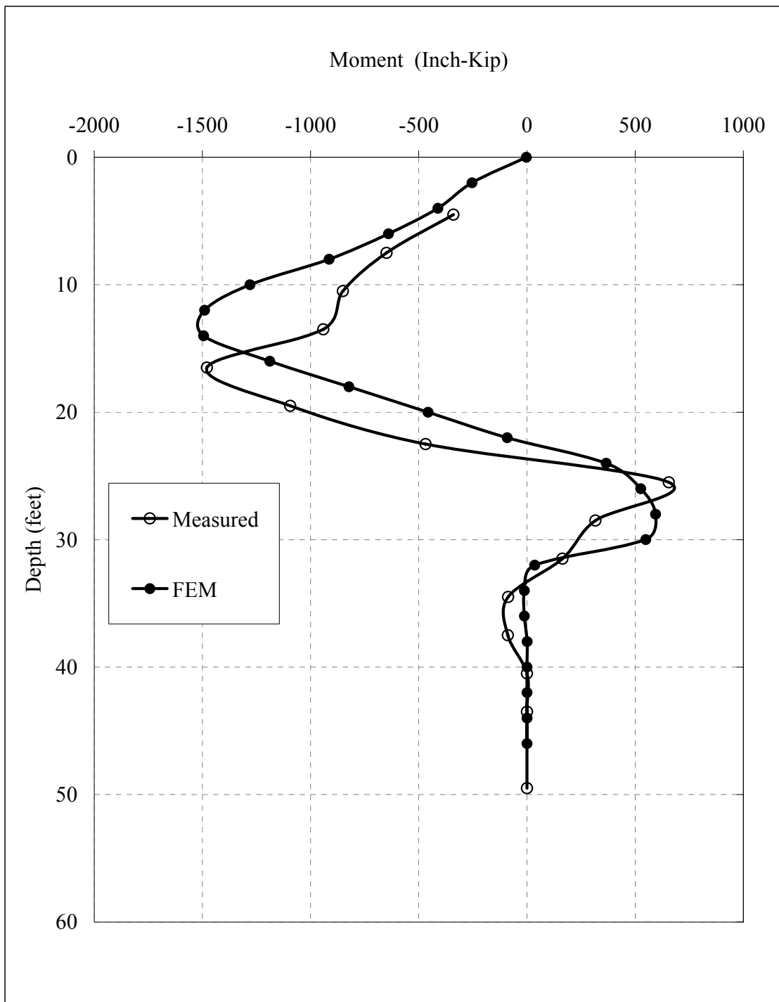
Figure 4.26: Comparison between Measured and FEM Computed Moments in Shaft #2: (b) due to Second Loading
