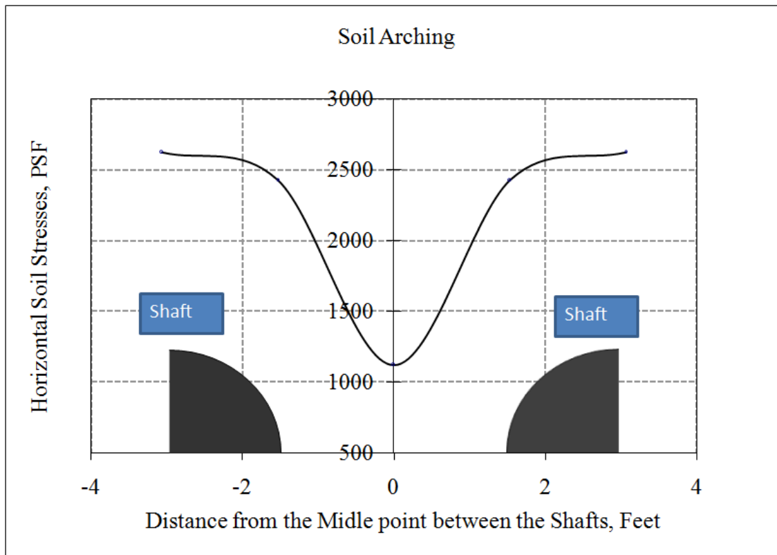
Figure 3.9 : A Graph of Soil Arching Between Two Shafts
