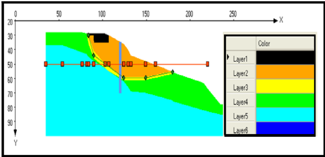
Figure 4.4: Simplified Cross-Section at the ATH-124 Site
