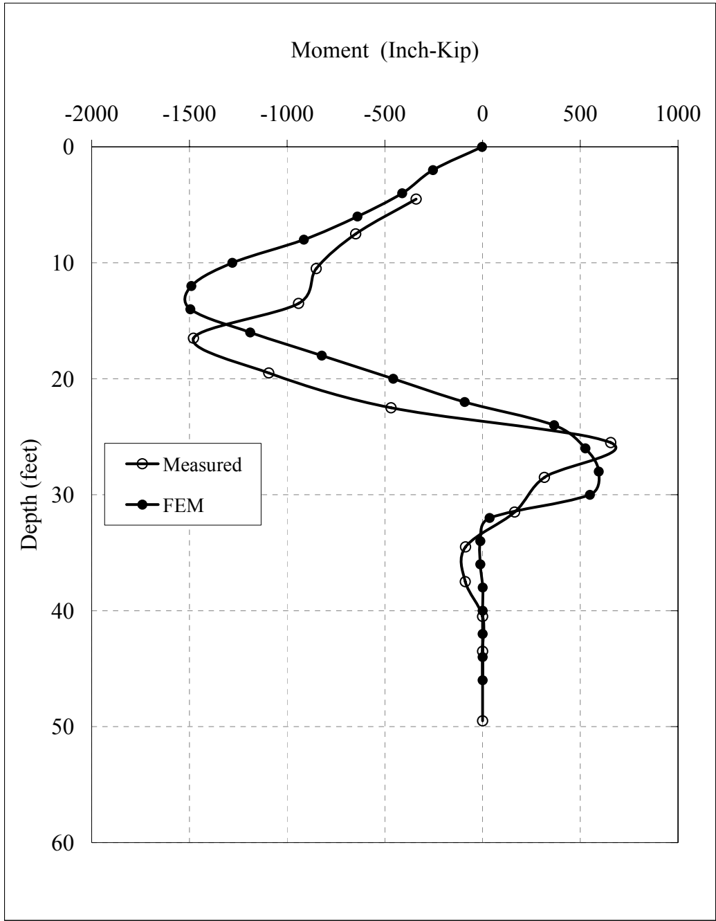
Figure 4.27: Comparison between Measured and FEM Measured Moments in Shaft #4: (b) due to Second Loading
