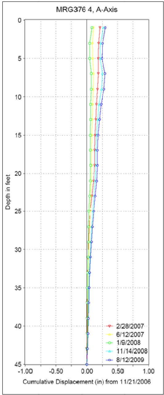
Figure 5.43: Cumulative Deflections of Shaft #11 at MRG-376 (Inclinometer #4)
