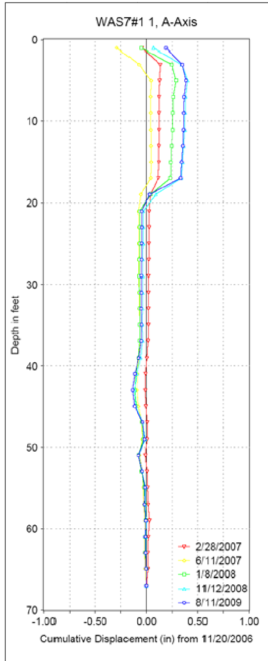
Figure 5.26: Cumulative Deflection in Shaft #53 at WAS-7 (Inclinometer #1)
