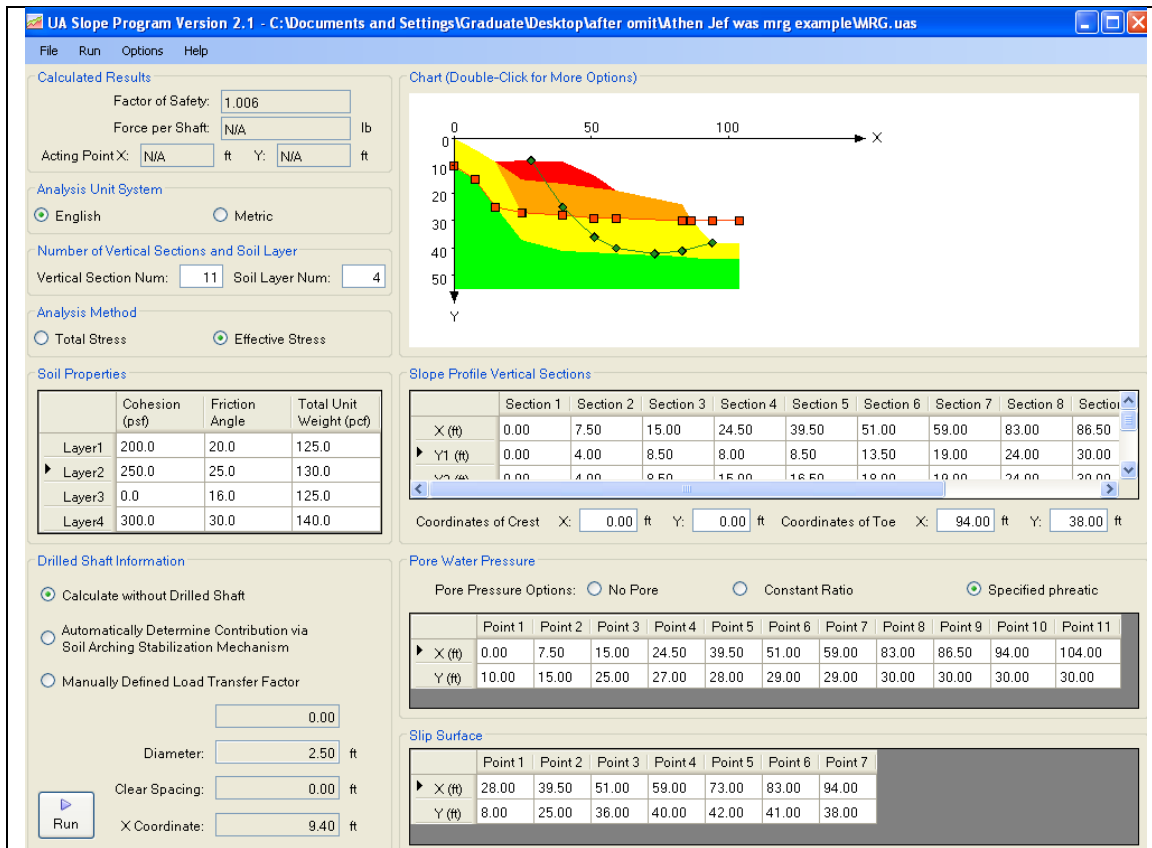
Figure 5.45: UA SLOPE 2.1 Analysis Results: a) without Drilled Shaft
