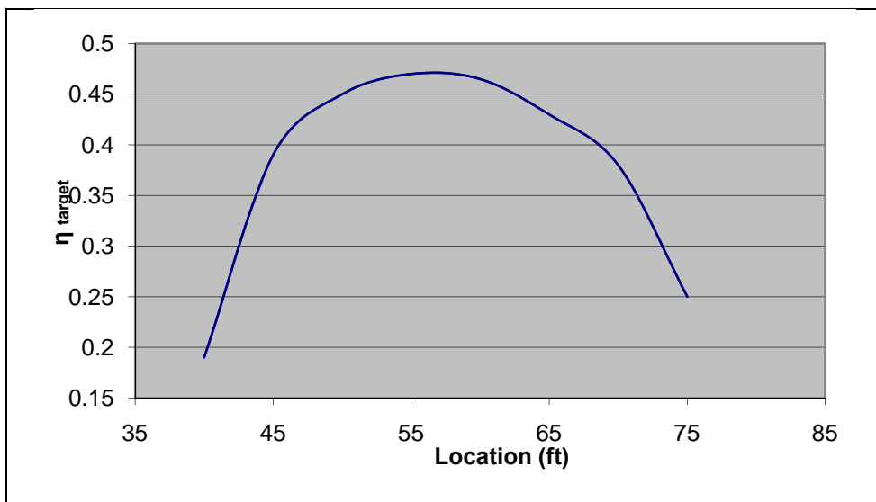
Fig. 4.10. \eta target vs. shaft location ( X ) for the illustrative example ( D = 3 ft and F_{\text{Starget}} = 1.5 )
