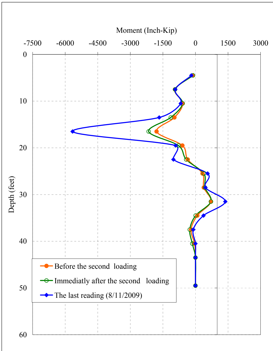
Figure 4.18: Measured Bending Moments in Shafts due to Surcharge Loading and Slope Soil Movement: (a) Shaft #2
