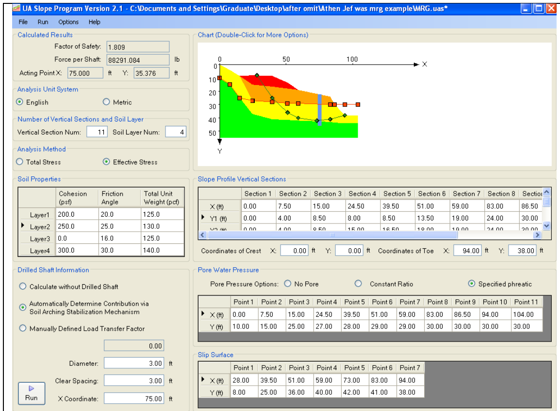
Figure 5.45: UA SLOPE 2.1 Analysis Results: b) with Drilled Shaft
