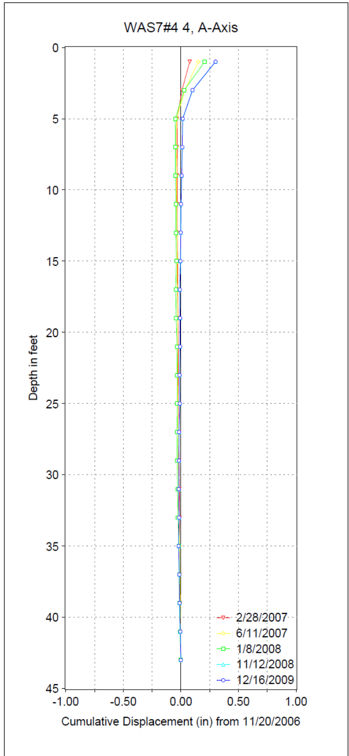
Figure 5.24: Cumulative Soil Movement at Upslope Side of the Drilled Shaft (Inclinometer #4) at WAS-7 Site.
