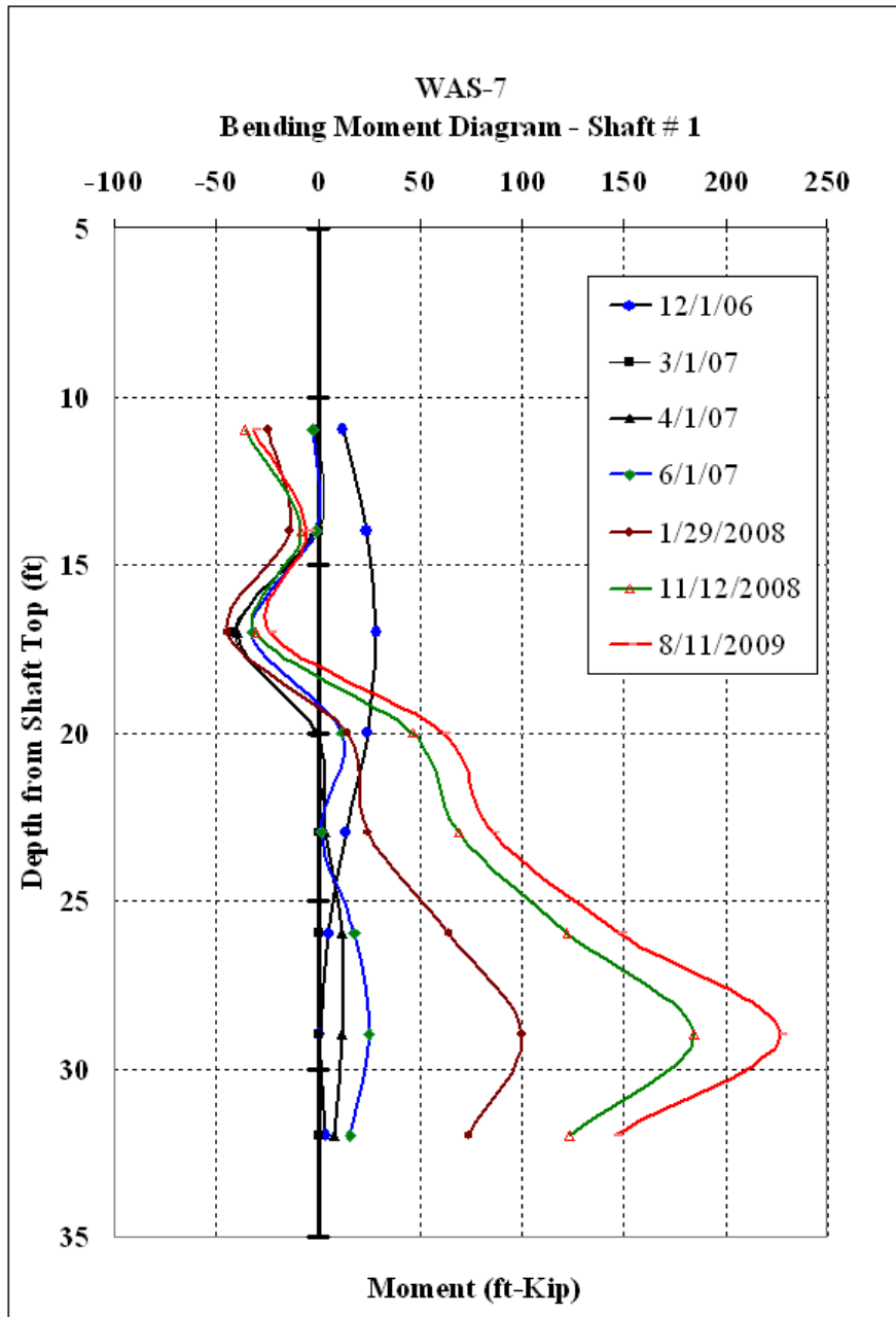
Figure 5.28: Moment Measurement from Shaft #53 at WAS-7 Site
