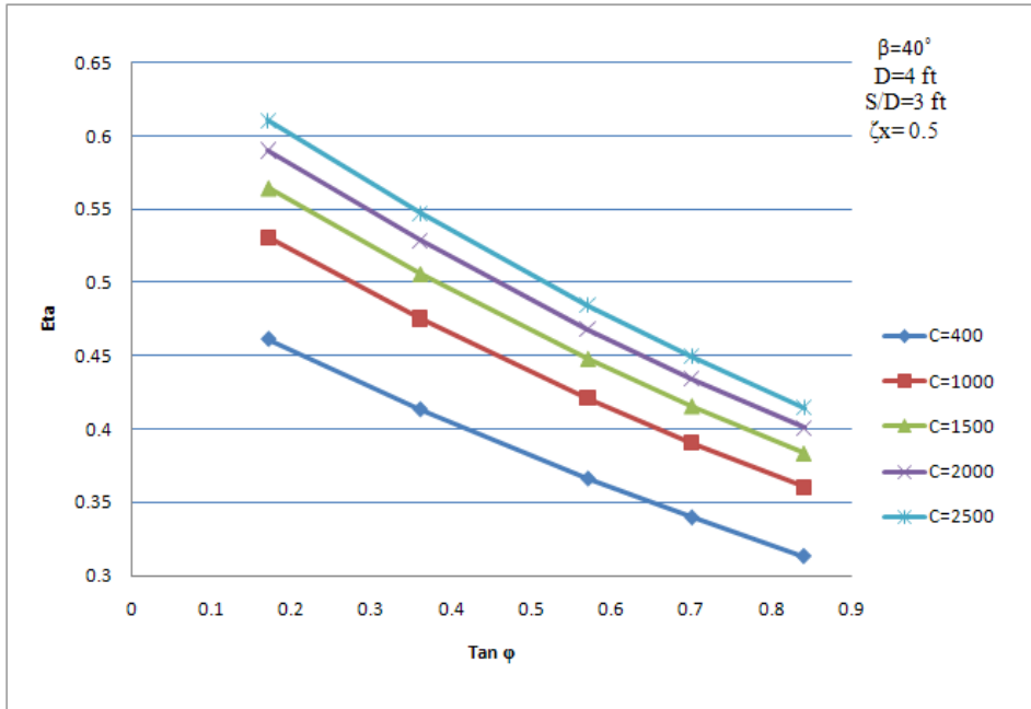
Figure 3.12: Variation of \eta Versus c and \tan(\phi)
