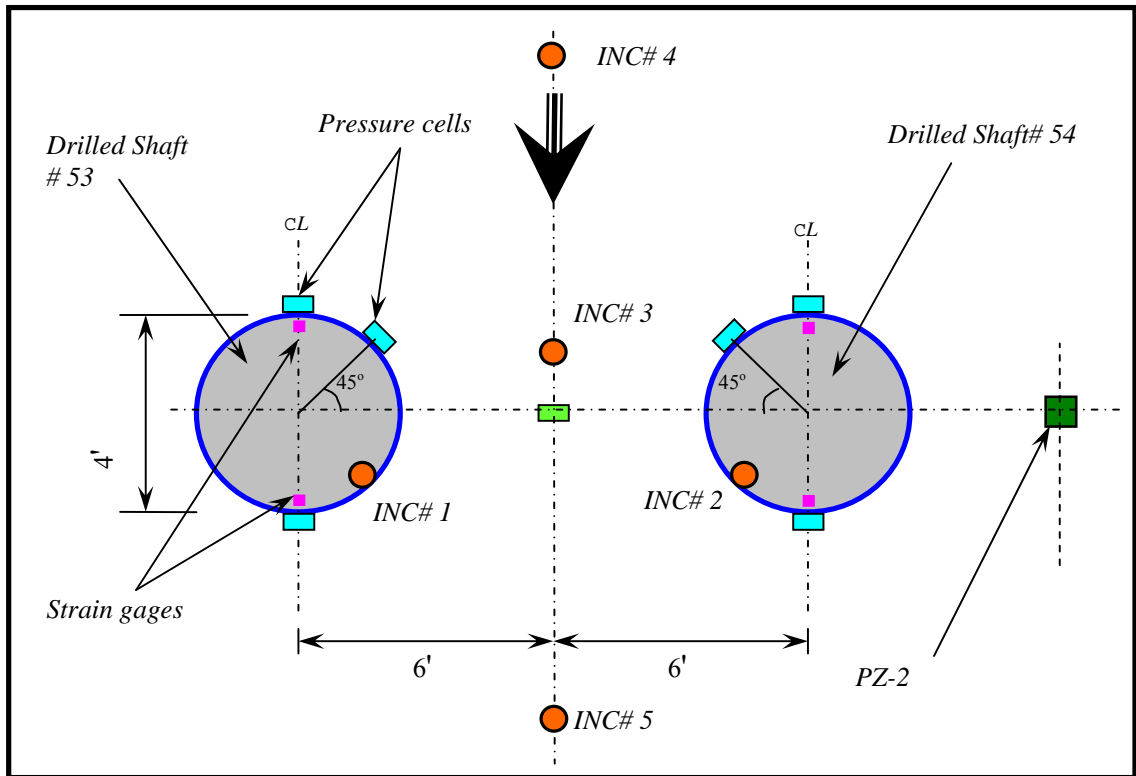
Figure 5.22: Plan View of Pressure Cell Locations Inside Drilled Shafts and on Ground at WAS-7 Site
