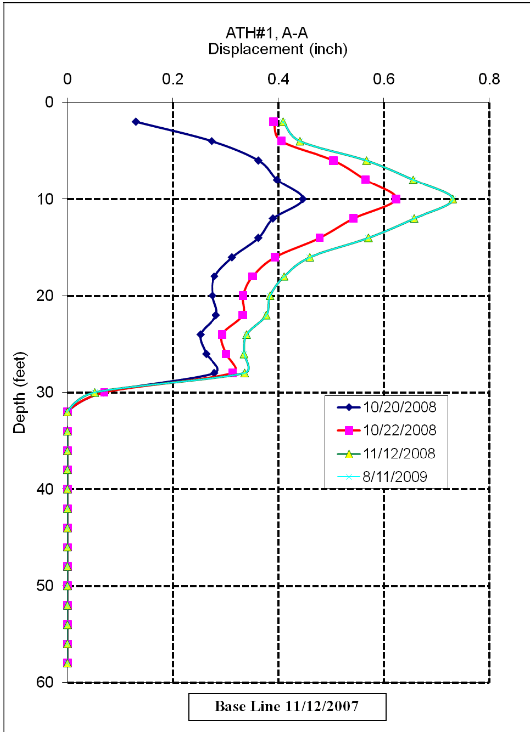
Figure 4.16: Measured Cumulative Slope Movements at Three Inclinometer Stations: (a) INC #1 at Upslope
