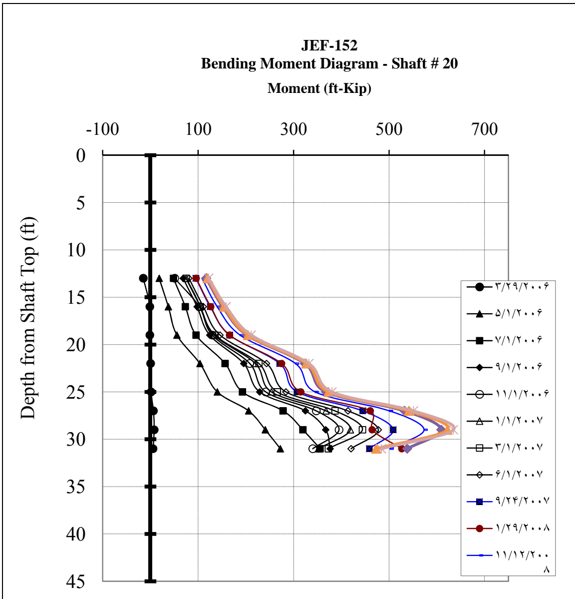
Figure 5.12: Measured Moments along Shaft #20 at JEF-152 Site
