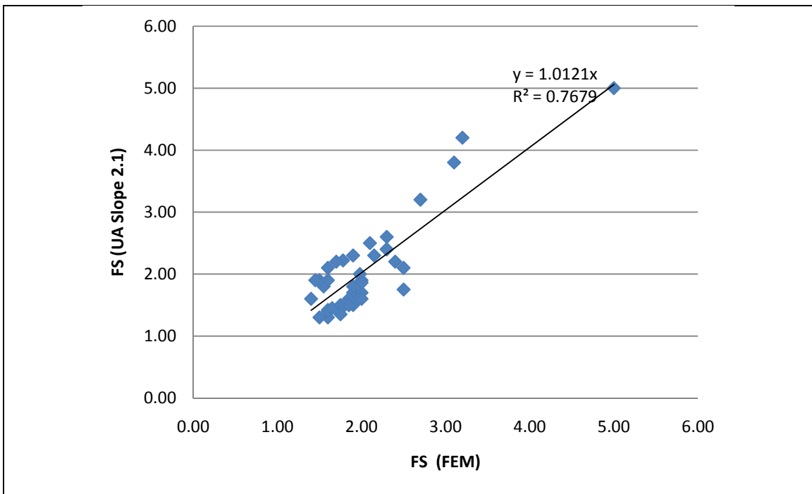
Figure 4.12: Validations of UA SLOPE 2.1 Program: (a) Comparison of FS
