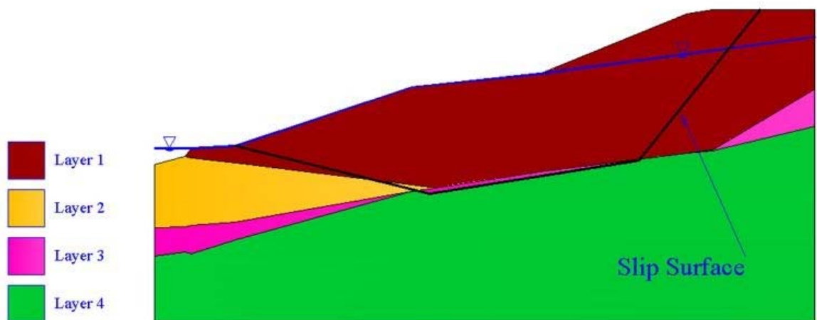
Figure 5.44: Simplified Slope Cross-Section Used in UA SLOPE 2.1 Analysis
