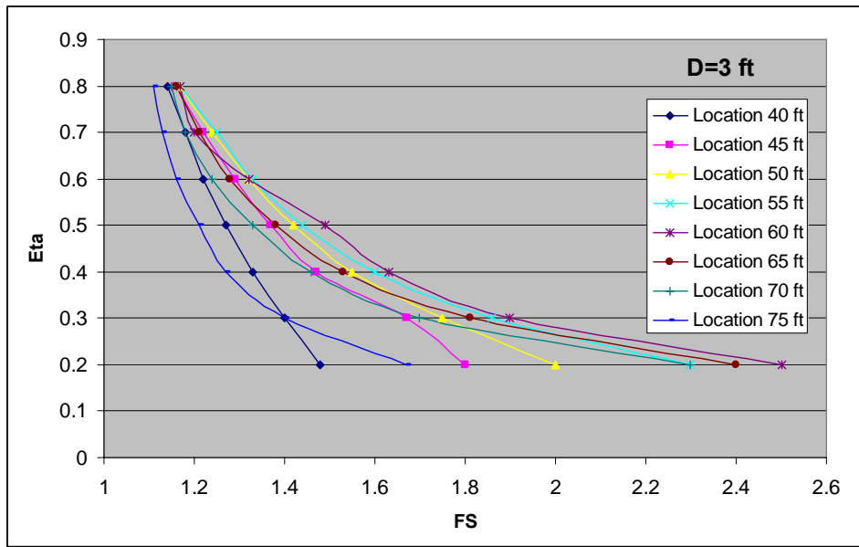
Fig. 4.9. \eta -FS diagram for the illustrative example at various drilled shaft locations ( D = 3 ft)
