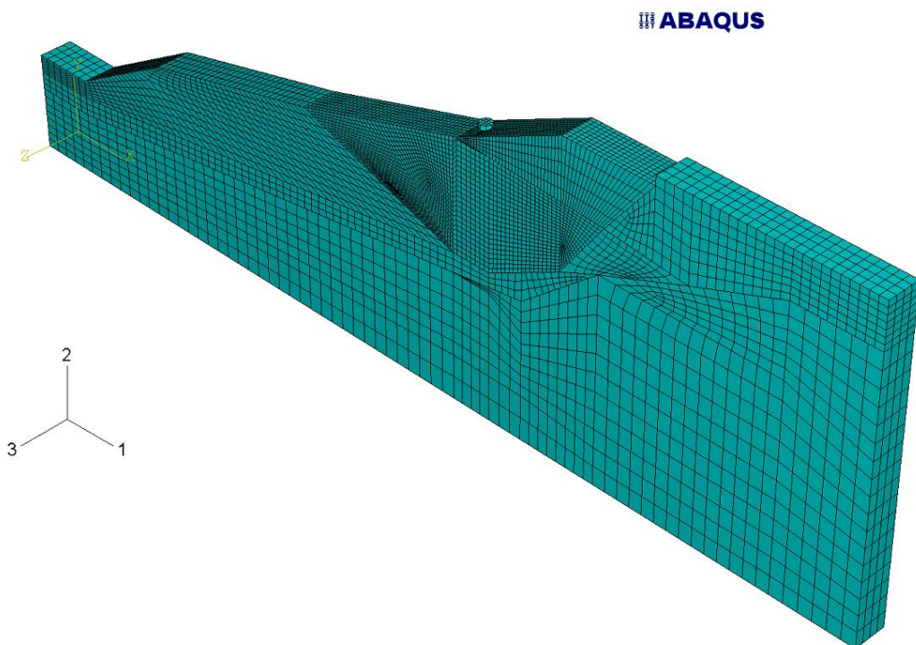
Figure 4.20: FEM Mesh of the ATH-124 Test Site
