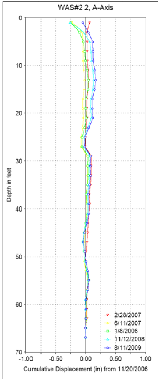
Figure 5.27: Cumulative Deflection in Shaft #54 at WAS-7 (Inclinometer #2)
