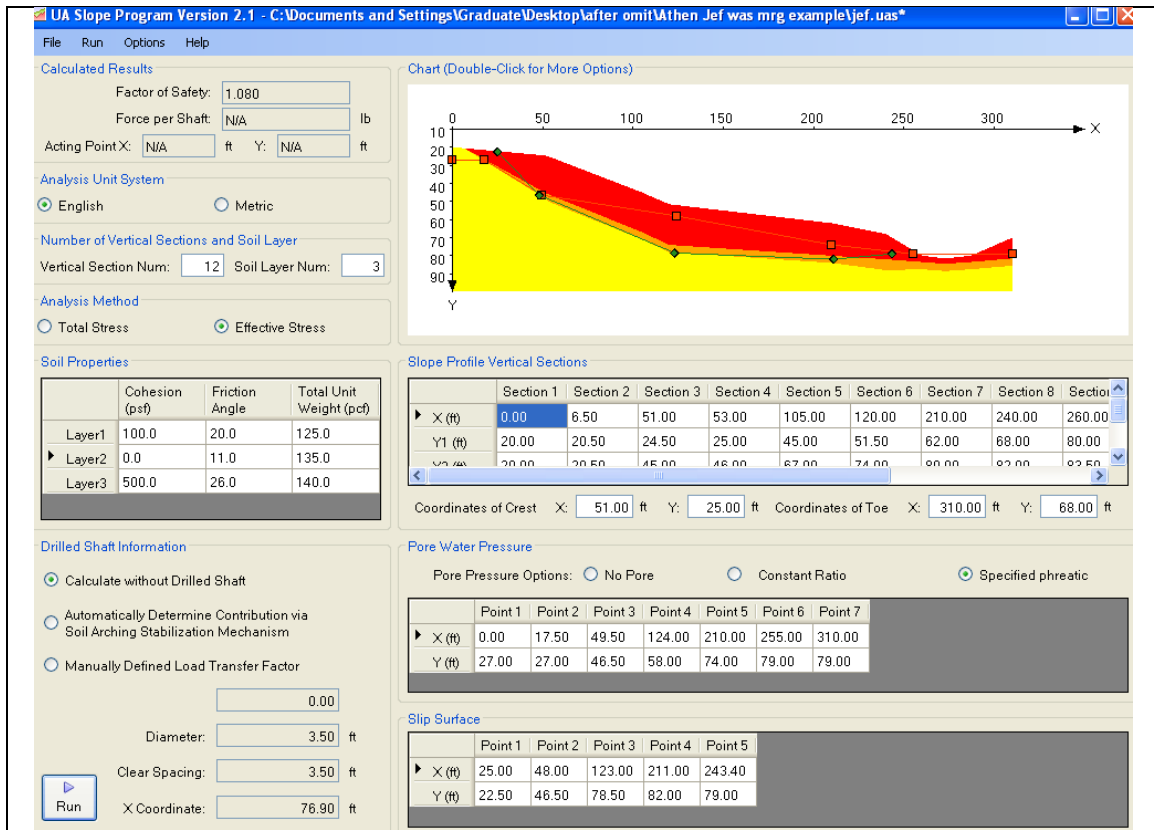
Figure 5.16: UA SLOPE 2.1 Analysis Results: a) without Drilled Shaft
