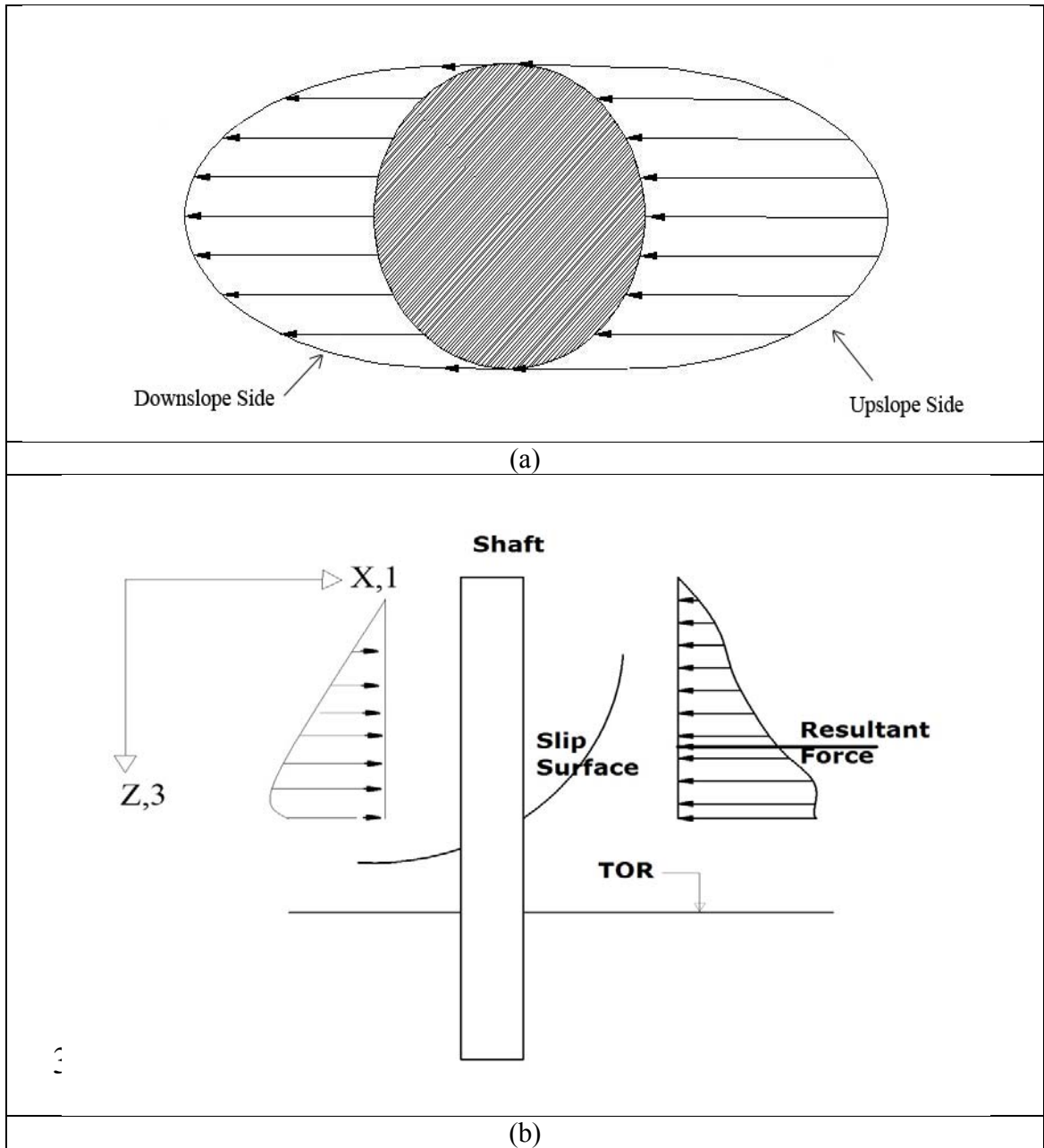
Figure 3.16: The Soil Stress Distribution a) Around the Shaft Perimeter b) From the Top of the Shaft Down to the Failure Surface
