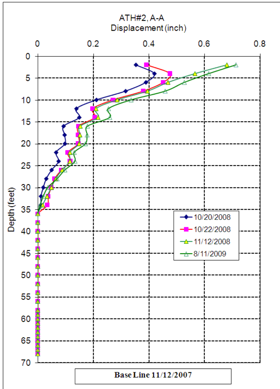
Figure 4.16: Measured Cumulative Slope Movements at Three Inclinometer Stations: (b) INC #2 Immediately Behind Drilled Shaft Down slope
