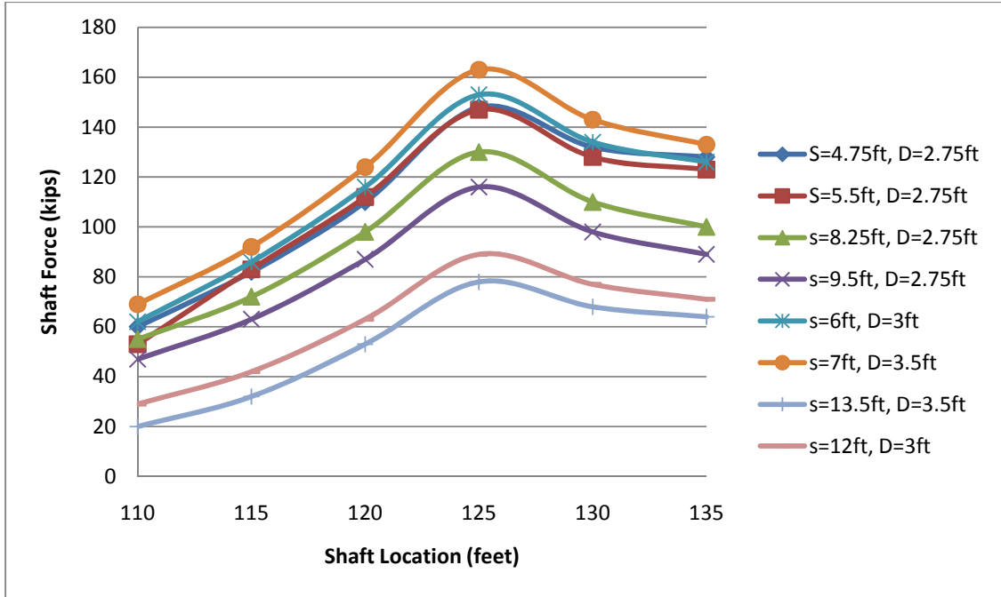
Figure 4.5: Shaft Force versus Shaft Location for Different (S, D) Combinations
