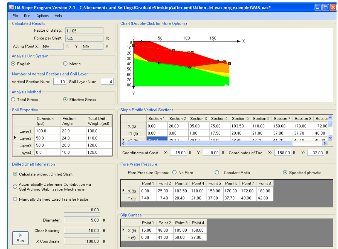
Figure 5.31: UA SLOPE 2.1 Analysis Results: a) without Drilled Shaft
