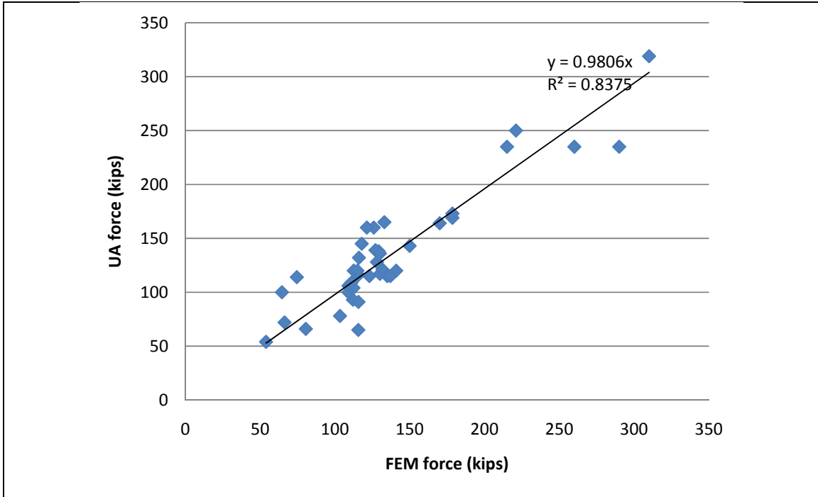
Figure 4.12: Validations of UA SLOPE 2.1 Program: (b) Comparison of the Net Force on Shaft.
