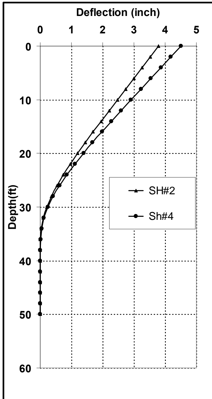
Figure 4.30: Computed Drilled Shaft Deflections at Extreme Surcharge Loads
