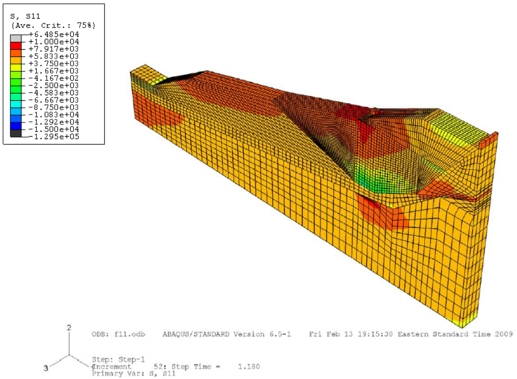
Figure 4.28: FEM Computed Stress Field at Failure Condition
