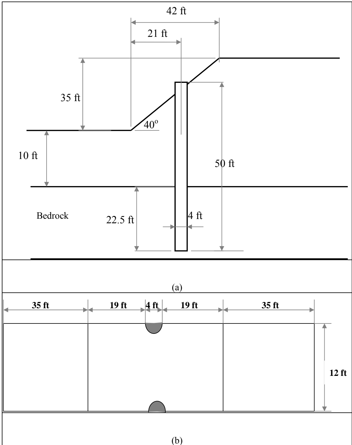
Figure 3.6 : Geometry and Dimensions of the Baseline Model a) Cross-Section b) Top View
