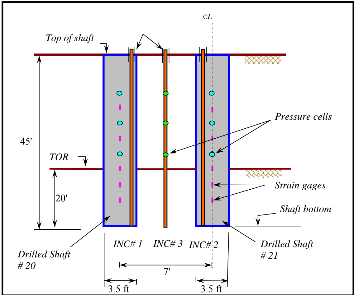
Figure 5.6: Schematic Diagram of Instrumentation Layout at JEF-152 Site
