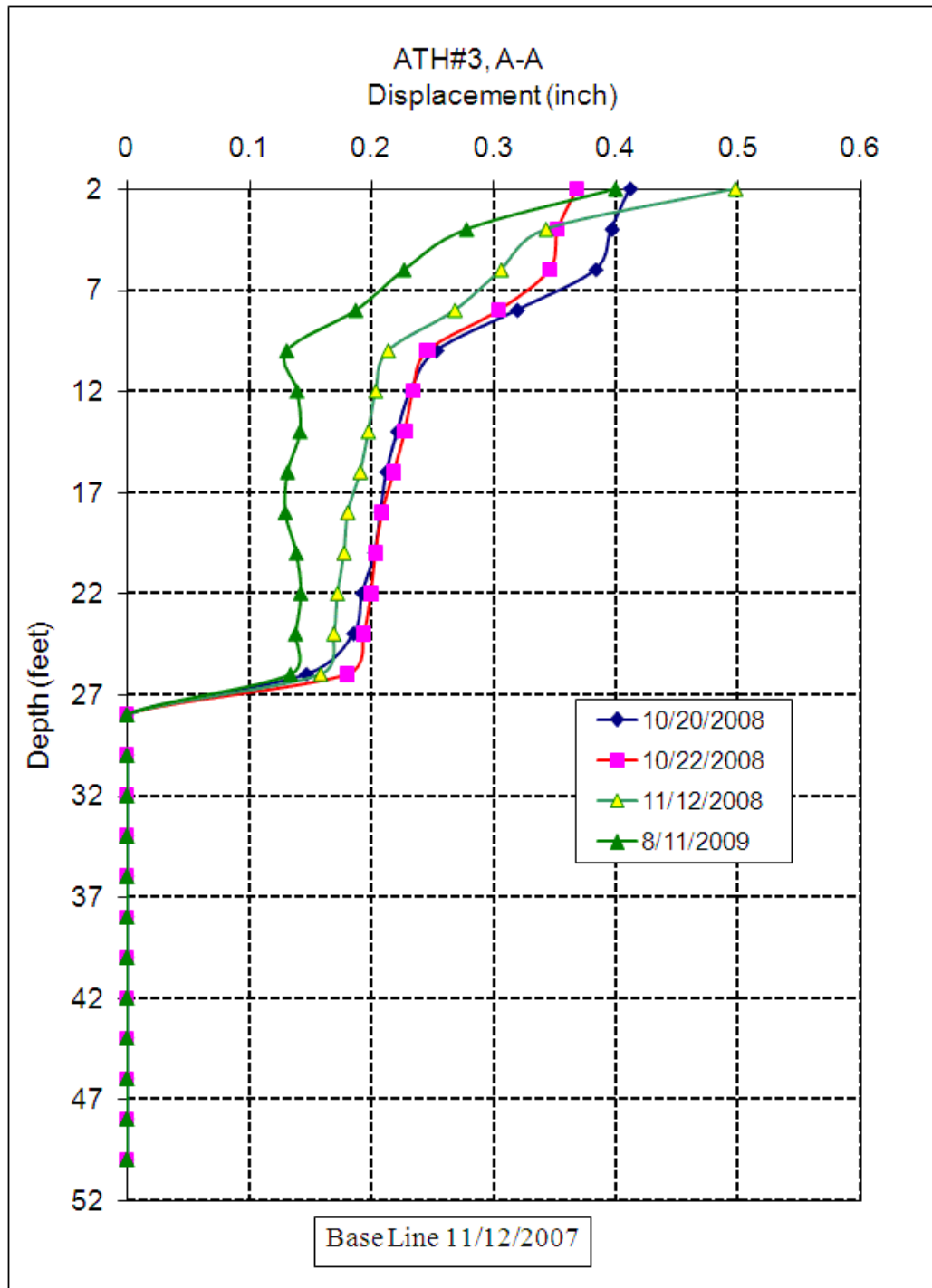
Figure 4.16: Measured Cumulative Slope Movements at Three Inclinometer Stations: (c) INC # 3 Near the Toe
