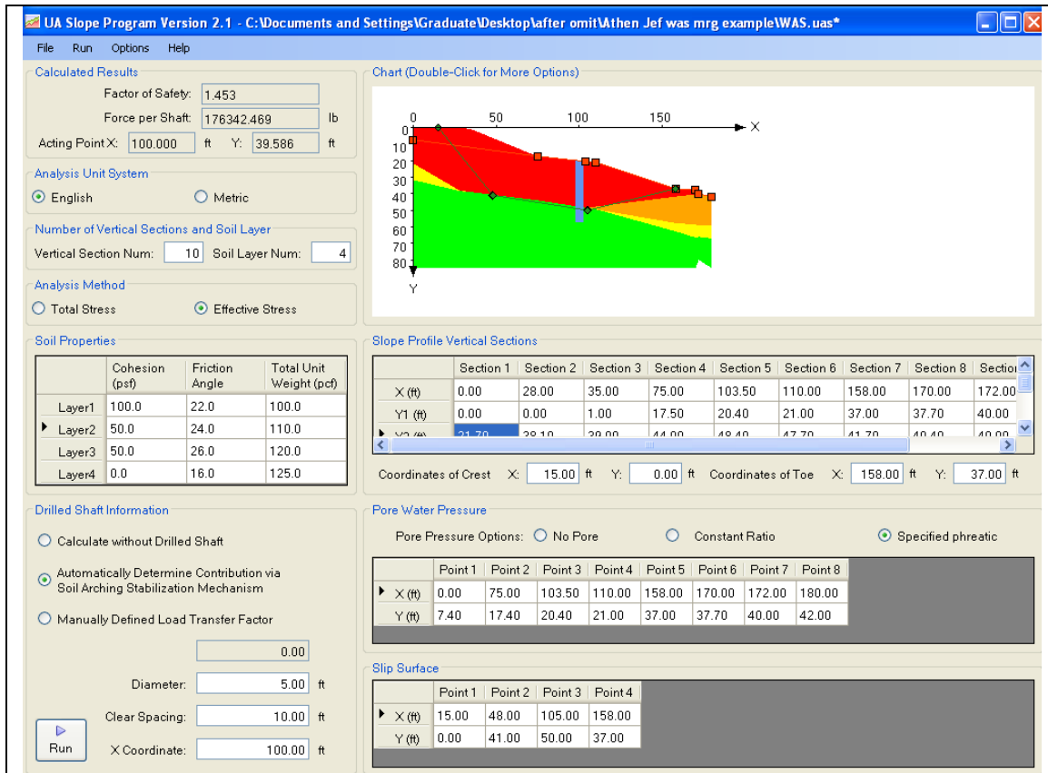
Figure 5.31: UA SLOPE 2.1 Analysis Results: b) with Drilled Shaft
