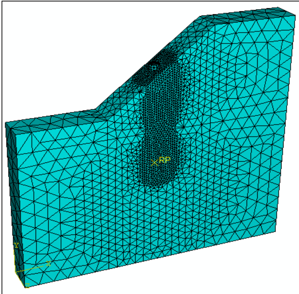
Figure 2.2: 3D Finite Element Model Developed by Yamin (2007)
