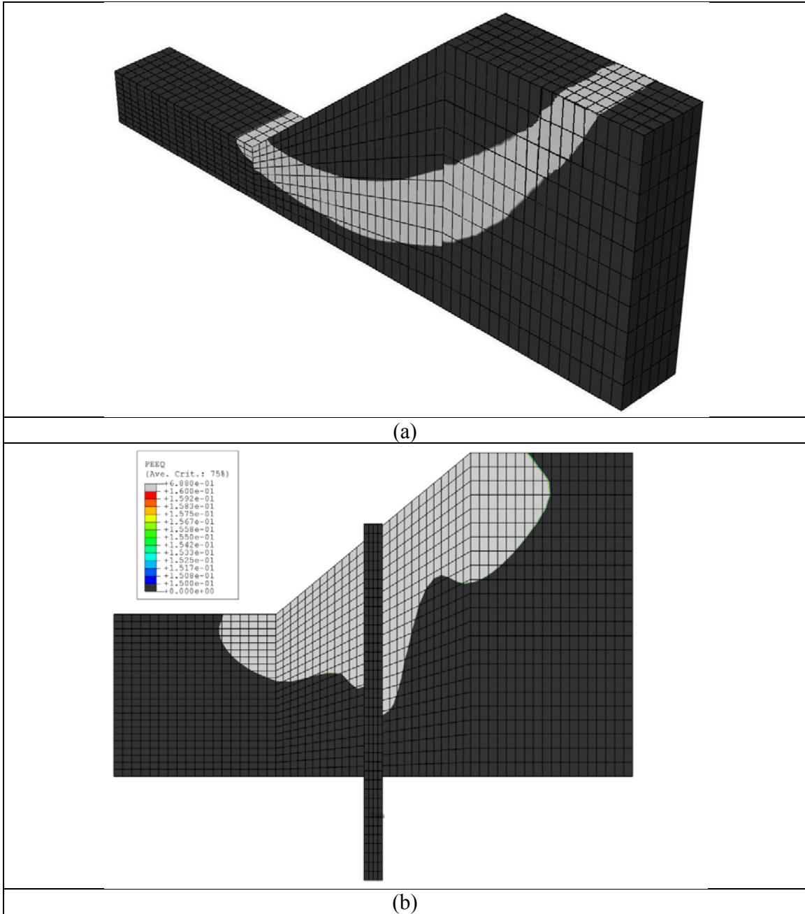
Figure 3.7 : Plastic Zone a) Failure Surface from The Equivalent Plastic Strain for the Baseline Model b) Failure Surface for a Reinforced Model
