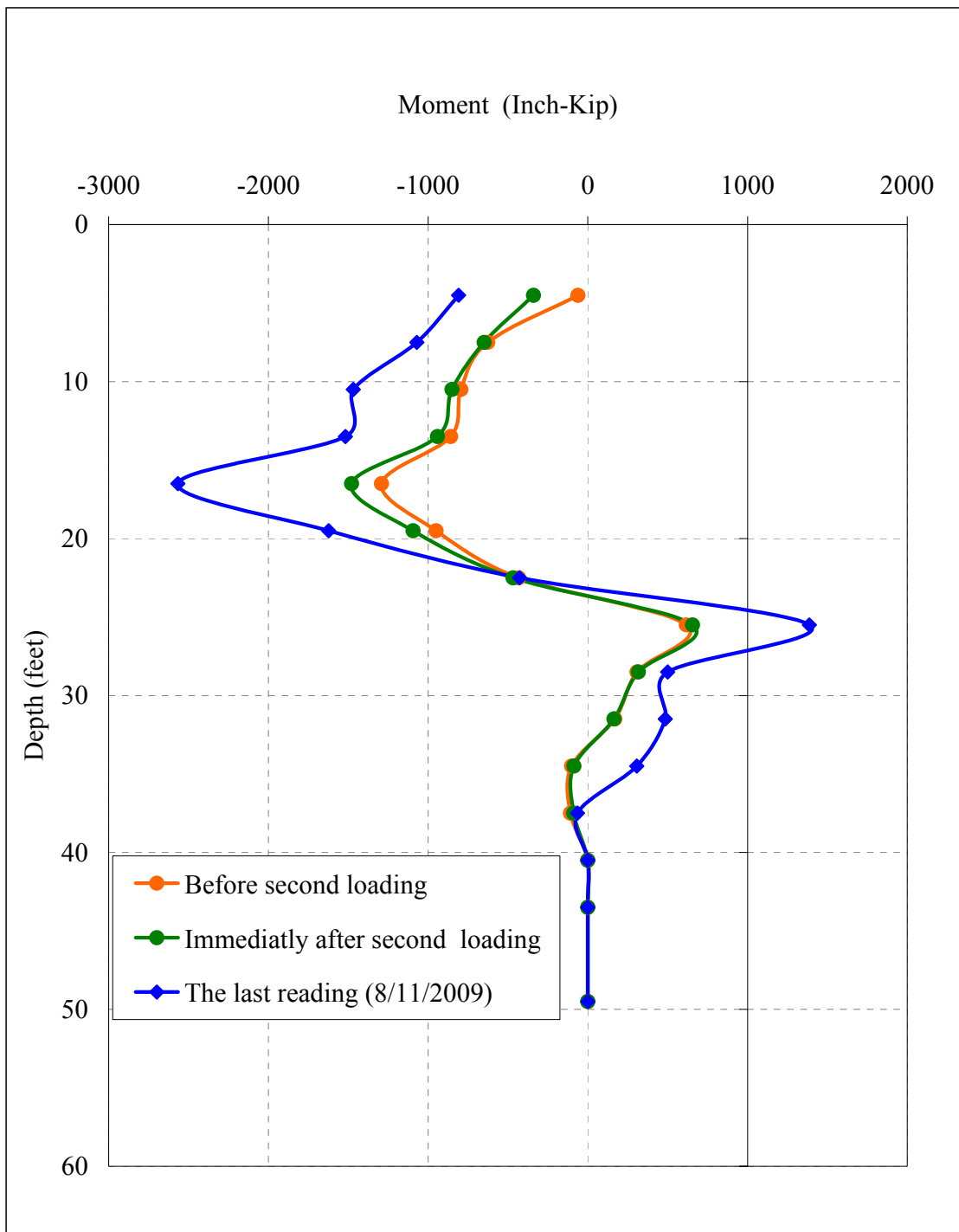
Figure 4.18: Measured Bending Moments in Shafts due to Surcharge Loading and Slope Soil Movement: (b) Shaft #4
