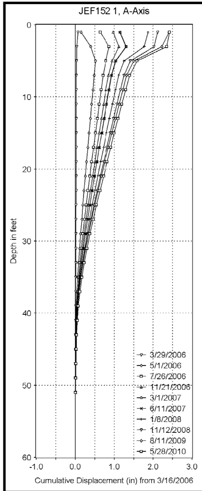
Figure 5.10: The Cumulative Deflection in Shaft #20 at JEF-152 (Inclinometer #1)
