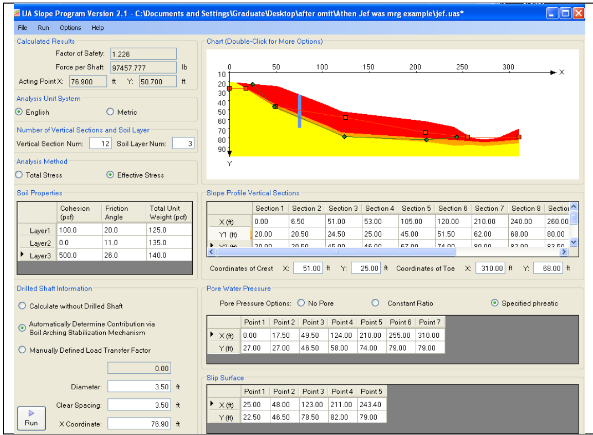
Figure 5.16: UA SLOPE 2.1 Analysis Results: b) with Drilled Shaft
