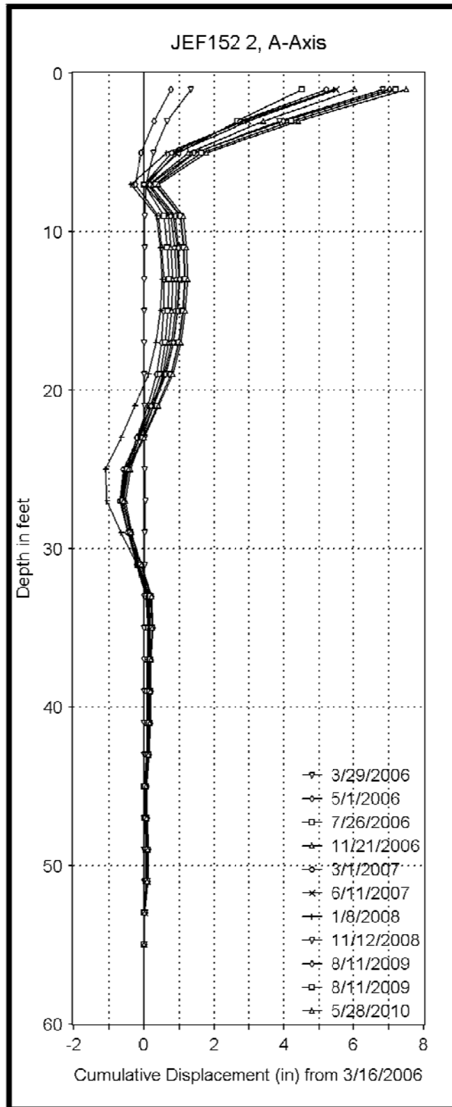
Figure 5.11: The Cumulative Deflection in Shaft #21 at JEF-152 (Inclinometer #2)
