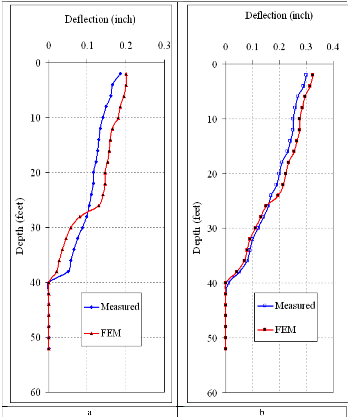
Figure 4.25: Comparison between Measured and FEM Computed Deflections for Shaft #4: (a) due to First Loading, and (b) due to Second Loading
