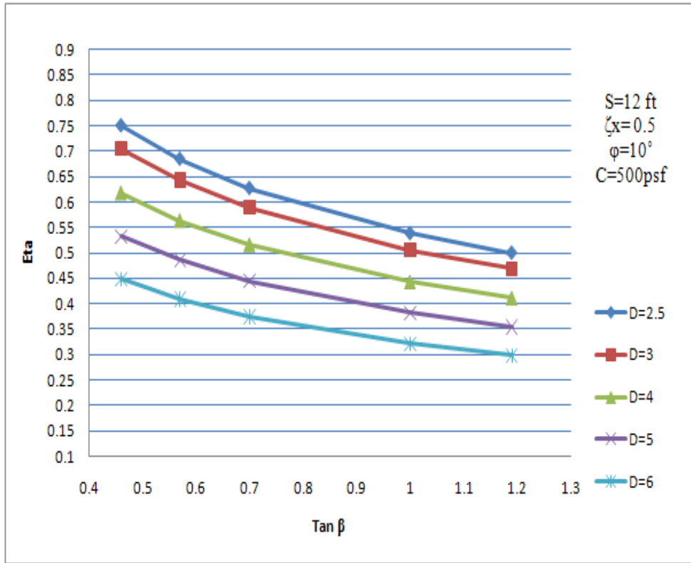
Figure 3.14: Variation of \eta Versus Shaft Diameter and \tan \beta .
