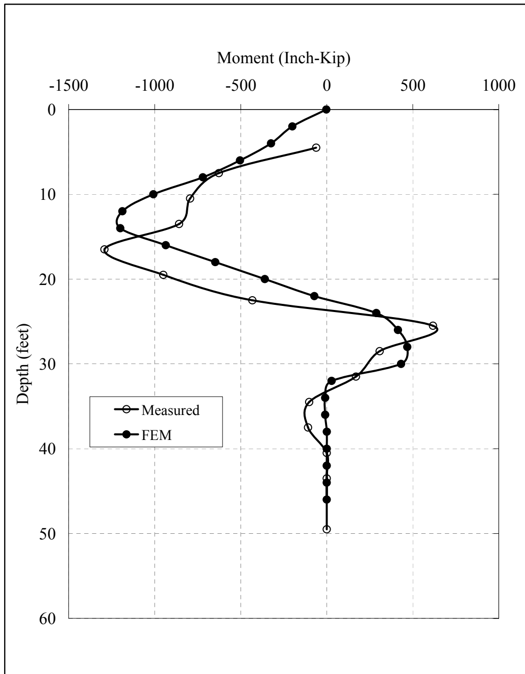
Figure 4.27: Comparison between Measured and FEM Measured Moments in Shaft #4: (a) due to First loading
