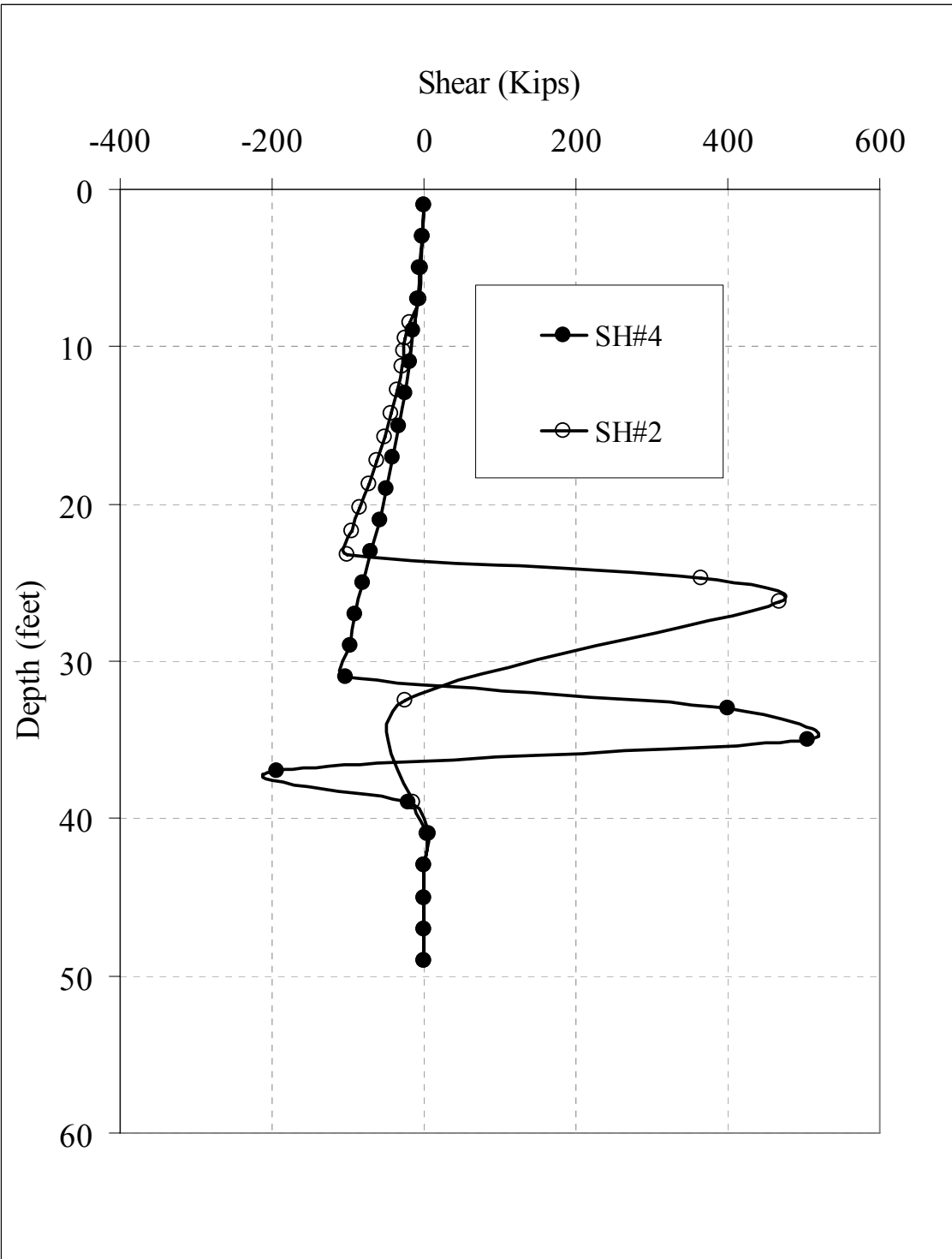
Figure 4.32: Computed Shear in Drilled Shafts at Extreme Surcharge Loads
