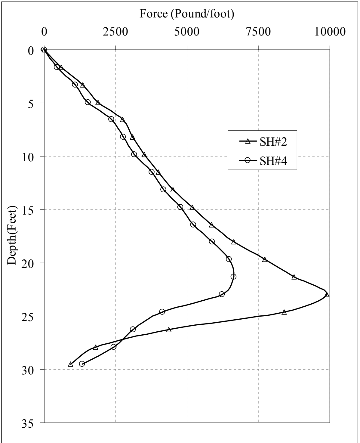
Figure 4.33: Computed Net Soil Reaction Force at Extreme Surcharge Loads
