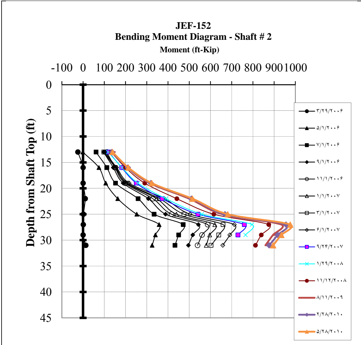
Figure 5.13: Measured Moments along Shaft #21 at JEF-152 Site
