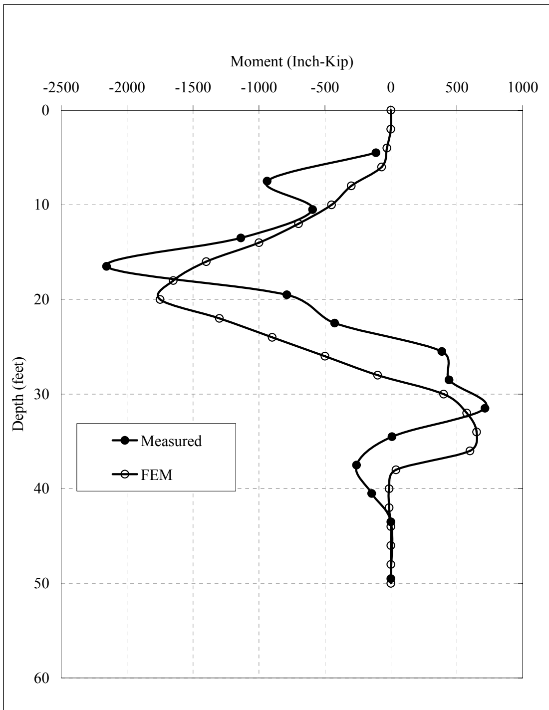
Figure 4.26: Comparison between Measured and FEM Computed Moments in Shaft #2: (a) due to First loading
