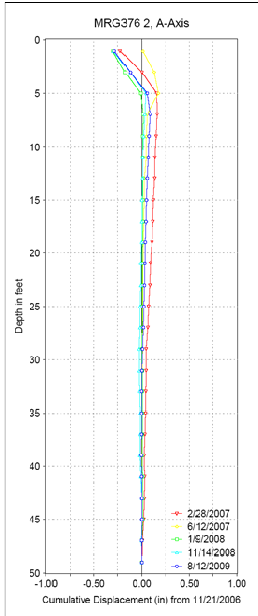
Figure 5.42: Cumulative Deflection of Shaft #10 at MRG-376 (Inclinometer #2)
