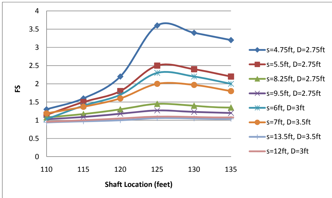
Figure 4.6: Factor of Safety of the Slope/Shaft System versus Shaft Location for Different (S, D) Combinations
