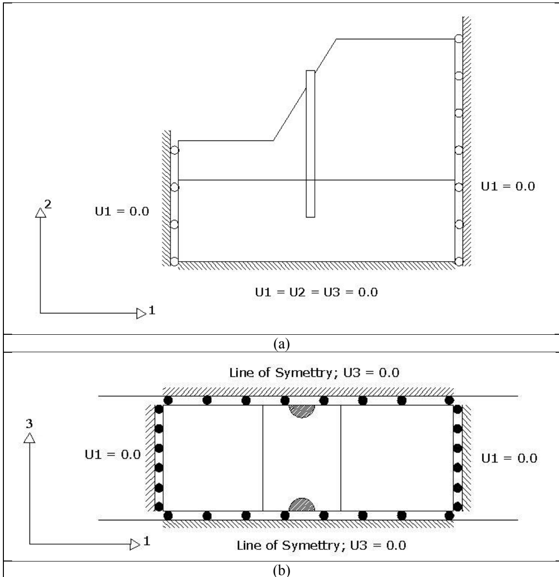
Figure 3.2: Boundary Conditions Used in the Finite Element Model (a) Elevation View (b) Top View
