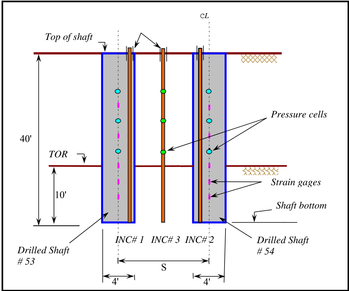
Figure 5.21: WAS-7 Instrumentation Plans (Cross-section 2)
