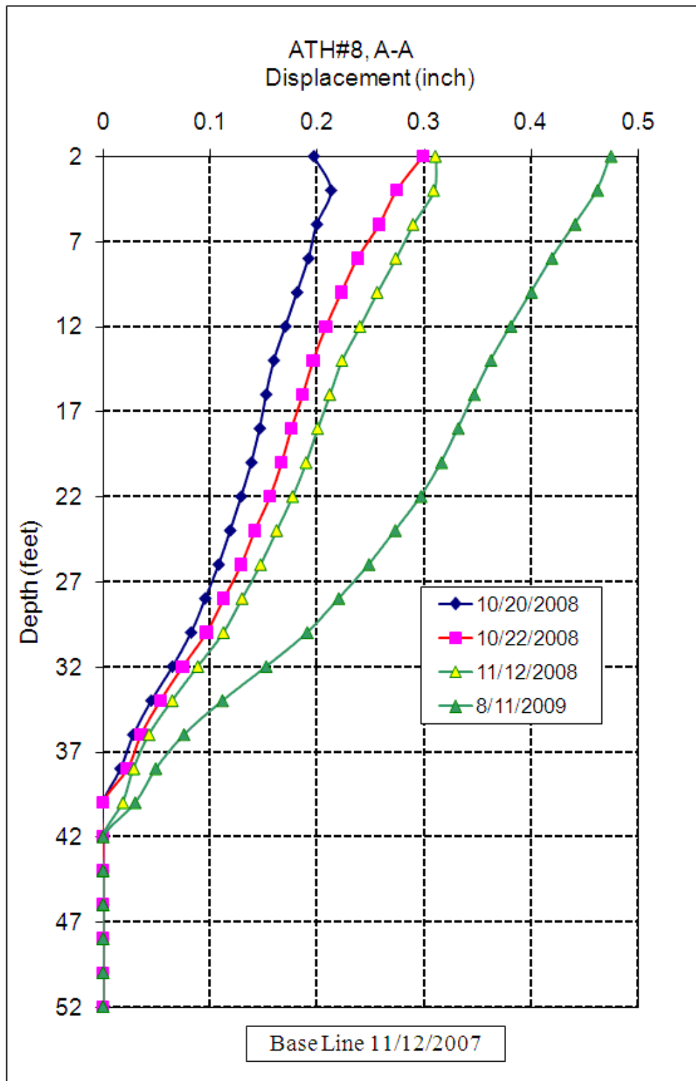
Figure 4.16: Measured Cumulative Deflections: (b) Shaft #4
