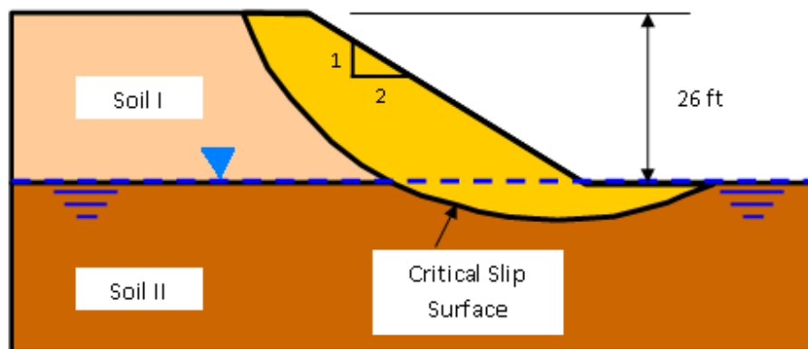
Figure 4.7: The Slope Geometry, Soil Profile, Slip Surface, and Ground Water Table for the Illustrative Example
