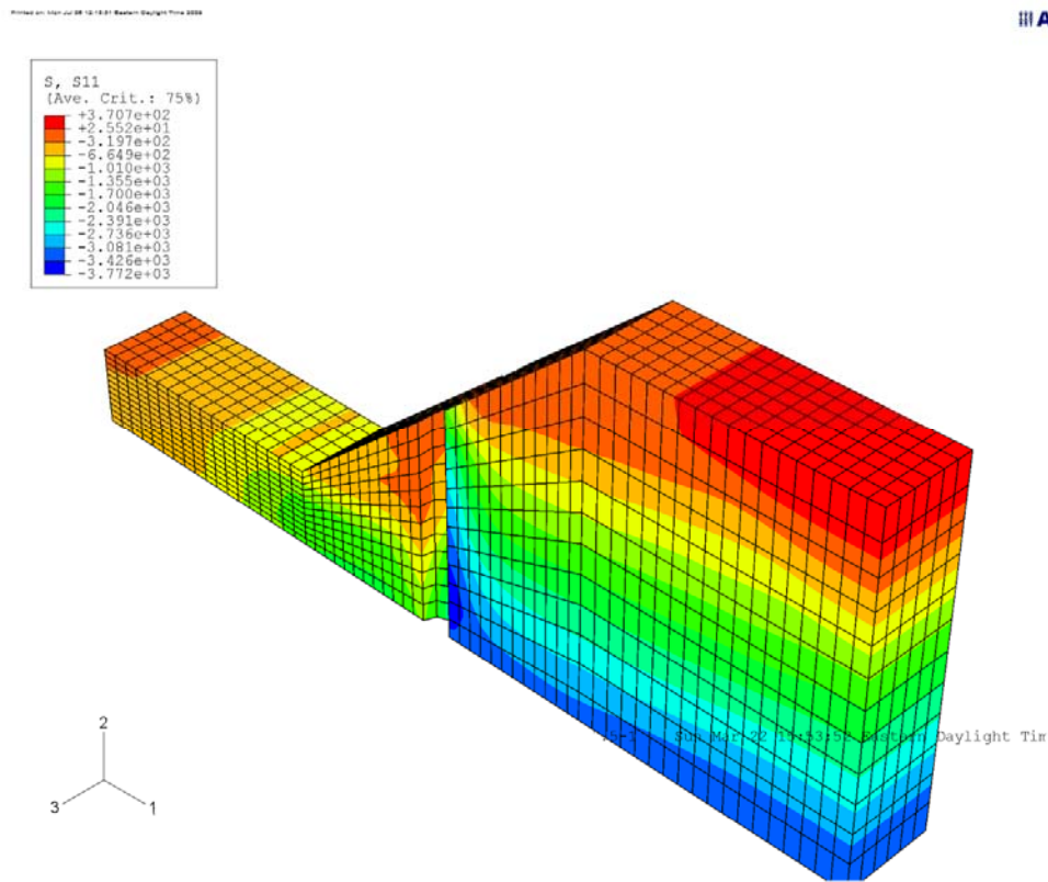
Figure 3.10: Horizontal Stresses at Failure (3D Isometric Stress Contours )
