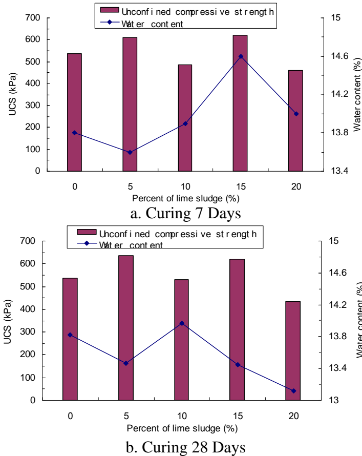
FIGURE 13 Summary of Lime sludge Content versus Unconfined Compressive Strength for Soil 1A
