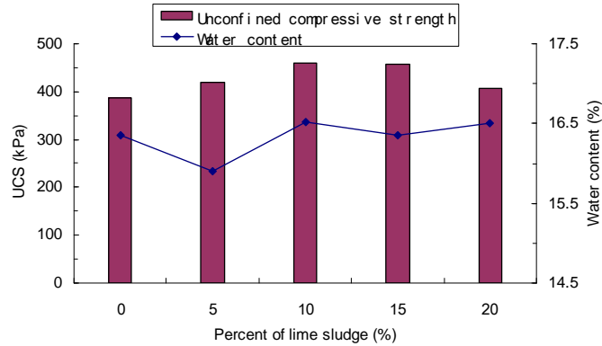
FIGURE 21 Lime sludge Content versus Unconfined Compressive Strength
