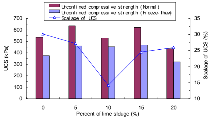
Figure 28 Lime Sludge Content versus Unconfined Compressive Strength under Normal Curing versus Subjected to Freezing-Thawing
