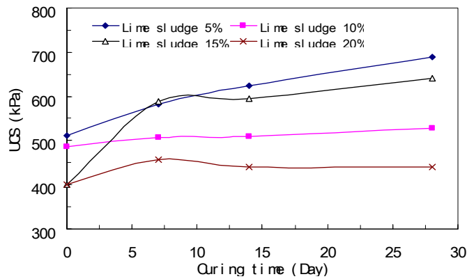
Figure 14 The Relationship of Curing Time to the Unconfined Compressive Strength with Different Lime Sludge Percentage
