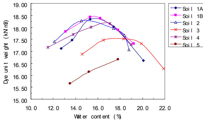
FIGURE 4 Compaction Curves of Five Soils
