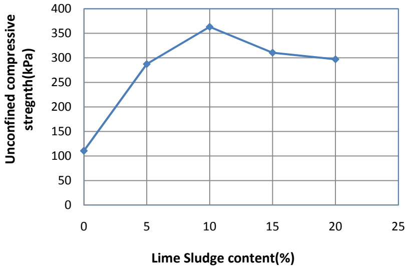
FIGURE 26 Lime sludge Content versus Unconfined Compressive Strength
