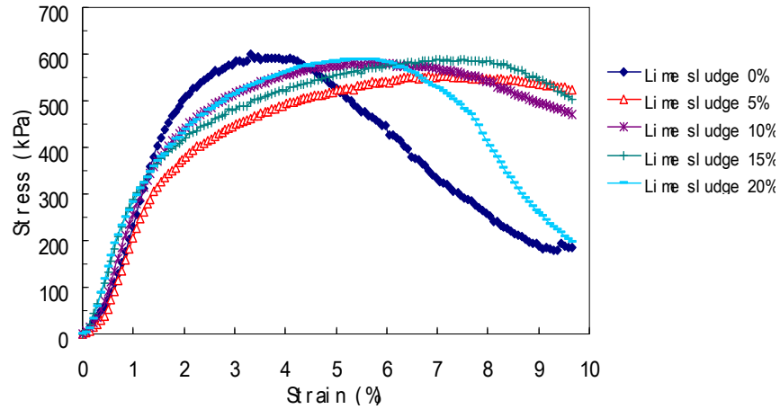
Figure 23 Stress-Strain Relationship of Soil Specimens with Different Lime Sludge Incorporating Ratio
