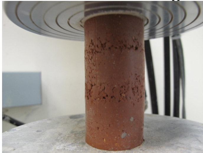
FIGURE 9 PICTURE of the Soil Specimen on the Apparatus
