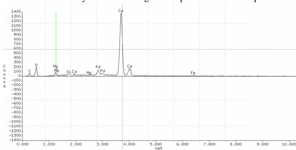
FIGURE 2 EDX Spectral of Measured Dry Lime Sludge Sample
