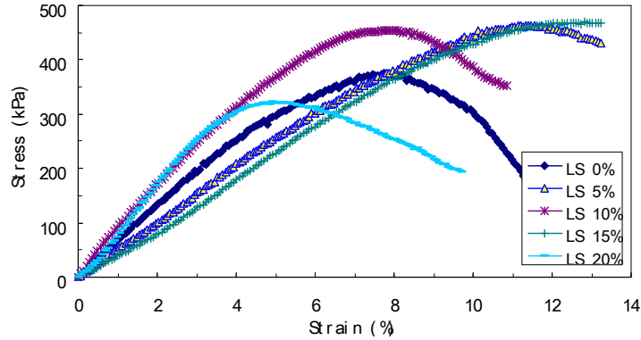
Figure 27 Stress-Strain Curves for Soil Specimens Treated with Different Lime Sludge Ratio subjected to Freeze-Thawing Cycles
