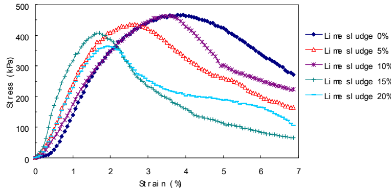
Figure 17 Stress-Strain Relationship of Soil Specimens with Different Lime Sludge Incorporating Ratio
