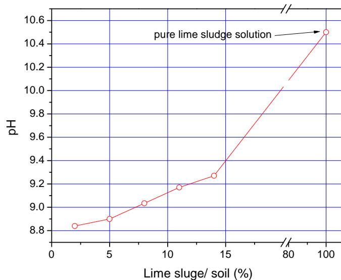
FIGURE 10 pH Test for estimating Soil-Lime Sludge Proportion.
