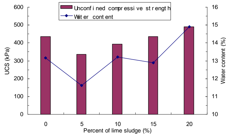
FIGURE 16 Lime sludge Content versus Unconfined Compressive Strength
