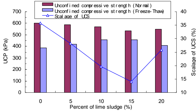
Figure 31 Lime Sludge Content versus Unconfined Compressive Strength under Normal Curing versus Subjected to Freezing-Thawing
