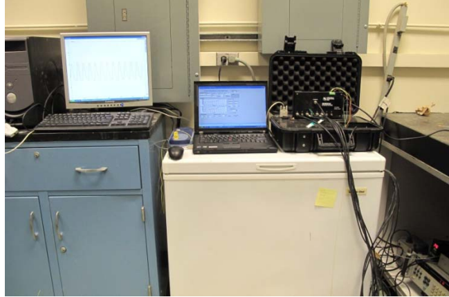
Figure 10 Picture of Freeze-Thaw Testing Apparatus System
