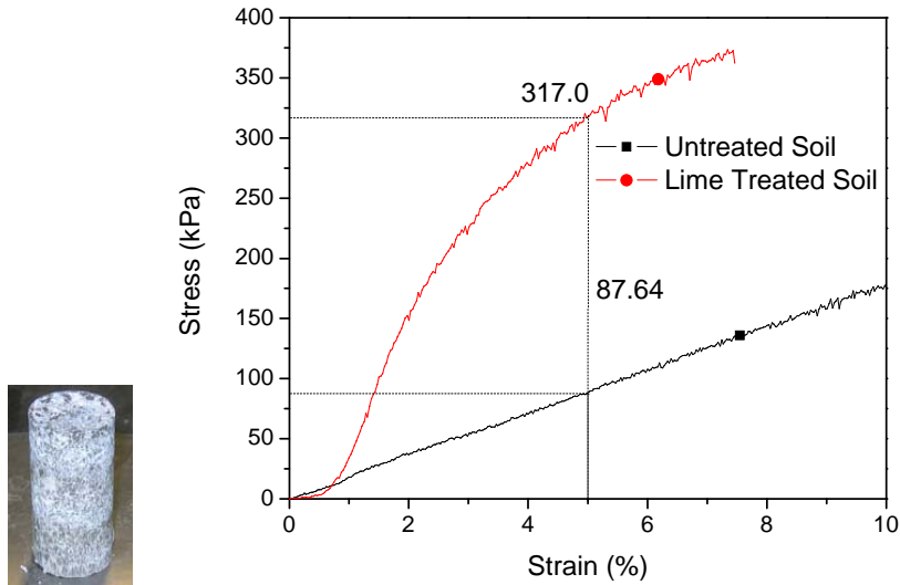
FIGURE 25 Deformation behaviors of soil specimen treated with lime sludge versus that of natural untreated soil
