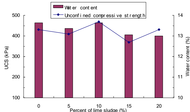
FIGURE 18 Lime sludge Content versus Unconfined Compressive Strength
