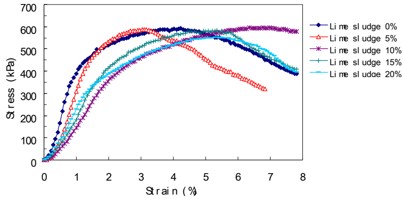
Figure 19 Stress-Strain Relationship of Soil Specimens with Different Lime Sludge Incorporating Ratio
