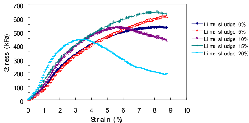
Figure 11 Stress-Strain Relationships of Soil Specimens with Different Lime Sludge Incorporating Ratio
