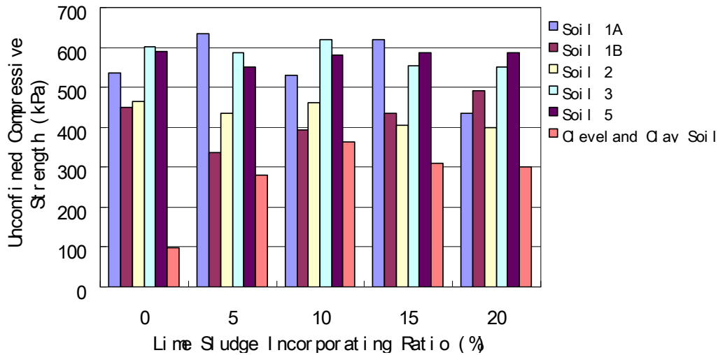
Figure 27 Effect of Unconfined Compressive Strength on Lime Sludge Ratio of Different Soil
