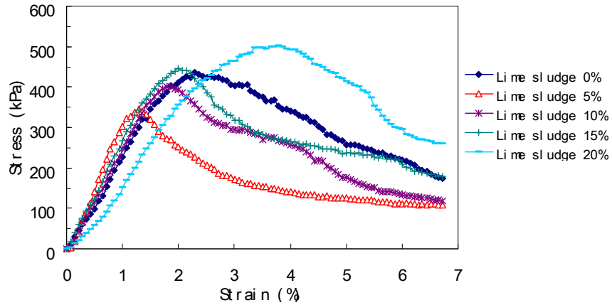
Figure 15 Stress-Strain Relationship of Soil Specimens with Different Lime Sludge Incorporating Ratio
