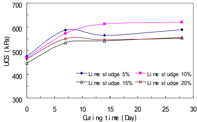
Figure 22 The Relationship of Curing Time to the Unconfined Compressive Strength with Different Lime Sludge Percentage
