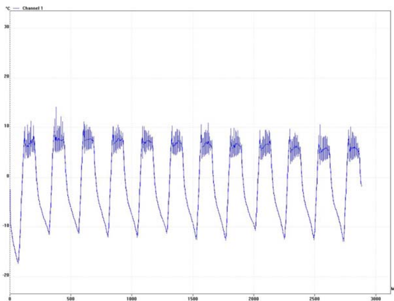
Figure 11 Temperature Curve Showing the Freezing-Thawing Cycles
