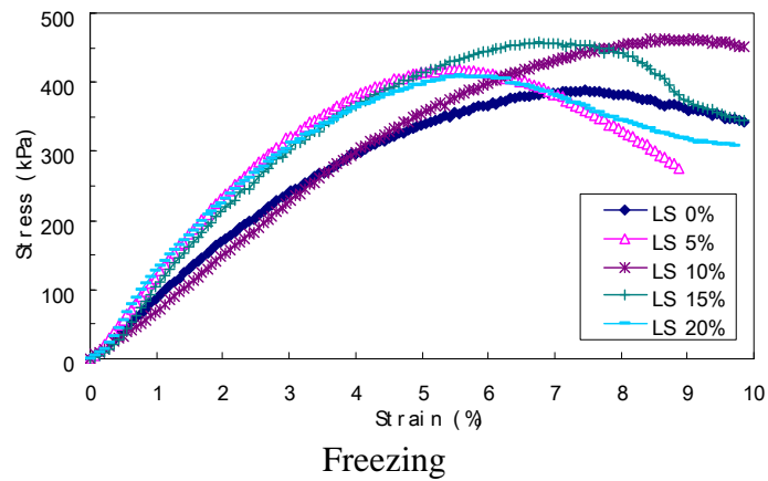
Figure 30 Stress-Strain Curves for Soil Specimens Treated with Different Lime Sludge Ratio subjected to Freeze-Thawing Cycles
