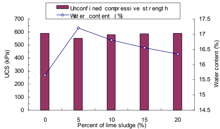
FIGURE 24 Lime sludge Content versus Unconfined Compressive Strength
