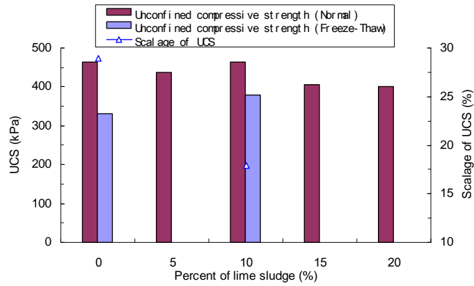
Figure 29 Lime Sludge Content versus Unconfined Compressive Strength under Normal Curing versus Subjected to Freezing-Thawing
