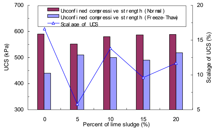
Figure 33 Lime Sludge Content versus Unconfined Compressive Strength under Normal Curing versus Subjected to Freezing-Thawing
