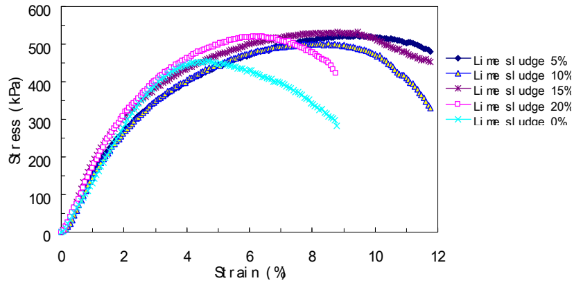
Figure 32 Stress-Strain Curves for Soil Specimens Treated with Different Lime Sludge Ratio subjected to Freeze-Thawing Cycles
