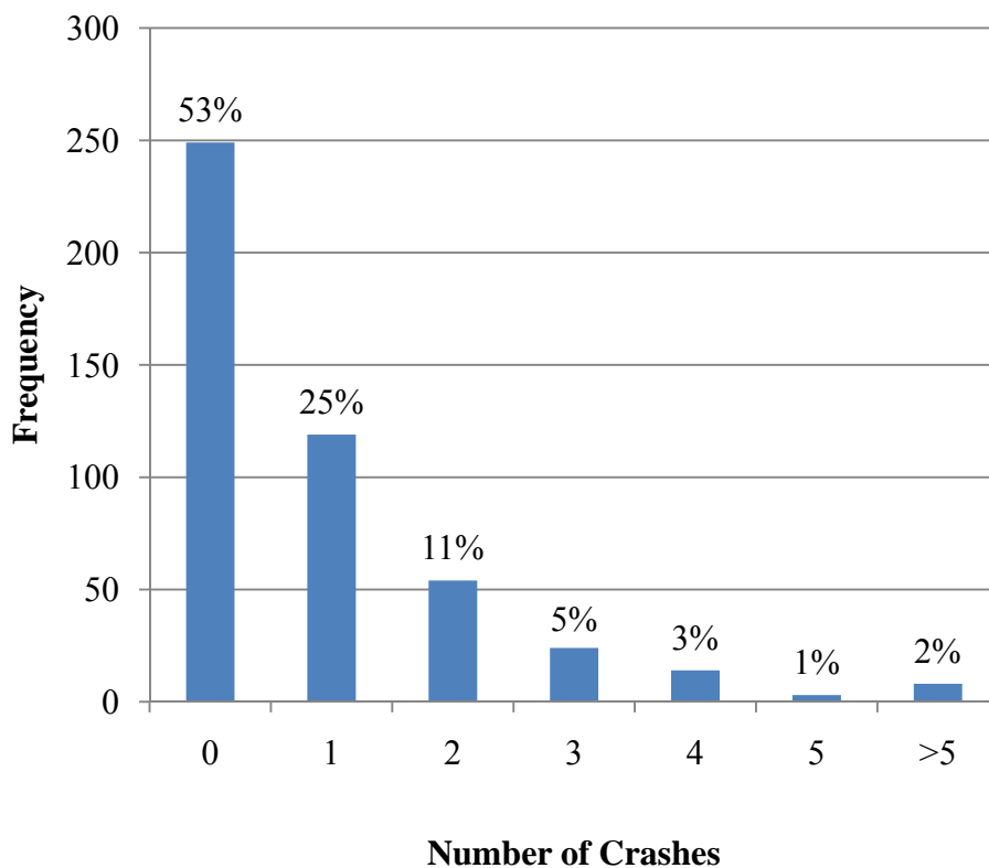
Figure 4-10: Histogram of crash counts on each segment for individual years.
