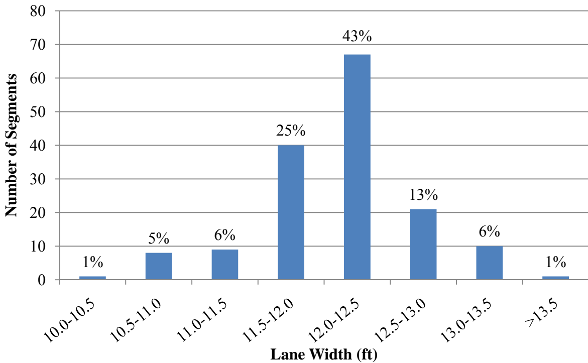
Figure 4-5: Histogram of lane widths for study segments.
