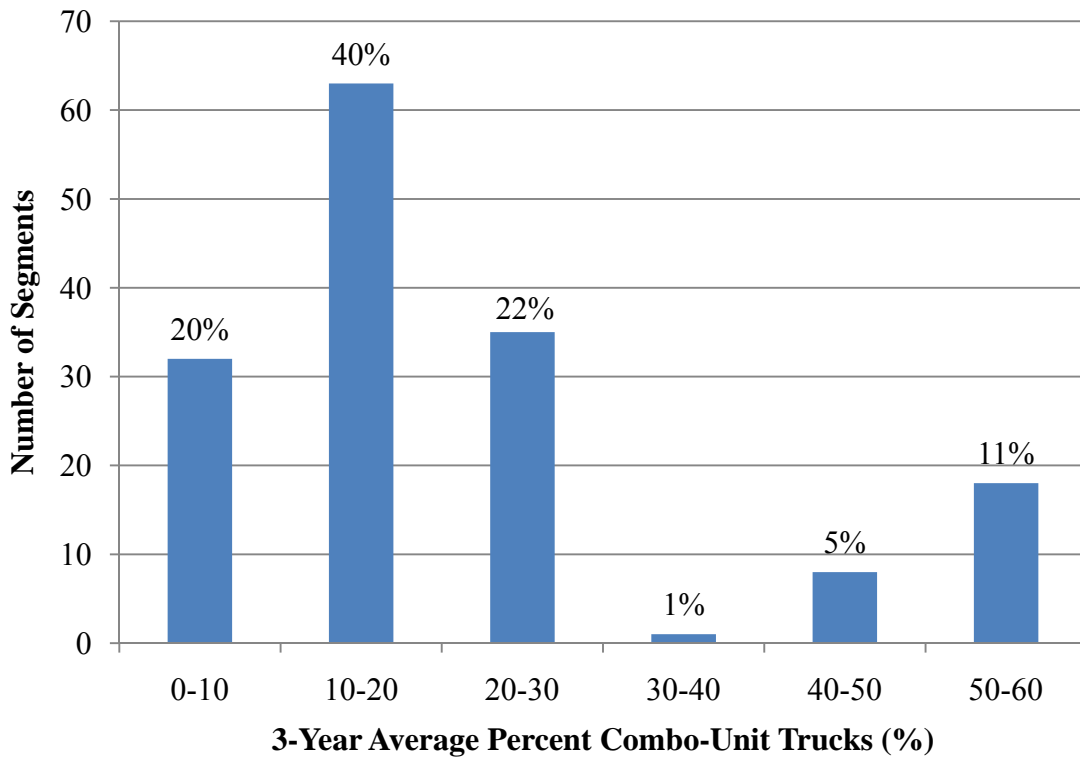
Figure 4-9: Three year average of combo-unit trucks as percent of AADT.
