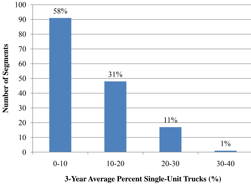
Figure 4-8: Three year average of single-unit trucks as percent of AADT.
