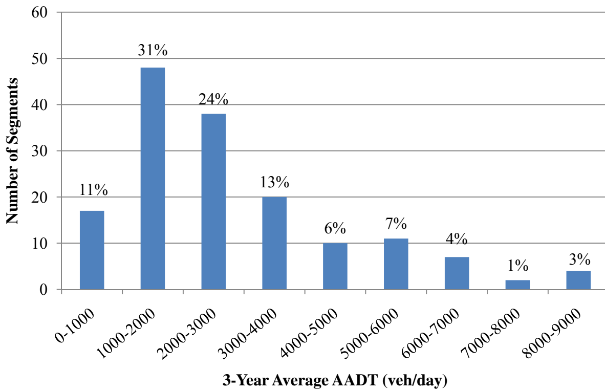
Figure 4-7: Histogram of average value of AADT over three years.
