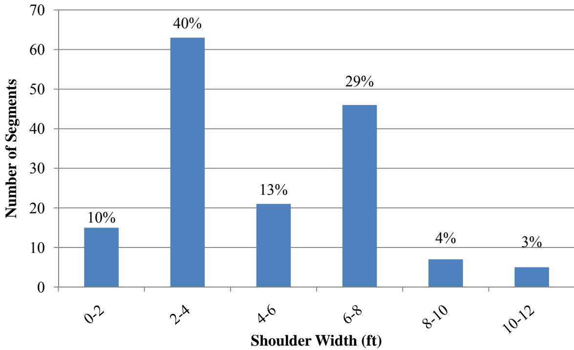
Figure 4-6: Histogram of shoulder widths for study segments.
