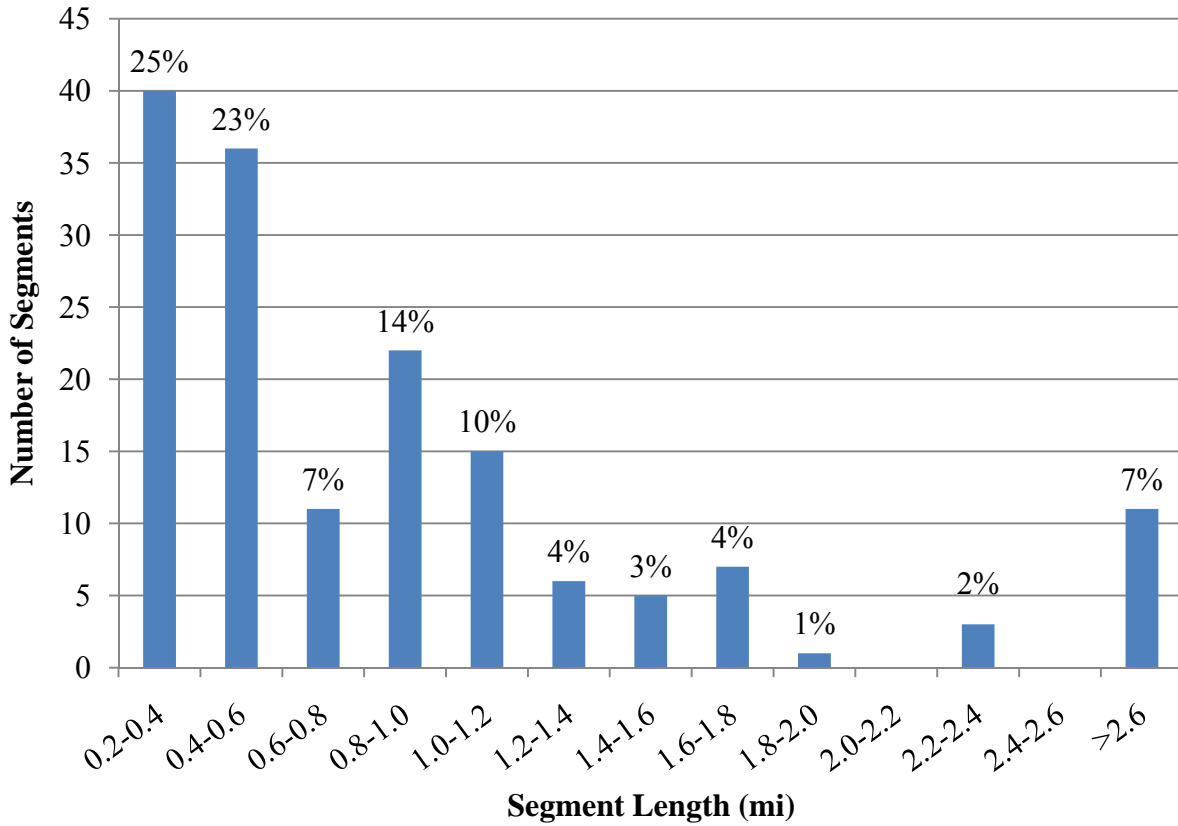
Figure 4-4: Histogram of segment length.
