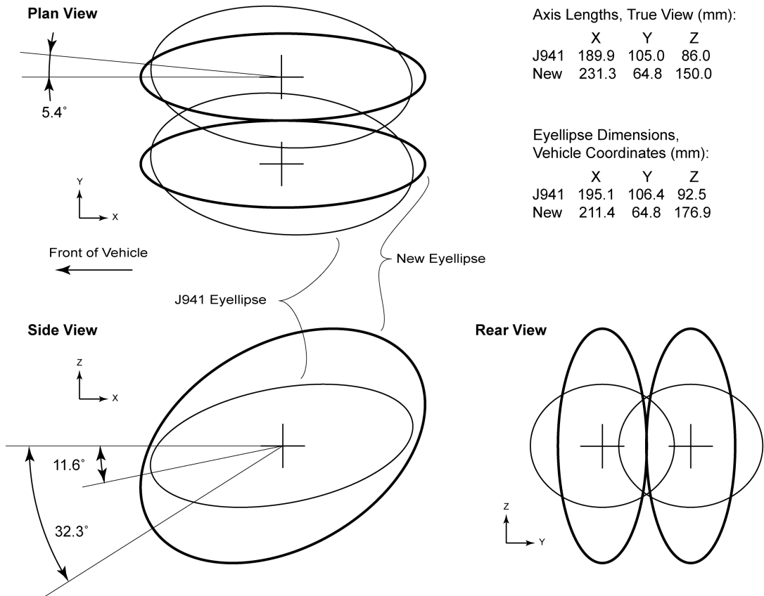
Figure 6. Comparison of J941 and new eyellipses for a 50/50 gender mix and seat track length >133 mm (J941). The new eyellipse was configured with the population from Table 7. Eyellipses are shown with the same centroid, although differences in the locator equations will usually result in different centroids.
