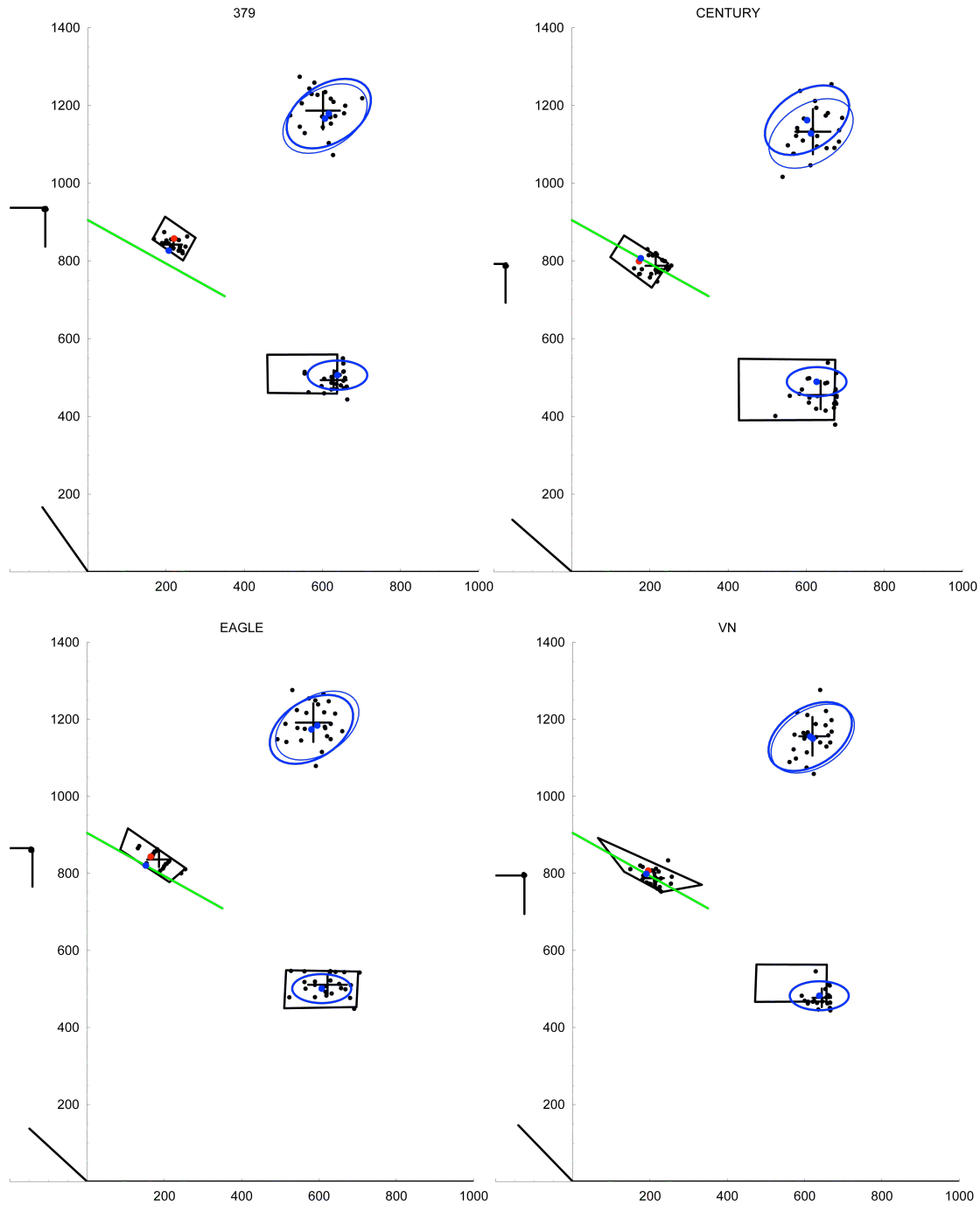
Figure 8. Comparison of accommodation models to in-vehicle driver data for four Class-8 cabs. Driver data are shown with black dots. Steering wheel and seat adjustment ranges are shown with black lines. Green line is steering wheel preference model. The seat position model is shown as 95% cutoff ellipse. The eyellipse based on mean predicted seat position is shown with a thick line. The eyellipse with a thin line is based on mean observed seat position.
