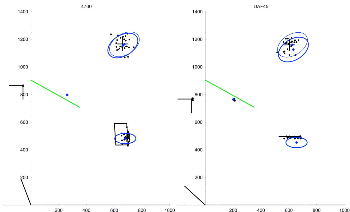
Figure 8 (continued). Comparison of accommodation models to in-vehicle driver data for two straight-truck cabs. Driver data are shown with black dots. Steering wheel and seat adjustment ranges are shown with black lines. Green line is steering wheel preference model. The seat position model is shown as 95% cutoff ellipse. The eyellipse based on mean predicted seat position is shown with a thick line. The eyellipse with a thin line is based on mean observed seat position.
