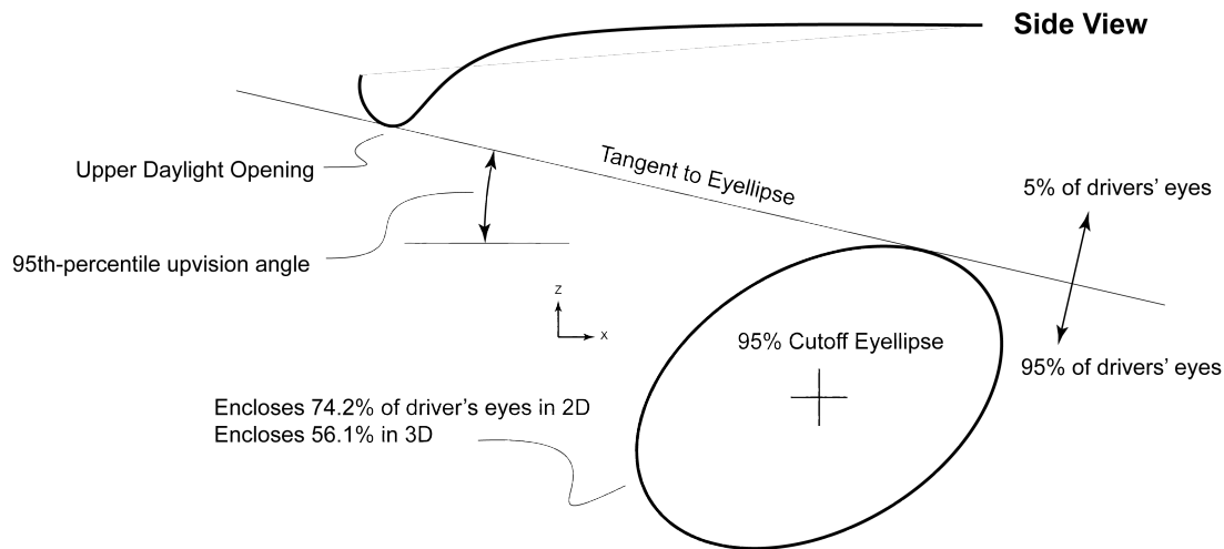
Figure 1. Illustration of side-view eyellipse with 95% cutoff characteristic.
