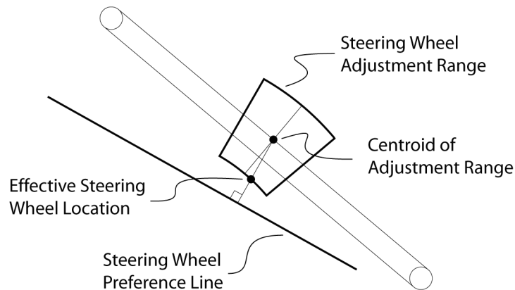
Figure 7. Calculating effective steering wheel location for a case in which the preference line does not pass through the adjustment range.
