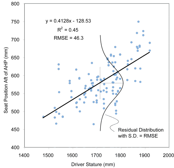
Figure 2. Plot of stature vs. fore-aft seat position for one test condition in the laboratory to illustrate regression analysis principles.
