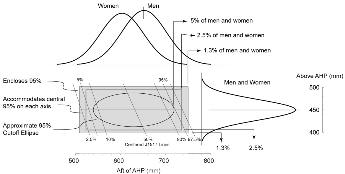
Figure 3. Calculating two-dimensional seat-position accommodation for the driver population in Table 7. Normal approximations to male and female seat position distributions are shown.
