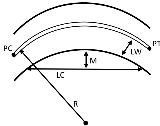
Figure 8. Horizontal Curve Layout [Findley and Foyle 2009]
