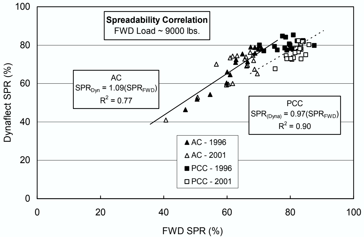
Figure 2.8 Correlation of FWD and Dynaflect Responses on SHRP Test Sections
