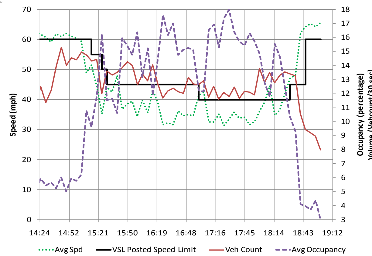
Figure S1.13.9. VSL System trigger point (13 th November 08) for detector 8D
