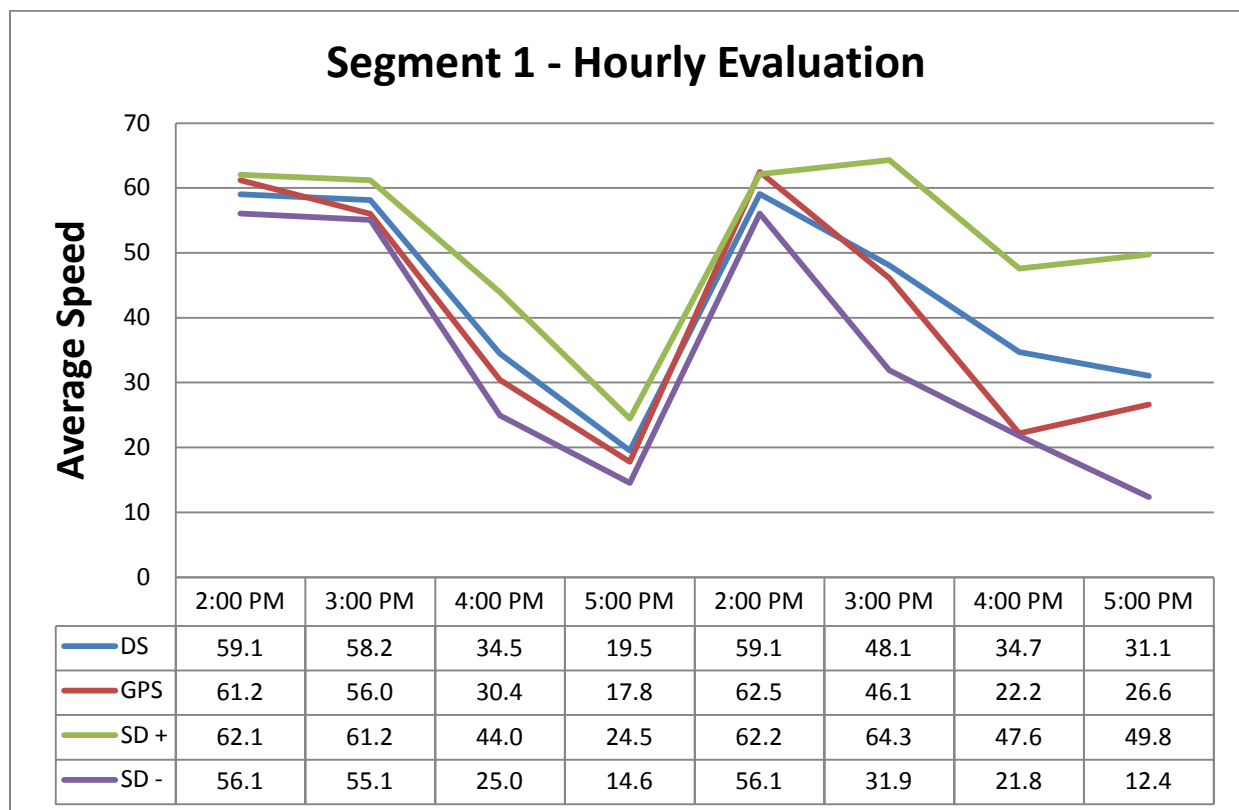
Figure 2.1. Segment #1 – Average Speed Comparison for Two Days' - PM Peak Periods
