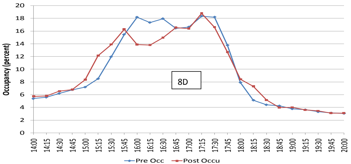
Figure S1.11.5 Comparison of Pre (Nov, 2007) and Post-VSL (Nov, 2008) Occupancy Profile
