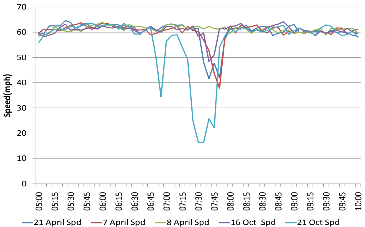
Figure S4.12.3 Post-VSL Speed Profile for five days at Detector 31D
