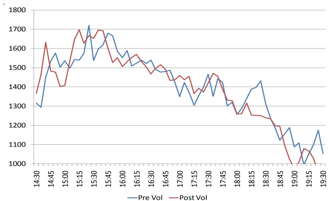
Figure S3.11.3 Comparison of Pre (Nov, 2007) and Post-VSL (Nov, 2008) Volume 25D
