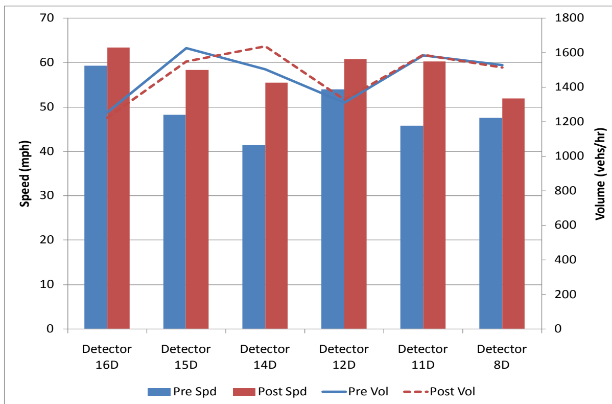
Figure S1.12.4. Comparison of Pre (25 th Oct, 07) and Post-VSL (23 rd Oct, 08) Average Speed and Volume
