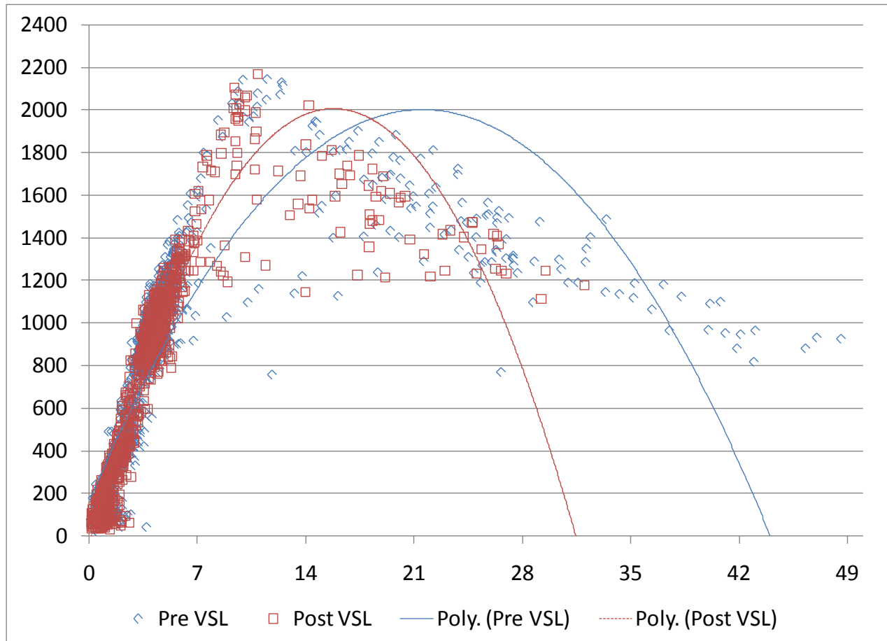
Figure S2.11.5. Flow-Occupancy Plot for 3D for Five days
