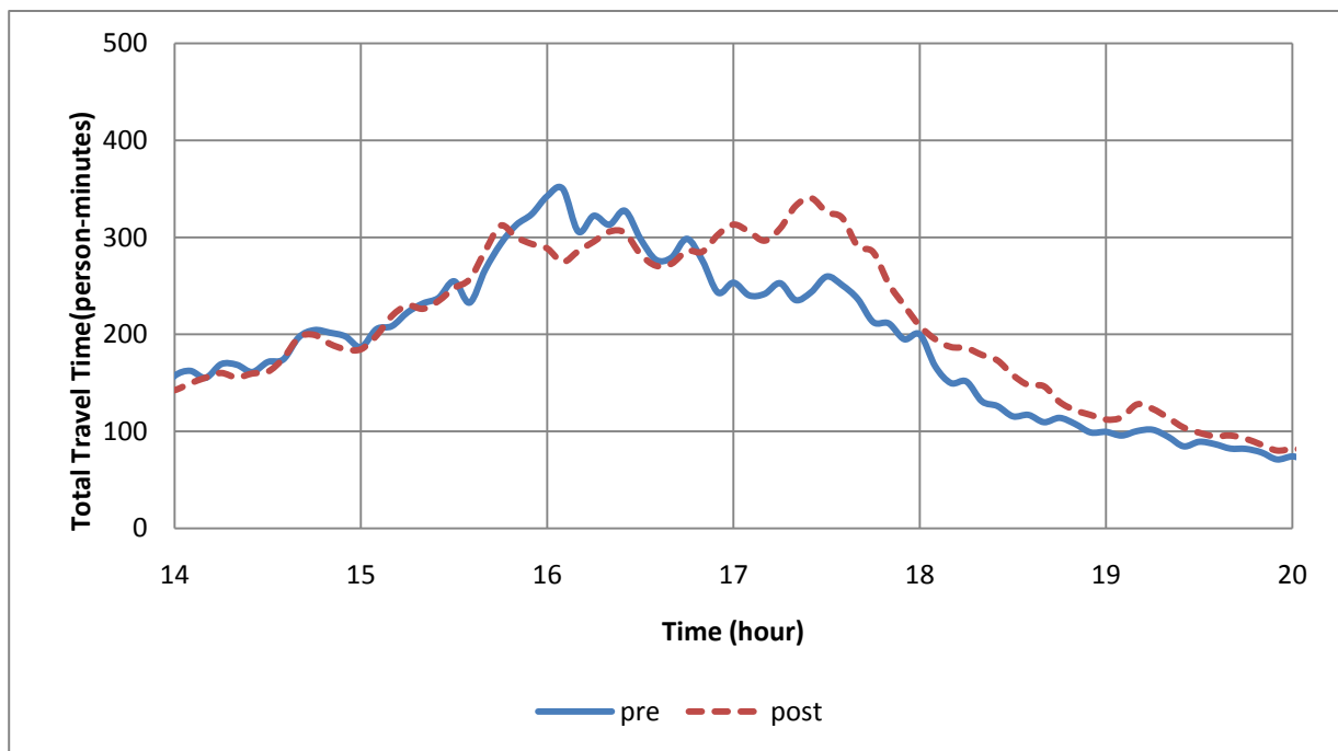
Figure S1.16.1 Comparison of Pre and Post-VSL average travel time data between 12D and 11D (October)
