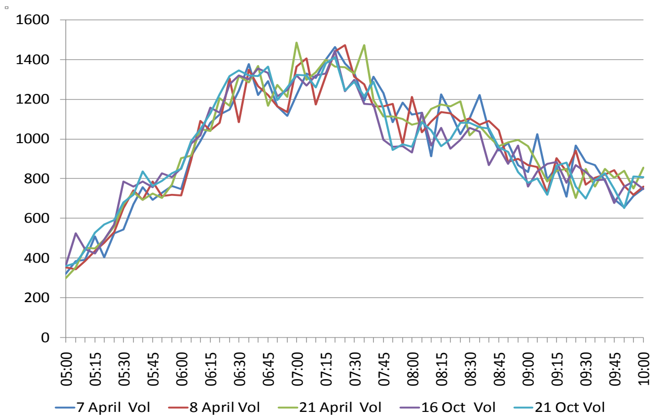
Figure S4.11.3 Post VSL Volume Profile for five days
