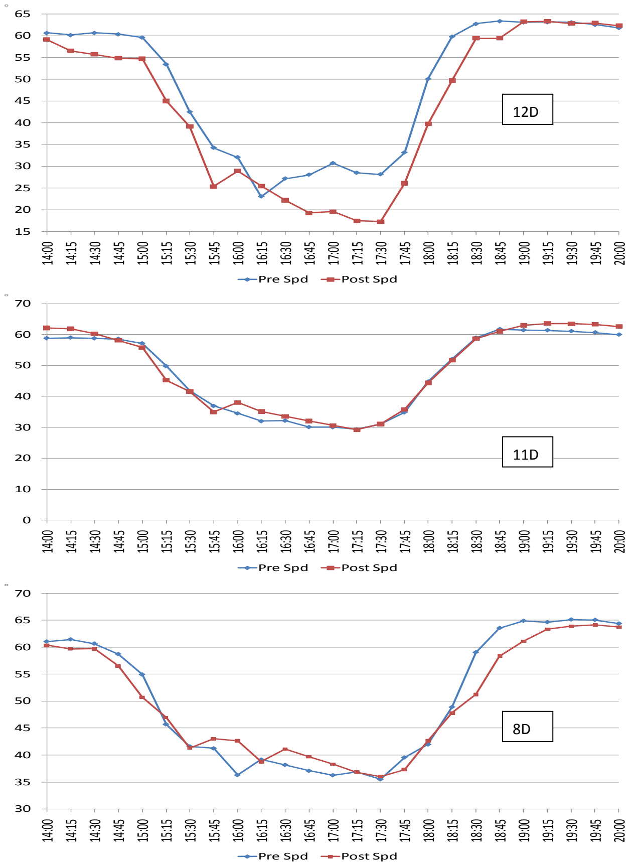
Figure S1.12.3 Comparison of Pre (April, 2008) and Post-VSL (April, 2009) Speed Profile
