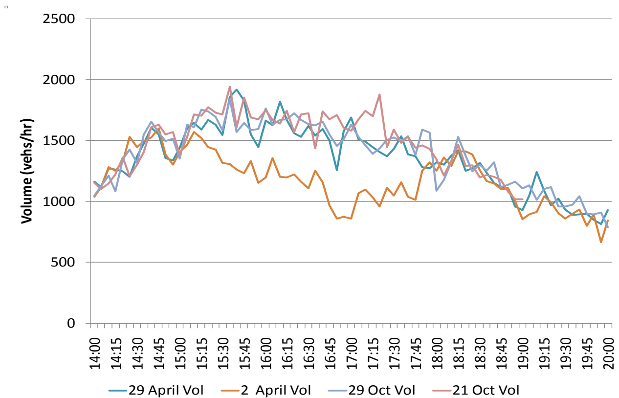
Figure S3.11.3 Post-VSL Volume Profile for four days
