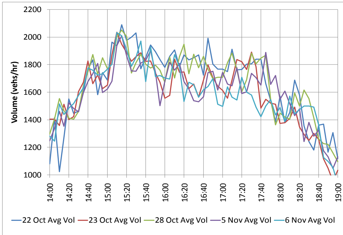
Figure S1.11.3 Post VSL Volume Profile for five days
