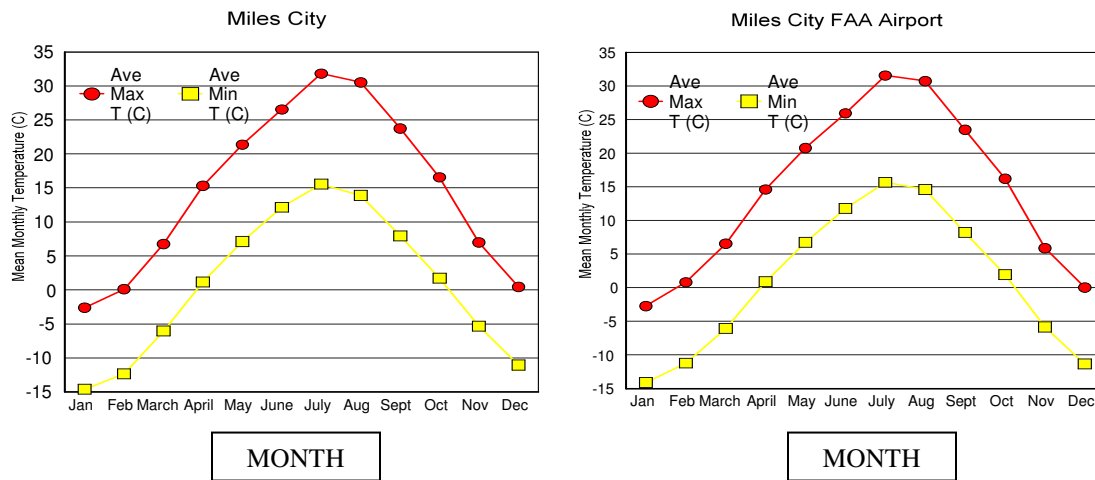
Figure 13. Mean monthly maximum and minimum temperatures for Miles City and Miles City FAA Airport climate stations.
