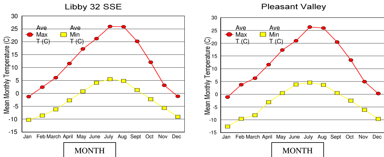
Figure 3. Mean monthly maximum and minimum temperatures at climate stations near the Happs Inn research sites.
