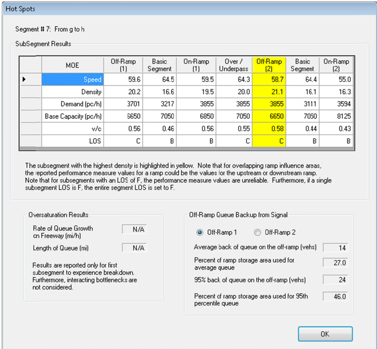
Figure 13. FREEPLAN Hot Spots screen
