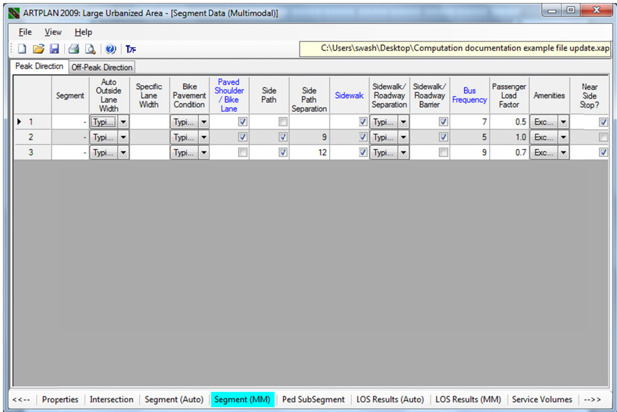
Figure 3. "Segment (MM)" screen with new inputs
