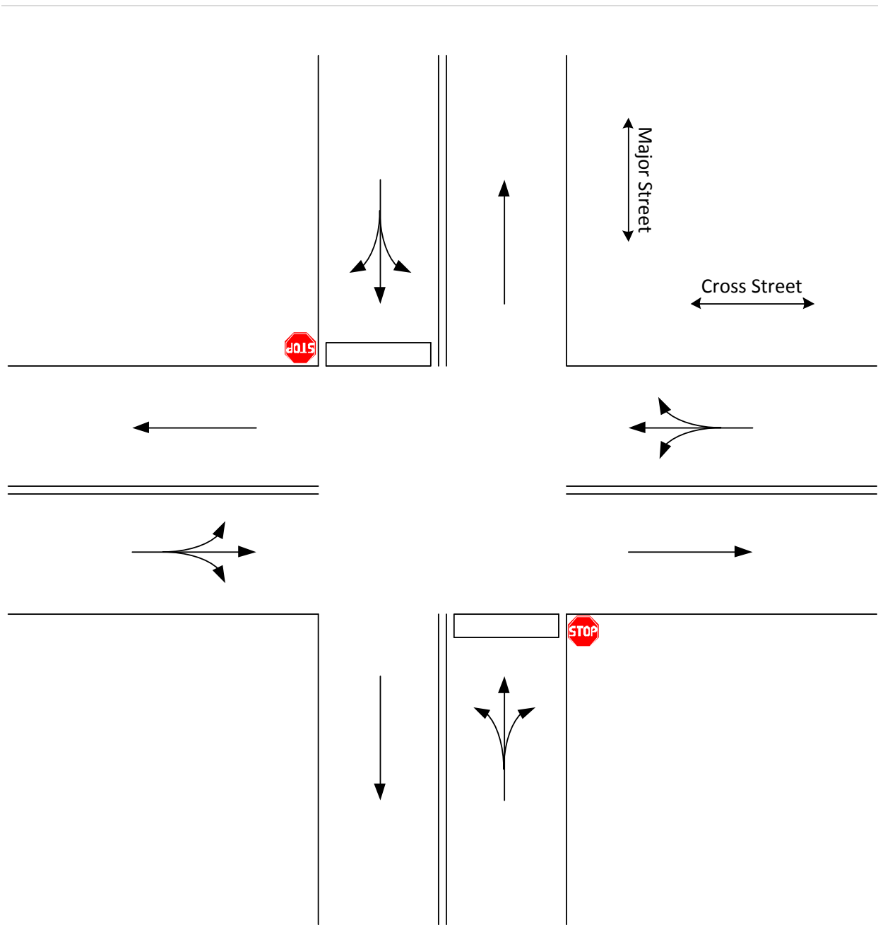
Figure 19. Two-way stop control intersection diagram with no left-turn bays
