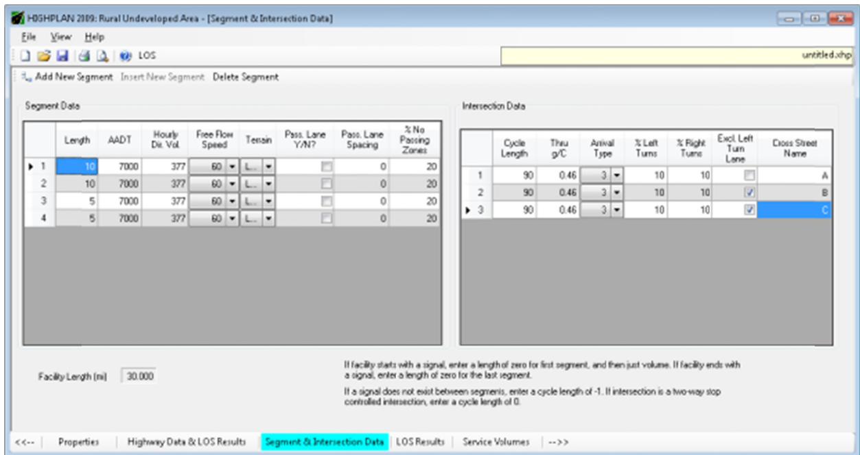
Figure 11. Two-lane highway facility inputs screen
