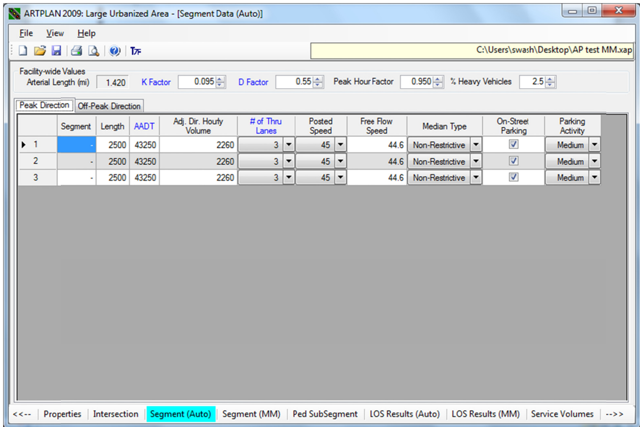
Figure 2. "Segment (Auto)" screen with new inputs
