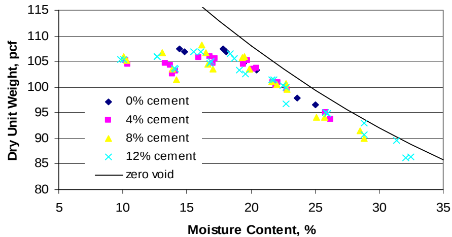
Figure 10 Compaction curves with and without cement for Soil I
