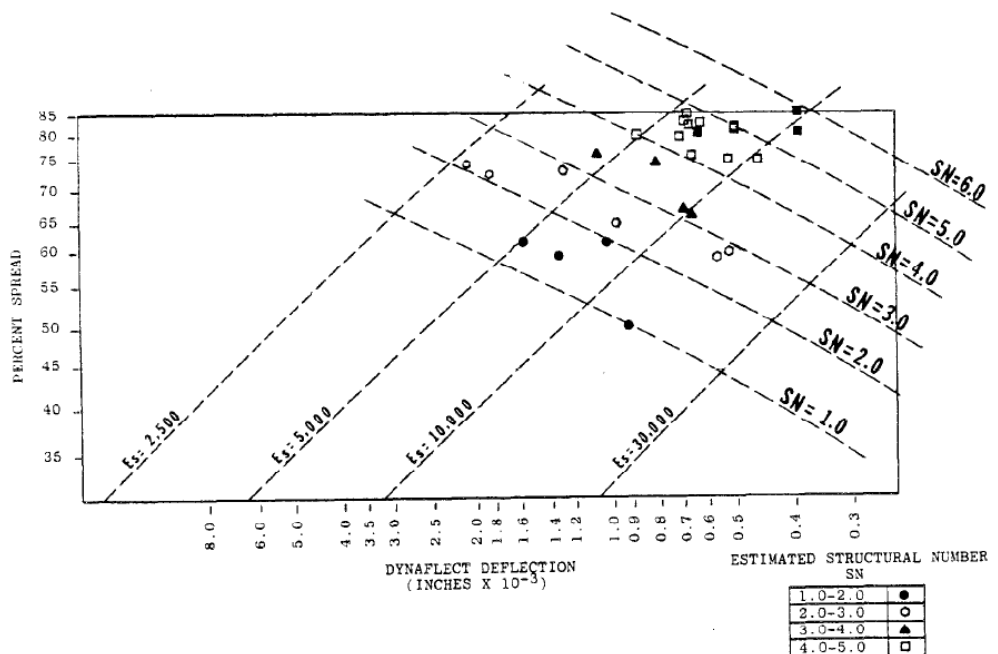
Figure 7 Louisiana pavement evaluation chart (Kinchen, 1980)
