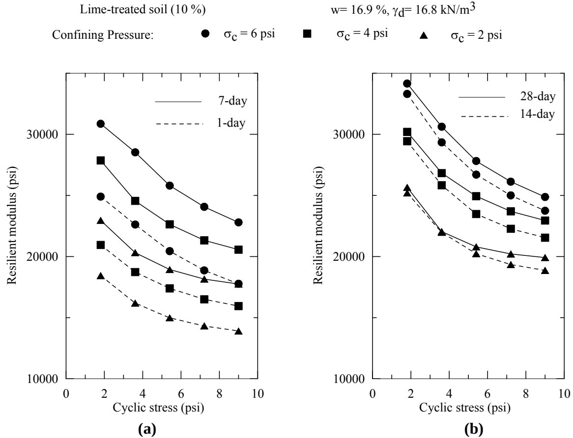
Figure 52 Resilient modulus of lime-treated soils (a) 1-day and 7-day curing (b) 14-day and 28-day curing
