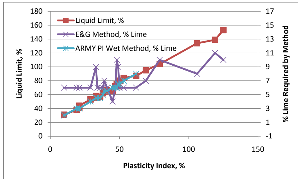
Figure 51 Lime percentage methods
