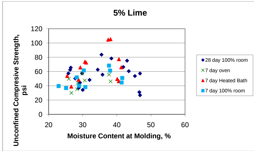
Figure 41 Strengths vs. molding moistures at 5 percent lime
