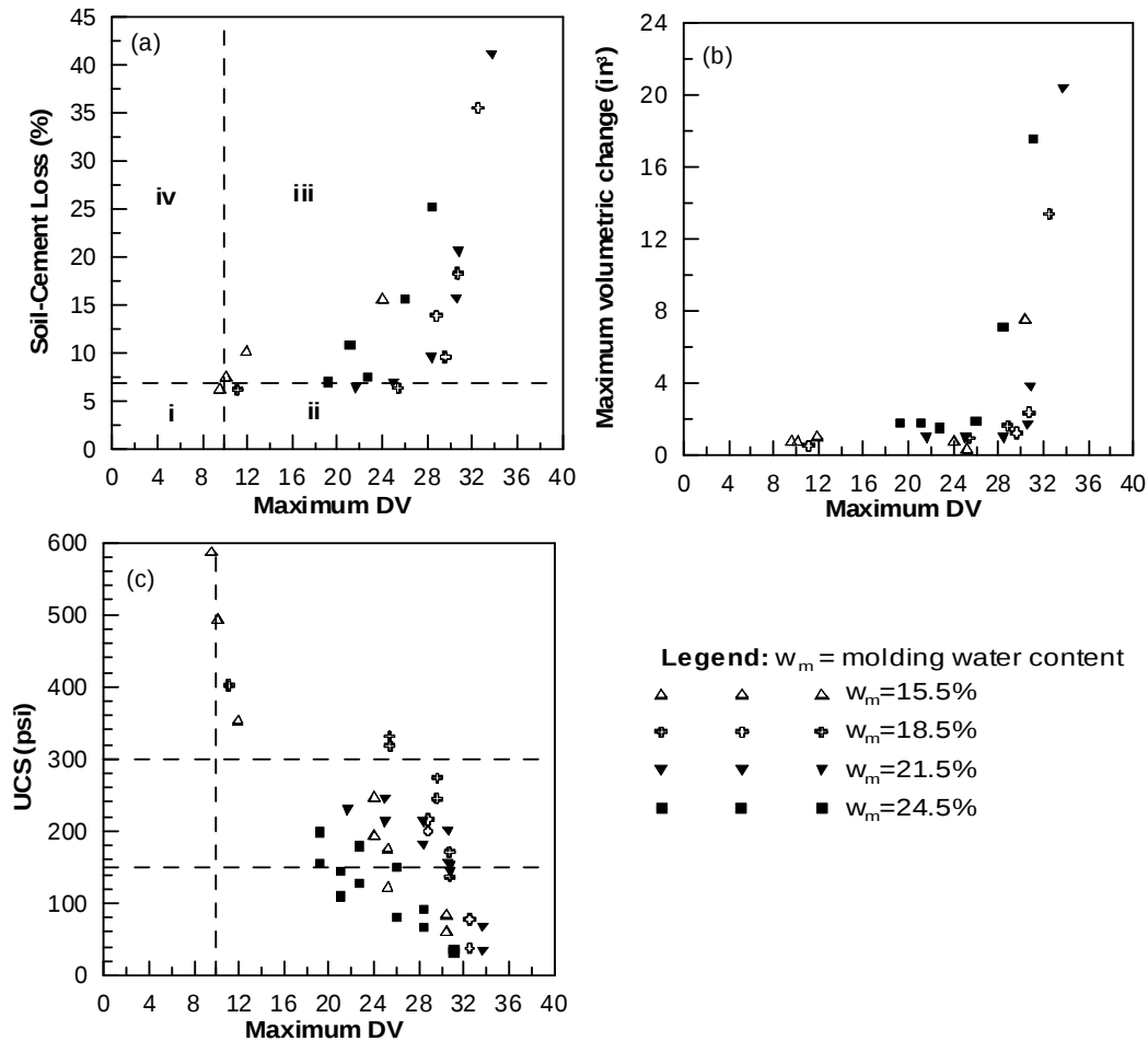
Figure 35 Maximum DV versus durability and UCS of stabilized soil: (a) maximum DV versus soil-cement loss; (b) maximum DV versus maximum volumetric change; and (c) maximum DV versus 7-day UCS
