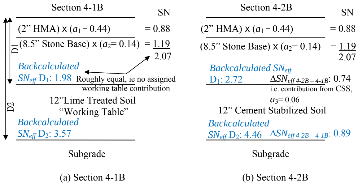
Figure 65 Estimation of effective structural number
