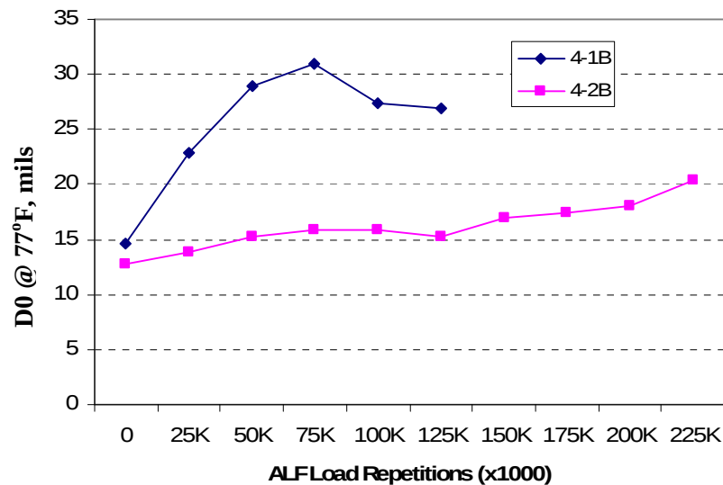
Figure 62 FWD center deflections
