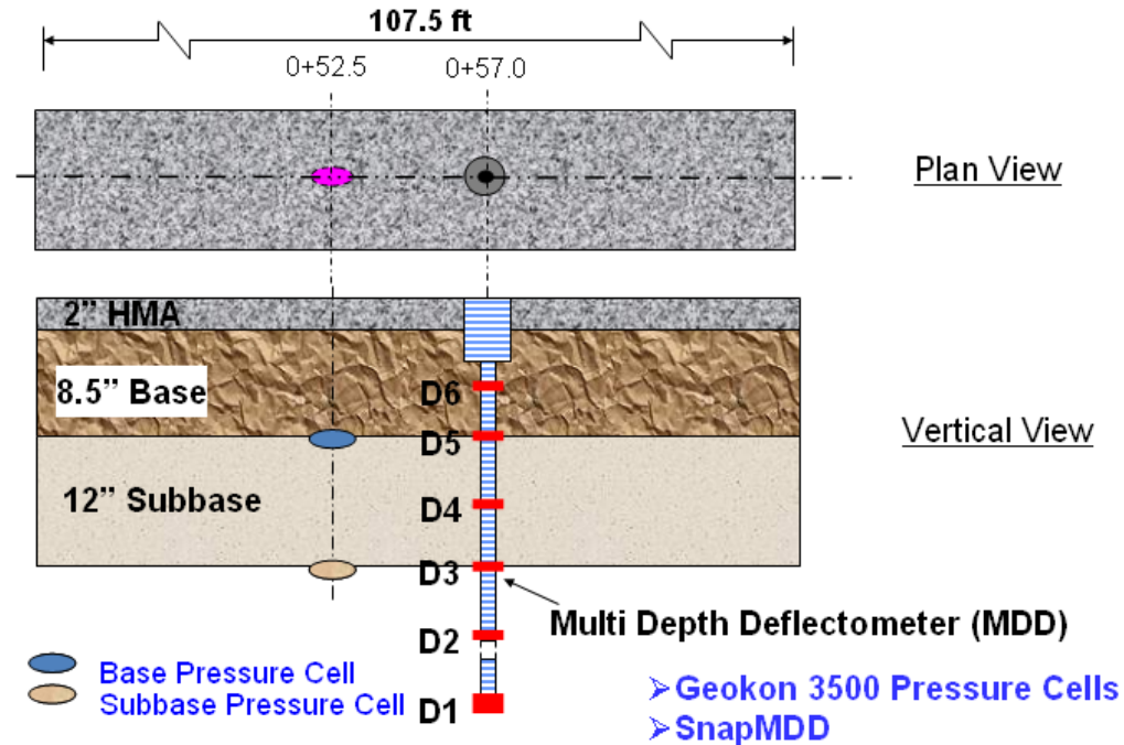
Figure 6 Field instrumentation layout
