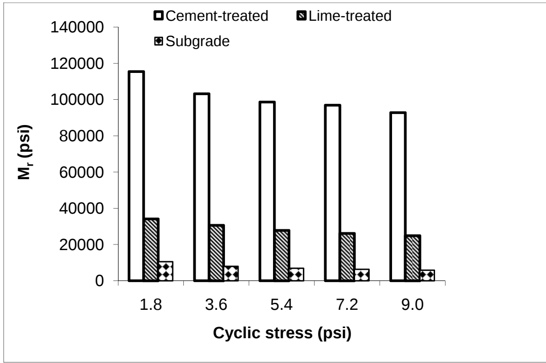
Figure 38 Resilient modulus of treated and untreated soils at confining pressure 6 psi
