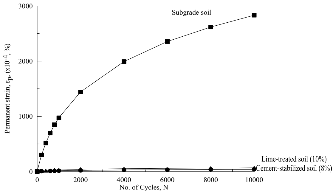
Figure 55 Permanent strains of cohesive soils at 28-day curing
