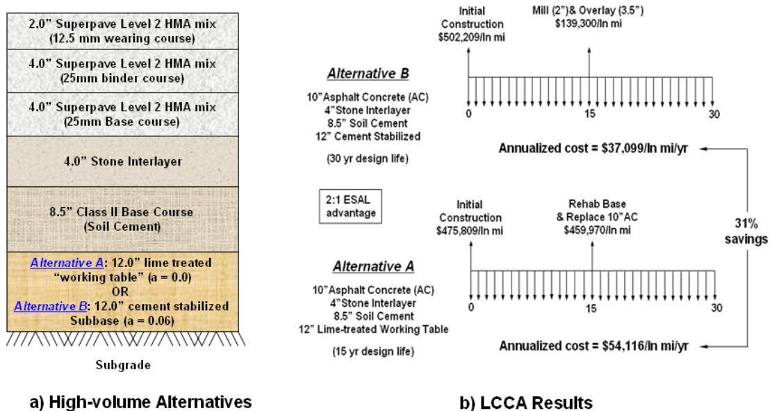
Figure 67 LCCA on high volume roads
