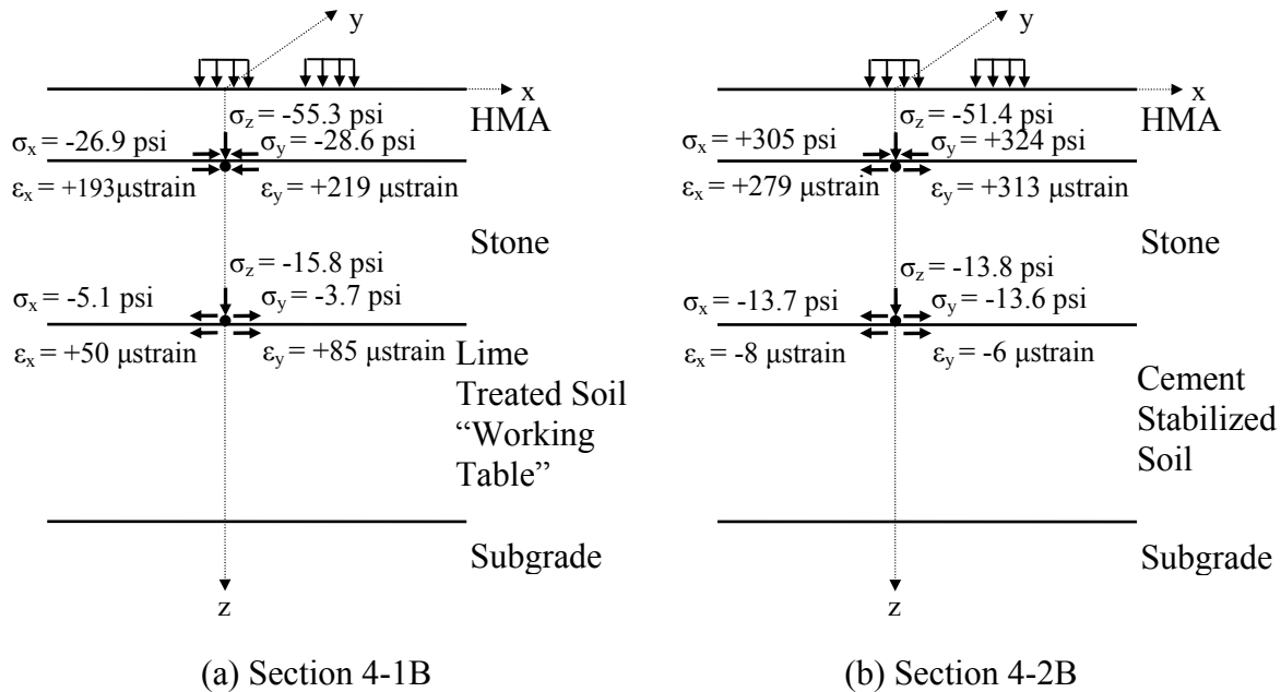
Figure 64 Stress and strain predictions ("+" tension, "-" compression)
