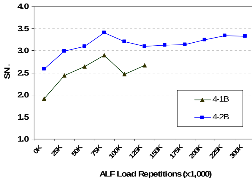
Figure 61 Dynalect structural number results
