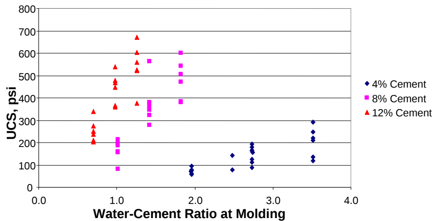
Figure 18 Performance along the compaction curve, Soil II, dry side
