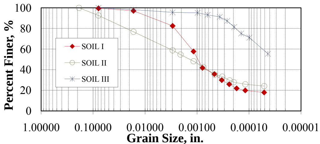
Figure 8 Particle size distribution of tested soils
