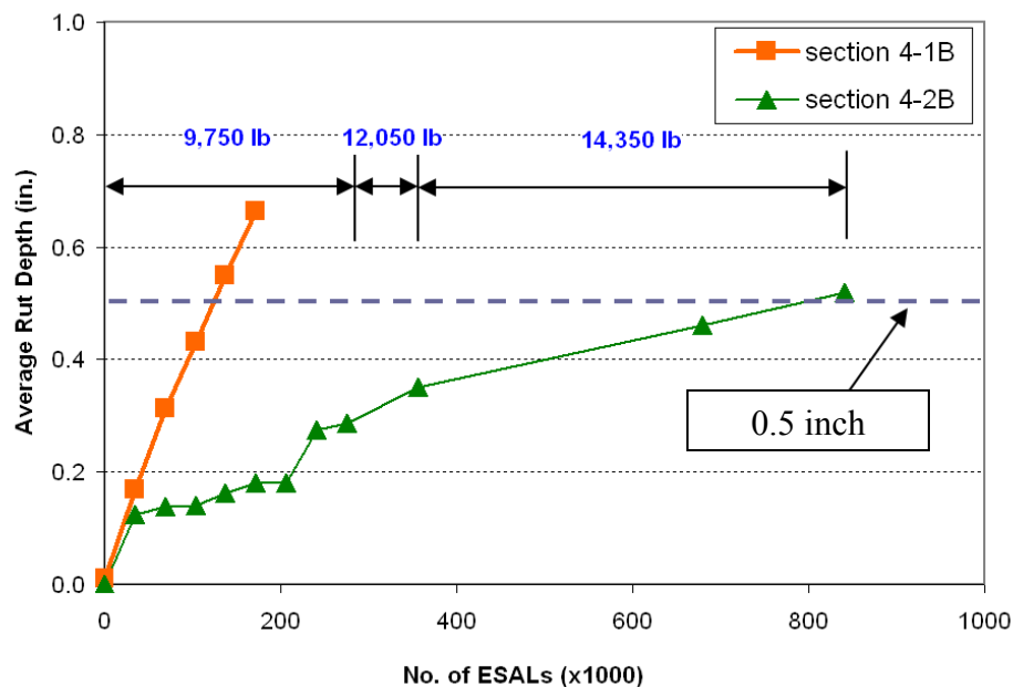
Figure 58 Rut depth development on test sections
