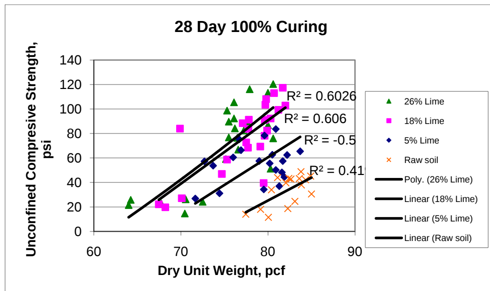
Figure 46 28-day strength vs. dry unit weight
