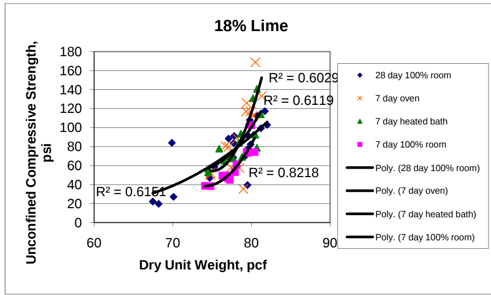
Figure 44 Strengths vs. dry unit weight at 18 percent lime
