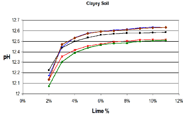
Figure 48 Eades & Grim pH results – clayey soil
