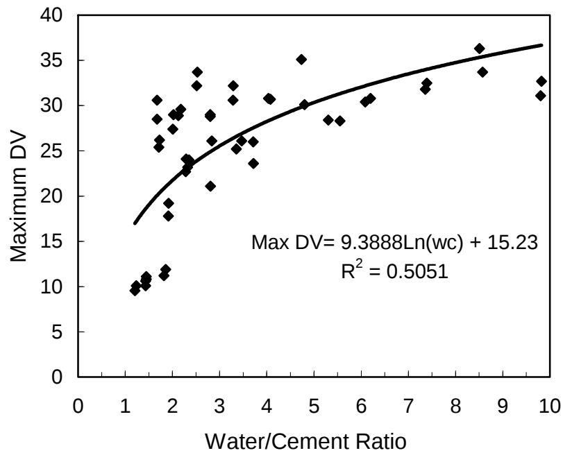
Figure 28 Maximum dielectric value versus water cement ratio
