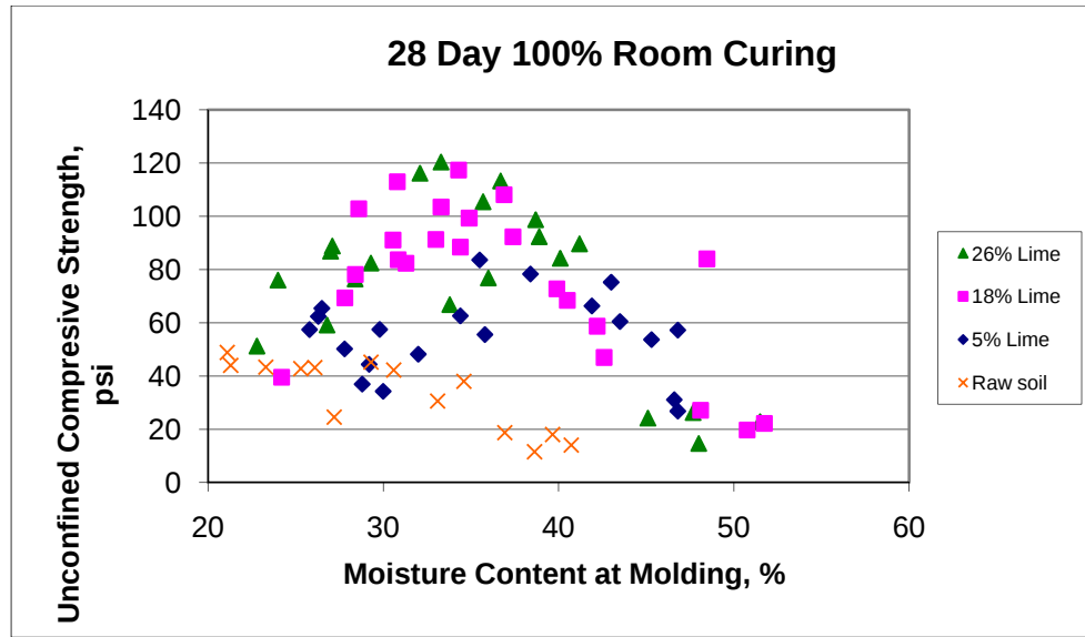
Figure 45 28-day strength vs. molding moisture
