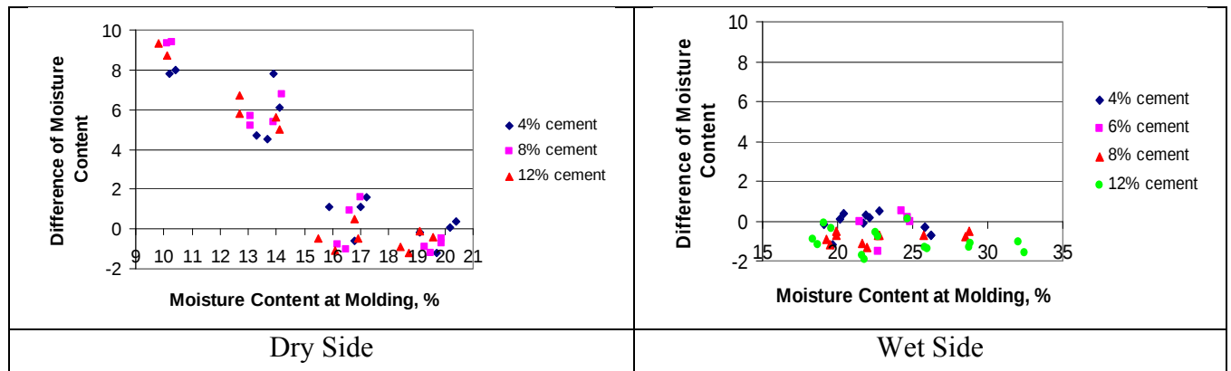
Figure 20 Variation of moisture content during curing, cement-stabilized Soil I
