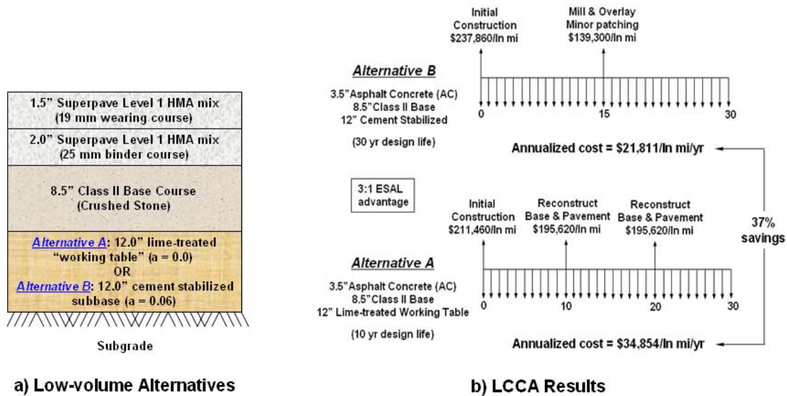
Figure 66 LCCA on low volume roads
