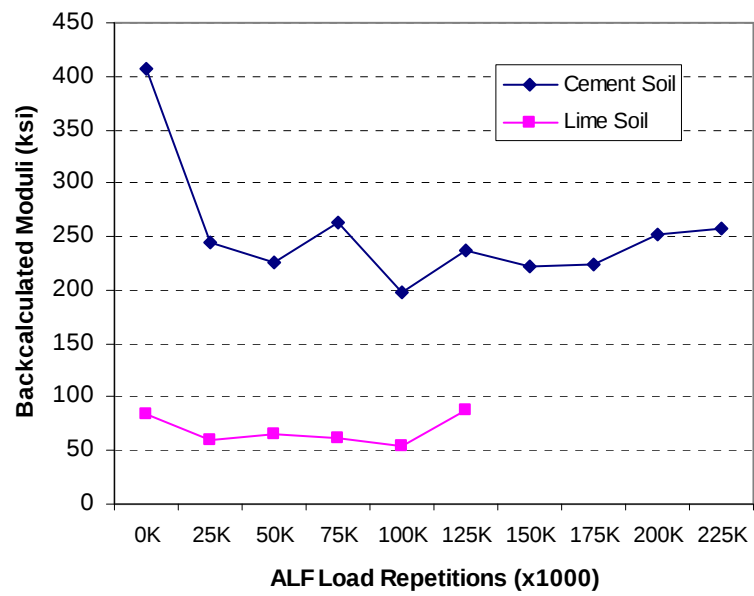
Figure 63 Backcalculated moduli of base materials
