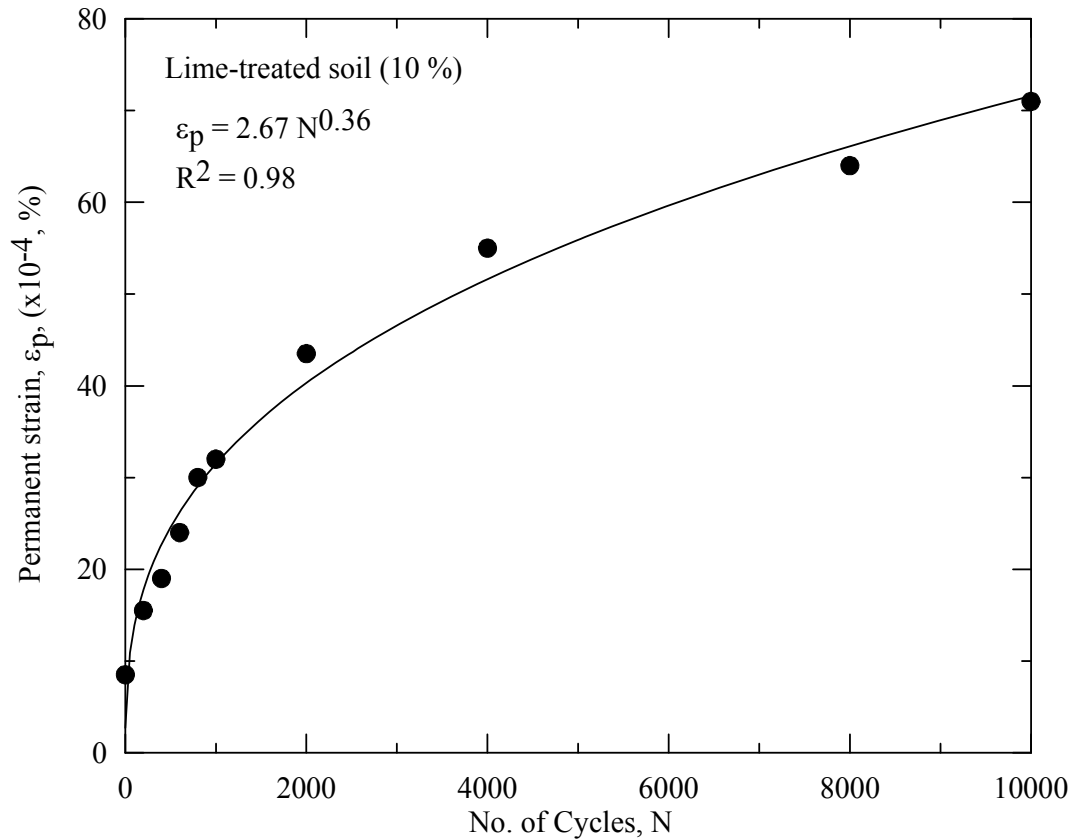
Figure 54 Permanent strains of lime-treated soils at 28-day curing
