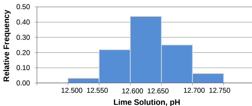
Figure 47 Lime pH histogram
