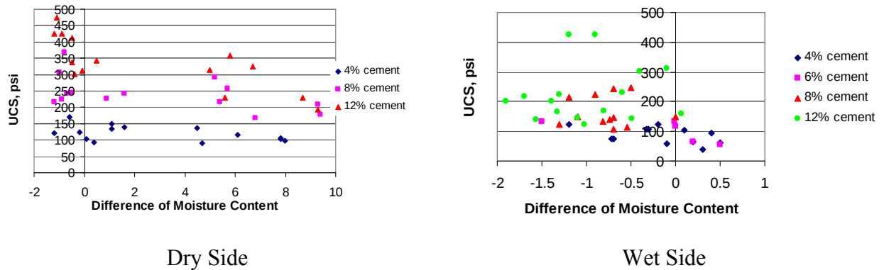
Figure 22 Impact of moisture changes on strength, cement-stabilized Soil I
