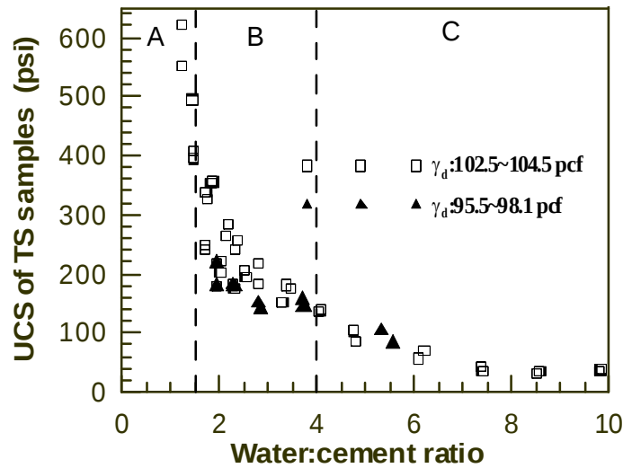
Figure 30 Residual UCS versus water/cement ratio
