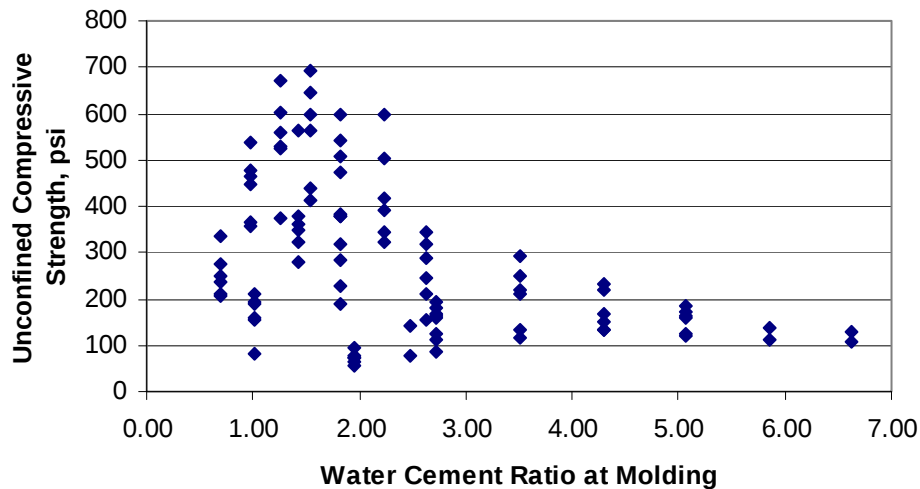
Figure 15 UCS and water-cement ratio at molding, Soil II
