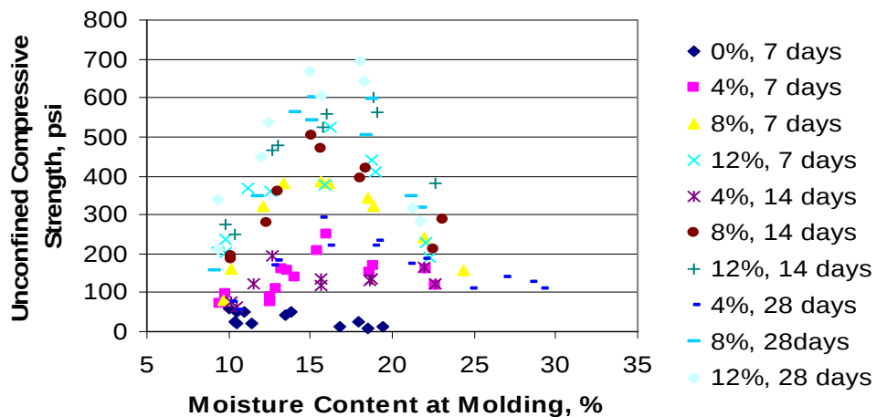
Figure 13 UCS and moisture content at molding of various conditions, Soil II
