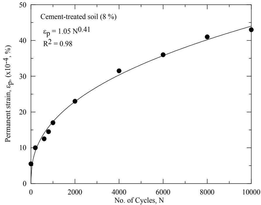
Figure 39 Permanent strains of cement-stabilized soils at 28-day curing
