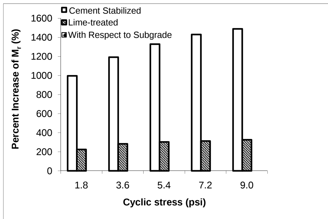
Figure 53 Increase in resilient modulus at confining pressure 6 psi
