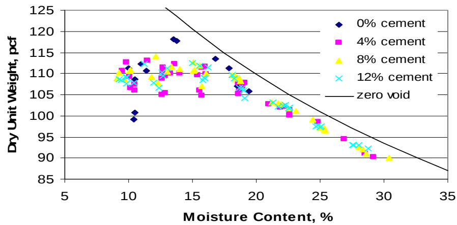
Figure 11 Compaction curves with and without cement for Soil II
