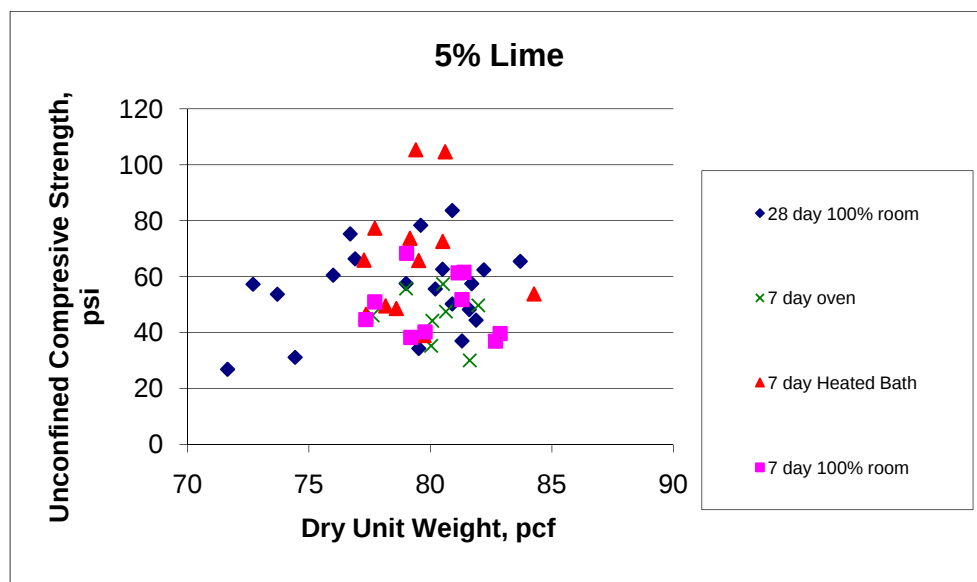
Figure 43 Strengths vs. dry unit weight at 5 percent lime
