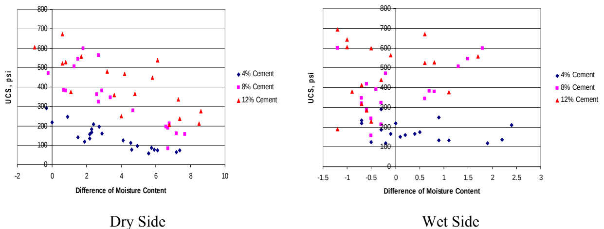
Figure 23 Impact of moisture Changes on strength, cement-stabilized Soil II
