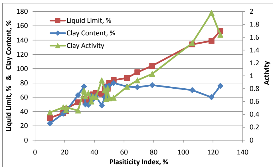
Figure 50 Clay content, activity, and Atterberg limit plot
