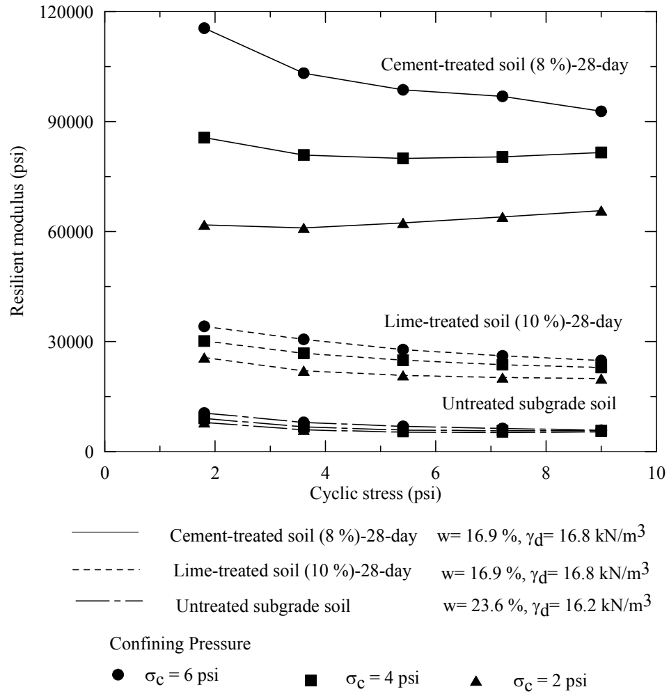
Figure 37 Resilient modulus of treated and untreated soils
