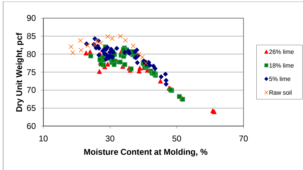
Figure 40 Dry unit weights at molding moisture
