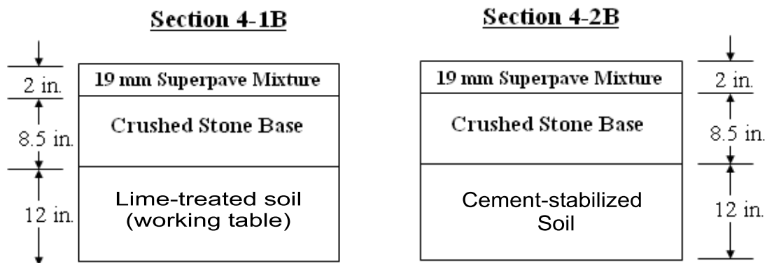
Figure 5 Pavement structures of ALF test sections
