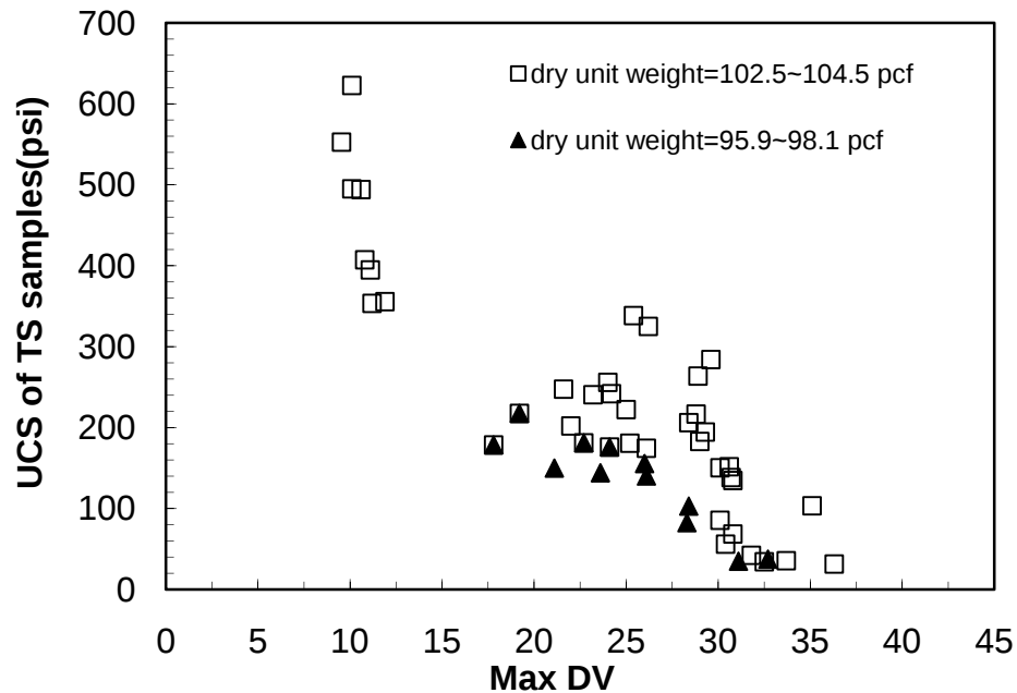
Figure 29 Relationship between UCS and maximum dielectric values
