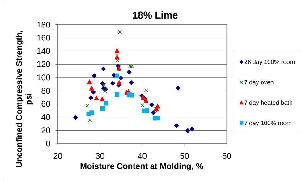
Figure 42 Strengths vs. molding moistures at 18 percent lime
