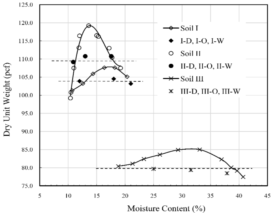
Figure 9 Standard compaction curves of tested soils
