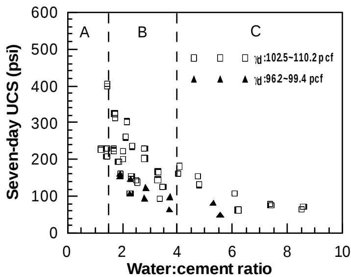
Figure 31 Correlation of 7-day UCS with water-cement ratio
