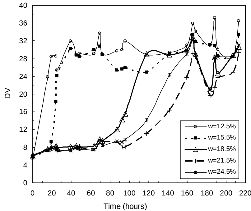
Figure 24 Variation of dielectric value (DV) with elapsed time
