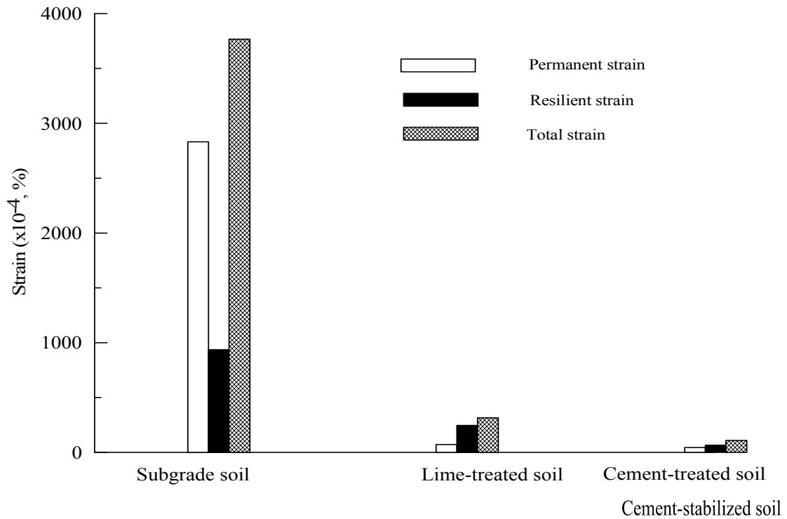
Figure 56 Strains of untreated and treated soils at the end of 10,000 cycles
