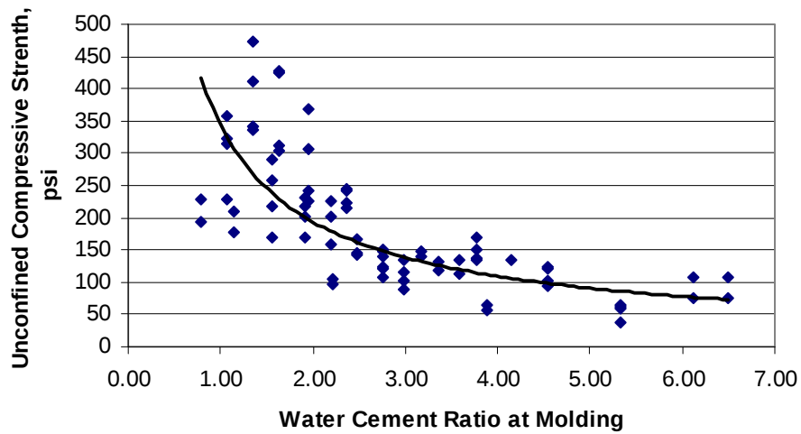
Figure 14 UCS and water-cement ratio at molding, Soil I
