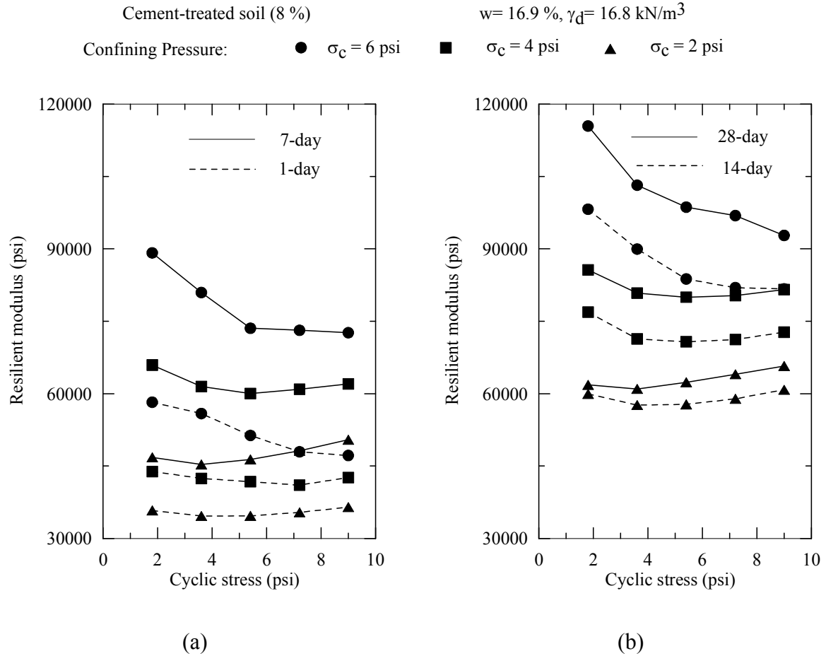
Figure 36 Resilient modulus of cement-stabilized soils (a) 1-day and 7-day curing (b) 14-day and 28-day curing
