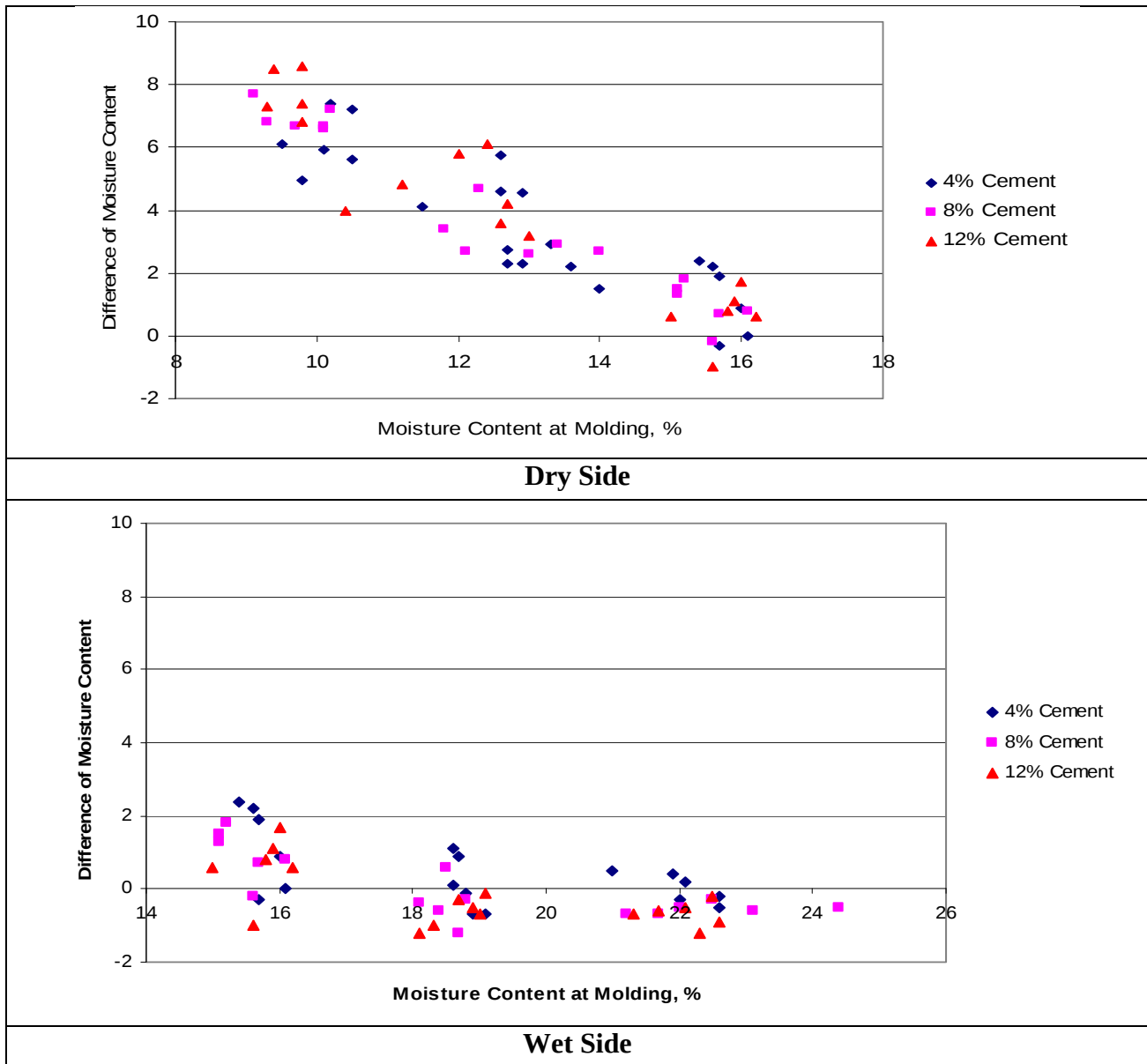
Figure 21 Variation of moisture content during curing, cement-stabilized Soil II
