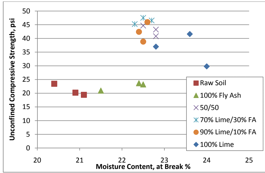
Figure 57 UCS results, various additives, and 7-day breaks
