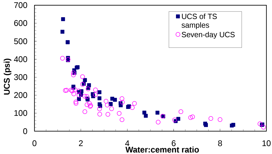
Figure 32 Correlation of UCS with water-cement ratio
