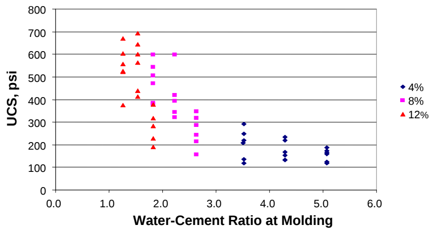
Figure 19 Performance along the compaction curve, Soil II, wet side
