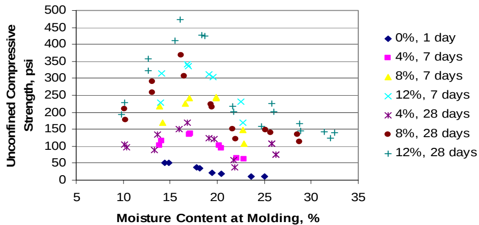
Figure 12 UCS and moisture content at molding of various conditions, Soil I
