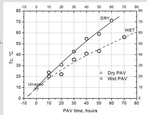
Figure 2 Variation of critical temperature of multiple PAV dry-aged and wet-aged PMAC samples
