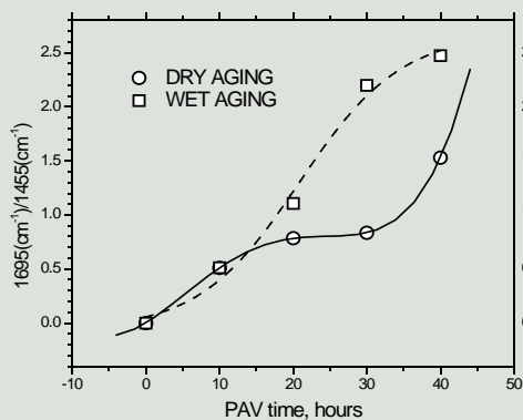
Figure 1 Carbonyl content of asphalt samples after dry and wet PAV aging
