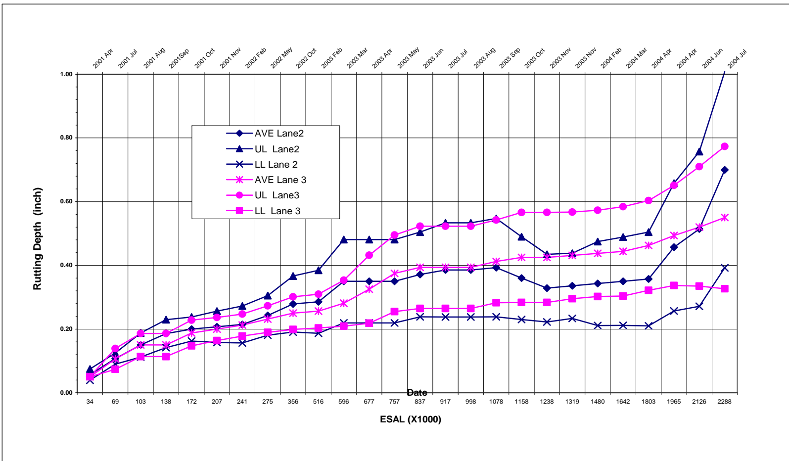
Figure 21 Rutting depth for lanes 2 and 3 with 95% confidence
