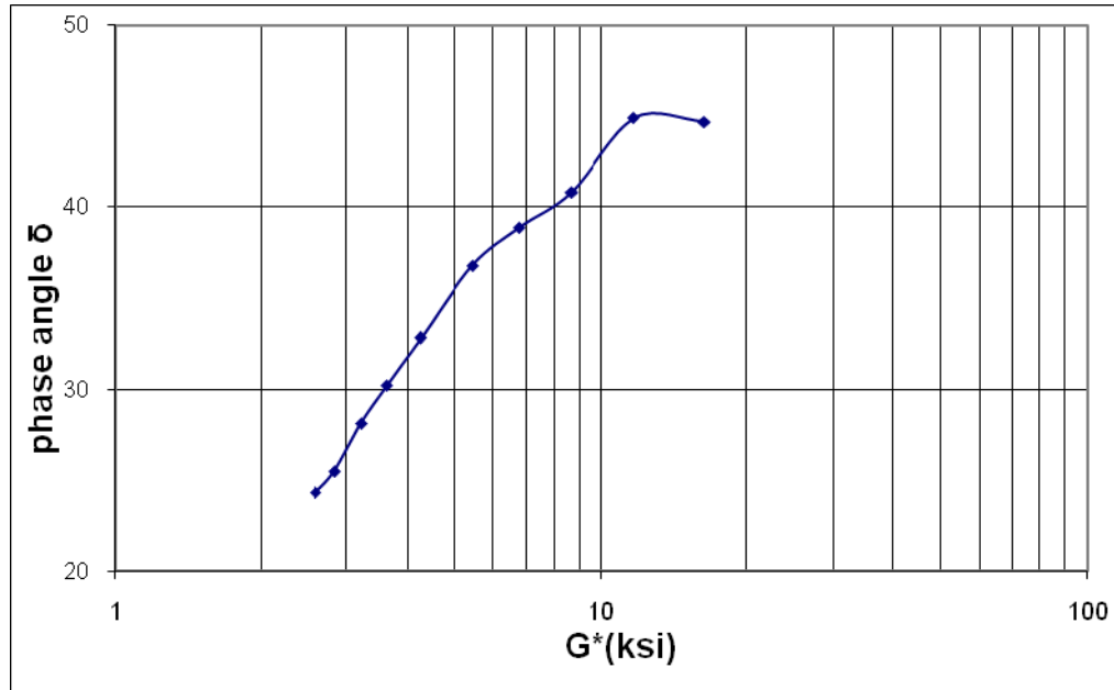
Figure 16 G* versus phase angle \delta of FSCH test
