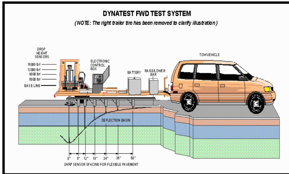
Figure 5 FWD illustration
