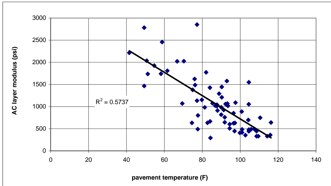
Figure 25 Relationship between modulus of surface AC and pavement temperature
