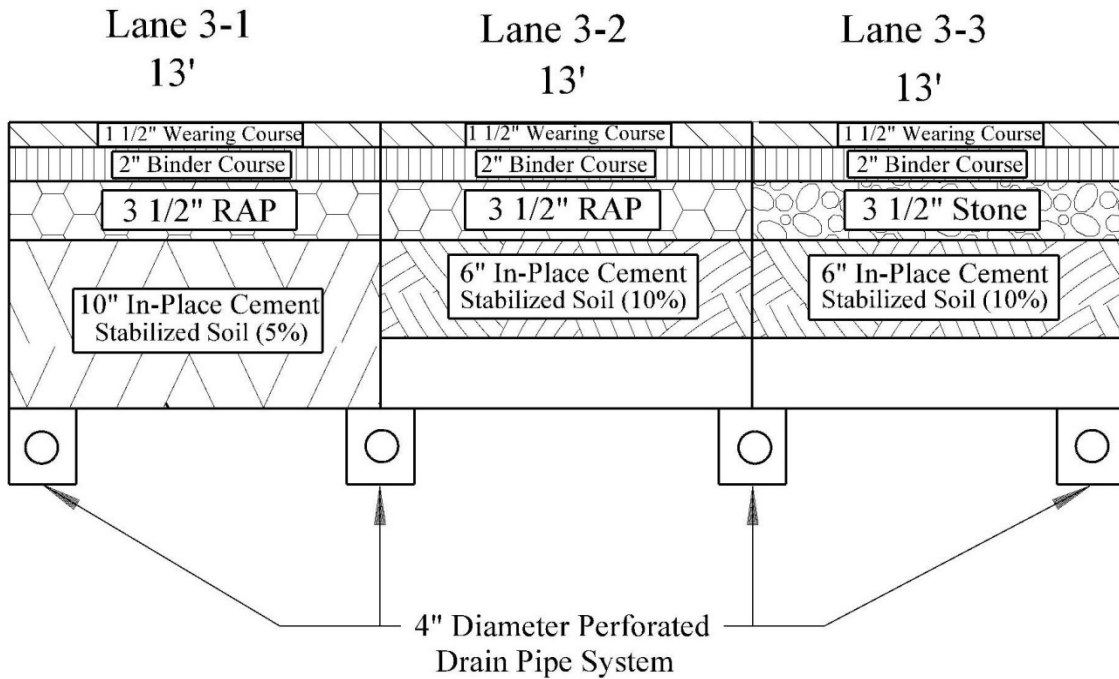
Figure 1 Test lanes cross-sections
