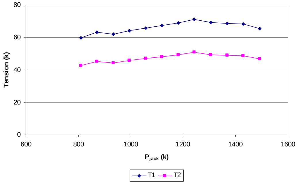
Figure 23. Force in T1 and T2 for PCBT-61, NWC, ½-in-diameter Strand
