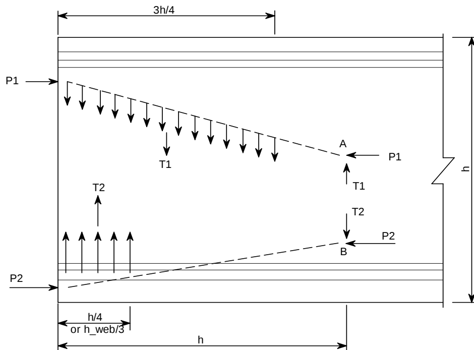
Figure 2. Strut-and-Tie Models Proposed by Davis et al. (2005)
