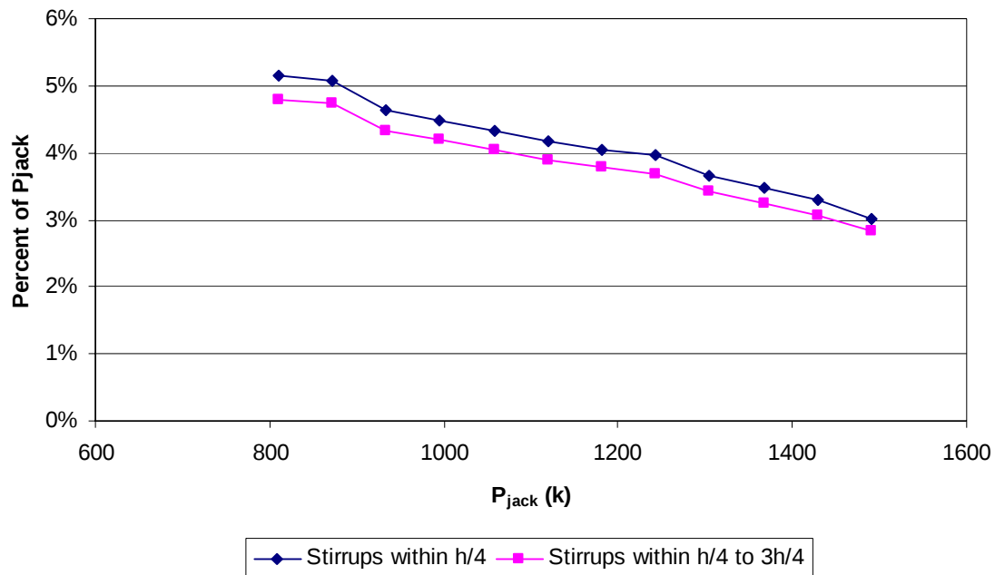
Figure 25. Required Bursting Resistance, PCBT-61, LWC, ½-in strand
