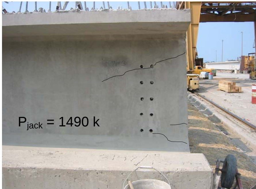
Figure 17. PCBT-61 Anchorage Zone Case Study – Fair Condition
