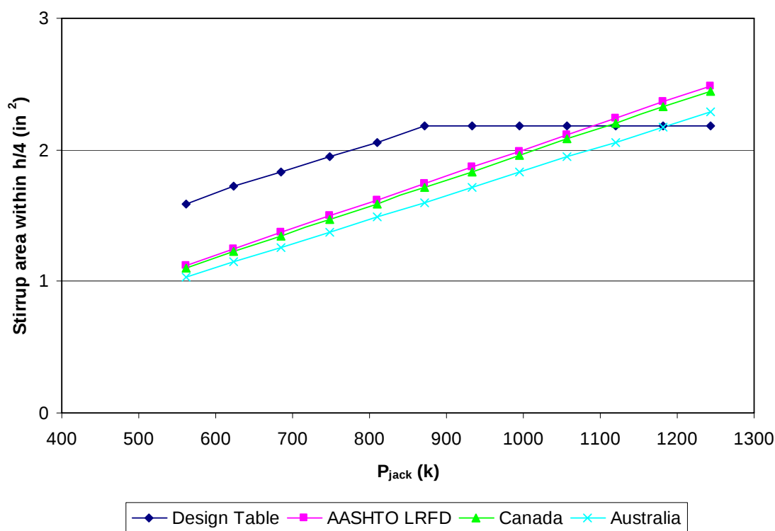
Figure 30. Design Code Comparison, PCBT-45, NWC, ½-in strand
