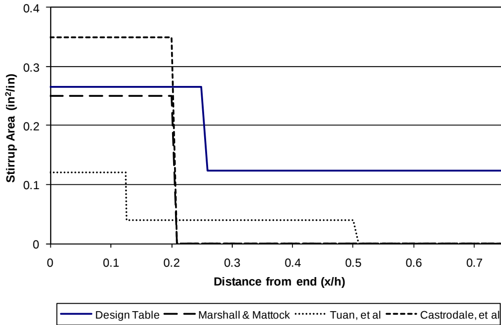
Figure 29. Design Method Comparison, PCBT-93, LWC, 46 ½-in strands
