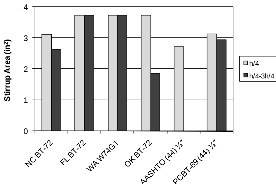
Figure 33. Standard Detail Comparison – PCBT-69, NWC, 44 1/2-in strands
