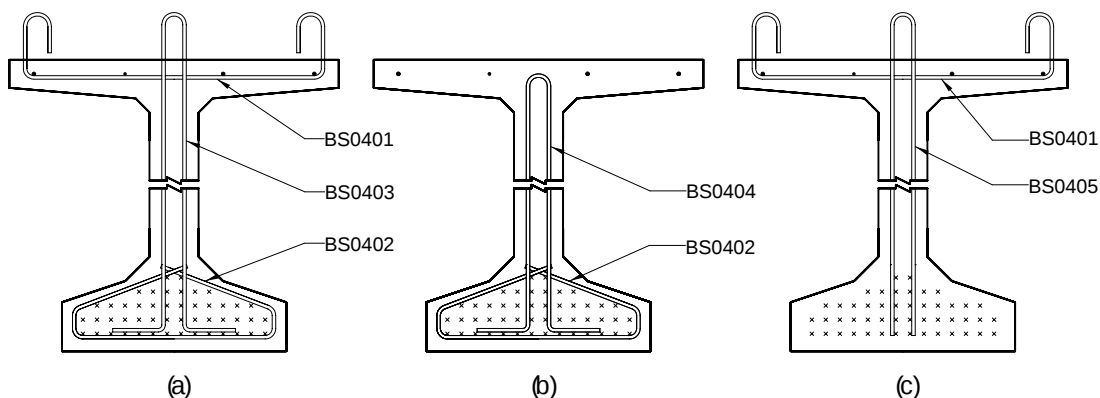
Figure 6. Proposed Stirrup Types
