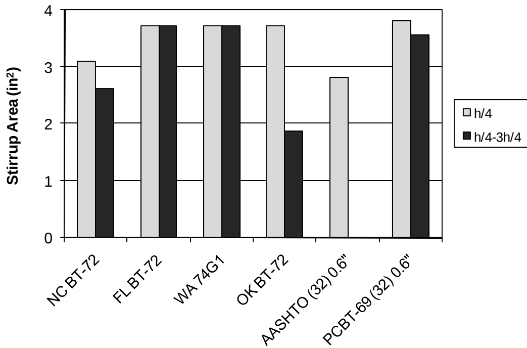
Figure 34. Standard Detail Comparison – PCBT-69, NWC, 32 0.6-in strands
