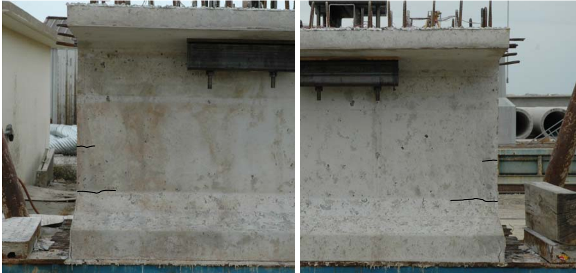
Figure 37. Crack Pattern in the 12 ksi Anchorage Zone After Lifting
