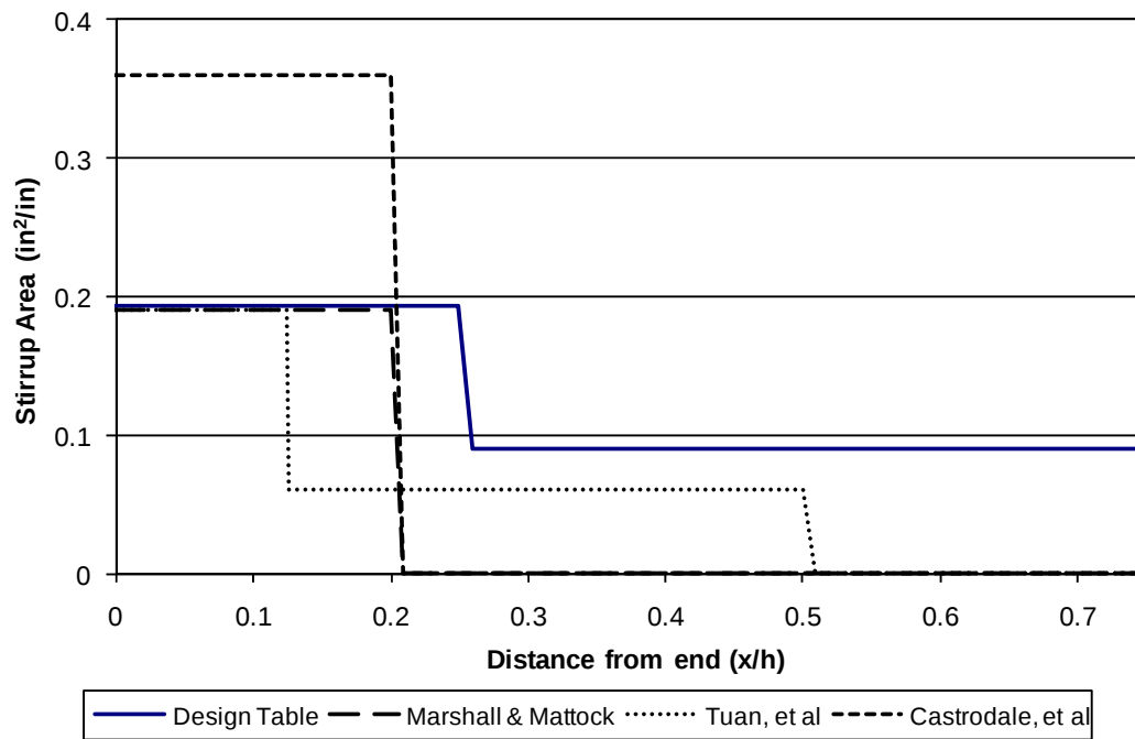
Figure 27. Design Method Comparison, PCBT-45, NWC, 34 ½-in strands
