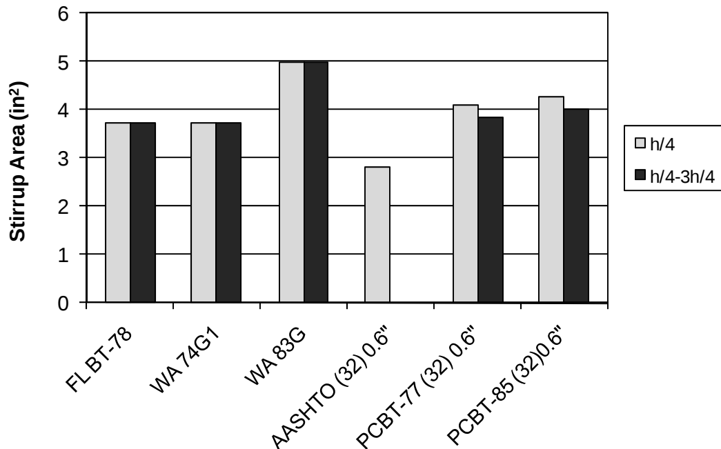
Figure 36. Standard Detail Comparison – PCBT-77 and PCBT-85, NWC, 32 0.6-in strands
