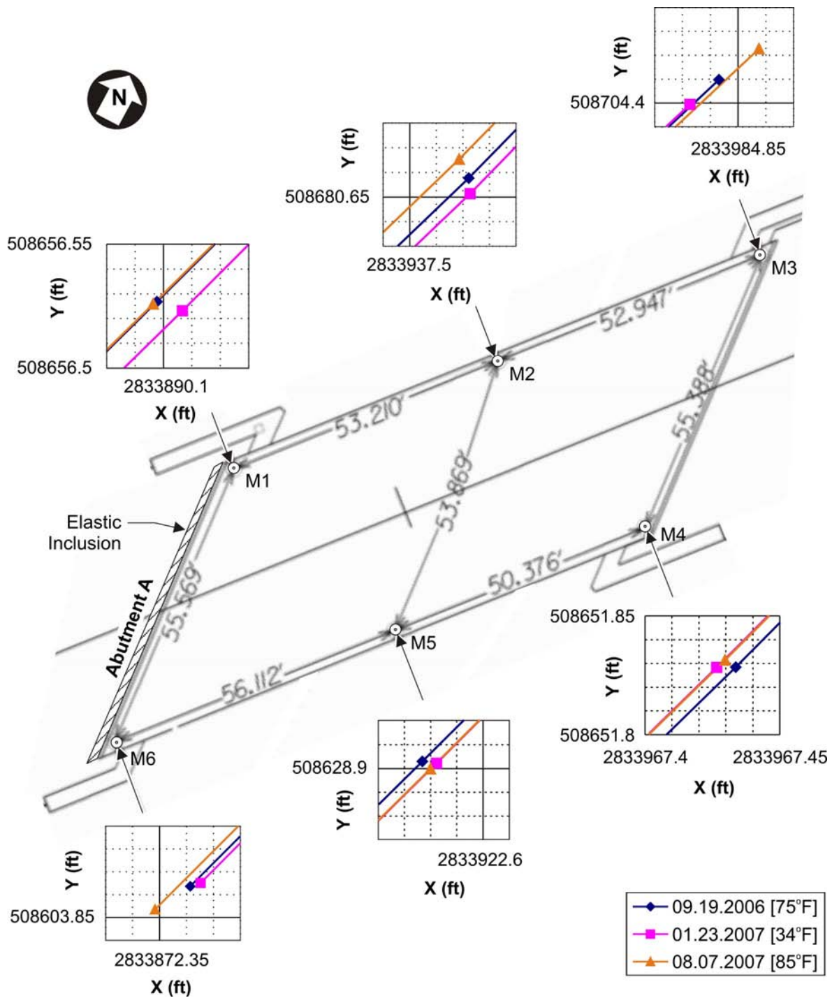
Figure 16. Results of Bridge Coordinate Surveys
