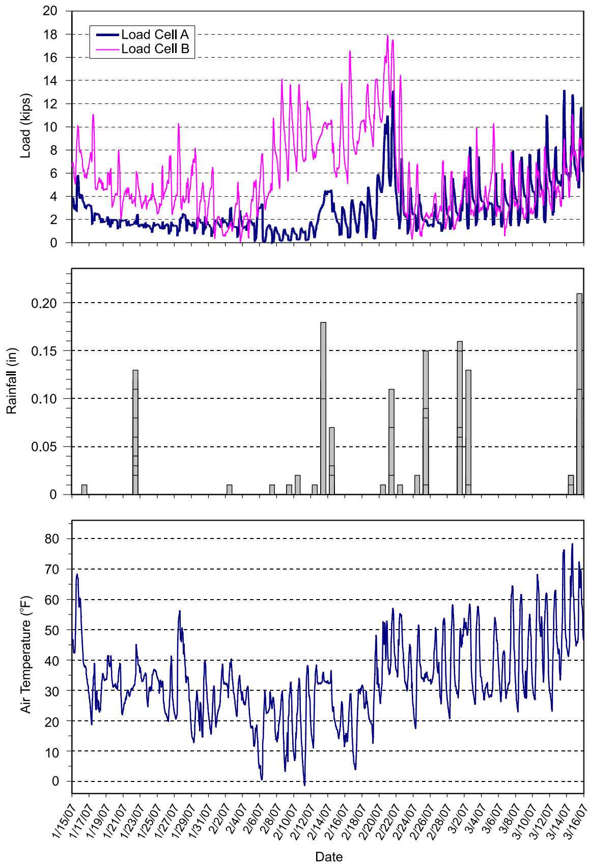
Figure 18. Load Cell Data: 1/15/07–3/15/07
