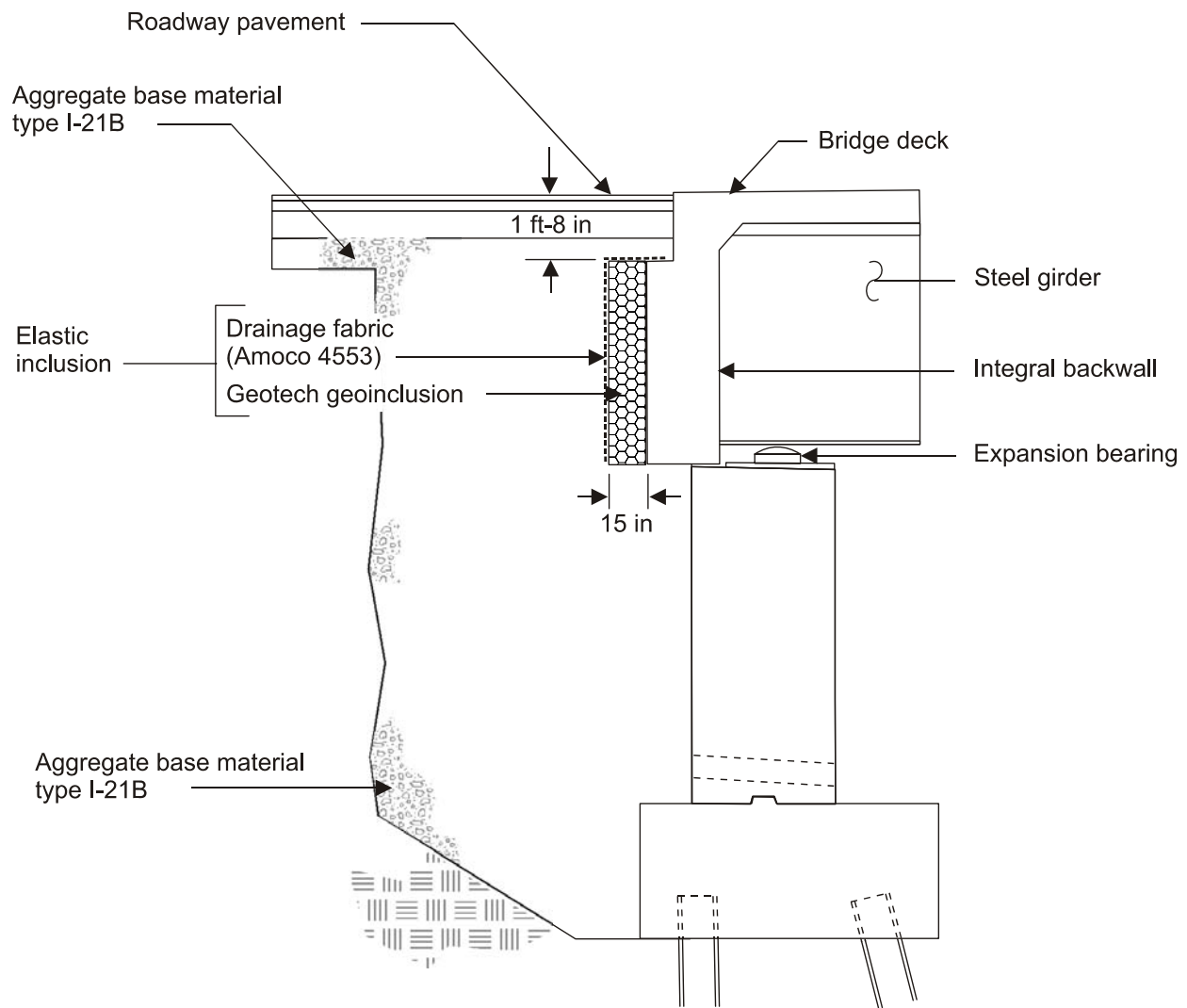
Figure 5. Abutment A Cross Section
