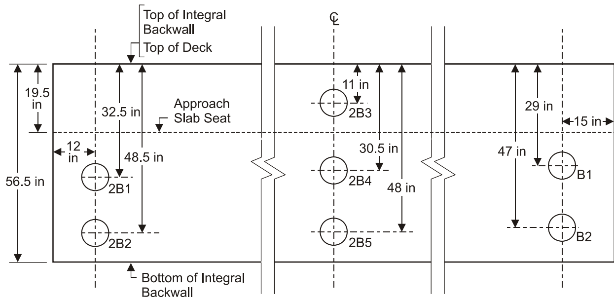
Figure 12. Locations of Earth Pressure Cells at Abutment B
