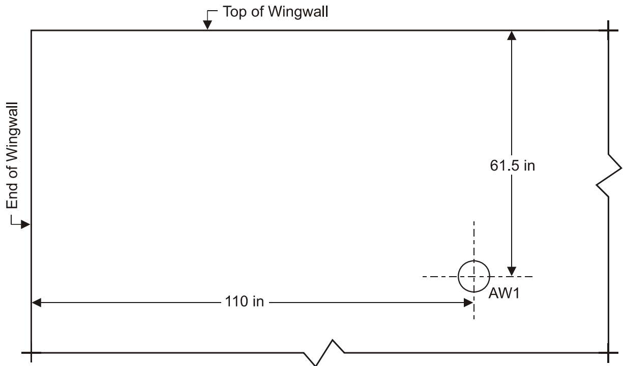
Figure 13. Location of Earth Pressure Cells at Wingwall A
