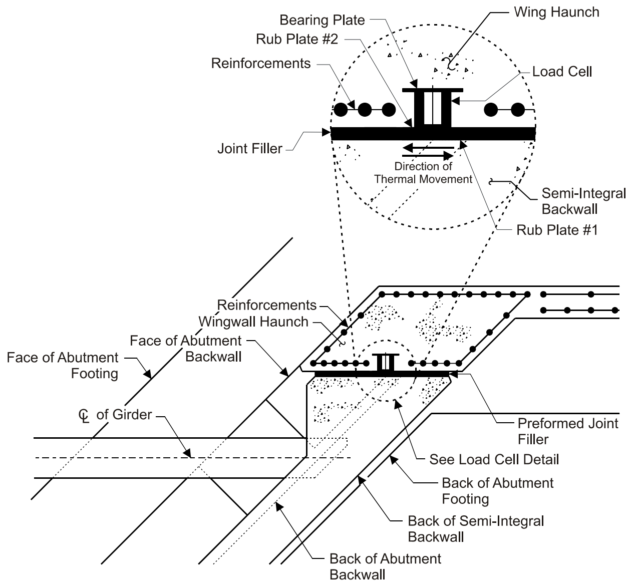
Figure 8. Integral Backwall and Butress Detail
