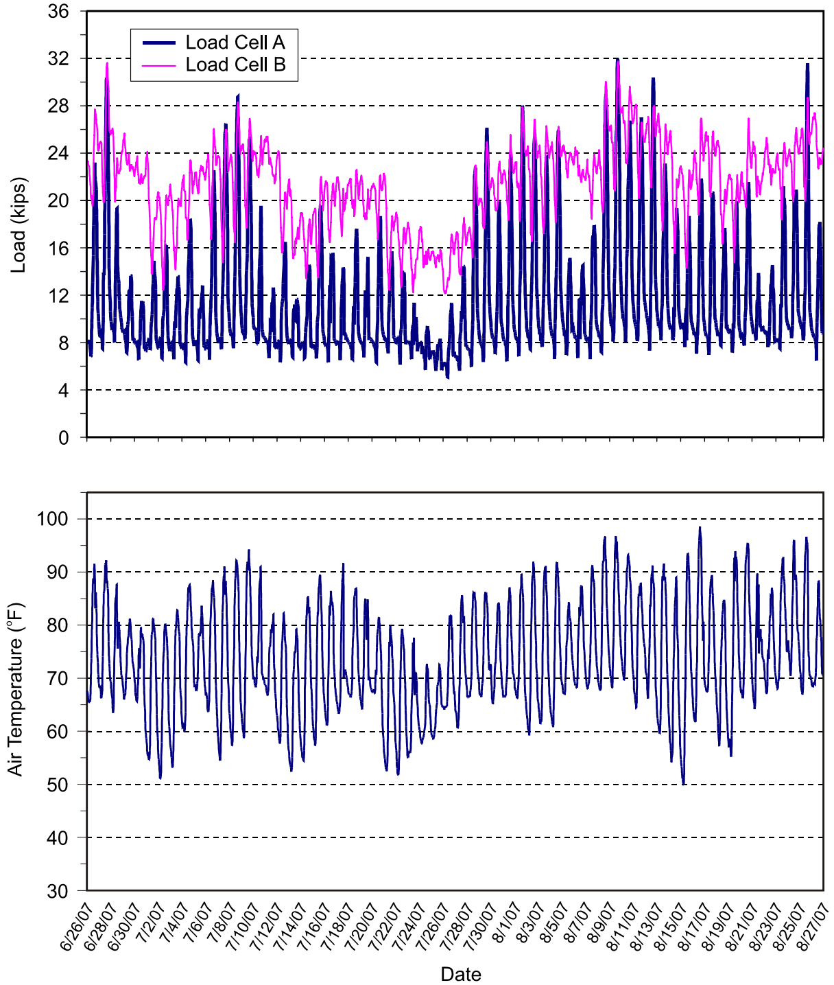
Figure 17. Load Cell Data: 6/26/07–8/26/07
