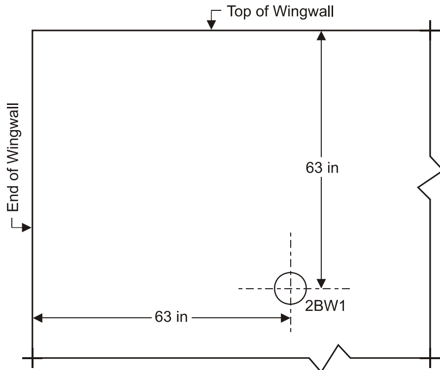
Figure 14. Location of Earth Pressure Cell at Wingwall B
