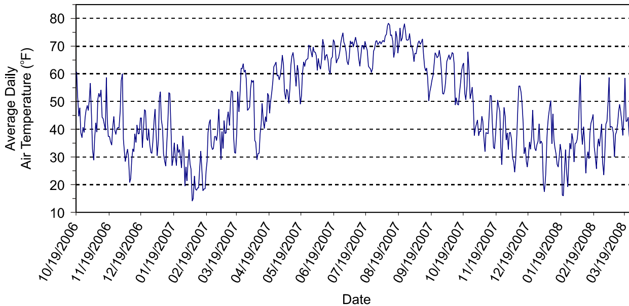
Figure 15. Average Daily Air Temperatures During Monitoring Period
