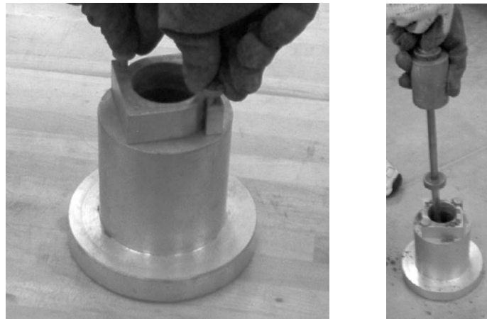
Figure 3. Cylinder Mold Stand (left) and Special Hammer (right)
