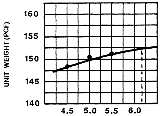
ASPHALT CONTENT (PERCENTAGE)
