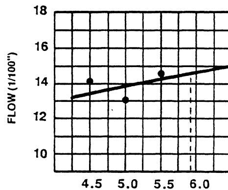
ASPHALT CONTENT (PERCENTAGE)
