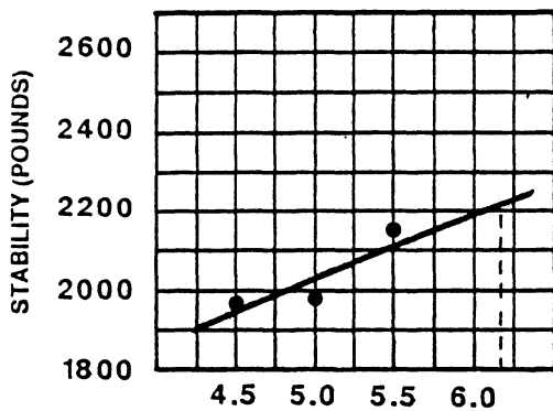
ASPHALT CONTENT (PERCENTAGE)
