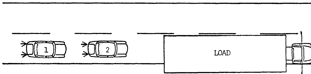
Figure 33. Indirect previous rear end vehicle conflict. Vehicle No. 1 brakes in response to vehicle No. 2, who brakes to avoid a collision with the wide load.
