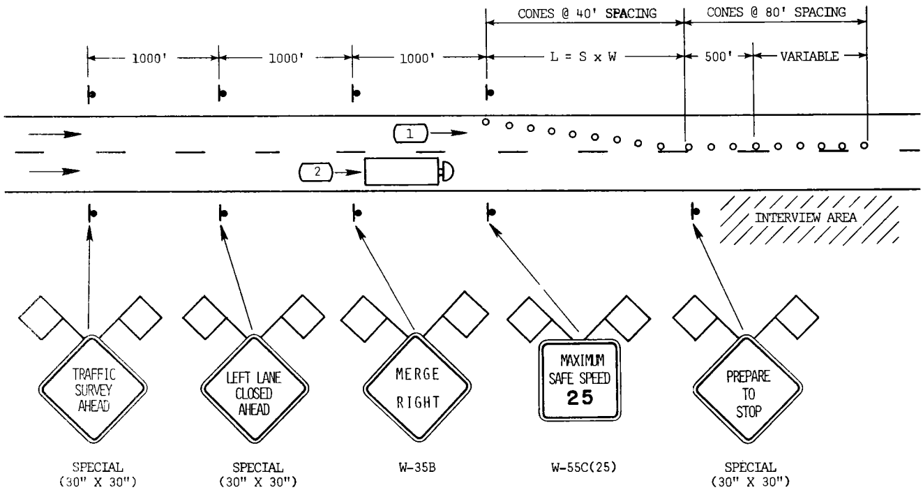
Figure 14. Interview setup and signing for interstate and four-lane divided highways.
