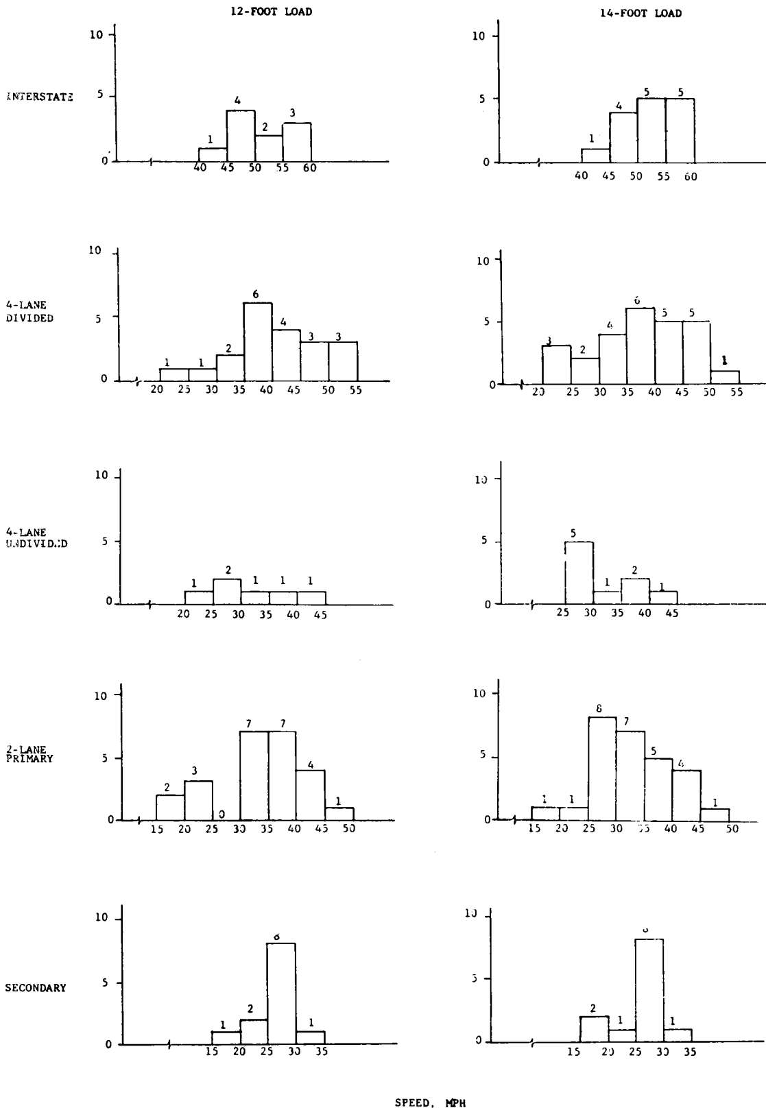
Figure 17. Wide load speed distributions.
