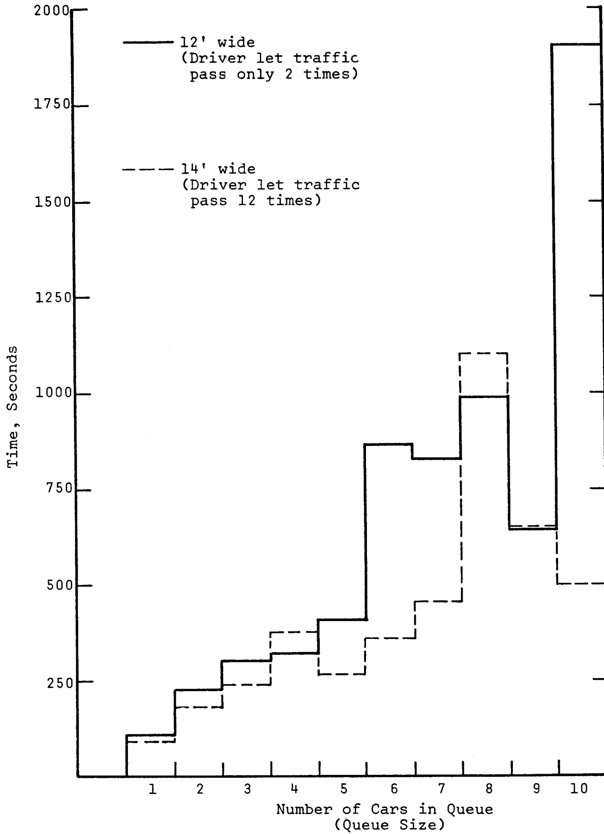
Figure 22. Effects of wide load drivers yielding to traffic on average vehicle impedance time.
