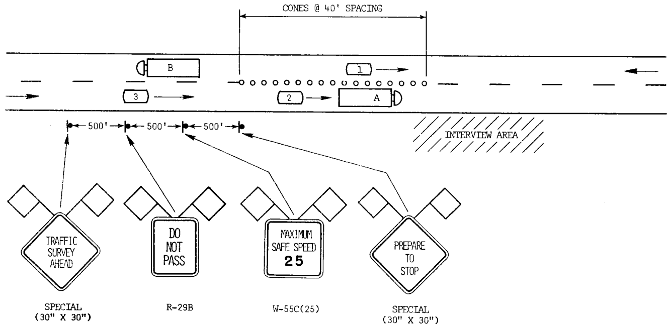
Figure 15. Interview setup and signing for two-lane roads.
