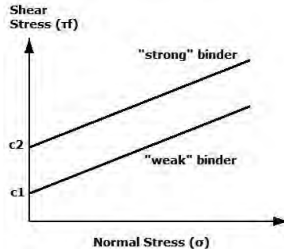
Figure 2.2: Asphalt Contribution to Shear Strength (McGennis et al., 1995)
