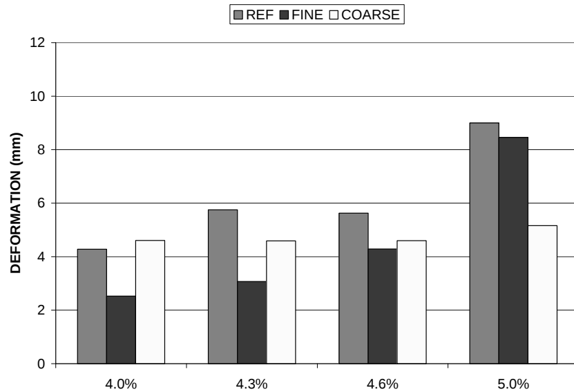
Figure 5.6: Deformation after 20,000 HWTD Passes (limestone Type C)
