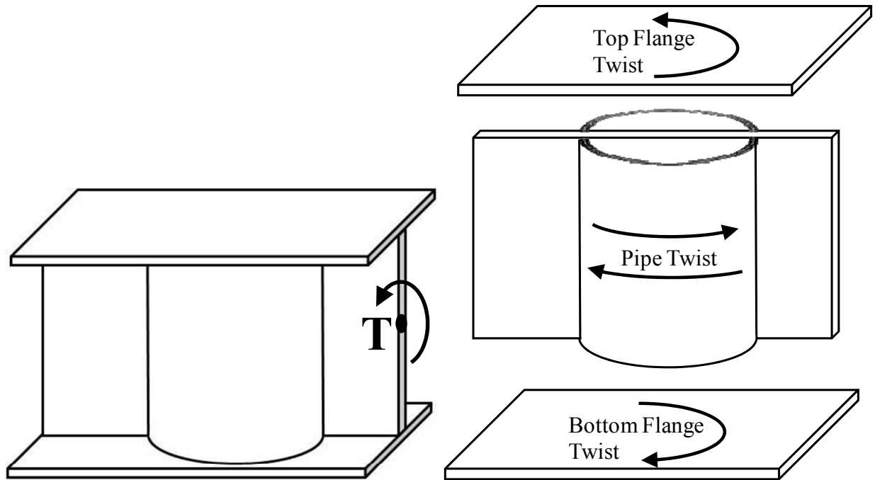
Figure 2: Pipe Stiffener Twist due to Flange Rotation Associated with Warping of the Girder's Ends (Quadrato 2010)
