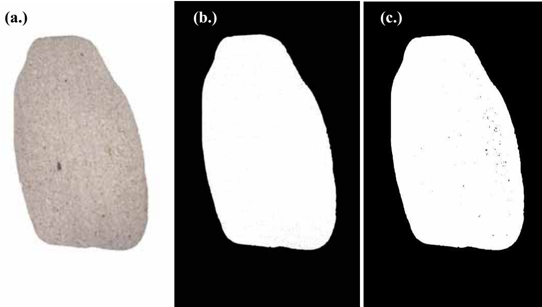
Figure A-3. Image Analysis for Crushed Gravel Sample #3 for (a.) Original Image, (b.) Image Processed for Blue Resin (Surface Porosity), and (c.) Image Processed for Yellow Resin (Internal Porosity).
