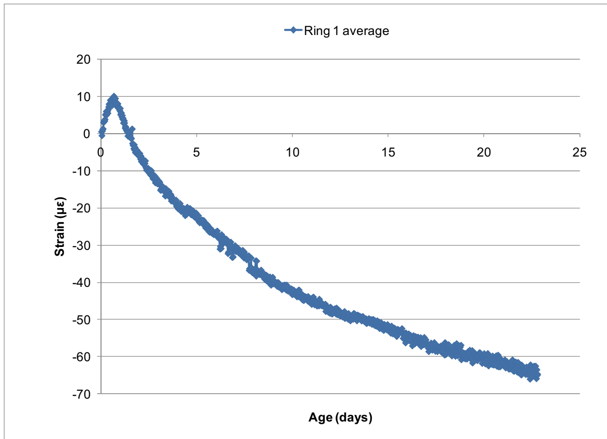
Figure C-2. Restrained Ring Shrinkage Strain for Crushed Gravel (He Pyc) MDOT P1 Concrete.
