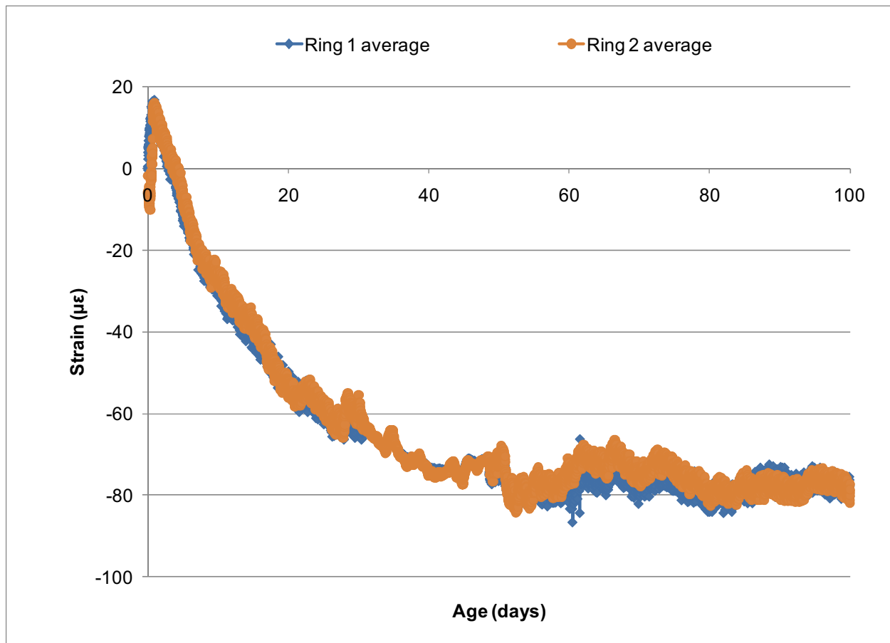
Figure C-6. Restrained Ring Shrinkage Strain for Limestone RCA MDOT P1 Concrete.
