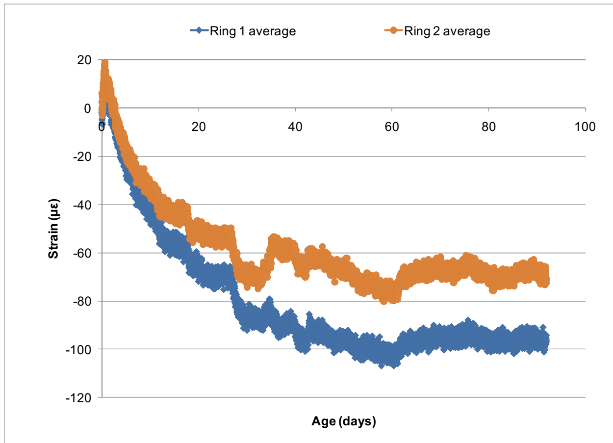
Figure C-4. Restrained Ring Shrinkage Strain for Crushed Gravel RCA (He Pyc) MDOT P1 Concrete.
