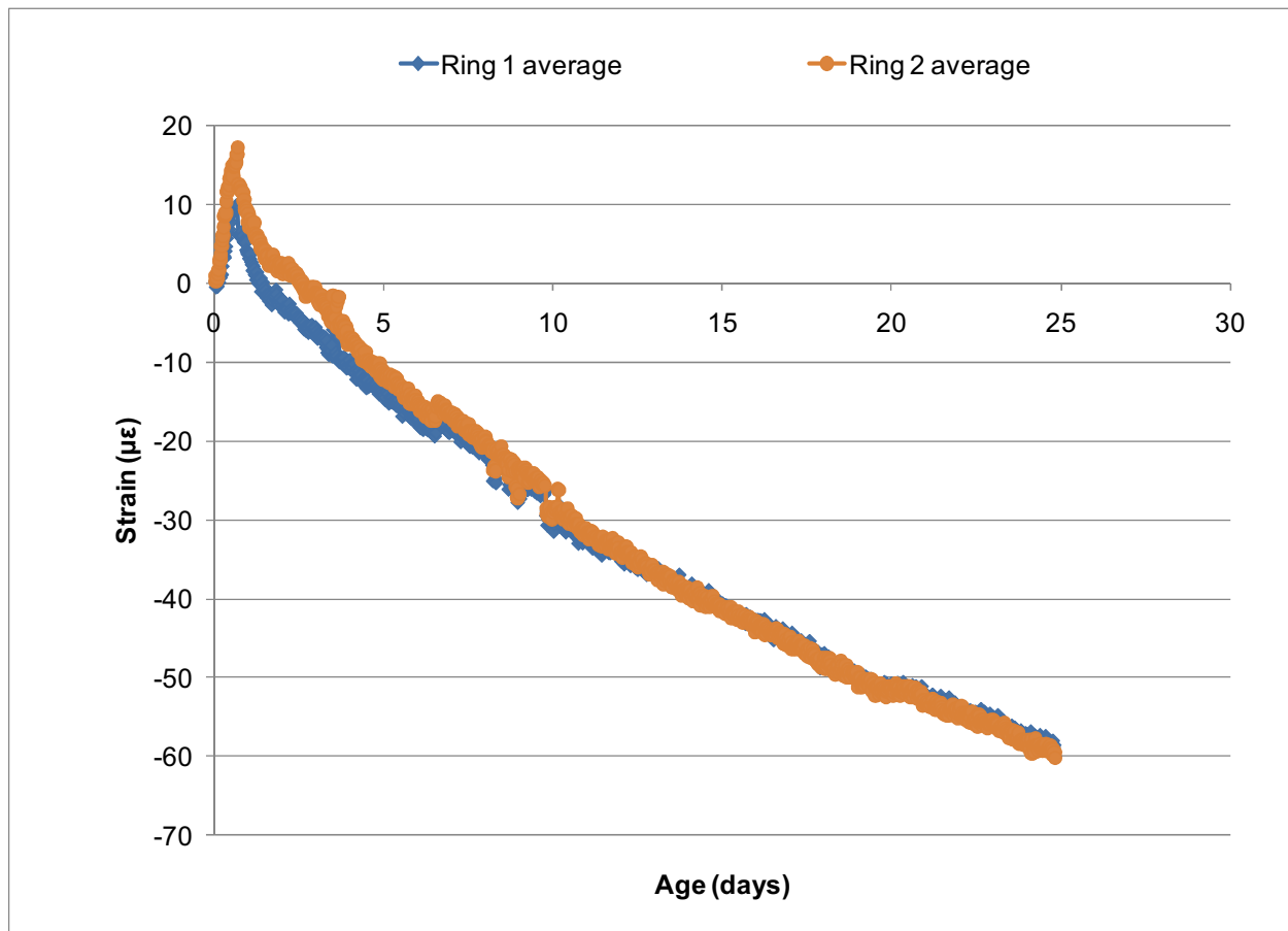
Figure C-5. Restrained Ring Shrinkage Strain for 3rdGen RCA MDOT P1 Concrete.
