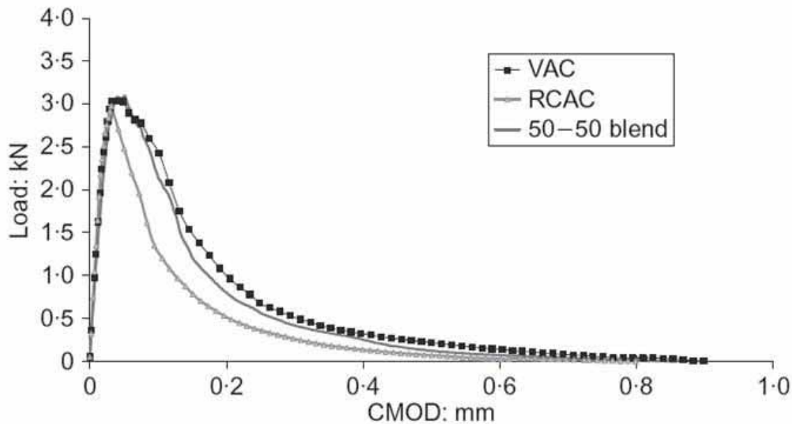
Figure 2-6. Average load-crack mouth opening displacement curves for virgin aggregate concrete (VAC), RCA concrete (RCAC), and 50-50 VA/RCA blend concrete mixtures after (Bordelon et al. 2009).
