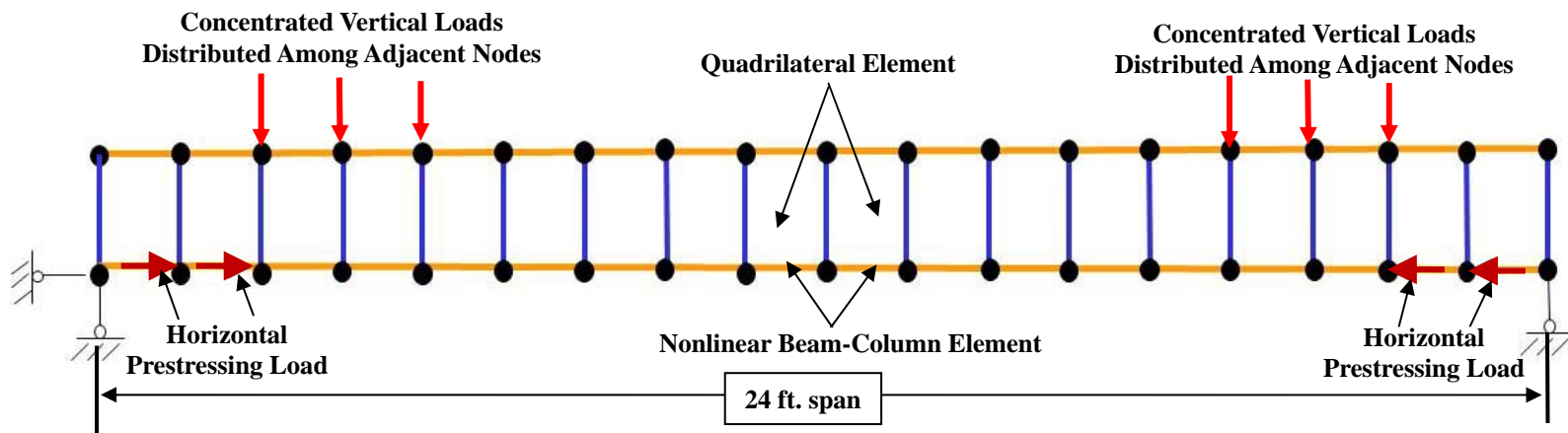
Fig. 9.5 Finite Element Model of Box-Beams Tested under Web-Shear ( a/d=2.5 )
