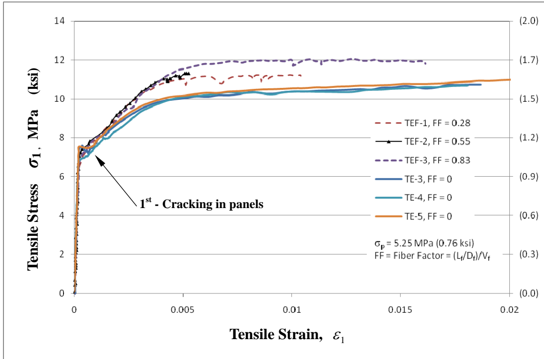
Fig. 5.1 \sigma_1 - \epsilon_1 Relationships in panels TEF-1, 2, and 3
