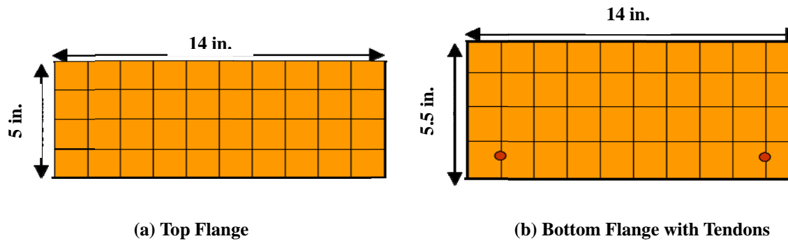
Fig. 9.7 Cross-Section Discretization of NonlinearBeamColumn Elements for Box-Beams Tested under Web-Shear
