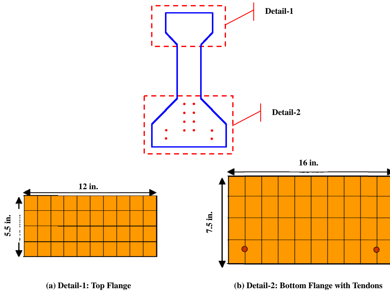
Fig. 9.3 Cross-Section Discretization of NonlinearBeamColumn Elements for PSFC I-Beams Tested under Web-Shear
