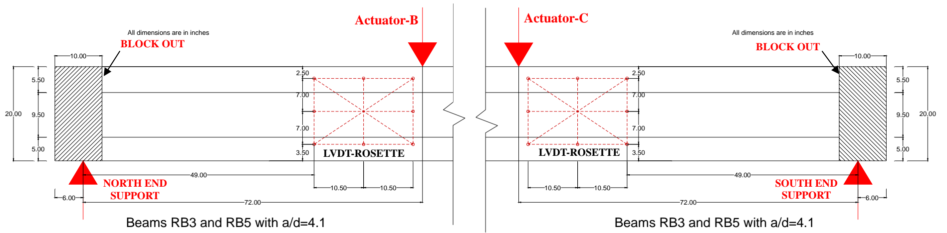
Fig. 8.8 (a): Load and Support Positions for PSFC Box-beams with a/d Ratio of 4.1
