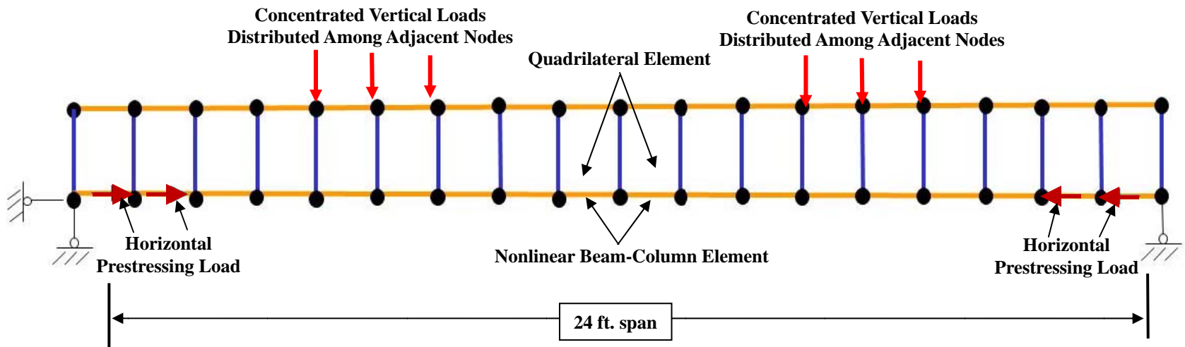
Fig. 9.6 Finite Element Model of Box-Beams Tested under Flexure-Shear ( a/d=4.1 )
