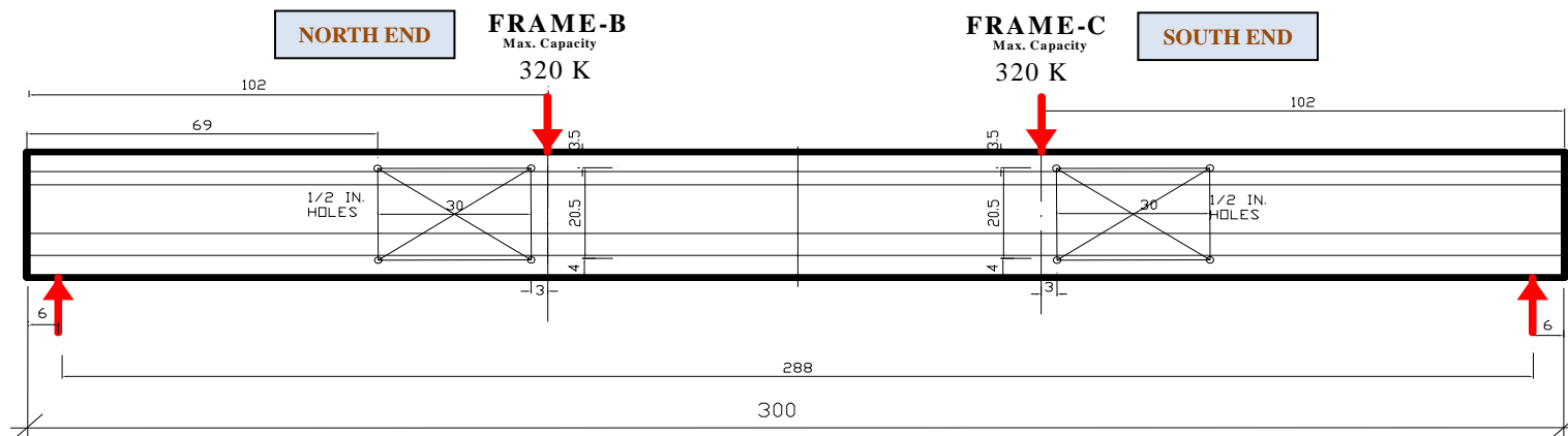
(b) Loading Points and LVDT Locations for Beams R5 and R6
