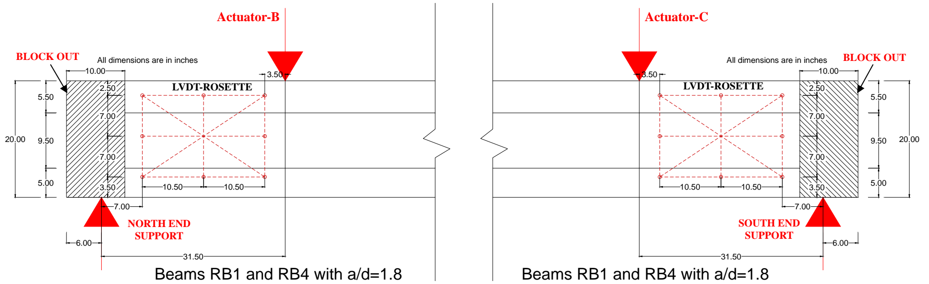
Fig. 8.8 (c): Load and Support Positions for PSFC Box-beams with a/d Ratio of 1.8
