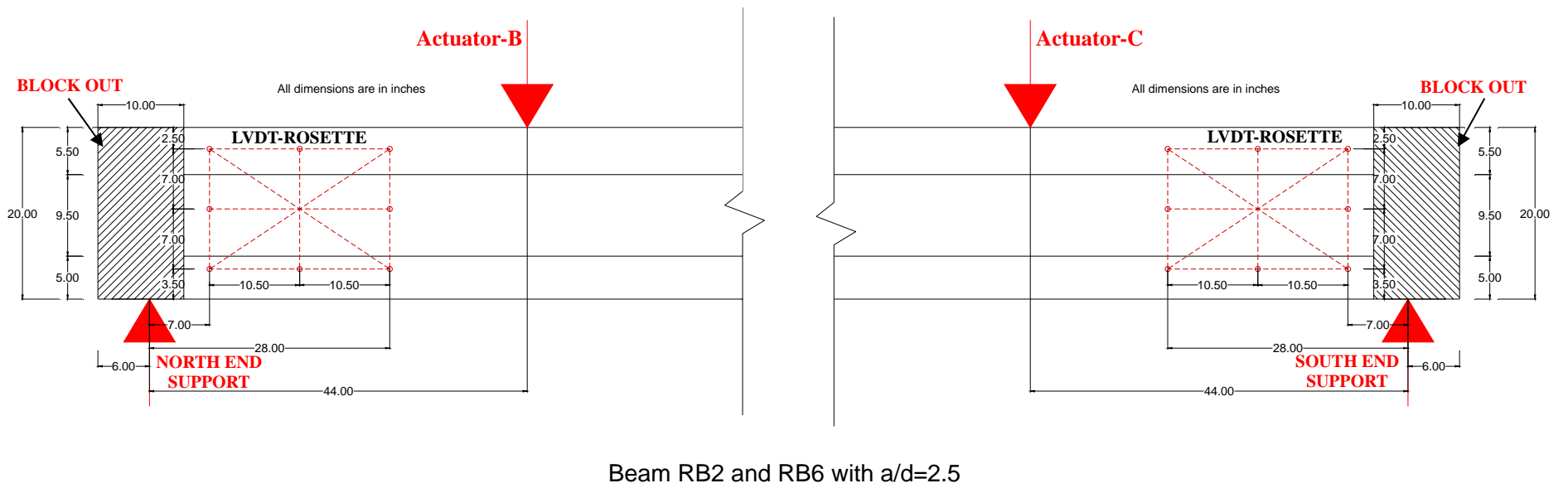
Fig. 8.8 (b): Load and Support Positions for PSFC Box-beams with a/d Ratio of 2.5
