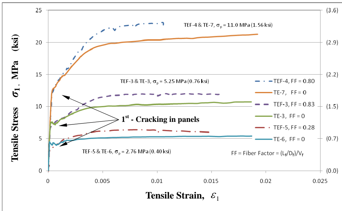
Fig. 5.2 \sigma_1 - \epsilon_1 Relationships in panels TEF-3, 4, and 5
