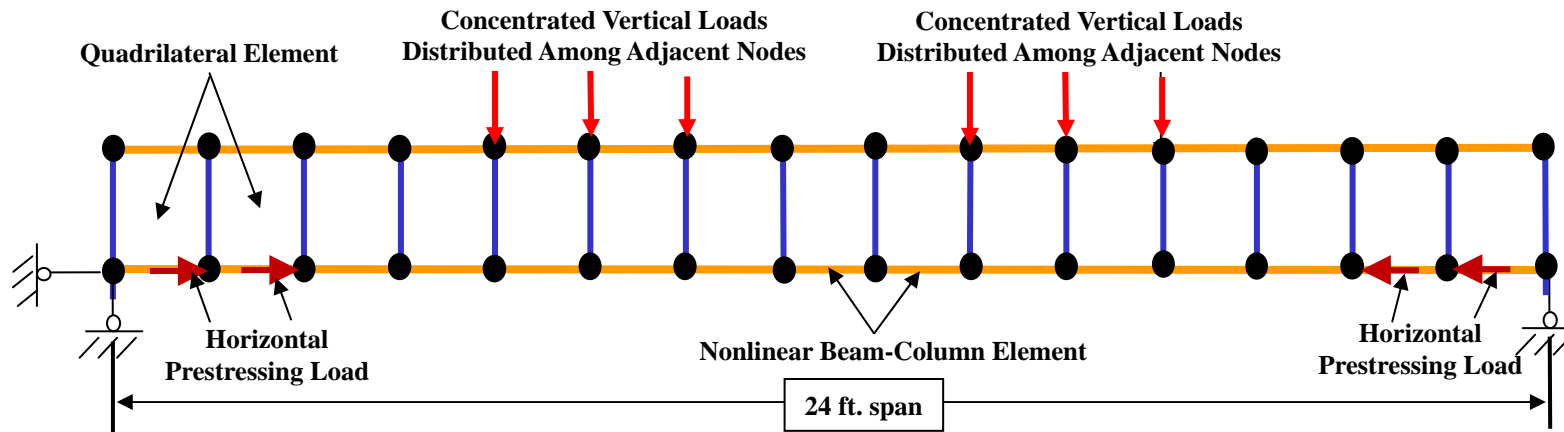
Fig. 9.2 Finite Element Model of PSFC I-Beams Tested under Flexural-Shear
