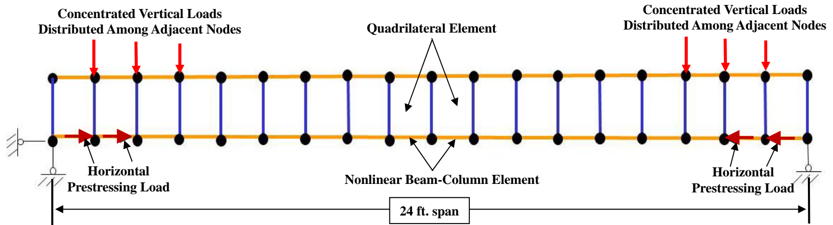
Fig. 9.4 Finite Element Model of PSFC Box-Beams Tested under Web-Shear ( a/d=1.8 )
