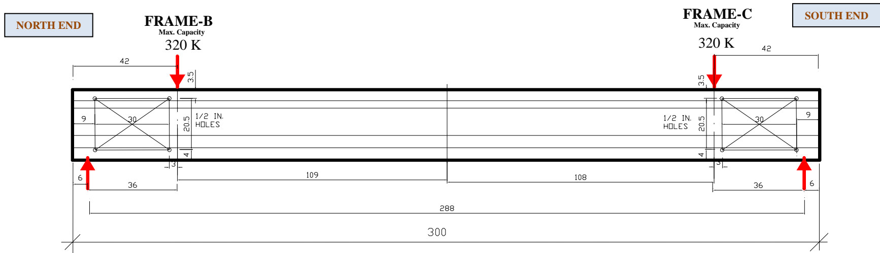
(a) Loading Points and LVDT Locations for Beams R1, R2, R3 and R4
