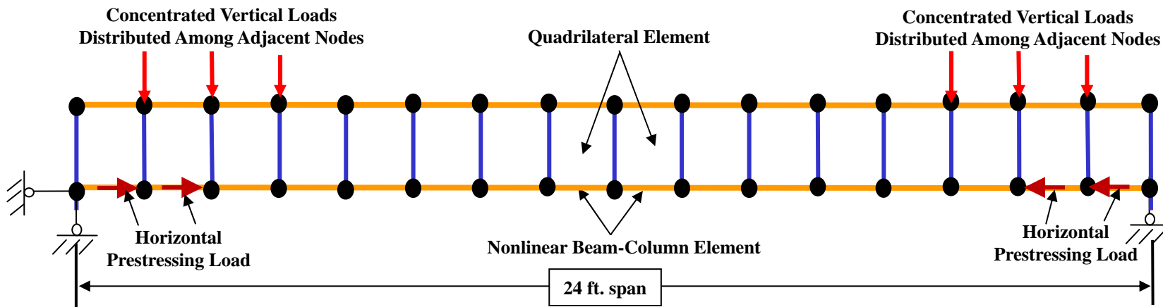
Fig. 9.1 Finite Element Model of PSFC I-Beams Tested under Web-Shear
