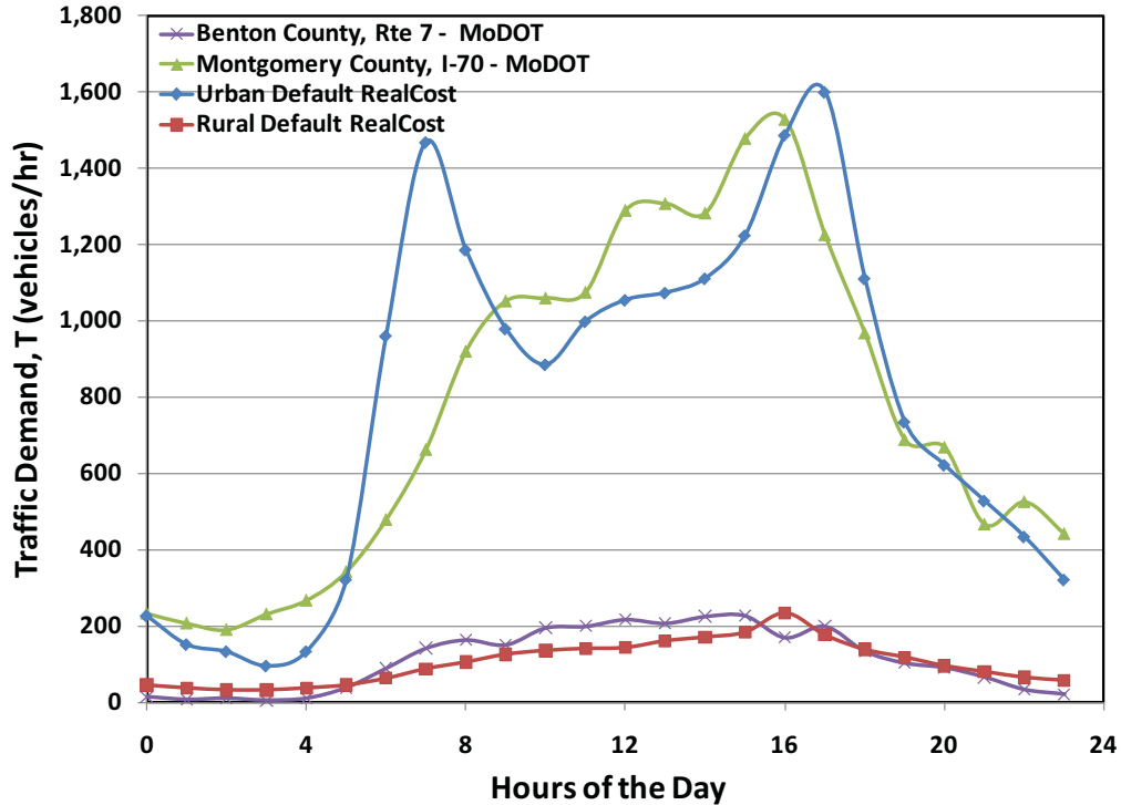
Figure 6-3: Hourly traffic demand history used for a typical urban (Montgomery County, I-70) and rural (Benton County, Rte. 7) used in the research are compared with default histories from RealCost.
