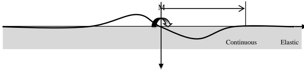
Figure 3-3 Slab of infinite length on continuous elastic support subjected to moment
