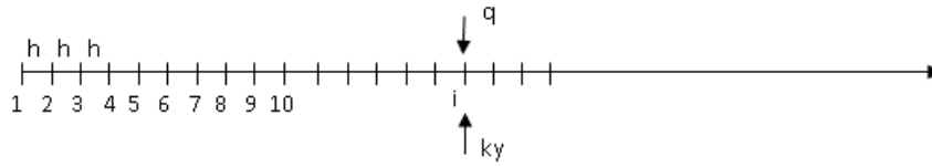
Figure 3-9 Finite length elements with distributed load, q , and soil pressure, k_y , on the nodes
