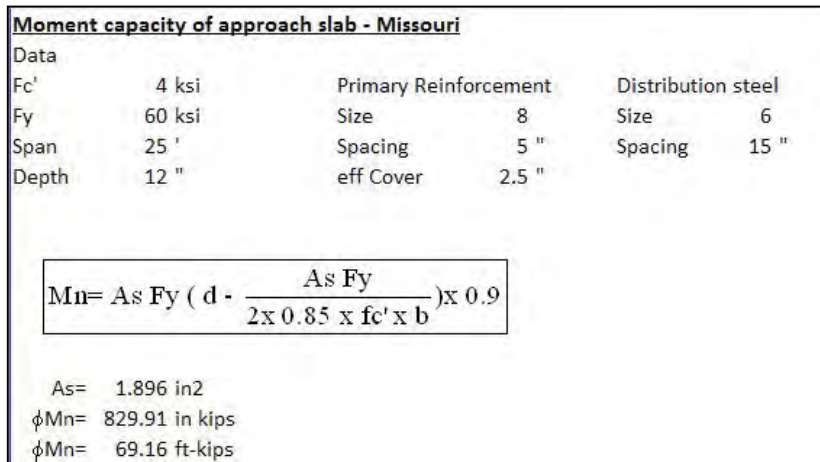
Figure 2-4: Singly reinforced moment capacity for Missouri BAS
