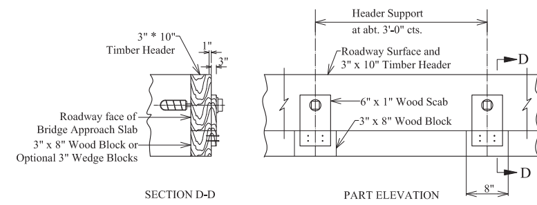
DETAILS OF TIMBER HEADER
