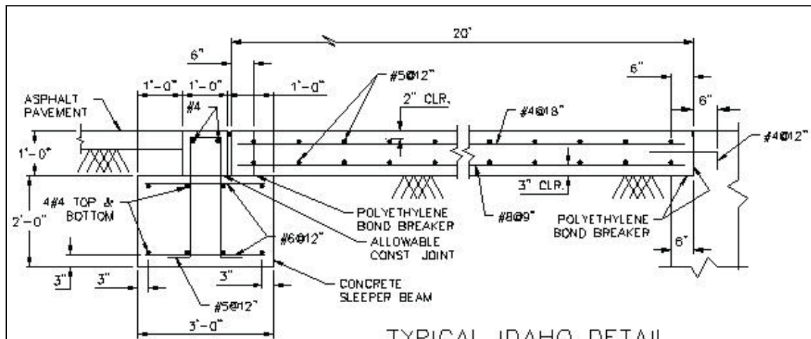
TYPICAL IDAHO DETAIL
