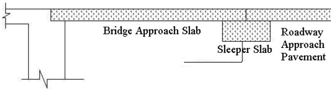
Figure 2-3: Missouri BAS Type 3
