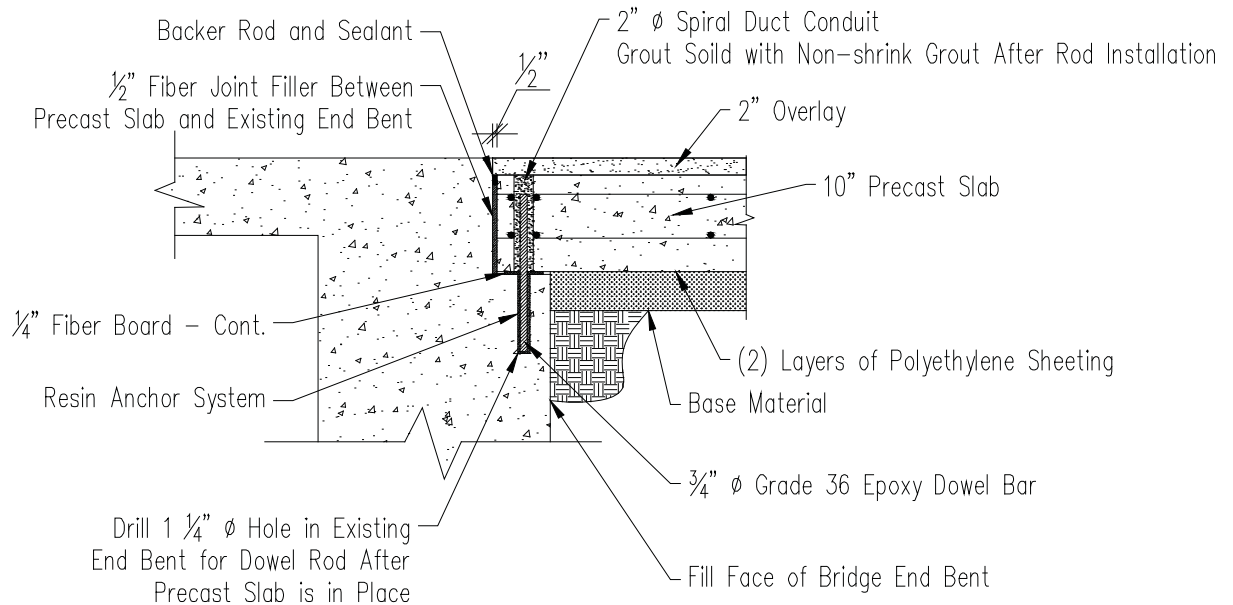
Figure 4-2 Abutment bearing detail
