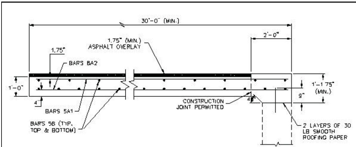
FLORIDA TYPICAL SECTION
