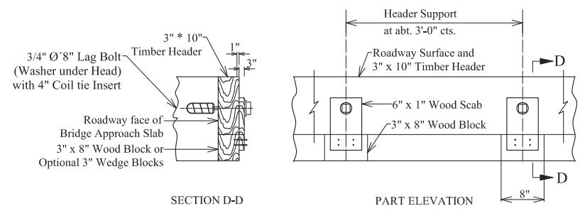
DETAILS OF TIMBER HEADER
