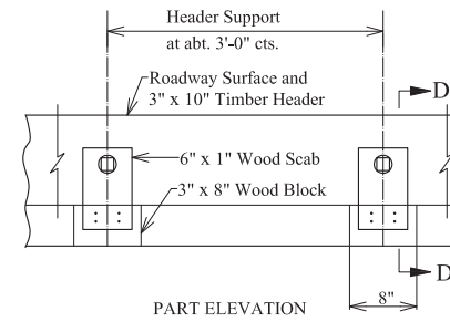
DETAILS OF TIMBER HEADER
