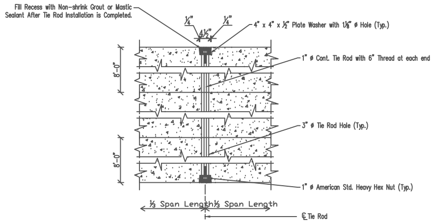
PART PLAN SHOWING 1" \phi TIE ROD
