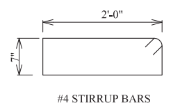
#4 STIRRUP BARS
