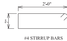
#4 STIRRUP BARS
