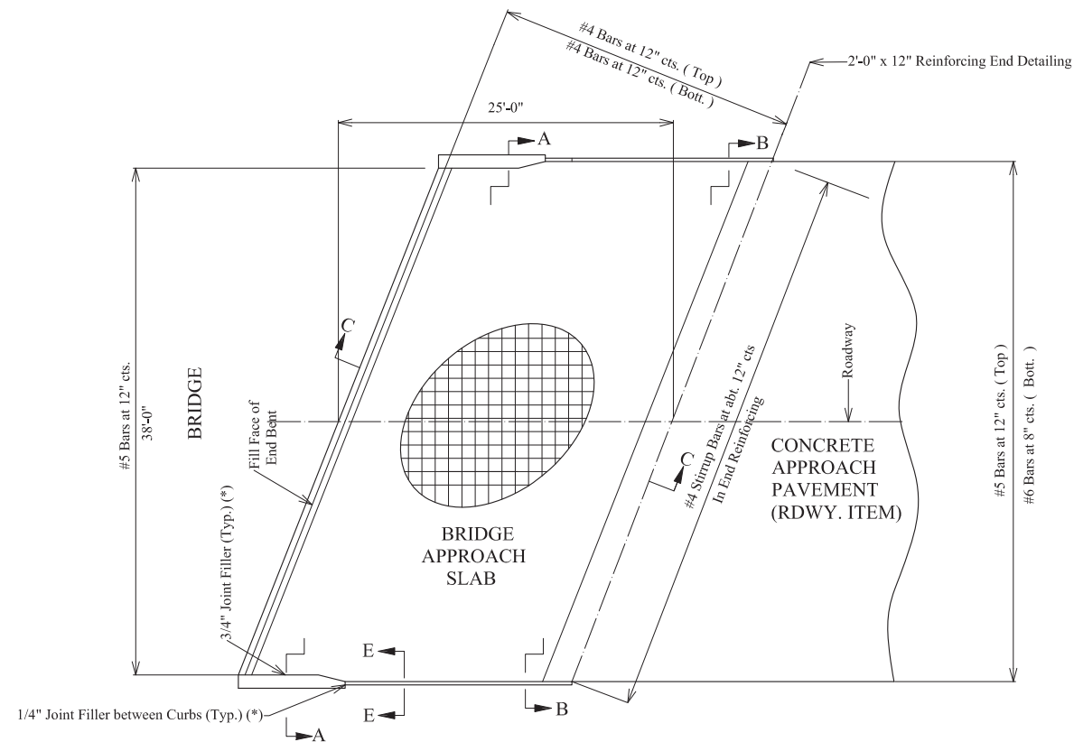
PART PLAN SHOWING REINFORCEMENT
