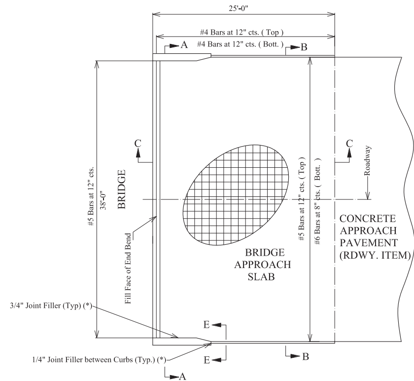
PART PLAN SHOWING REINFORCEMENT
