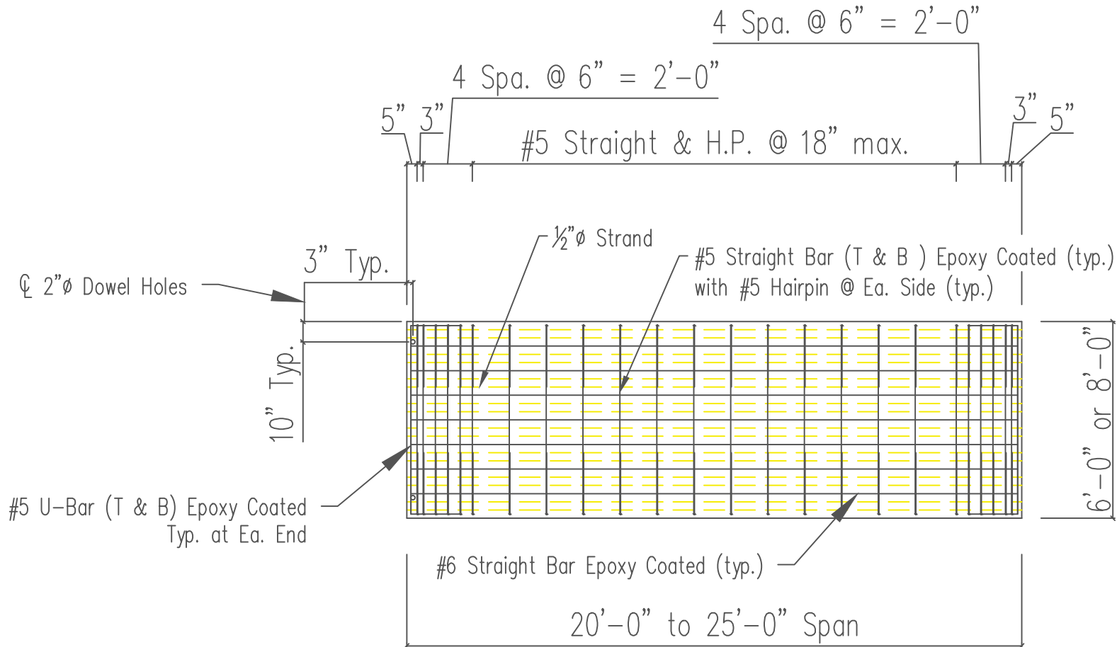
PANEL REINFORCEMENT - PLAN
