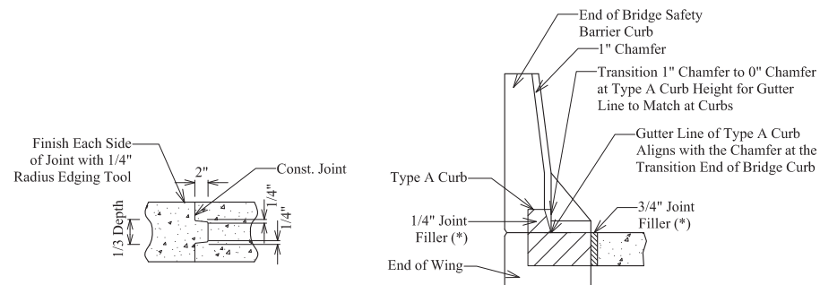
CONST. JOINT DETAIL (IF REQUIRED)
