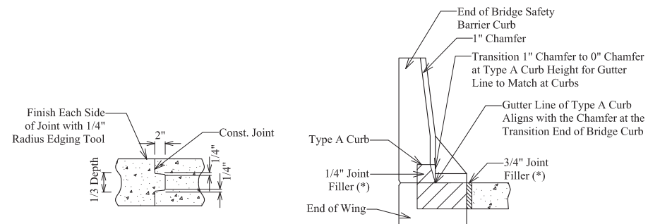
CONST. JOINT DETAIL (IF REQUIRED)
