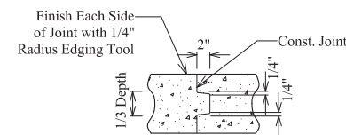
CONST. JOINT DETAIL (IF REQUIRED)
