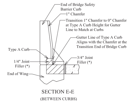
CONST. JOINT DETAIL (IF REQUIRED)
