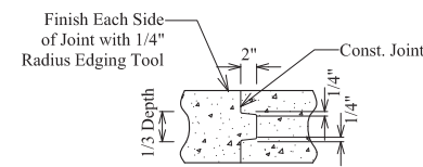
CONST. JOINT DETAIL (IF REQUIRED)
