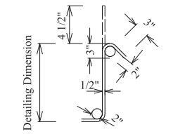
Typical 135° Stirrup Hook Dimensions Ending Diagram
