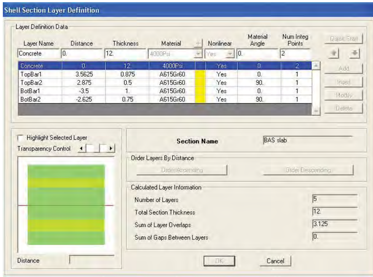
Figure 2-25: Shell area element layer definition
