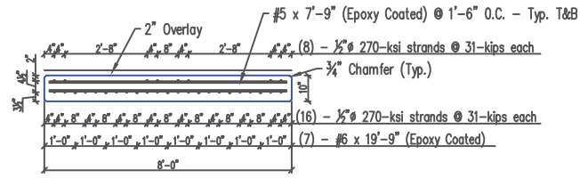
SECTION THROUGH SLAB
