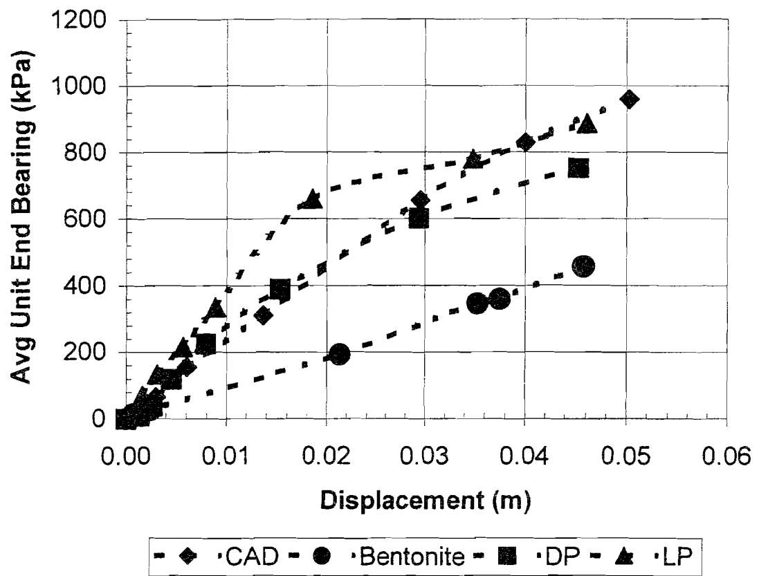
Figure 7 Load Transfer in End Bearing
