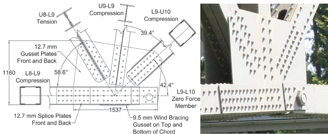
Figure 3-9 Joint L9 from BR 31-36
