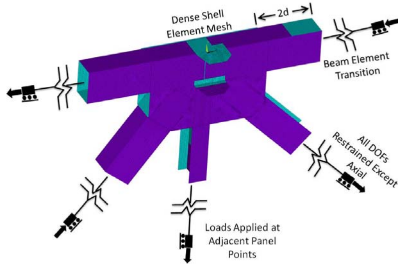
Figure 4-1 General Gusset Plate Connection Model
