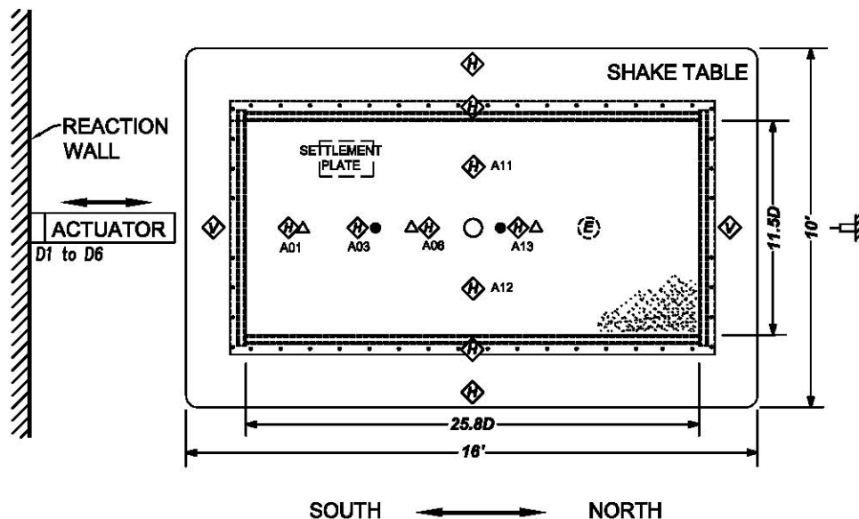
Figure 2-8. Accelerometers within the saturated soil layer (plan view)
