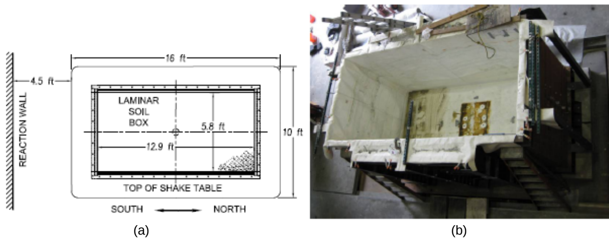
Figure 2-2: (a) Schematic of laminar soil box on shake table and (b) photograph of laminar box on shake table (plan views).
