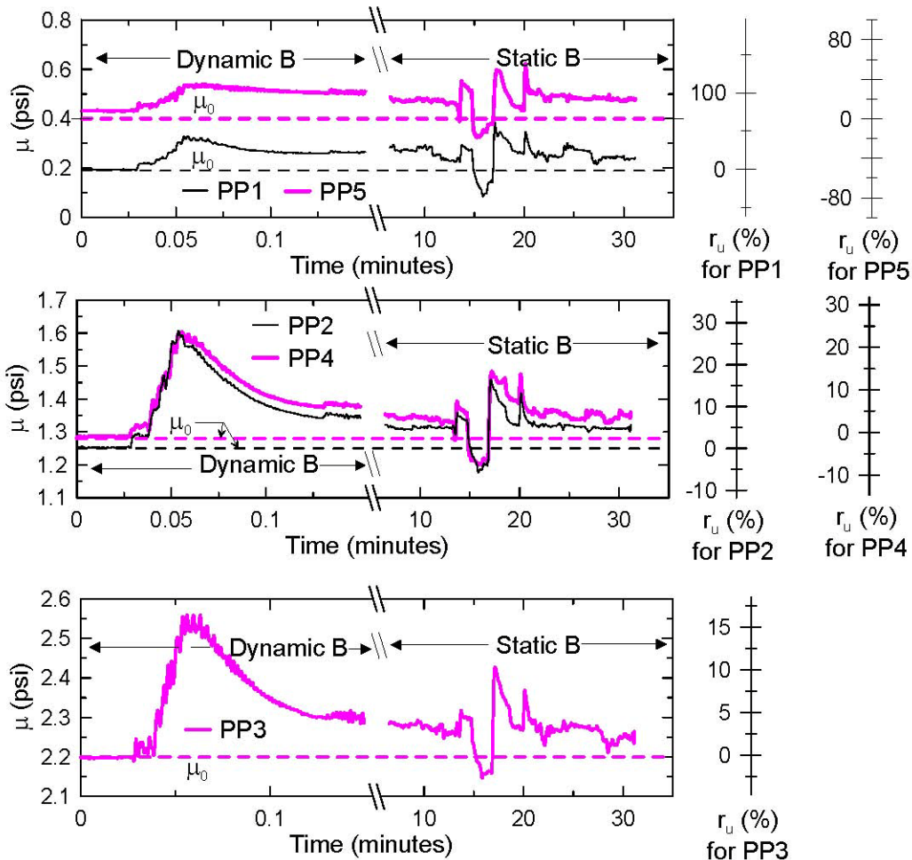
Figure 3-13. Pore pressure time history for Day 2 (dynamic B and static B)
