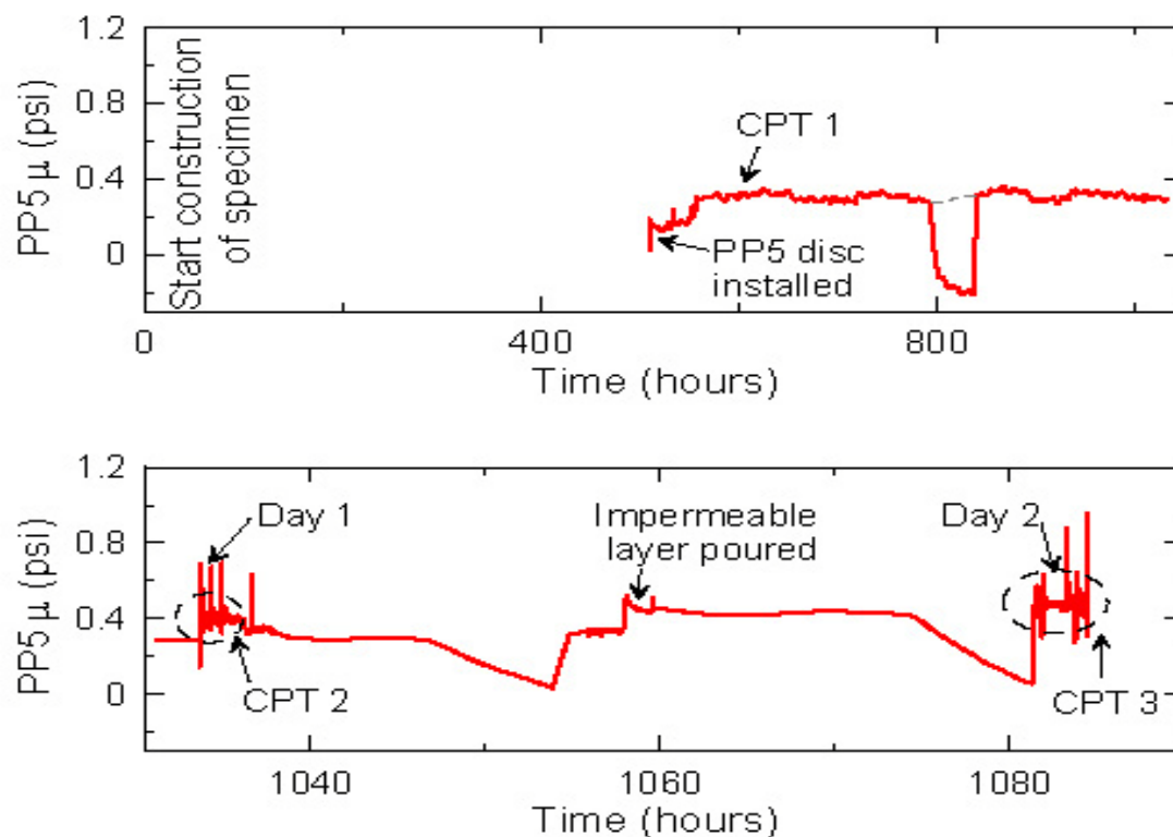
Figure 3-7. Test program duration pore pressure time history for instrument PP5
