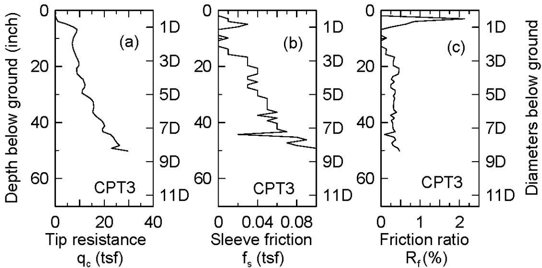
Figure 2-16: (CPT3, after second day of testing): (a) corrected tip resistance, (b) sleeve friction, and (c) friction ratio.
