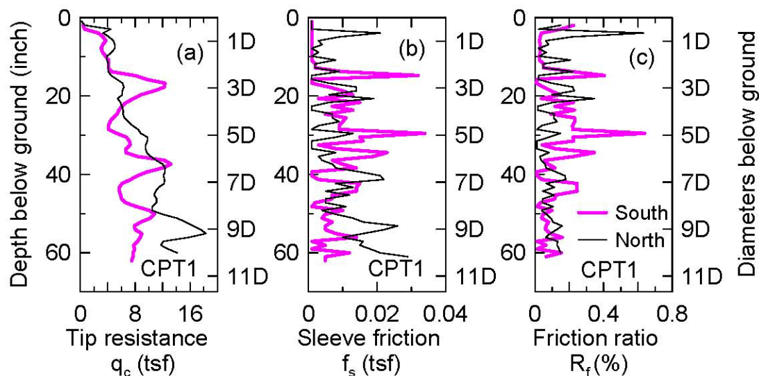
Figure 2-14: (CPT1, before testing of specimen): (a) corrected tip resistance, (b) sleeve friction, and (c) friction ratio.
