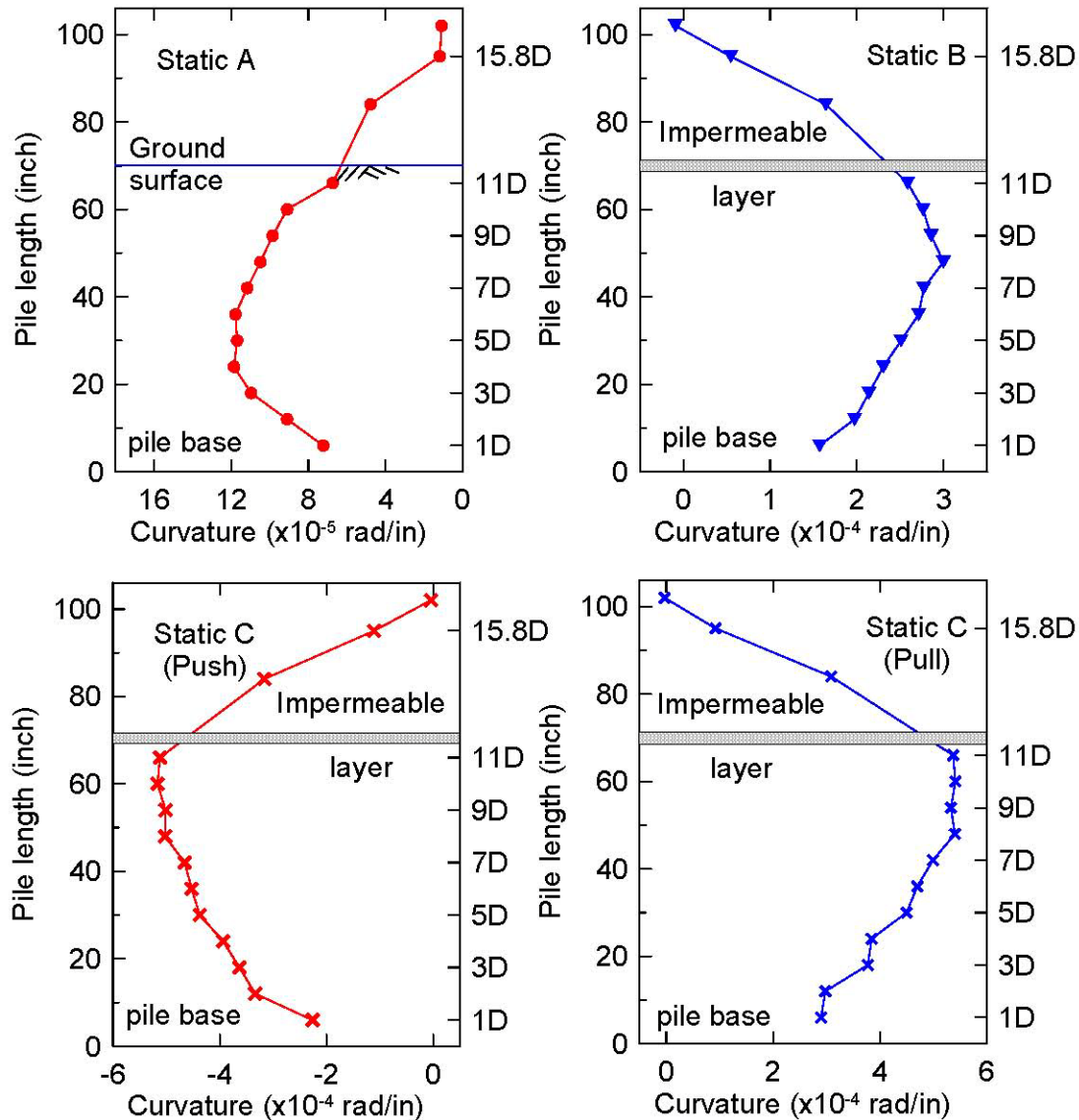
Figure 3-27. Maximum curvature distribution in the pile for static tests A, B, and C
