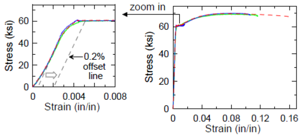
Figure 2-10. Stress-strain plots for steel coupons
