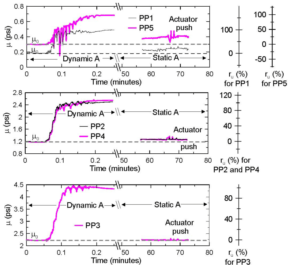
Figure 3-12. Pore pressure time history for Day 1 (dynamic A and static A)
