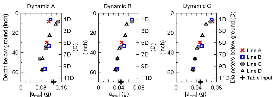
Figure 3-22: accelerations are uncorrelated, i.e. may occur at different times
