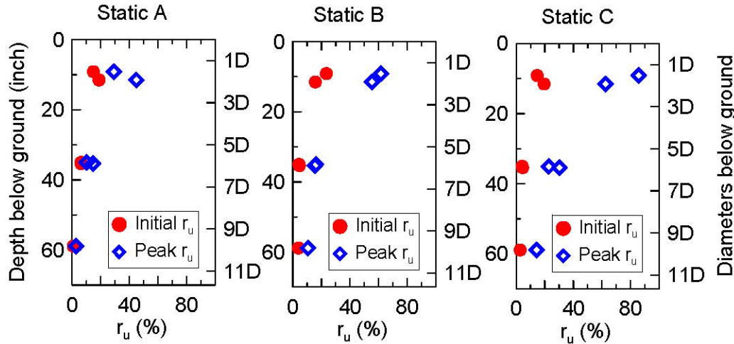
Figure 3-18. Profile of initial and peak r_u versus depth for static tests
