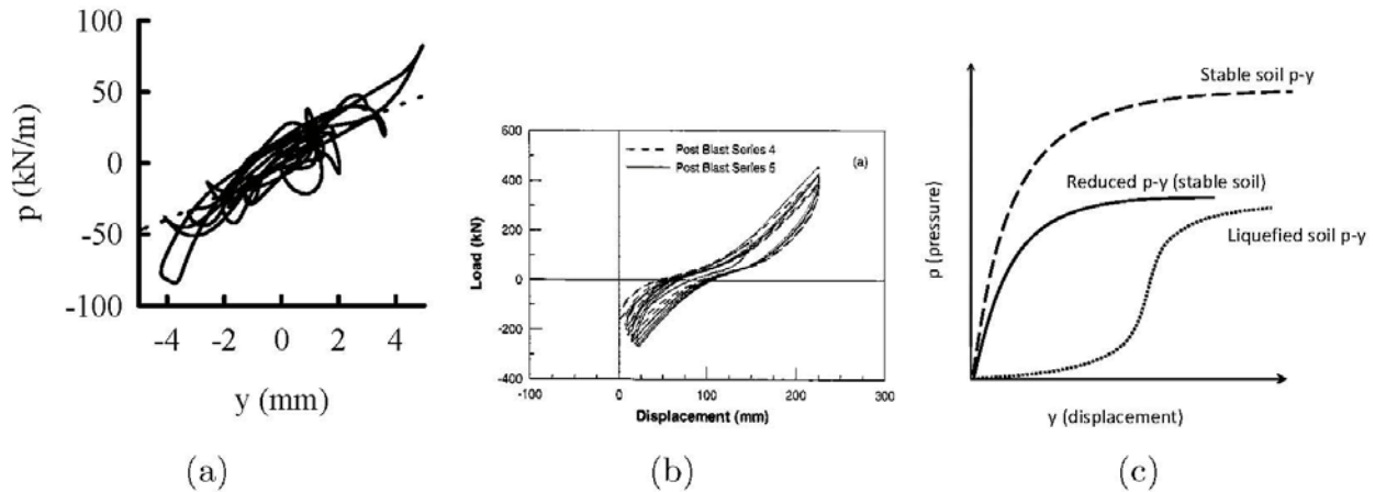
Figure 1-1: (a) sample p-y curve in liquefied soil (Wilson, 1998), (b) sample p-y curve in liquefied soil (Weaver, 2001), and (c) schematic of p-y curves with stable soil (API, 1993) and liquefied soil.
