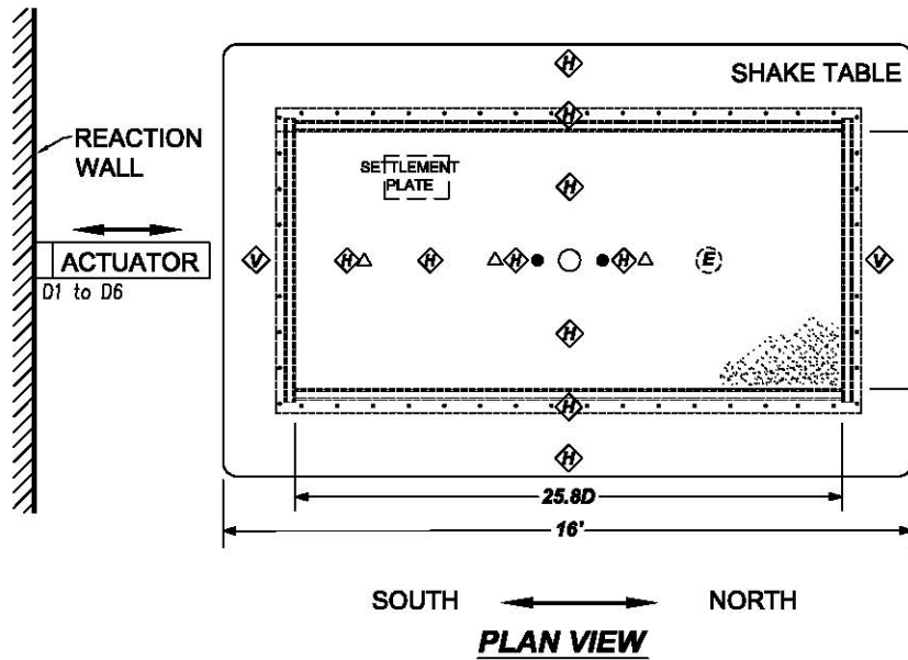
Figure 2-5. Instrumentation of saturated soil layer (plan view)
