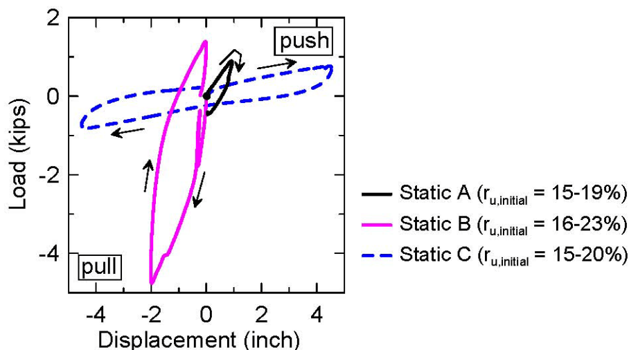
Figure 3-24. Overlay of lateral load versus displacement for all static tests
