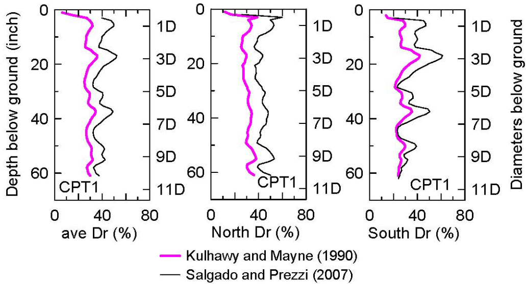
Figure 2-17. Comparison of average relative density, North boring, and South boring for CPT1
