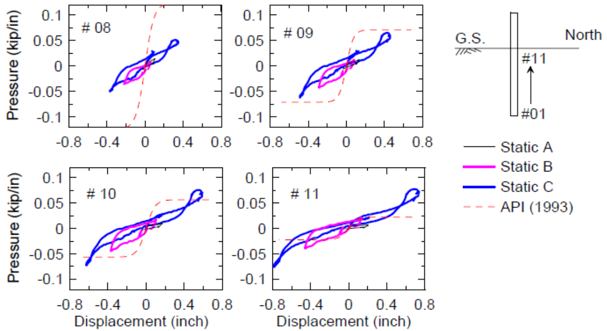
Figure 3-32: Dashed line denotes bilinear API p-y curve.
