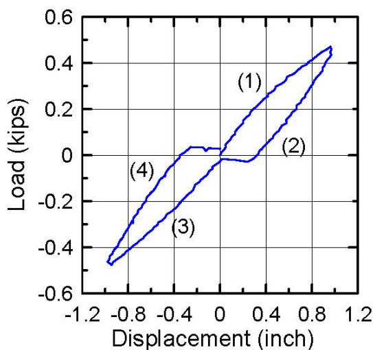
Figure 3-5. Actuator load versus top of pile displacement -push test without soil
