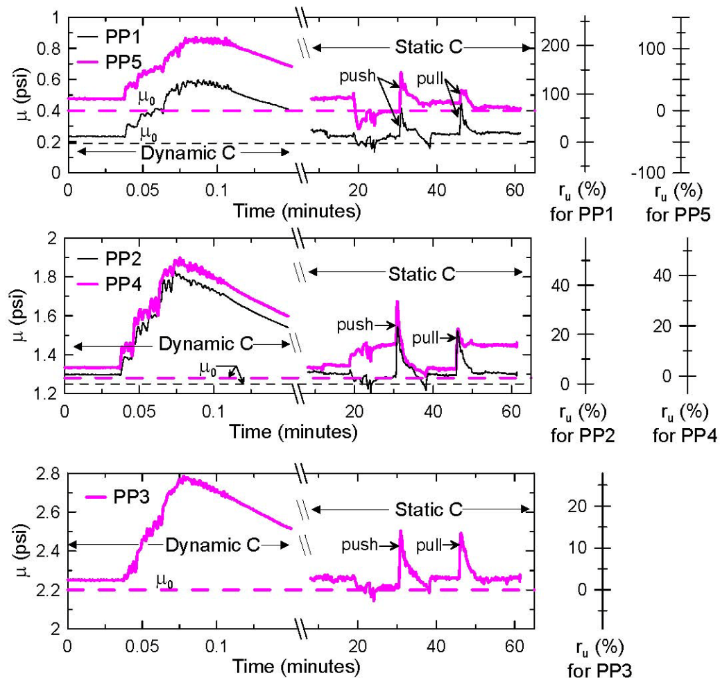
Figure 3-14. Pore pressure time history for Day 2 (dynamic C and static C)
