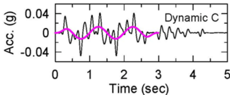
Figure 3-3. Dynamic C input motion time history (input shown in pink)
