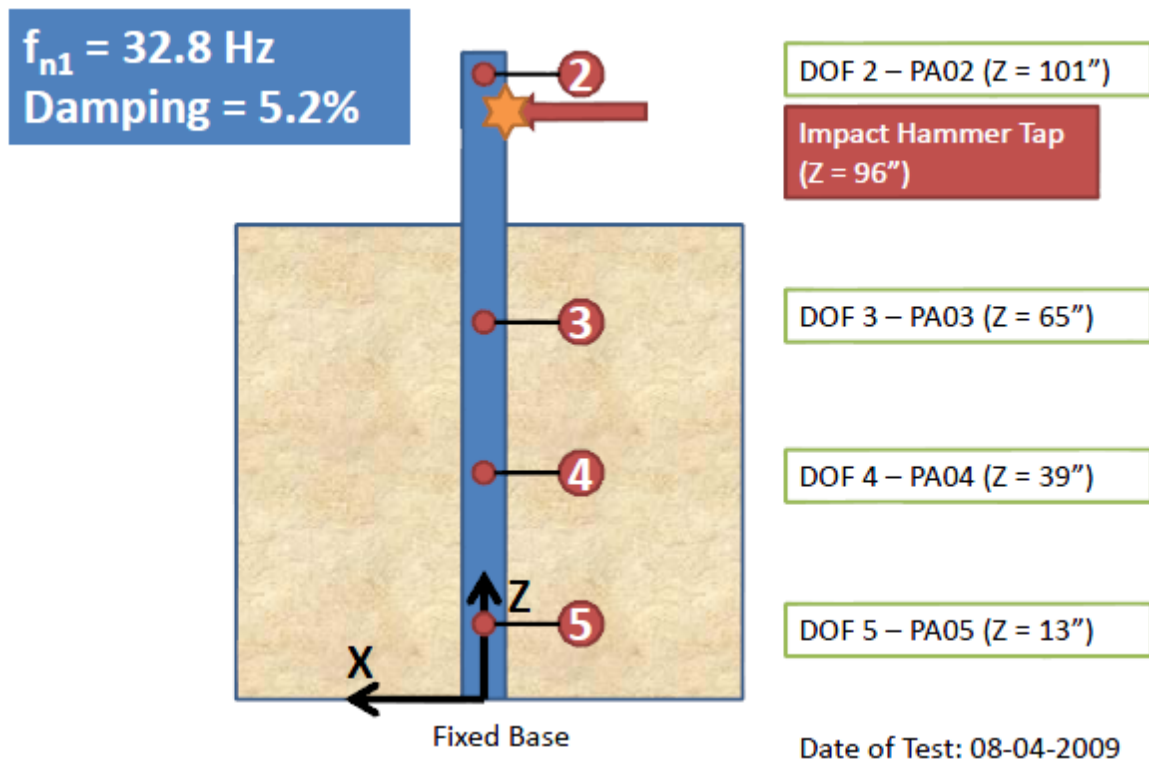
Figure 2-22. Non-destructive hammer test on pile soil system to obtain the natural frequency
