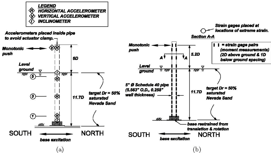
Figure 2-6: (a) accelerometers spaced vertically below the ground surface at 26" O.C. and (b) strain gages installed at north and south extreme sides of the steel pile.
