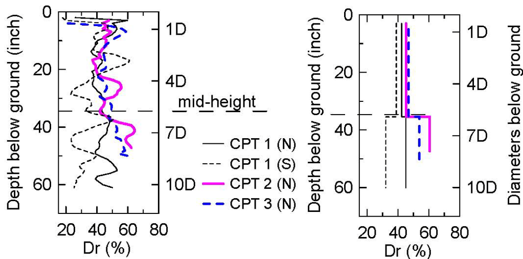
Figure 2-19: [Correlation of CPT data to relation of Salgado and Prezzi (2007)]
