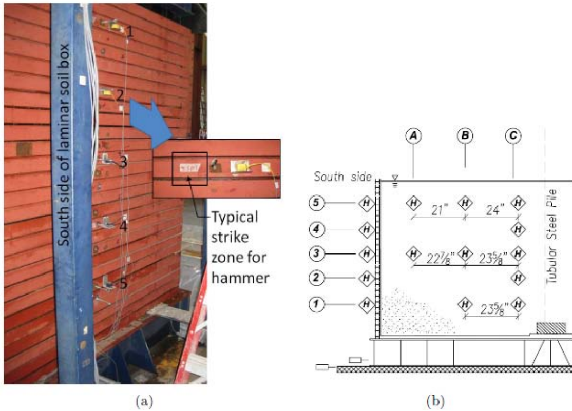
Figure 2-20: (a) South side of box with hammer strike zones indicated and (b) schematic of south side of soil box.
