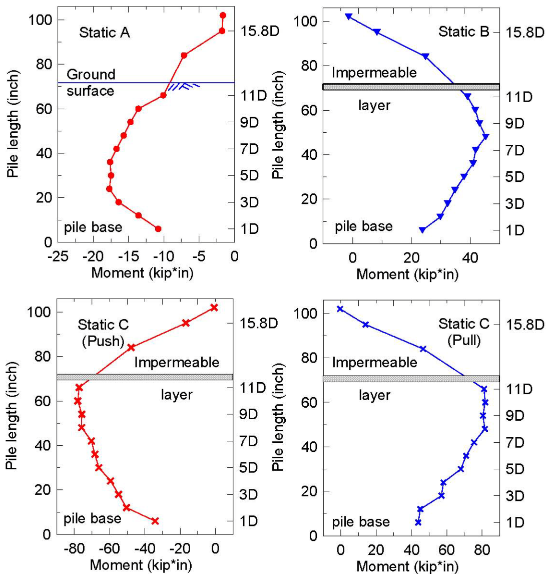
Figure 3-26. Maximum moment distribution in the pile for static tests A, B, and C
