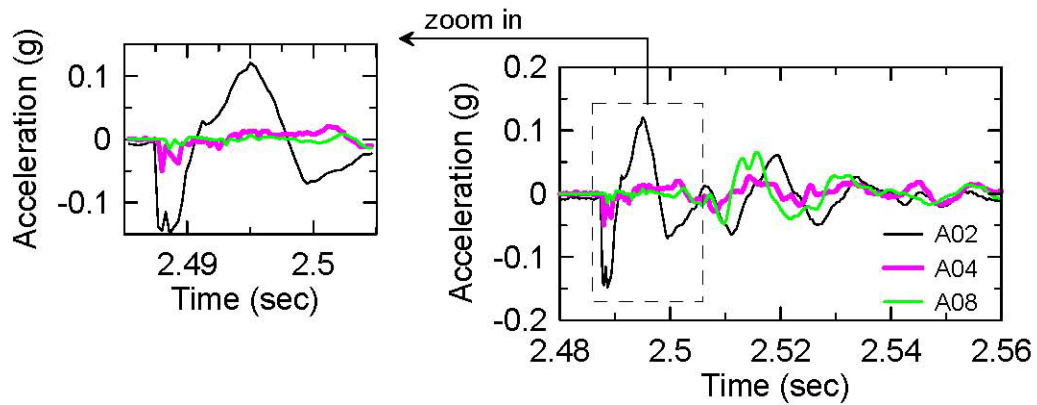
Figure 2-21. Sample acceleration pulses from accelerometers used for determining p-wave velocity
