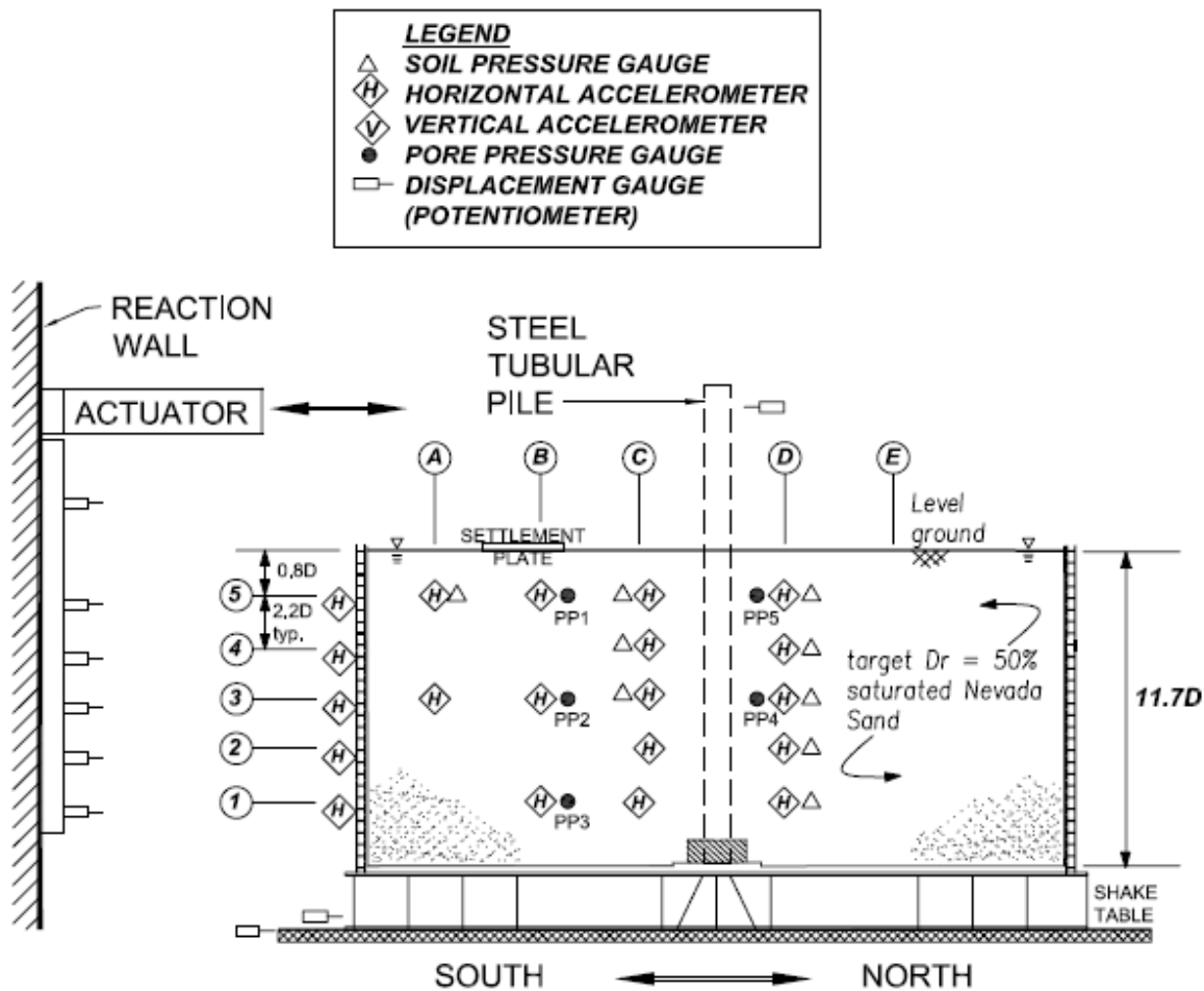
Figure 2-4: Lines 1 to 5 are vertically spaced at 13" O.C. Instruments at line A are 10D away from the pile face; instruments at line B are placed 6D from the pile face; instruments at lines C and D are placed 3D away from the pile face. Line E denotes the location of the CPT profiles and is located 6D from the pile face.
