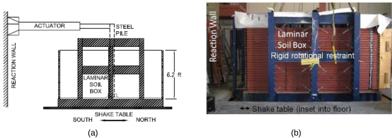
Figure 2-1: (a) Schematic of laminar soil box on shake table and (b) photograph of laminar box on shake table (elevation views).
