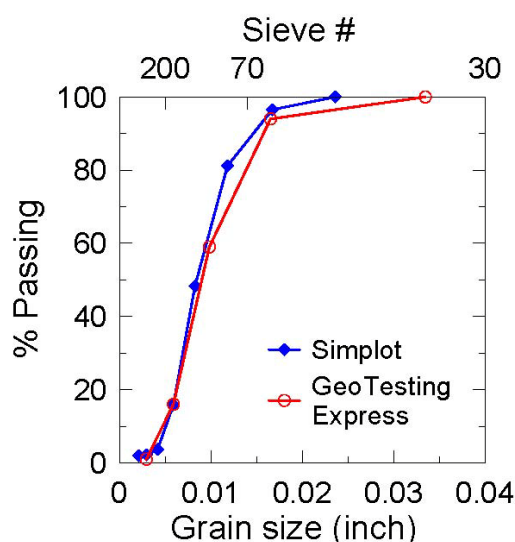
Figure 2-12. Nevada Sand #60 grain size distribution
