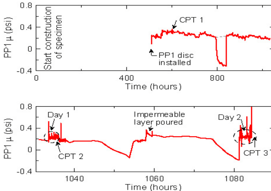
Figure 3-6. Test program duration pore pressure time history for instrument PP1
