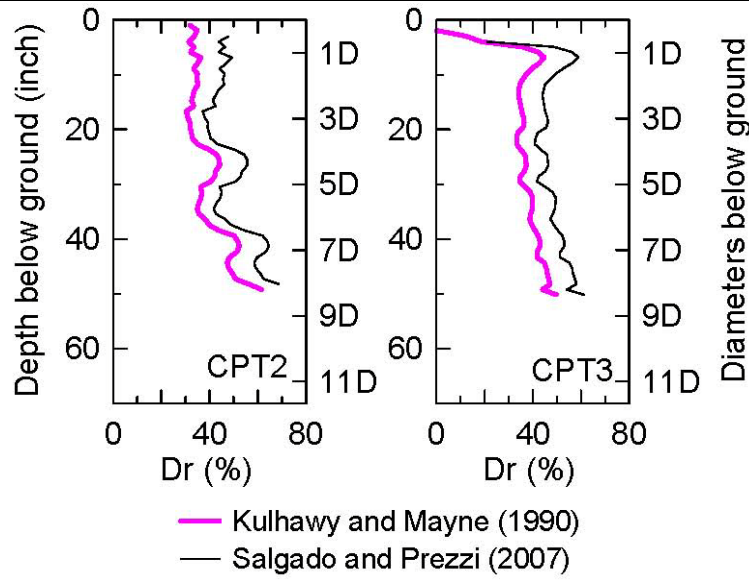
Figure 2-18. Comparison of relative density, North boring only for CPT2 and CPT3
