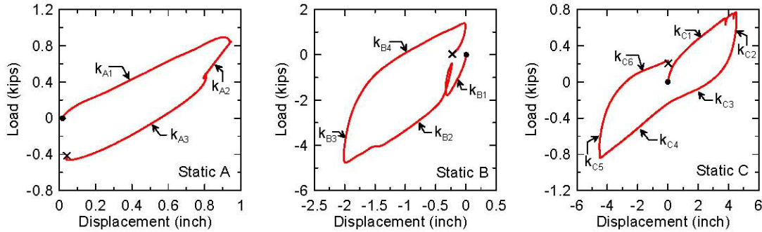
Figure 3.23: Closed "o" denotes the beginning of the test; "x" denotes the end of the test.
