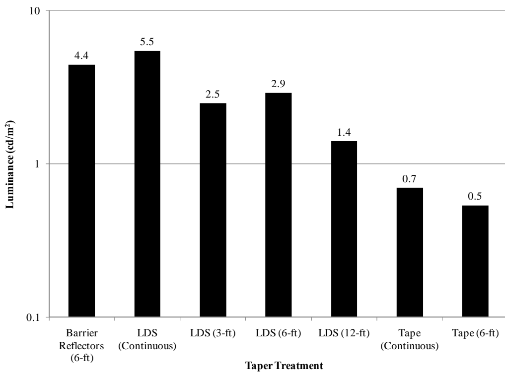
Figure 23. Luminance Data for Phase II Taper Treatments.
