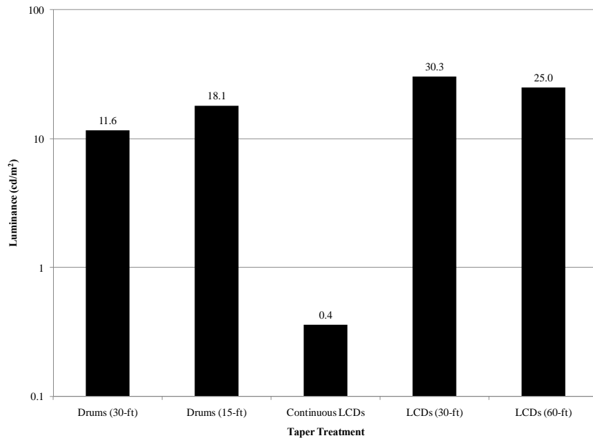
Figure 21. Luminance Data for Phase I Taper Treatments.
