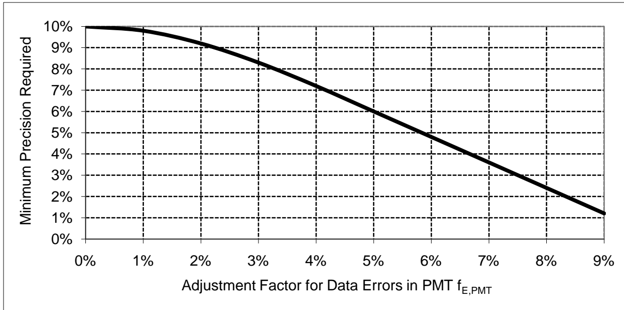
Figure 4.3. Errors in Unadjusted PMT and Minimum Precision
