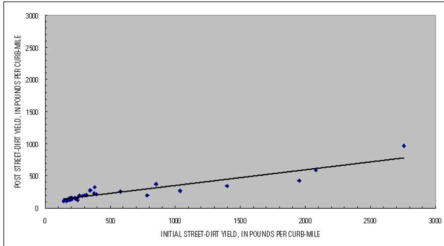
Figure 3-2. Post cleaning street dirt yields as a function of initial street dirt yields for the vacuum assisted street cleaner.
