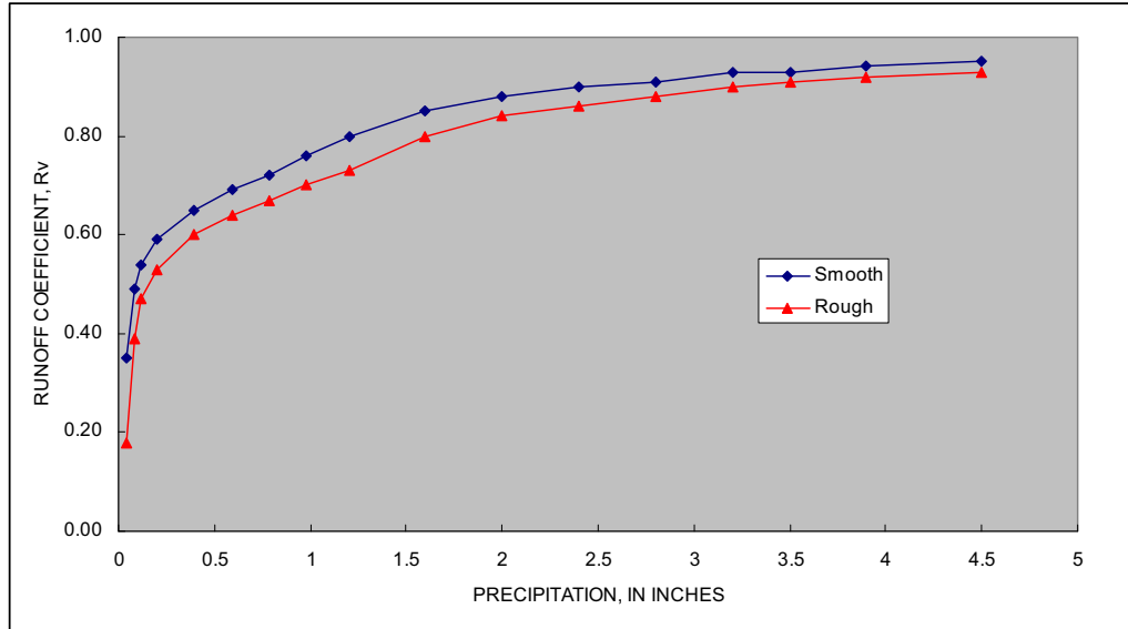
Figure 3-3. Street-runoff coefficients used in WinSLAMM.
