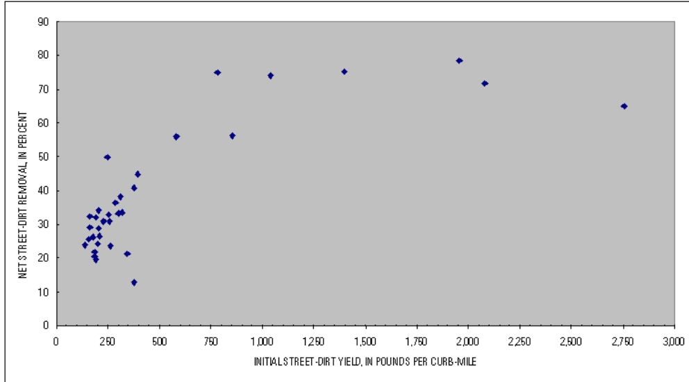
Figure 12. Change in street cleaning efficiency of the vacuum assisted machine with increasing street-dirt yields.
