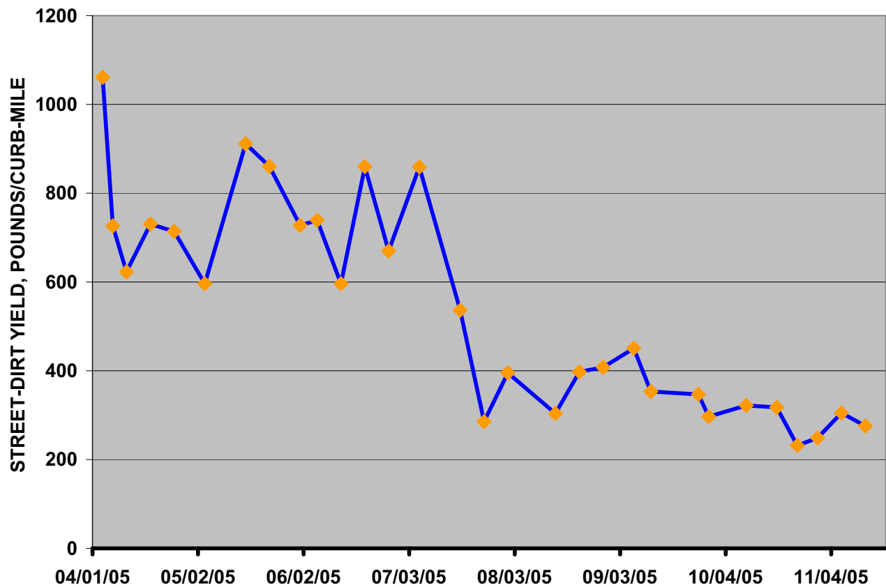
Figure 3-1. Measured changes in street-dirt yield over time at the unswept section.
