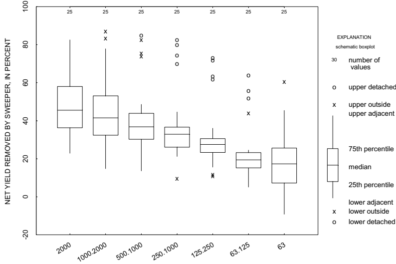
Figure 13. Street cleaning removal for the vacuum assisted machine by particle-size distribution in the swept-section.
