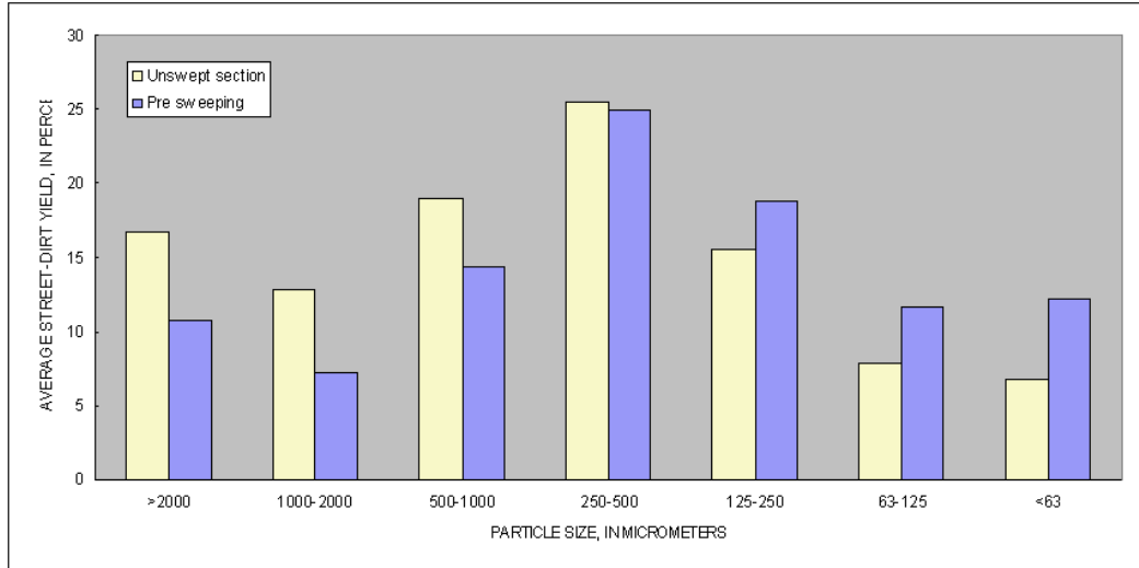
Figure 7. Average particle-size distributions in the street dirt at the swept and unswept sections.
