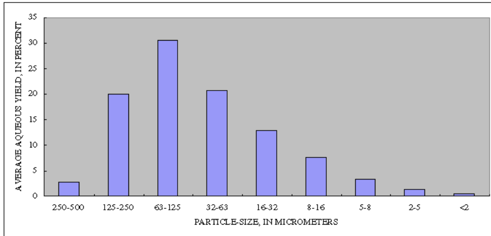
Figure 22. Average percent mass in each particle size for sediment in the water-quality samples.
