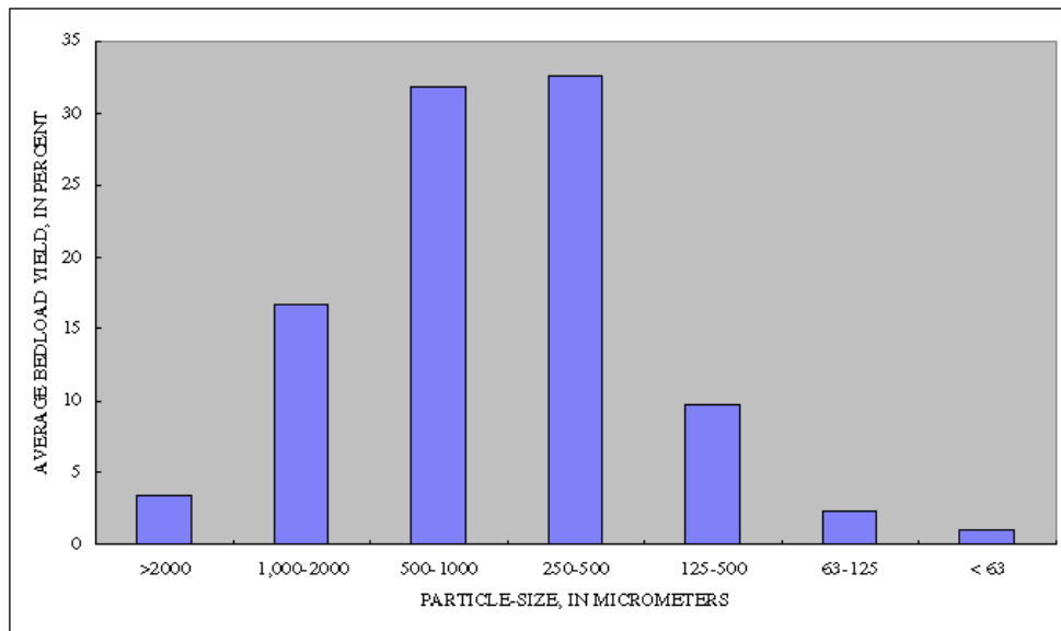
Figure 24. Average percent mass in each particle size for sediment collected in the bedload sampler.
