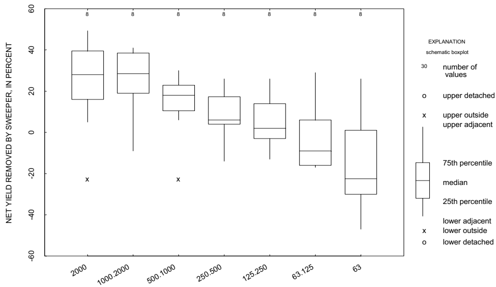
Figure 15. Street cleaning removal for the mechanical broom machine by particle-size distribution in the swept-section.
