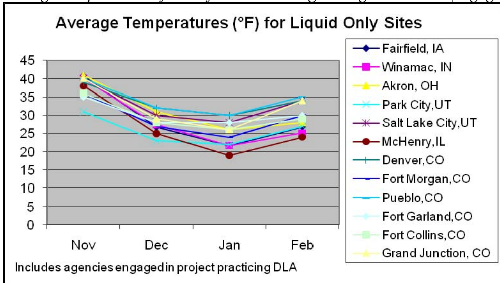
Average Temperatures of Identified Areas Using During-Storm DLA (engaged in study)
