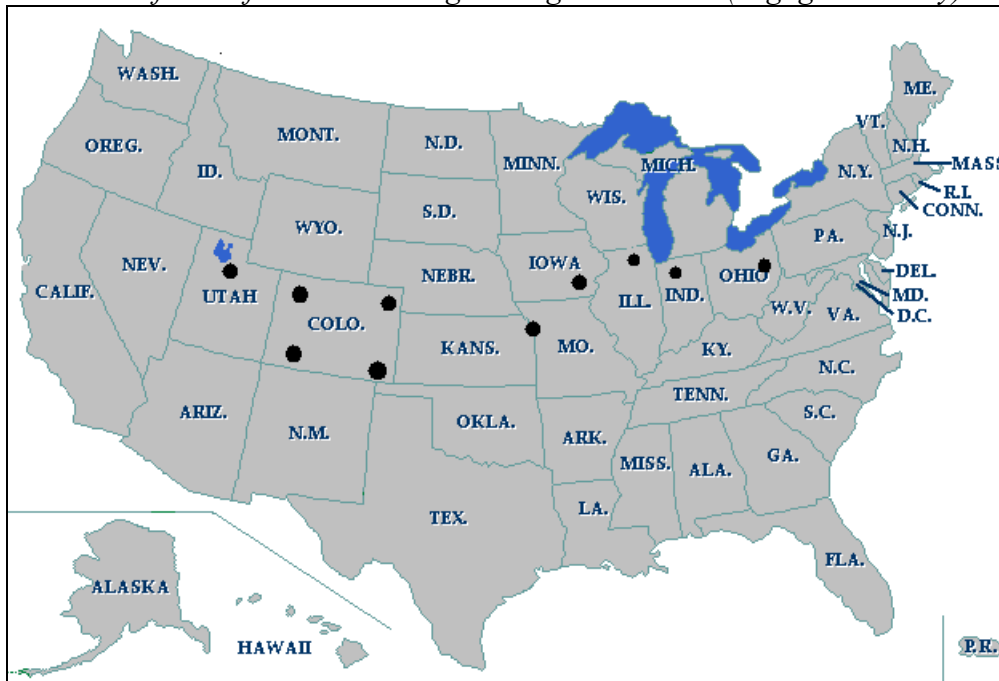
Locations of Identified Areas Using During-Storm DLA (engaged in study)
