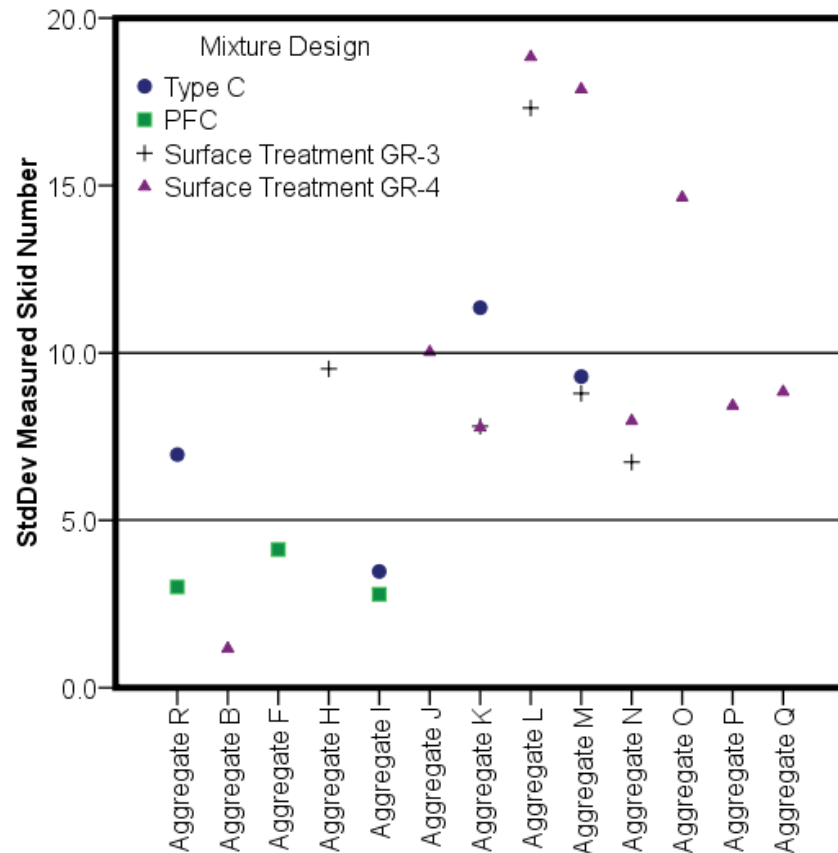
Figure 11. Standard Deviation of the Measured SN Values for Low TMF Level.
