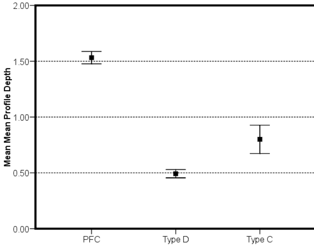
Figure 20. Measured MPD Values for Different Mix Types.
