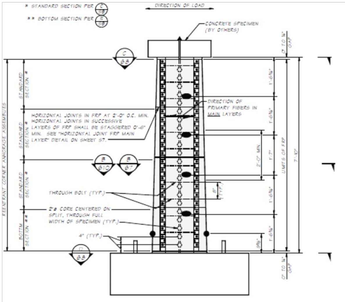
Figure 13 – Retrofit Details for the Split Columns (1 in. = 25.4 mm)
