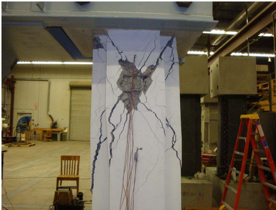
Figure 18 – Column 1 Shear Cracking Near the End of Testing
