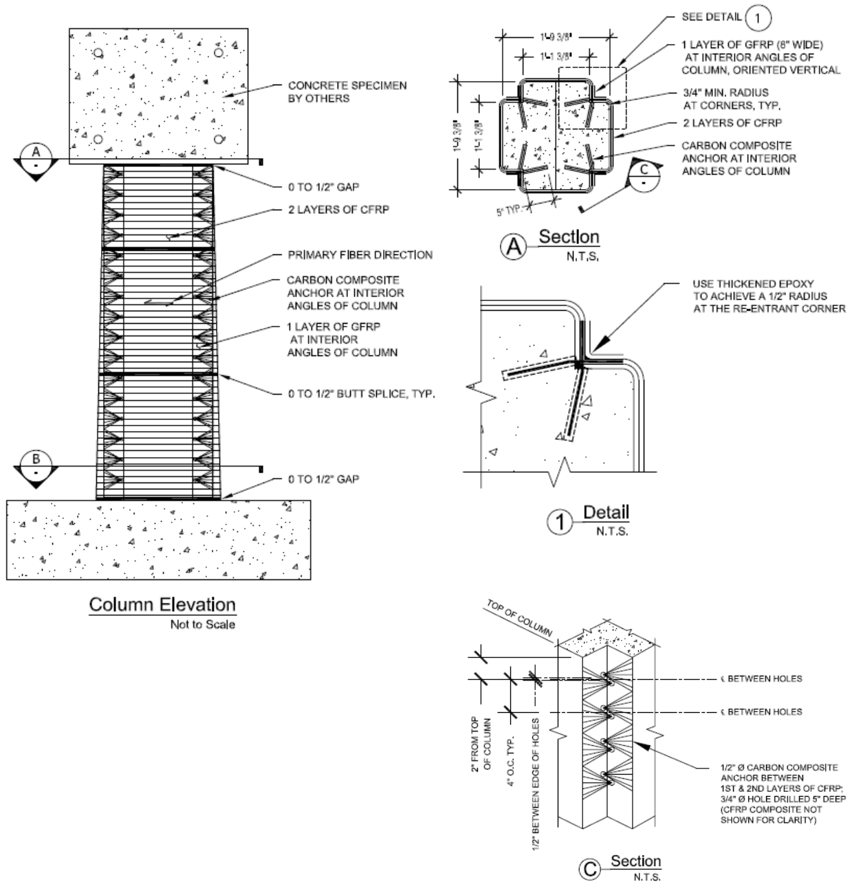
Figure 11 – FRP Anchor Retrofit Details (1 in. = 25.4 mm)
