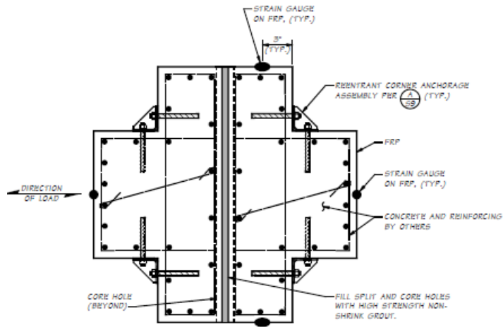
SECTION A SPLIT SPECIMEN
