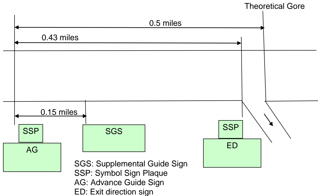
Figure 28 Placement of Different Types of Signs
