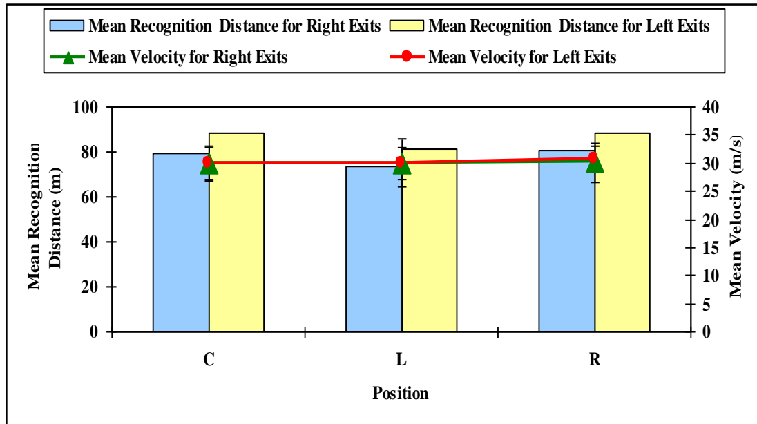
Figure 19 Mean Recognition Distance and Velocity at Different Positions
