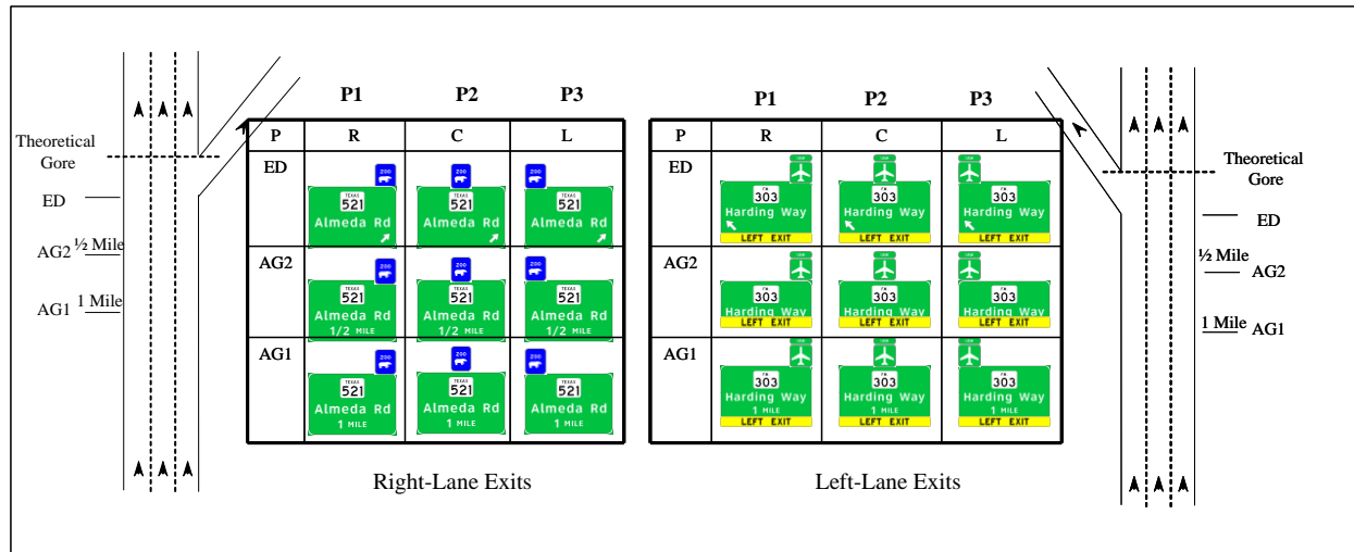
Figure 14 Positions of Symbol Signs on Advance Guide Signs and Exit Direction Signs.
