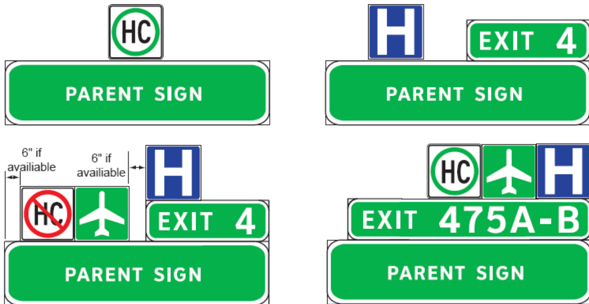
Figure 16 Overhead Freeway Guide Sign and Routing Plaque Typical Assemblies
