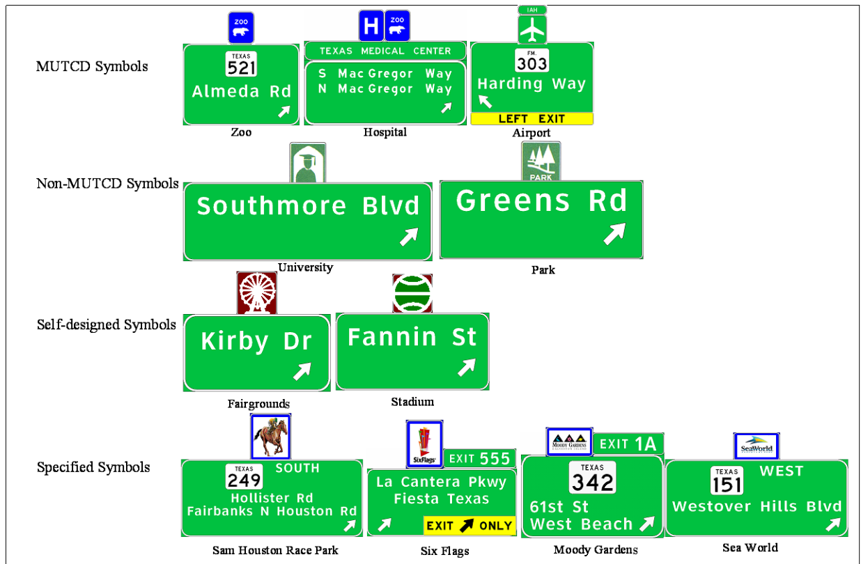
Figure 13 Test Symbols on Top of Various Guide Signs
