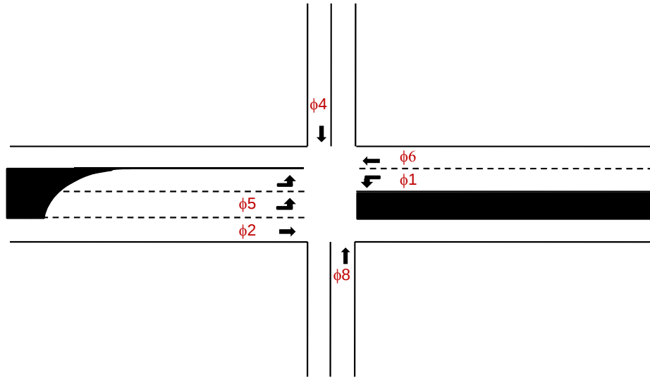
Figure 20. Geometric Layout for Dual Left-Turn Bay Experiments.
