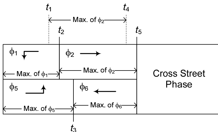
Figure 19. Phasing Sequence Example for Fully-Actuated Control.
