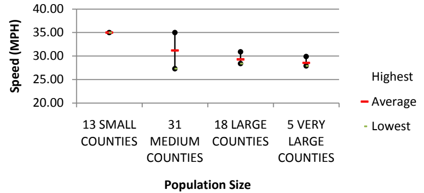
Urban Arterial Street Speeds and County Size - 2006 (Aggregate)
