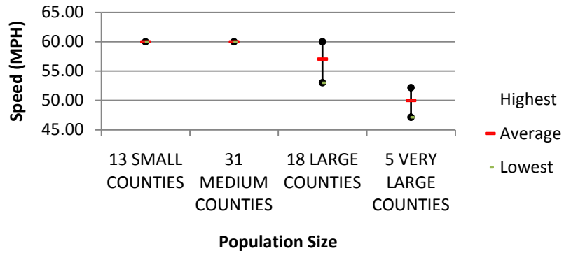
Urban Freeway Speeds and County Size - 2007 (Aggregate)
