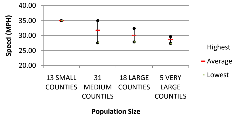
Urban Arterial Street Speeds and County Size - 2004 (Disaggregate County)
