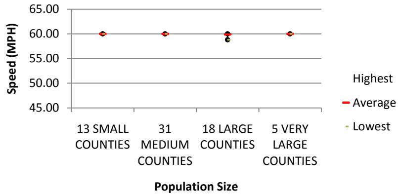
Rural Freeway Speeds and County Size - 2004 (Disaggregate Roadway)
