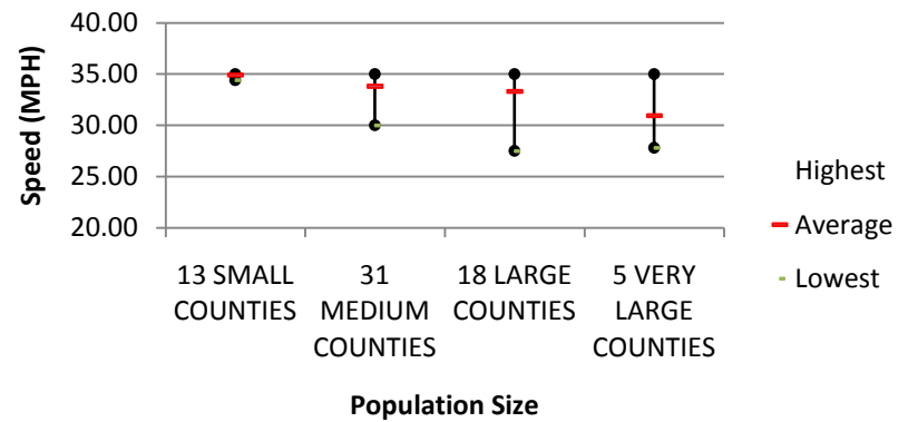
Rural Arterial Street Speeds and County Size - 2004 (Aggregate)
