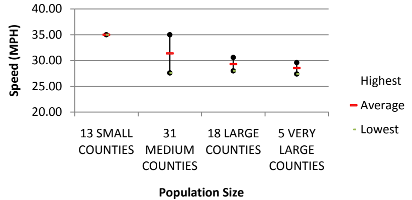
Urban Arterial Street Speeds and County Size - 2004 (Disaggregate Roadway)
