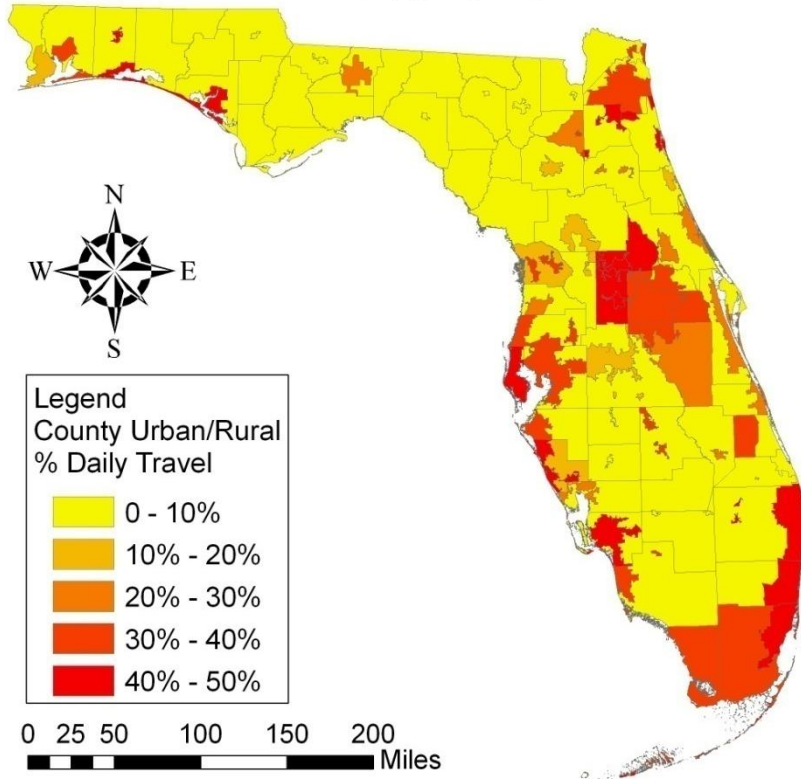
Percent of Daily Travel in Congested Condition - 2005 (Aggregate)
