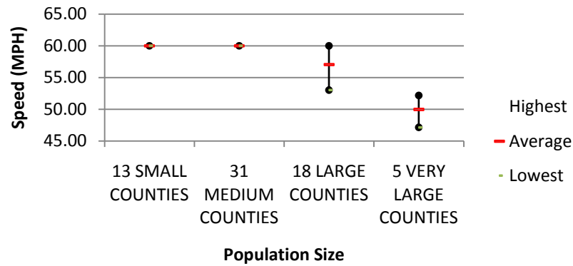
Urban Freeway Speeds and County Size - 2007 (Disaggregate Roadway)
