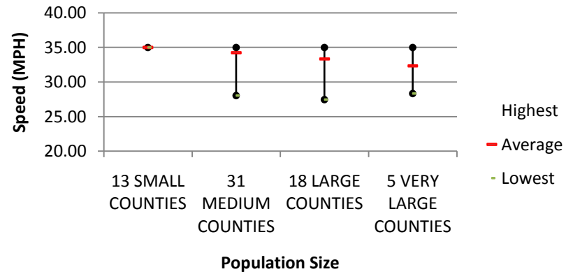
Rural Arterial Street Speeds and County Size - 2006 (Disaggregate County)
